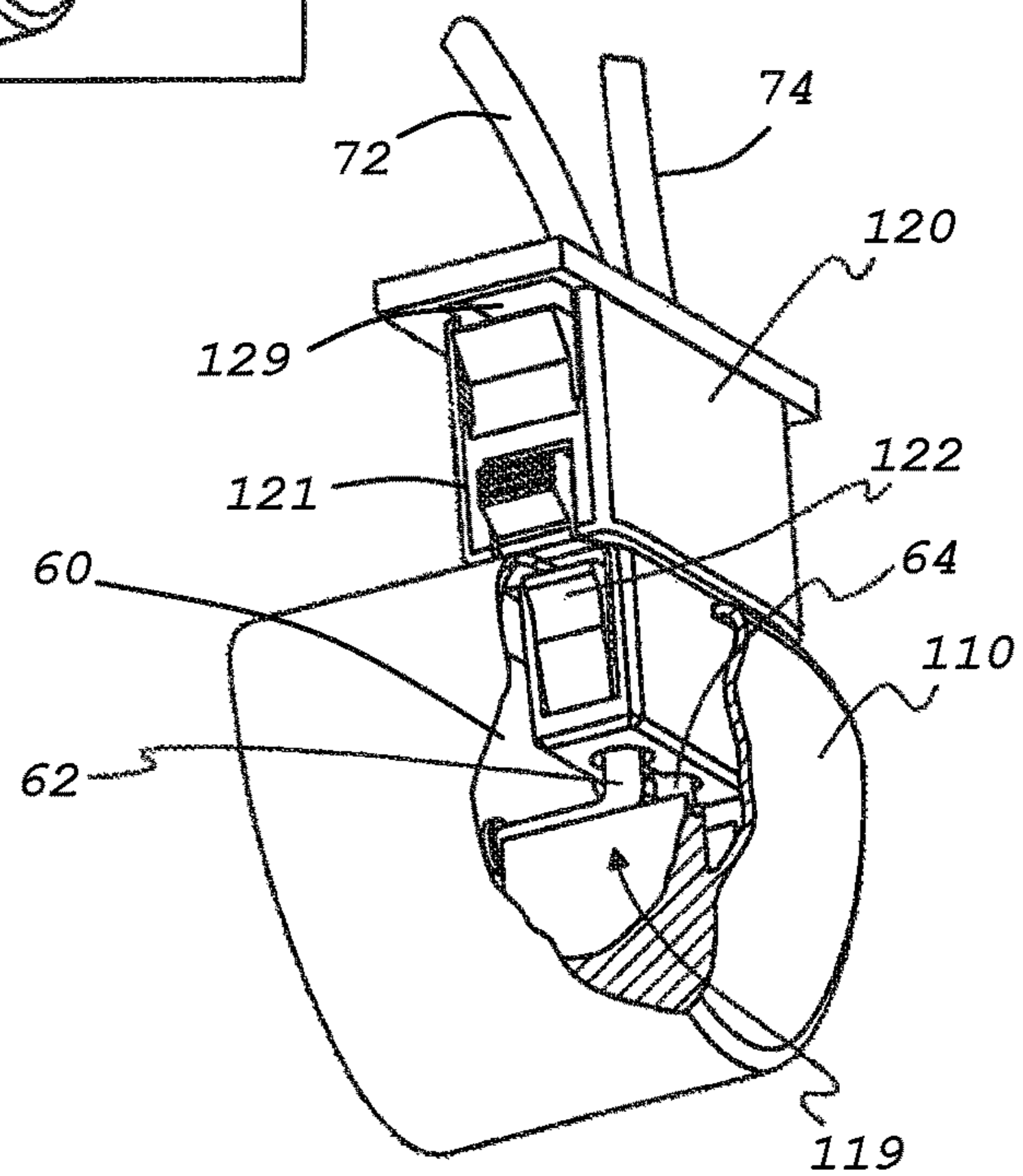
FIG. 7 (Prior Art)
