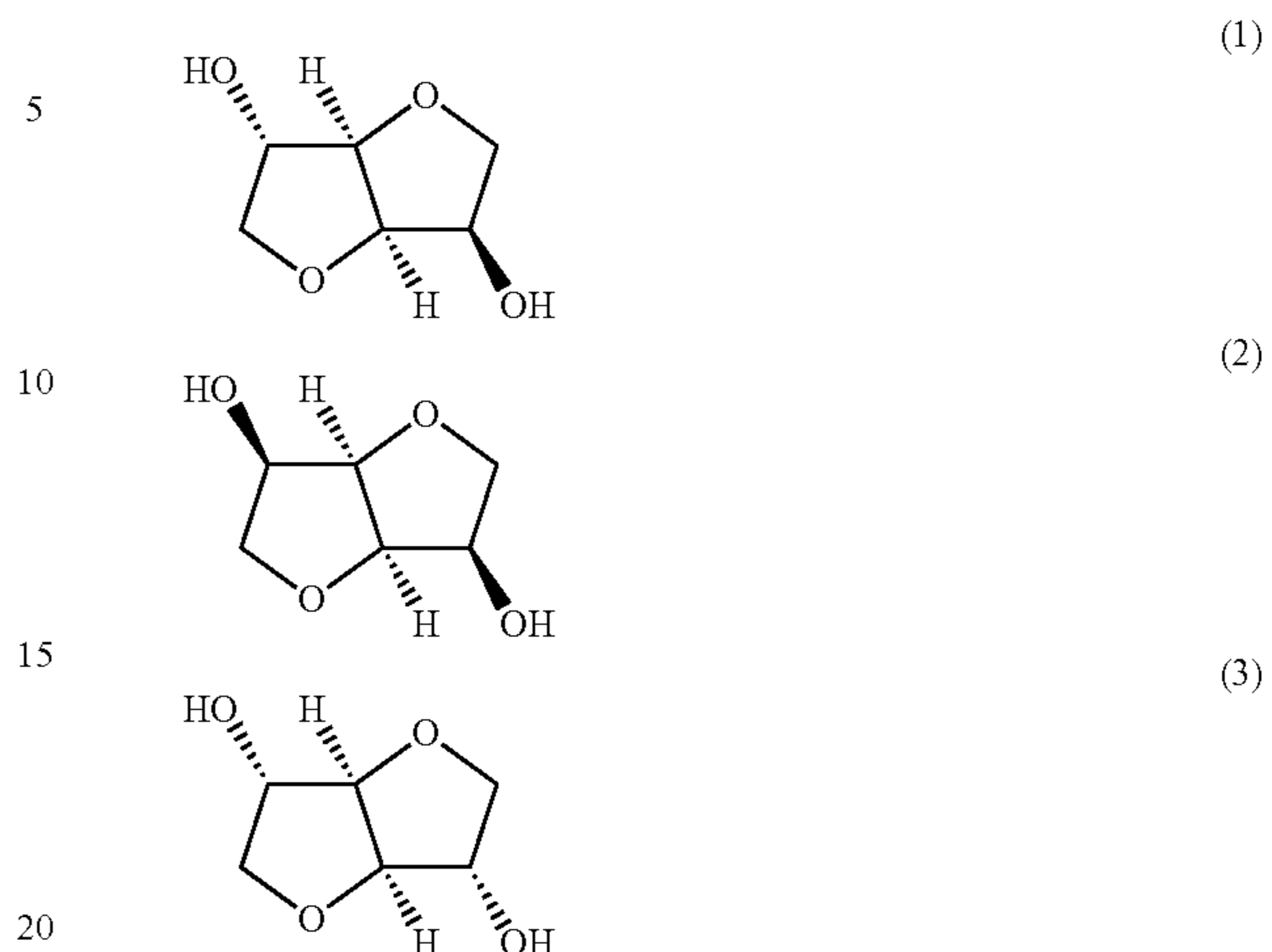
Scheme 1
