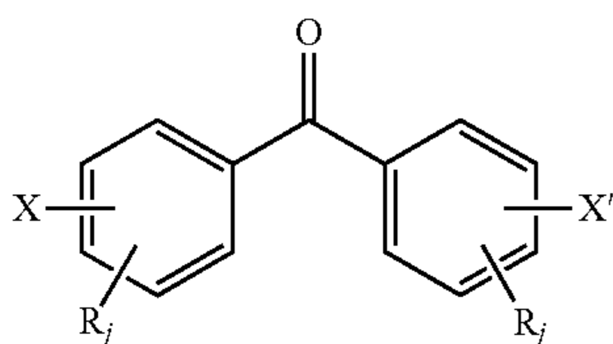
dihalo (B'B')
