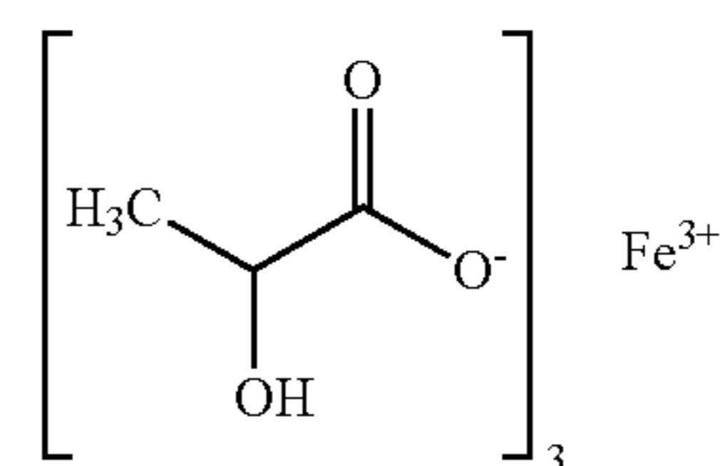
ferric lactate (denoted Fe-Lac)
