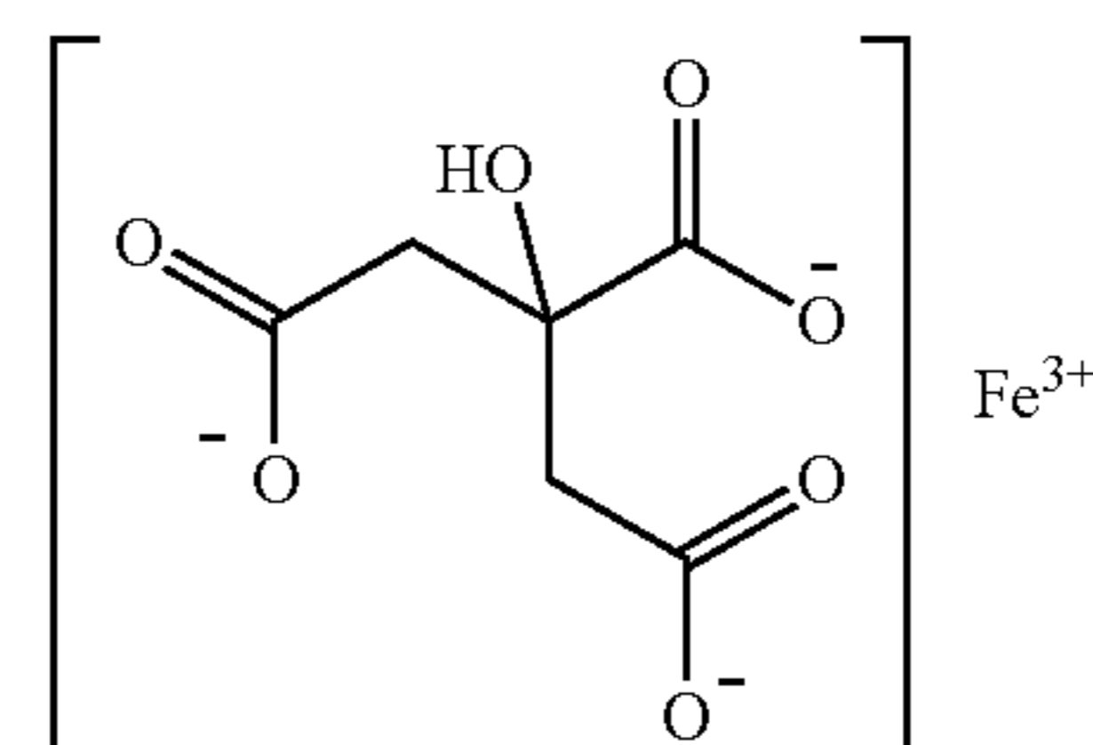
ferric citrate (denoted Fe-Cit)
