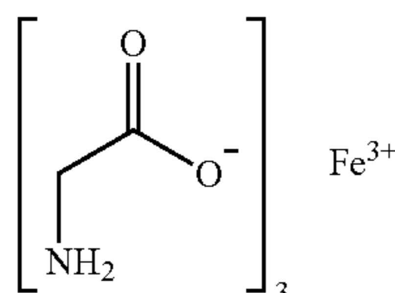
Ferric glycinate (denoted Fe-Gly)
