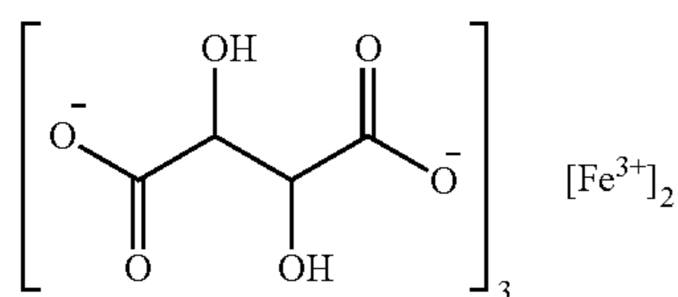
ferric tartrate (denoted Fe-Tart)
