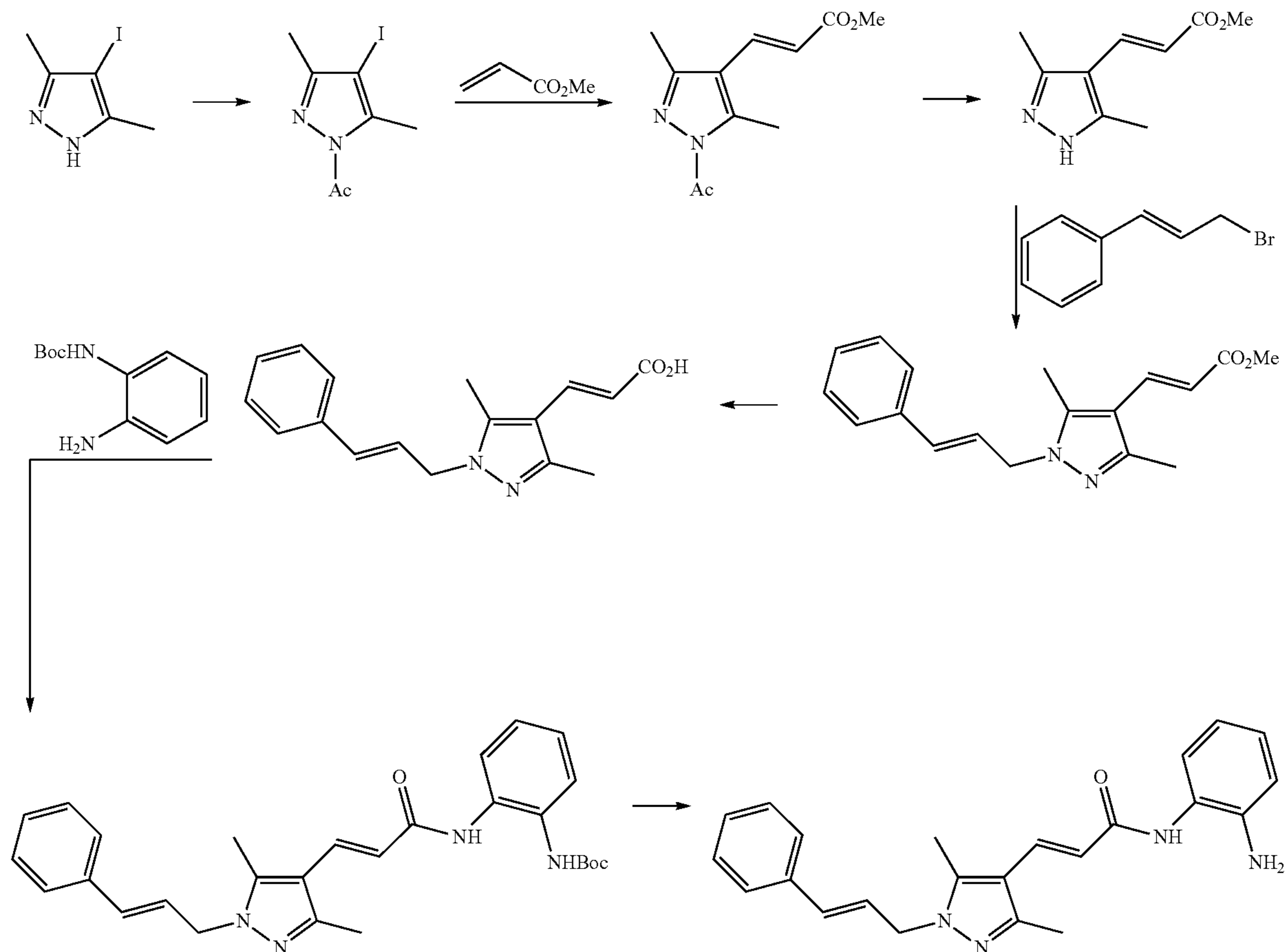
(E)-methyl 3-(3,5-dimethyl-1H-pyrazol-4-yl)acrylate
