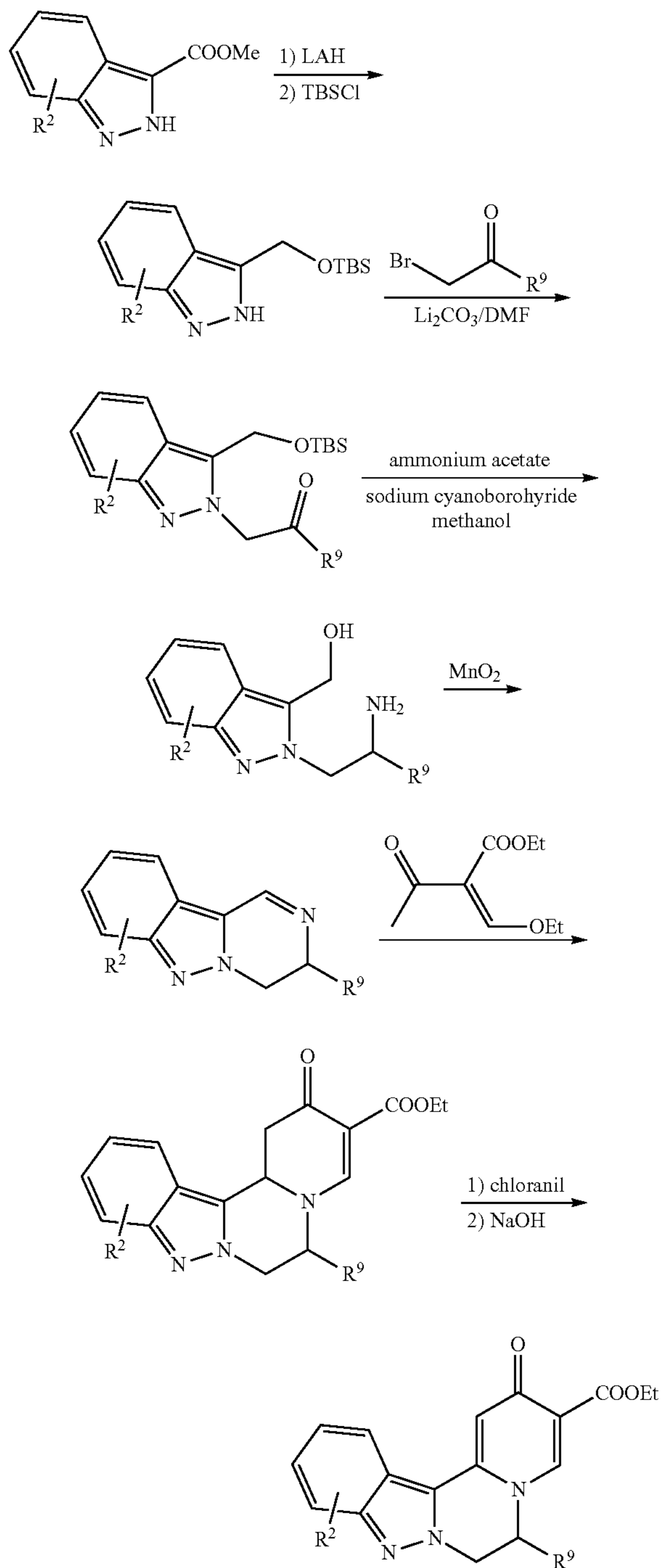
Scheme 1. General method to synthesize compounds of Formula (I).
