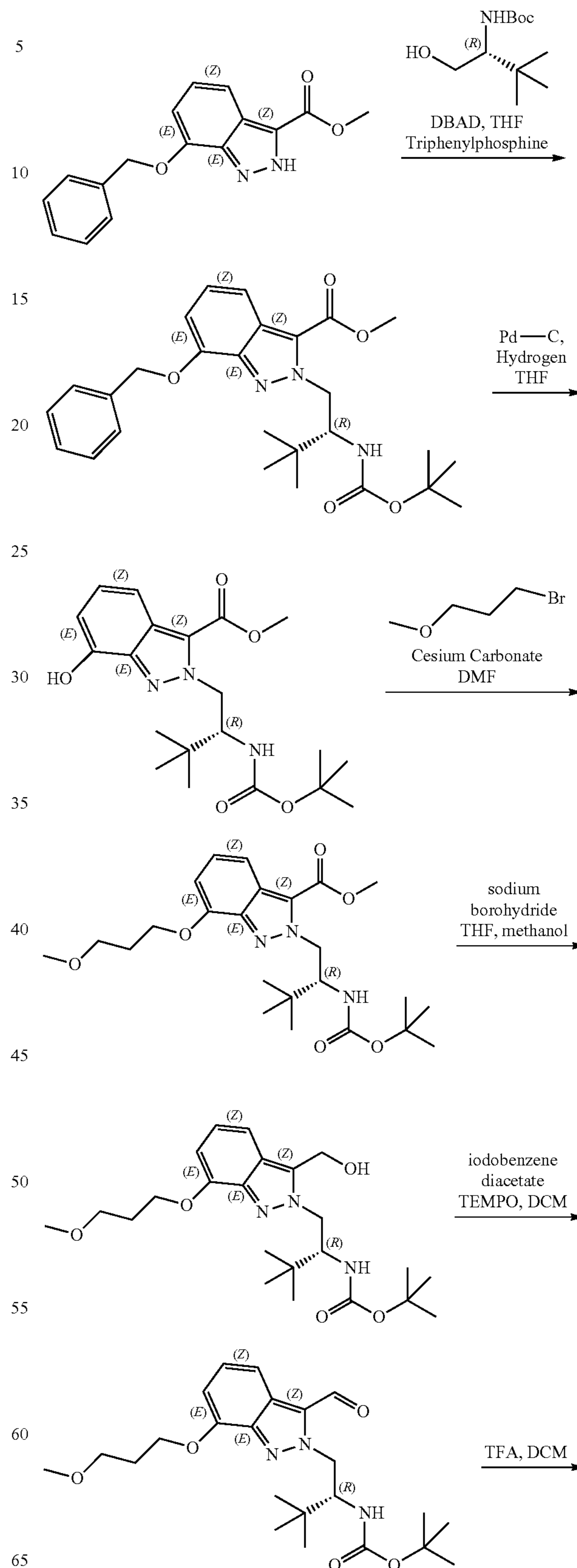
Scheme 2. Stereoselective method to synthesize compound of Formula (II).
