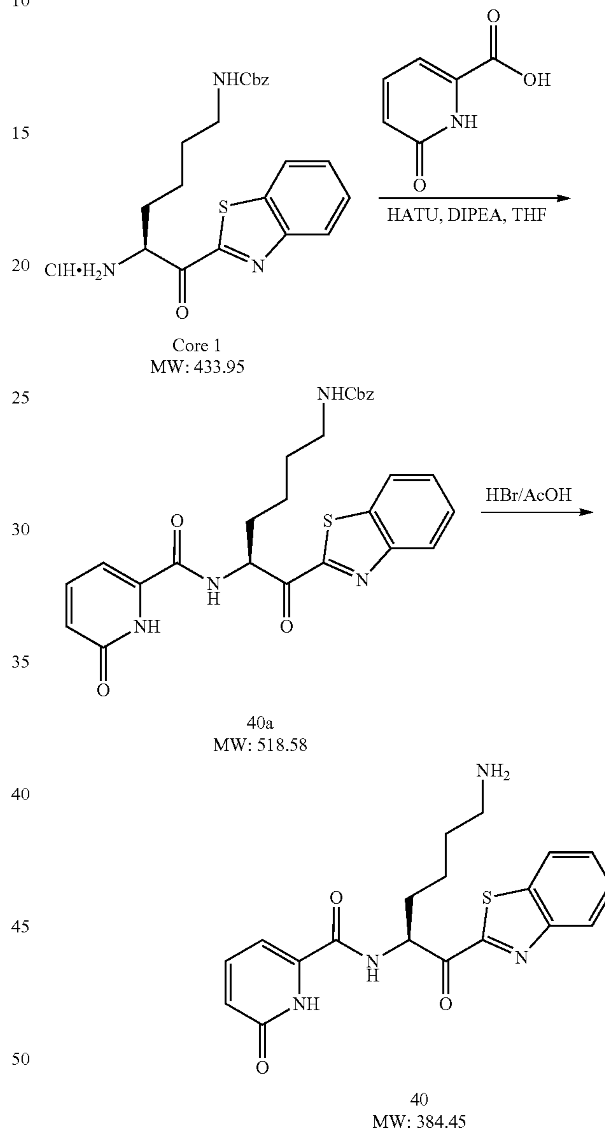
Scheme 31
