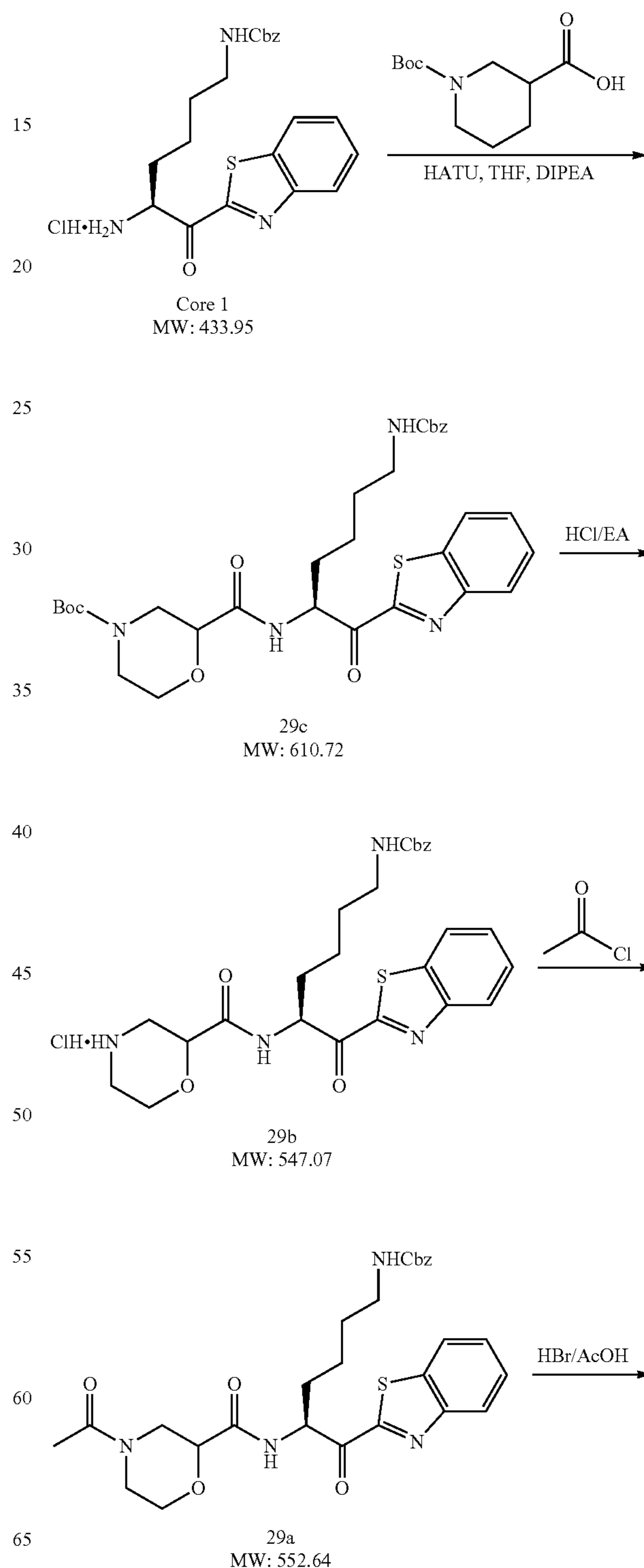
Scheme 23
