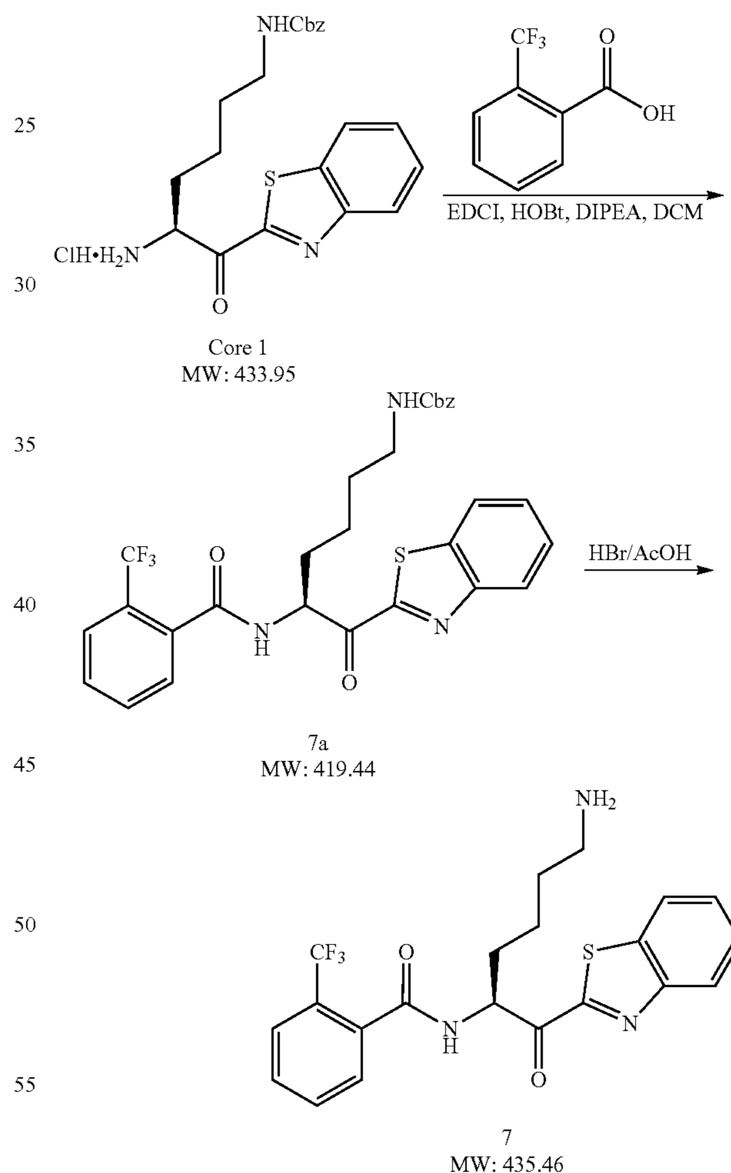
Scheme 12
