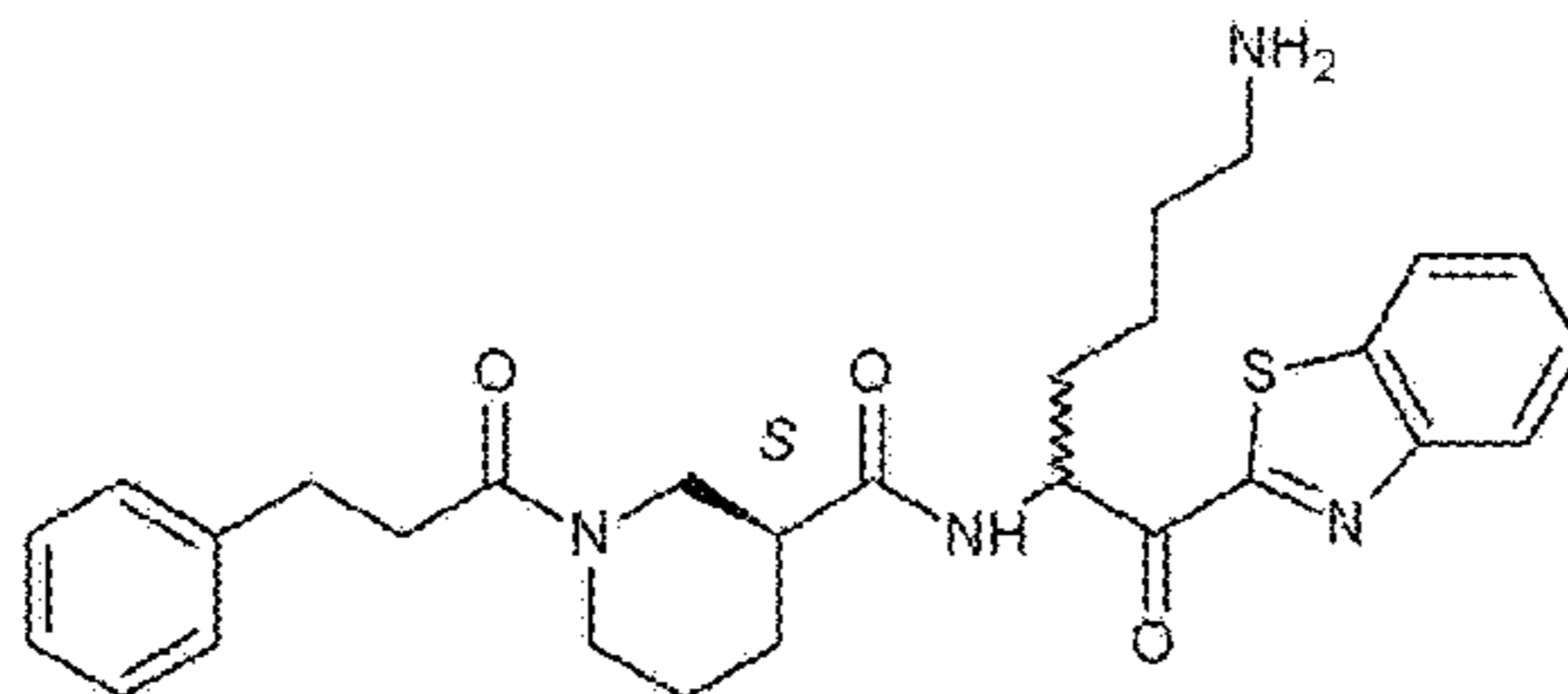
Compound 3
