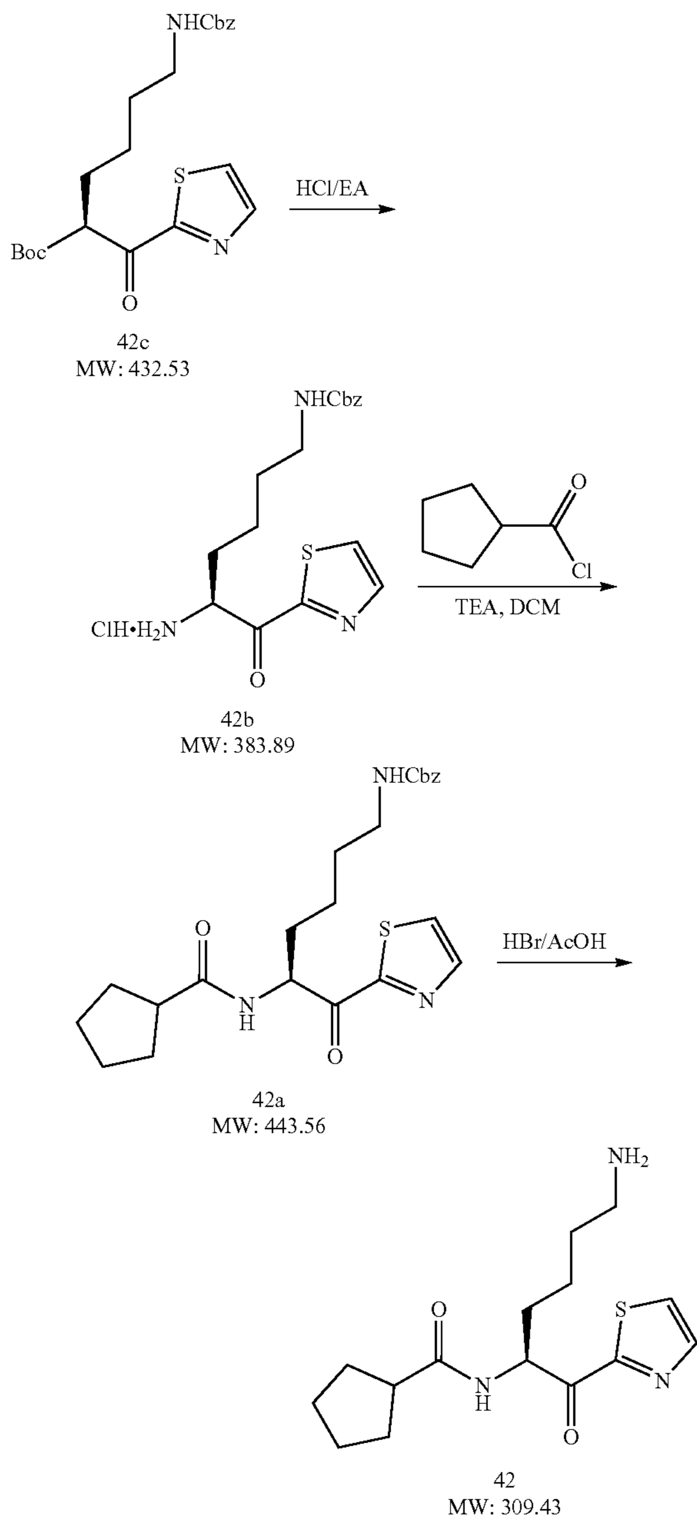
Scheme 33
