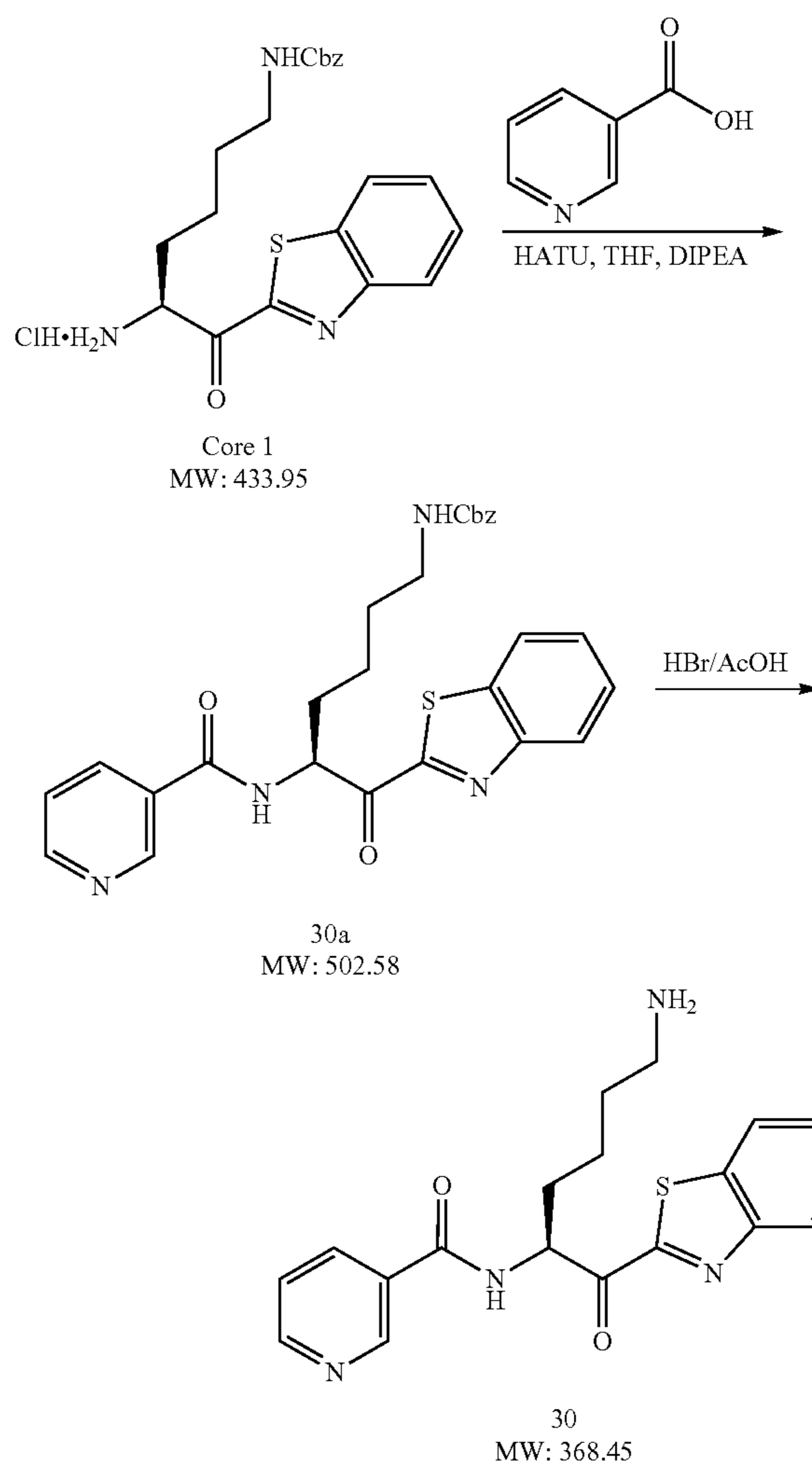
Scheme 24
