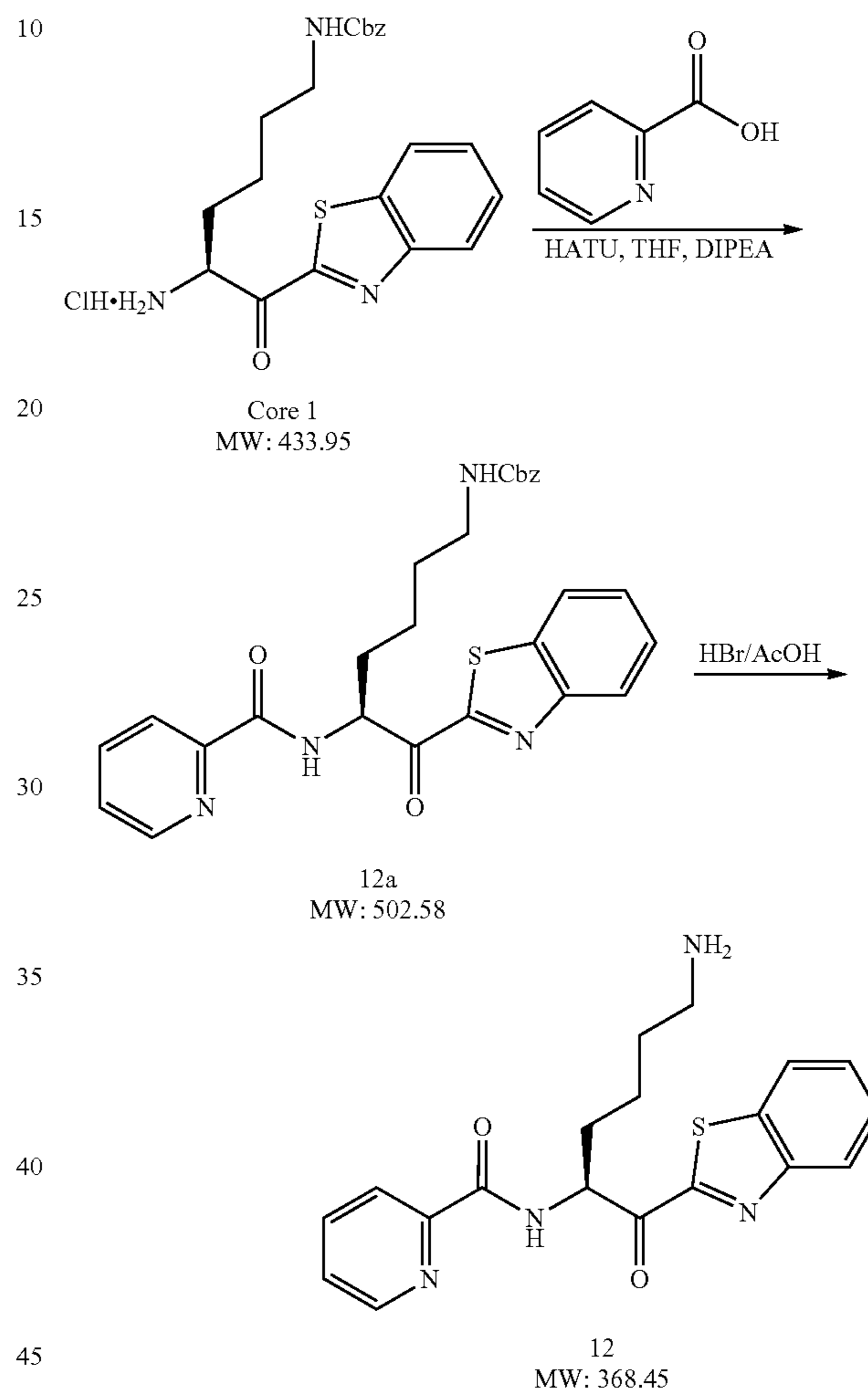
Scheme 15
