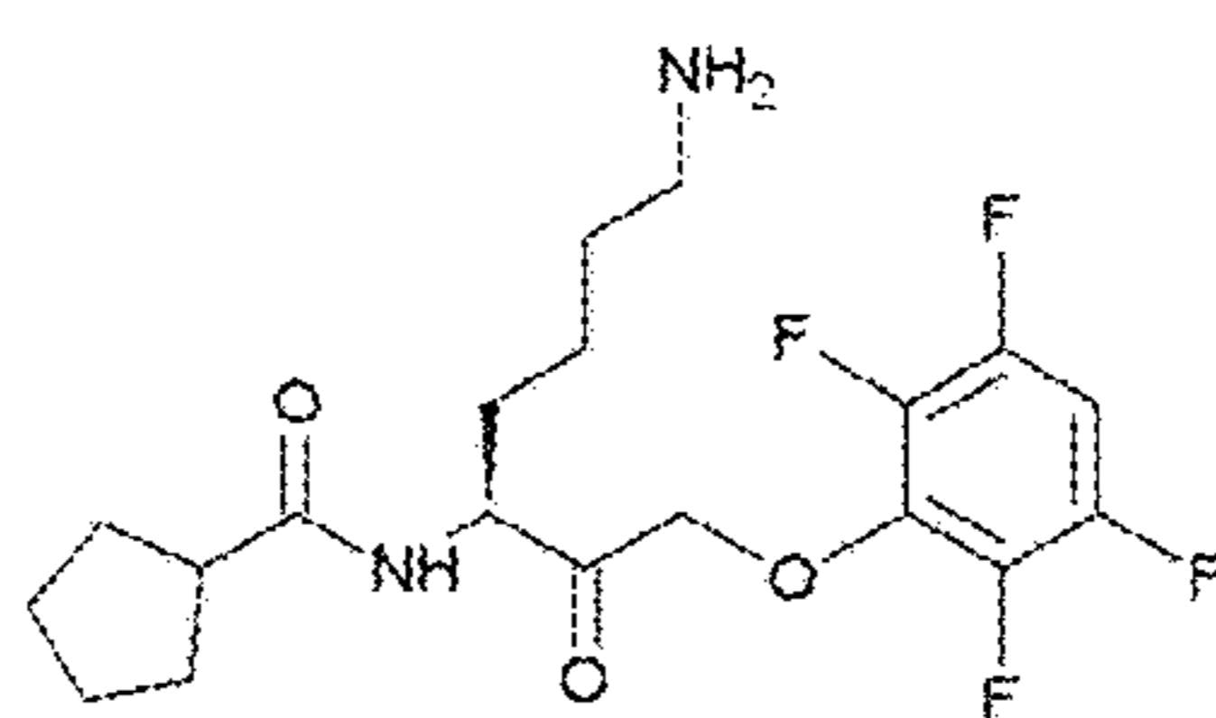
Compound 43
