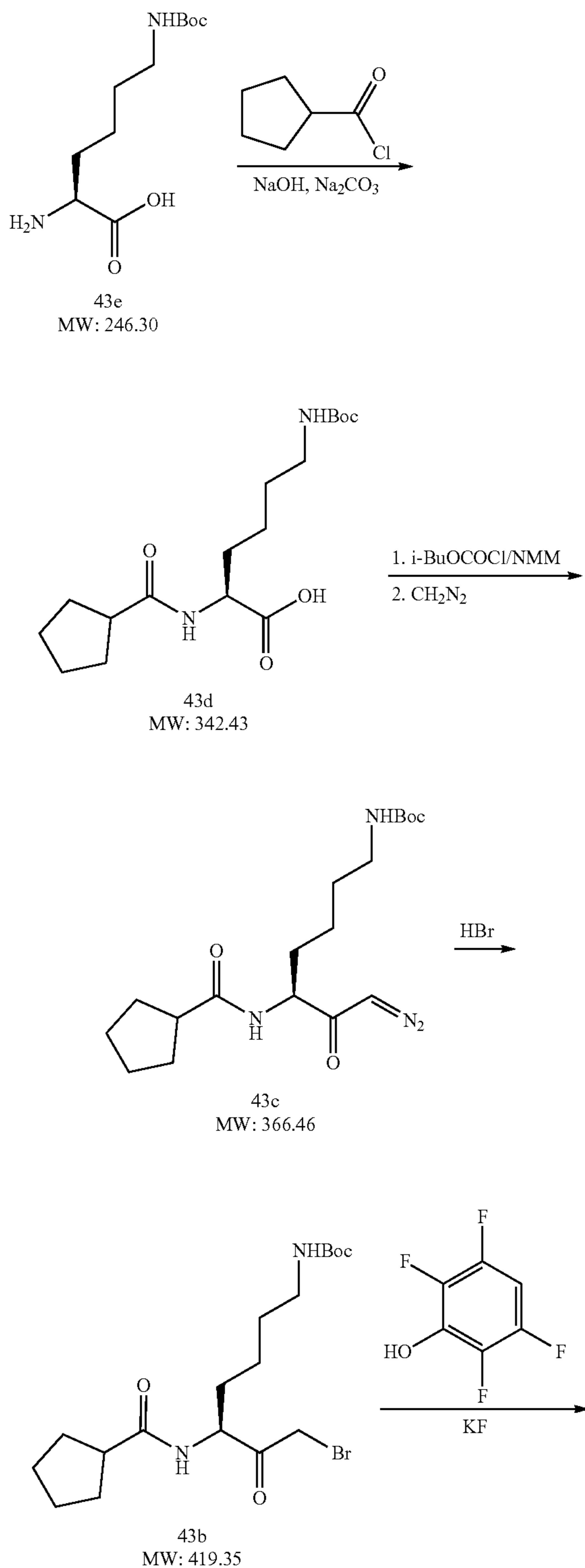
Scheme 34
