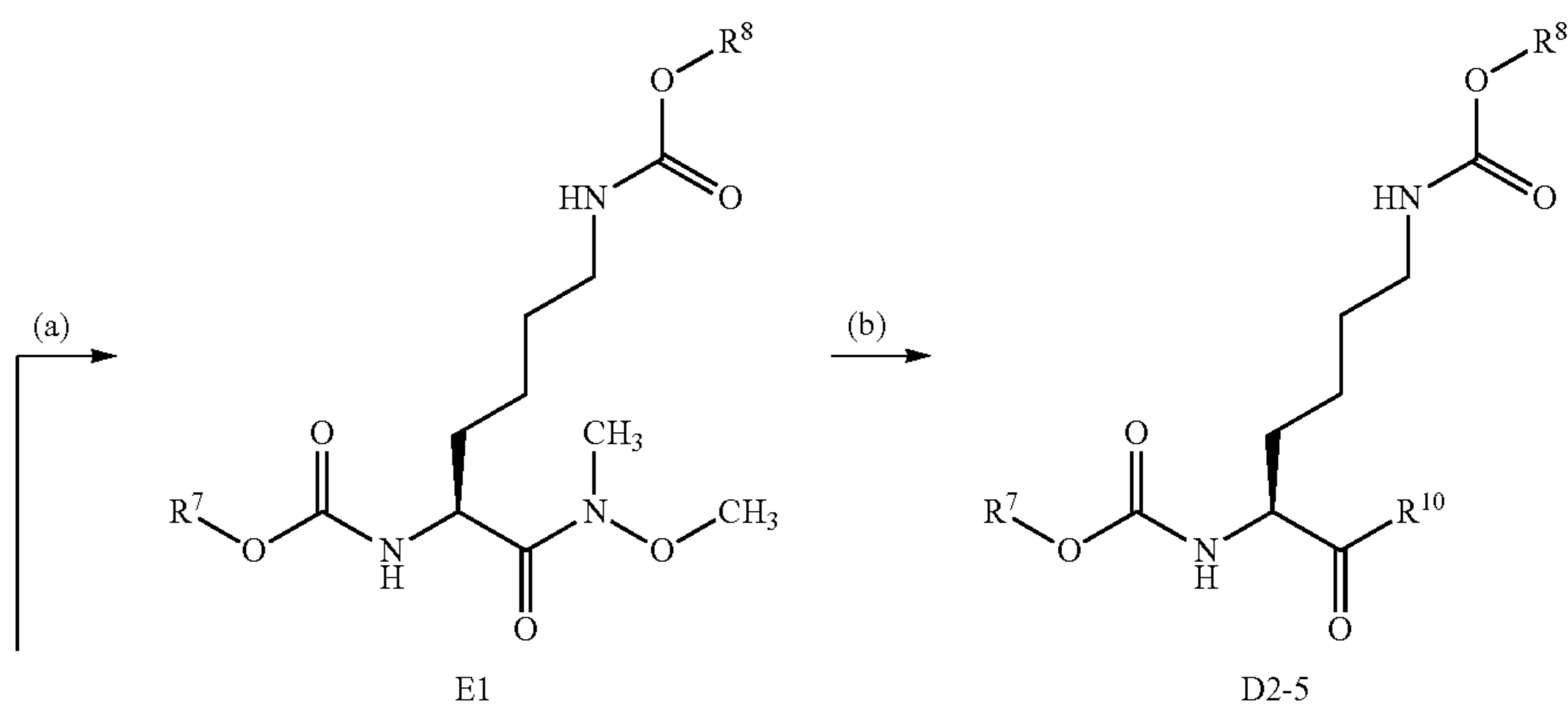
Scheme 2
