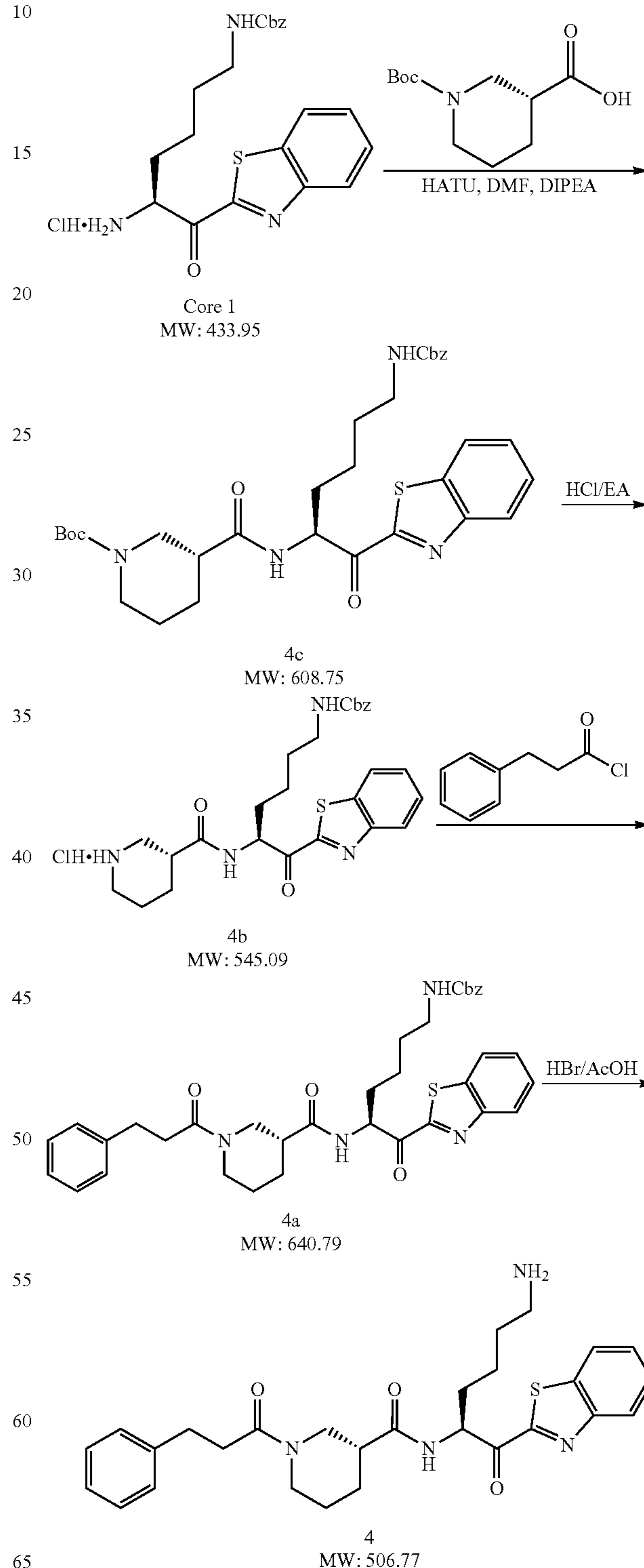
Scheme 11
