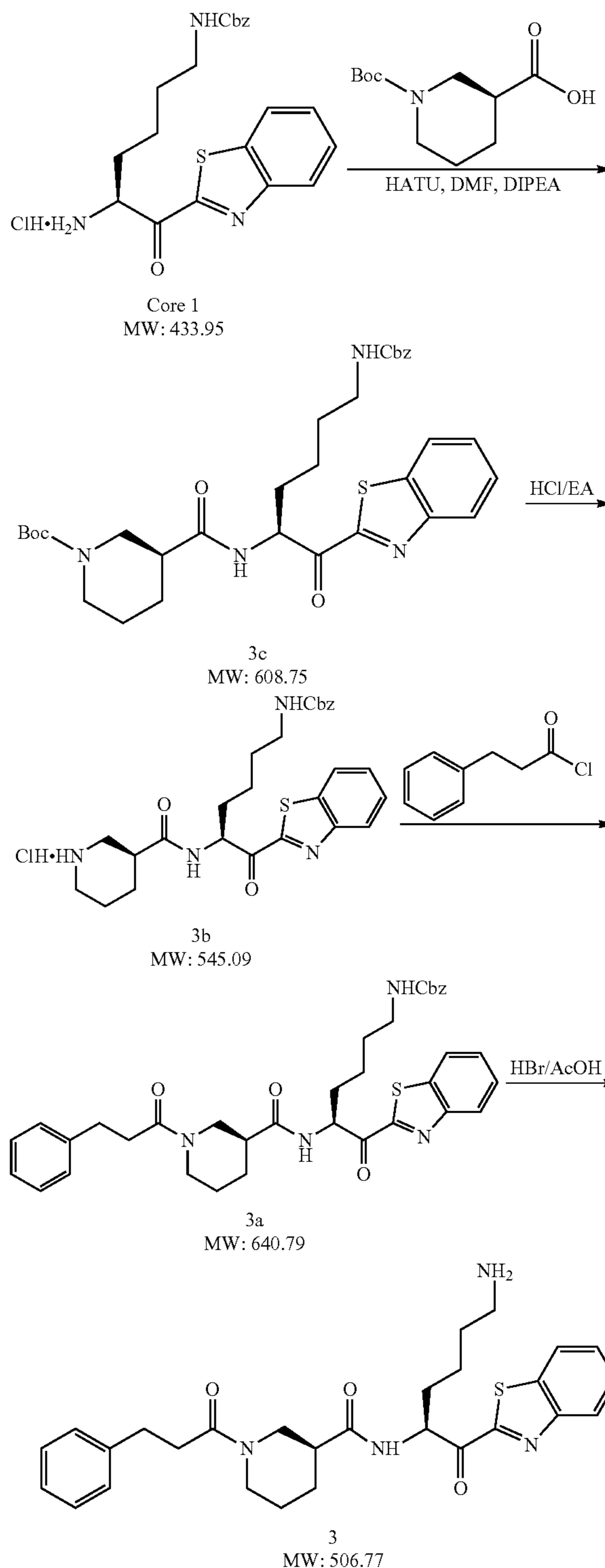
Scheme 10
