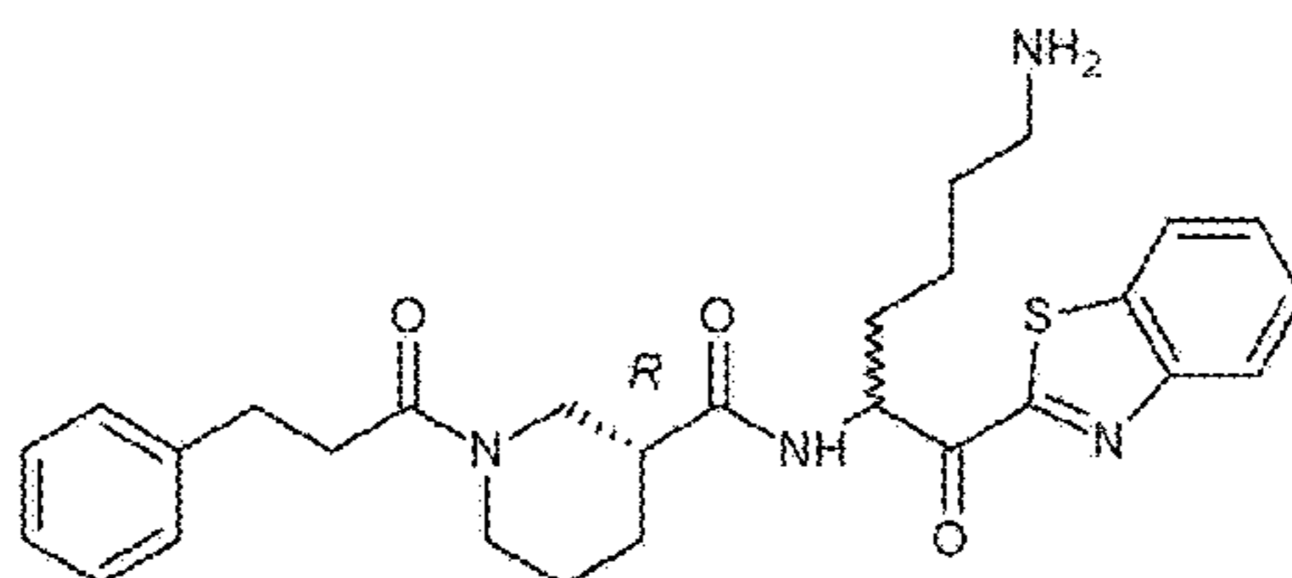
Compound 4
