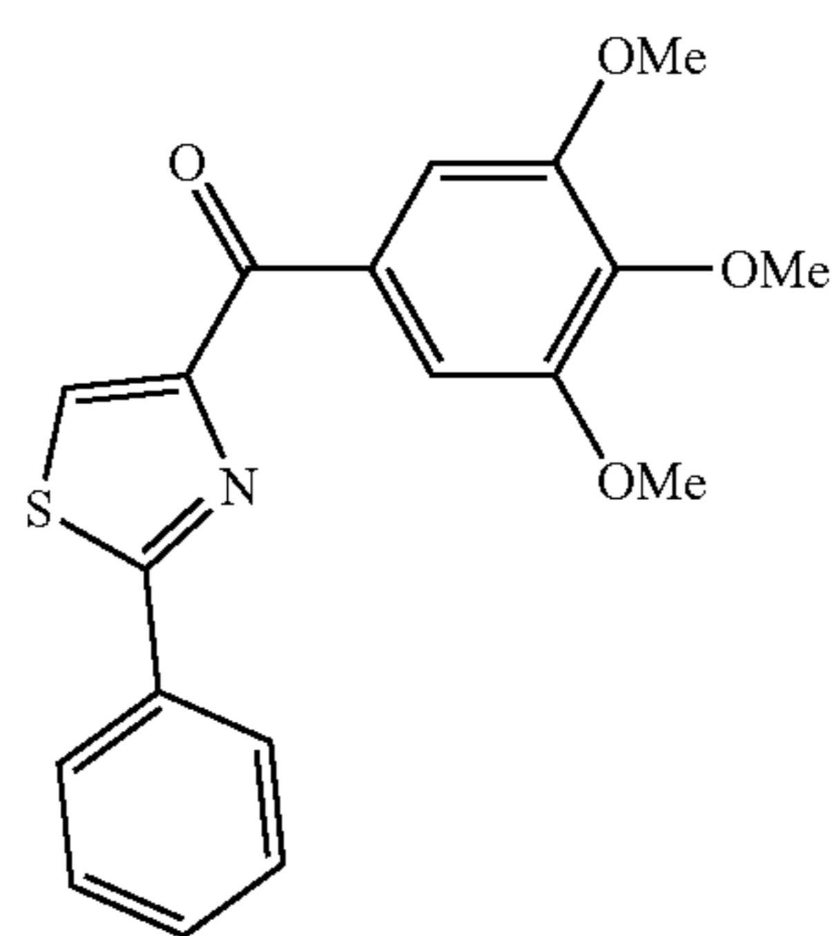
(2-Phenyl-thiazol-4-yl)-(3,4,5-trimethoxy-phenyl)-methanone (1-h)
