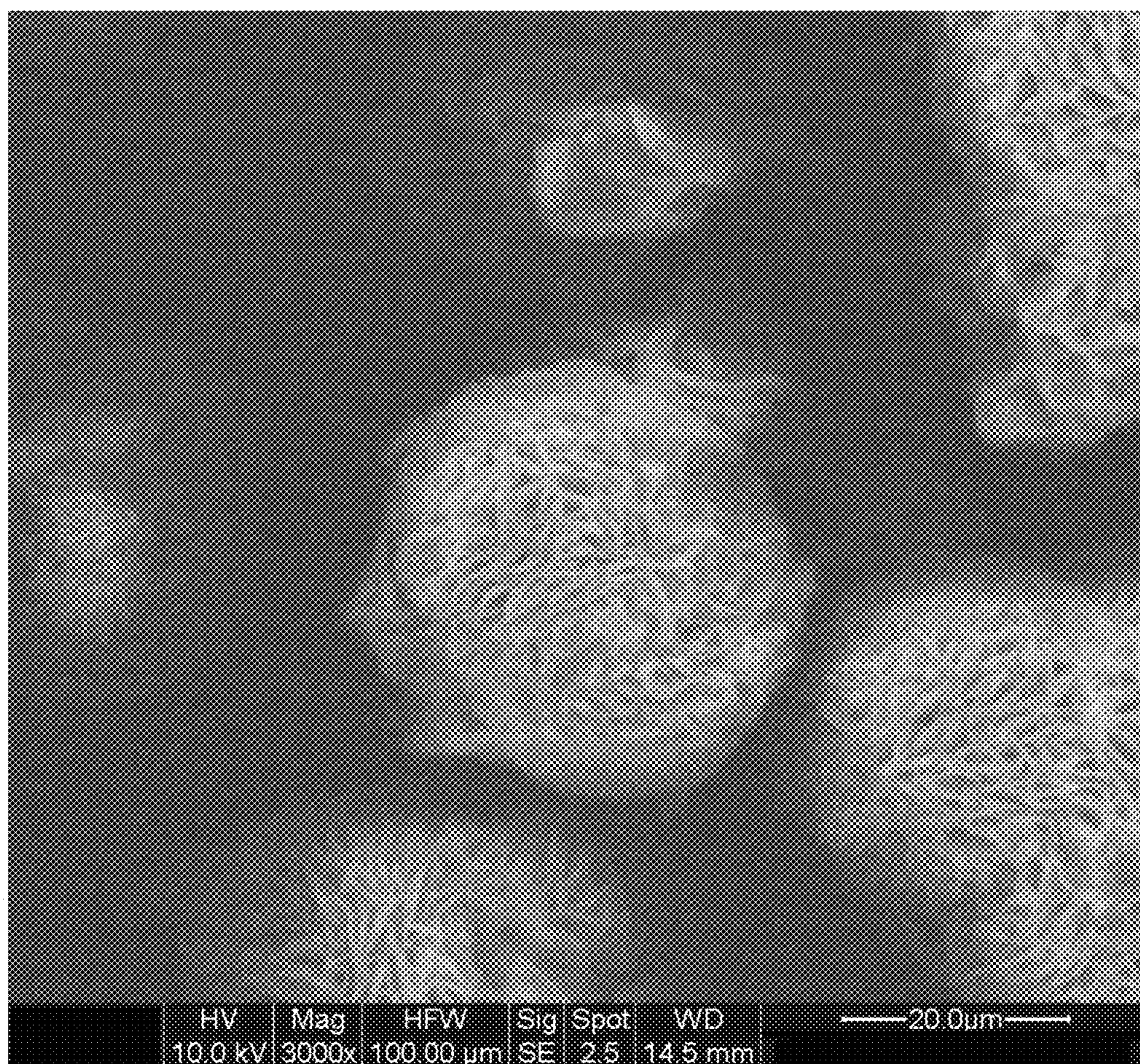
Scanning Electron Micrograph of Spherulites (See Example 1)
