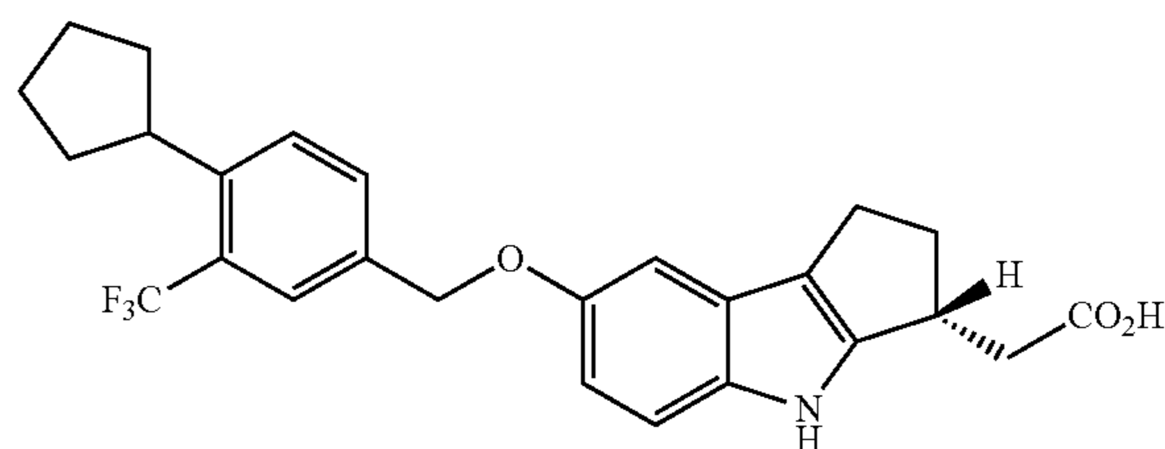
Compound 1
