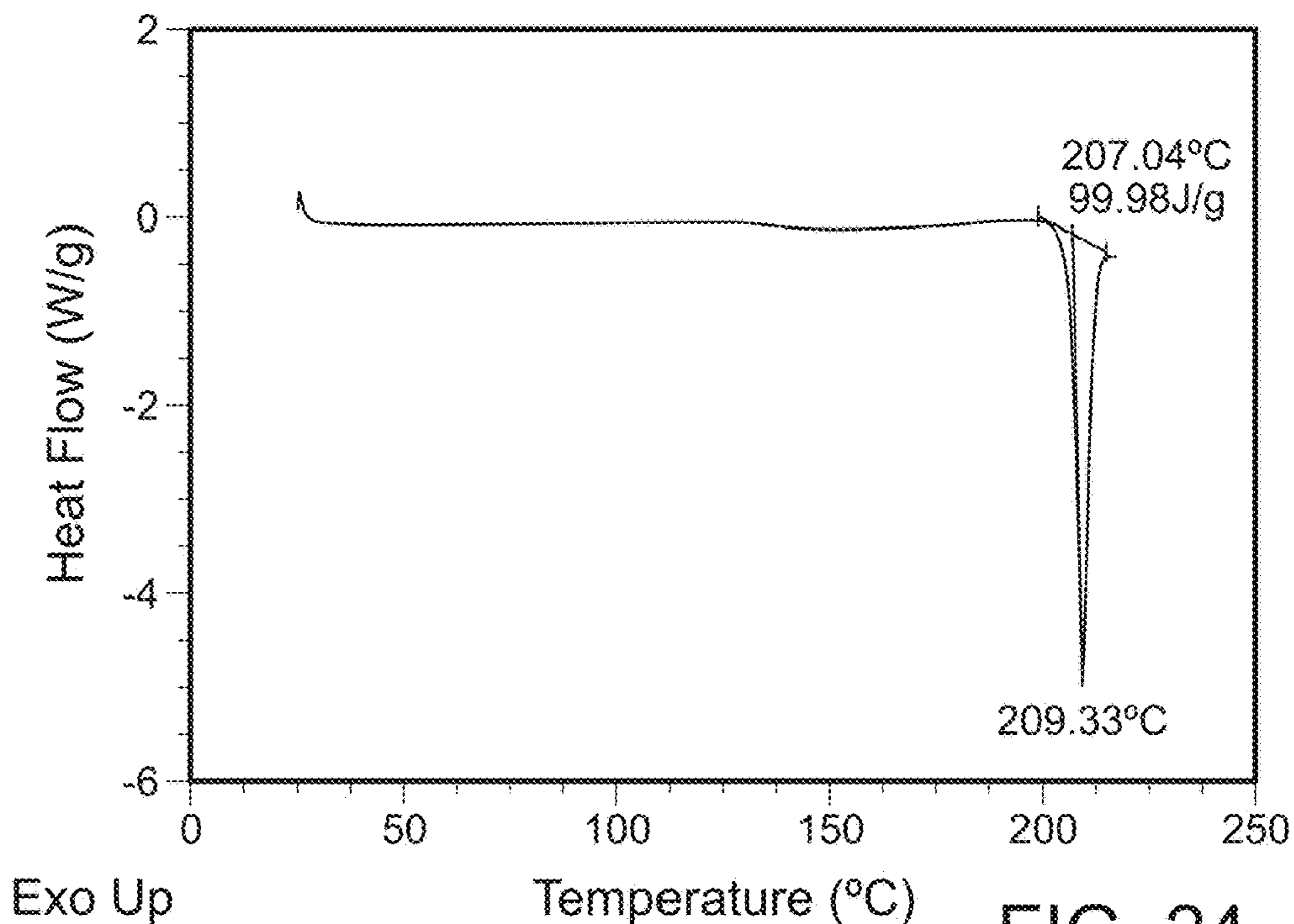
Differential Scanning Calorimetry for Lot A8 (Plates)
