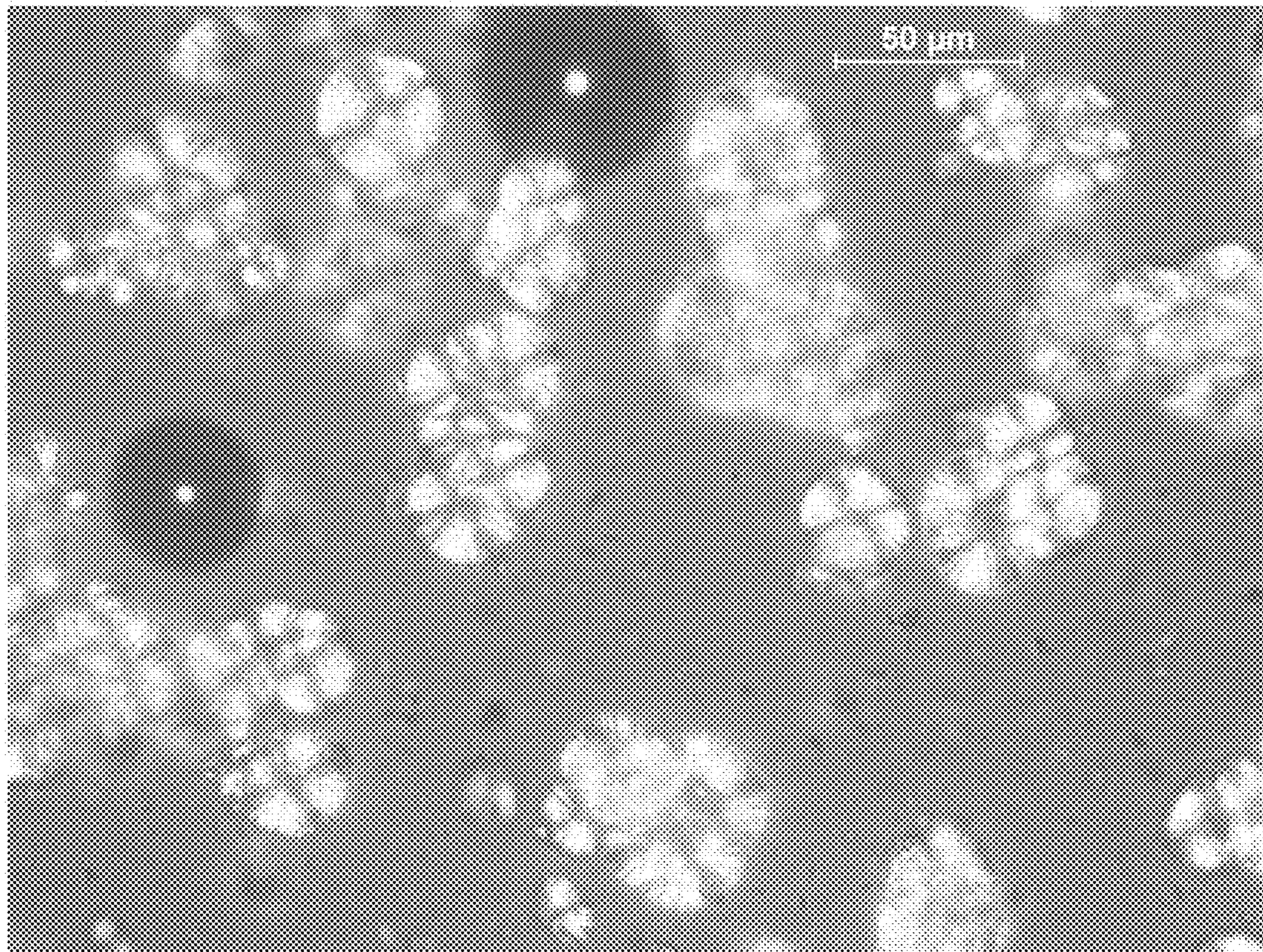
Polarized Light Micrograph of Spherulites (See Example 1)
