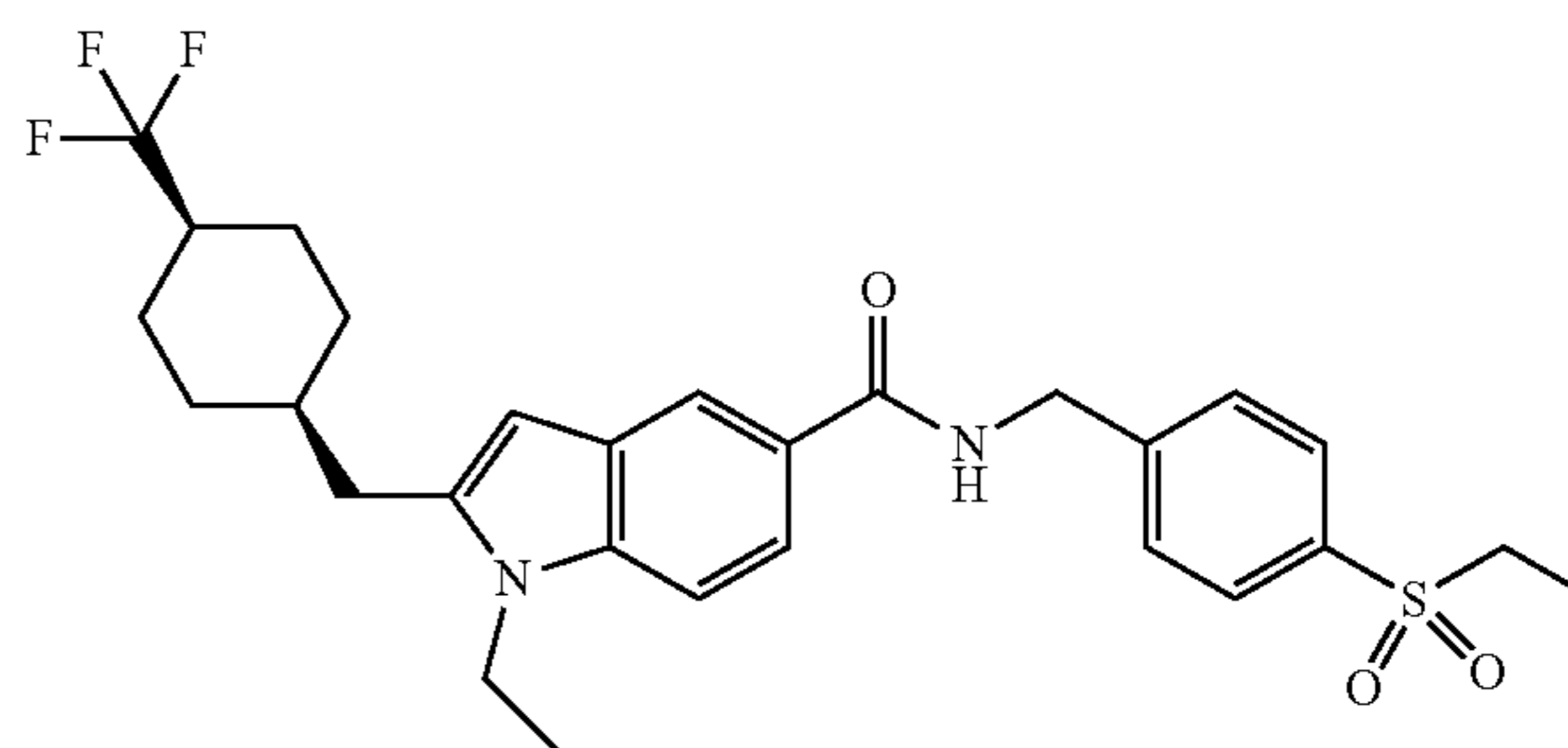
Compounds IN-17.1 and IN-17.2
