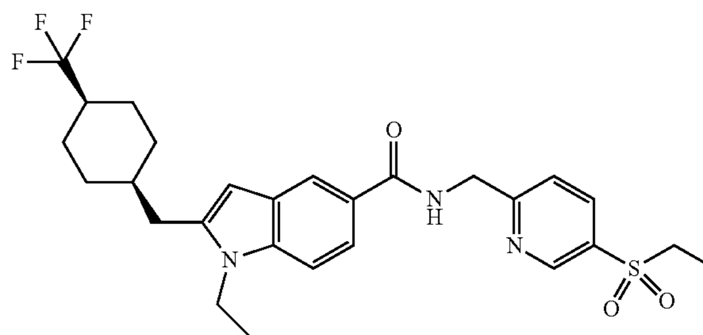
Compounds IN-15.1 and IN-15.2
