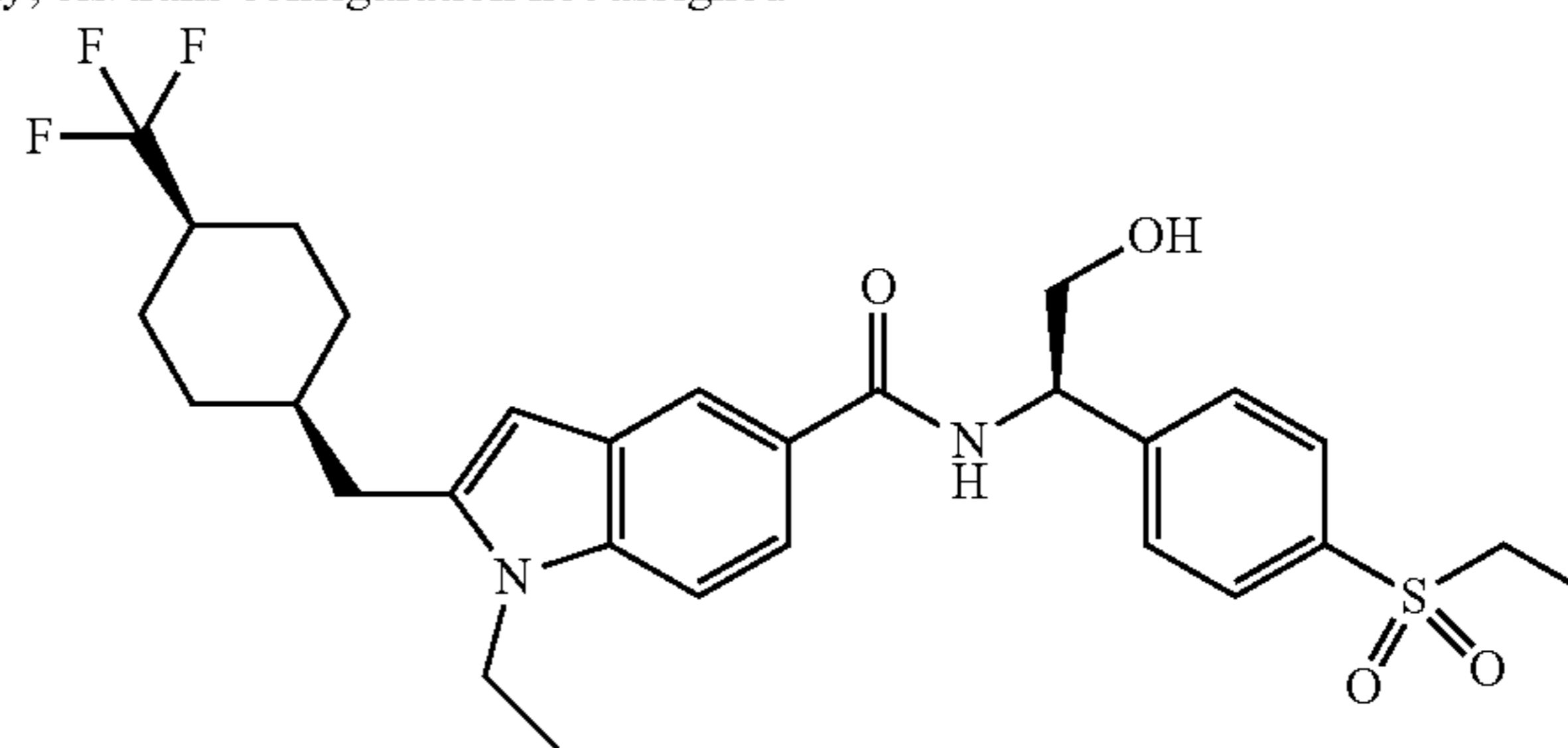
Compounds IN-16.1 and IN-16.2
