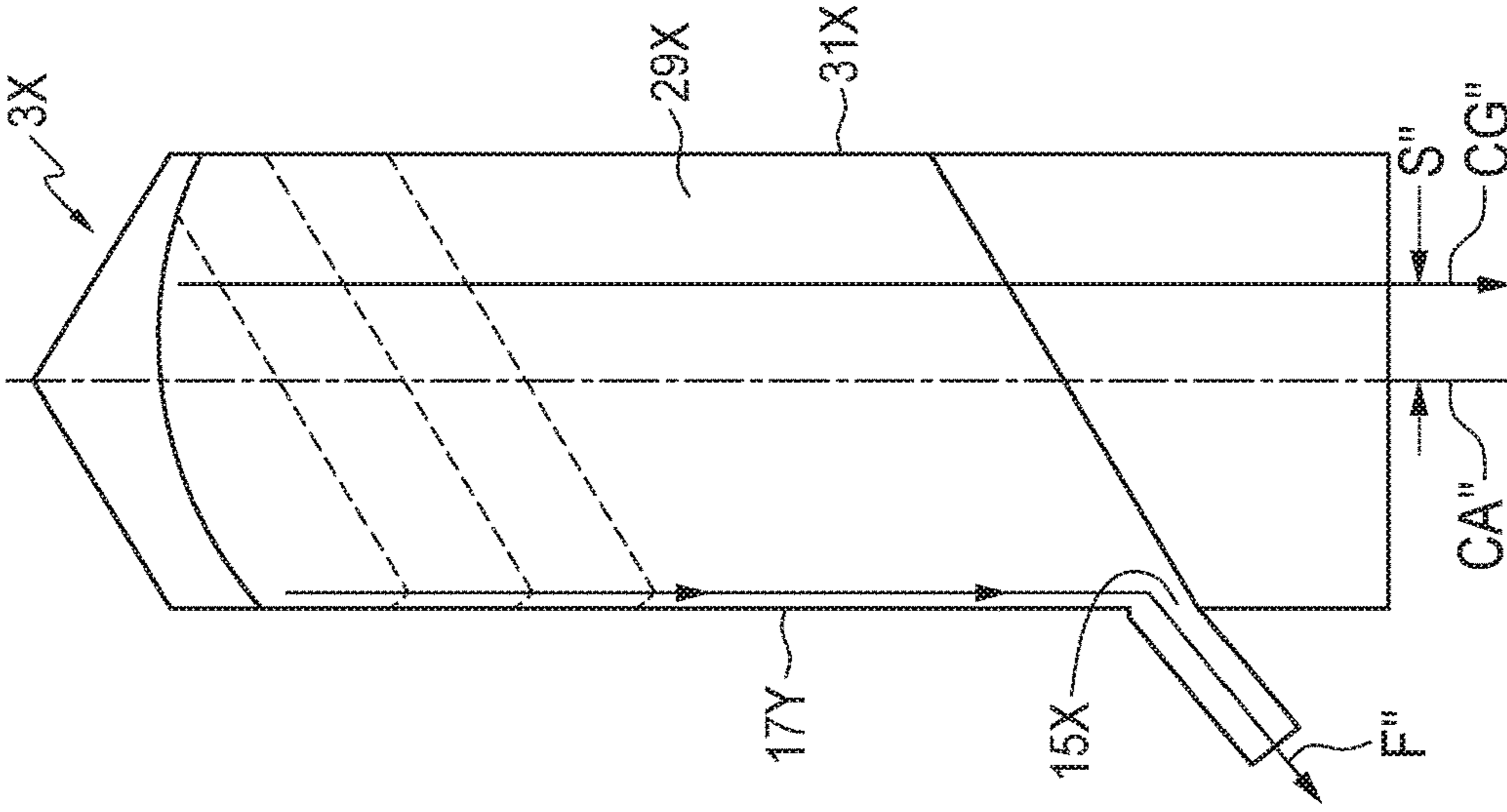
FIG. 4 (PRIOR ART)
