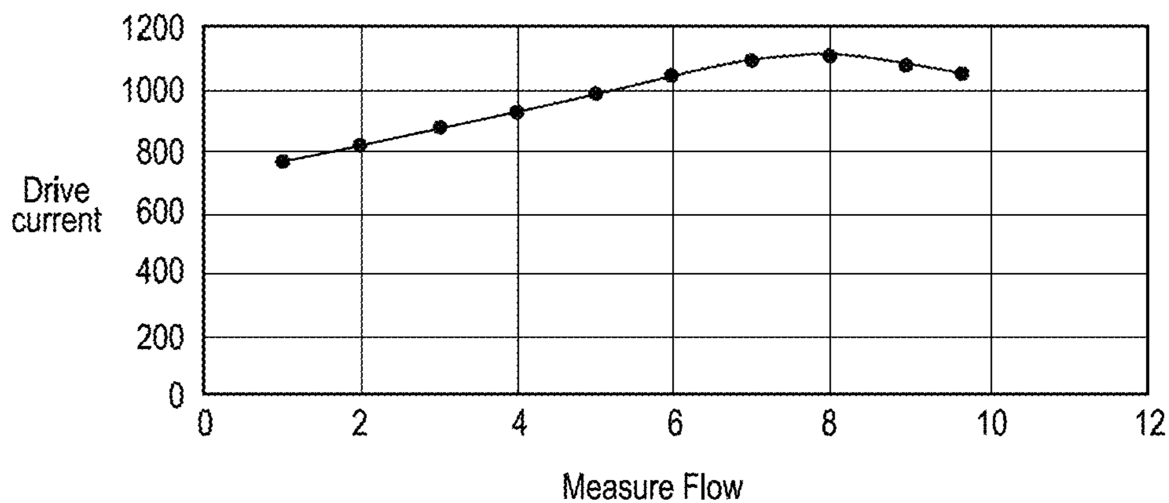
Driving Current
