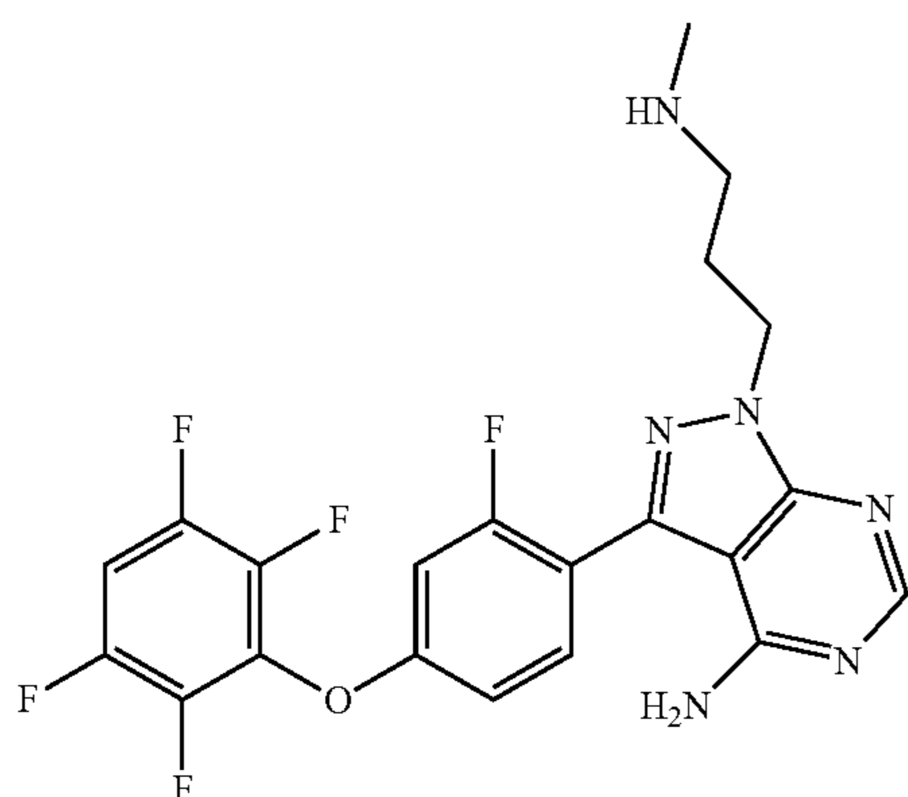
3-(2-fluoro-4-(2,3,5,6-tetrafluorophenoxy)phenyl)-1-(3-(methylamino)propyl)-1H-pyrazolo[3,4-d]pyrimidin-4-amine
