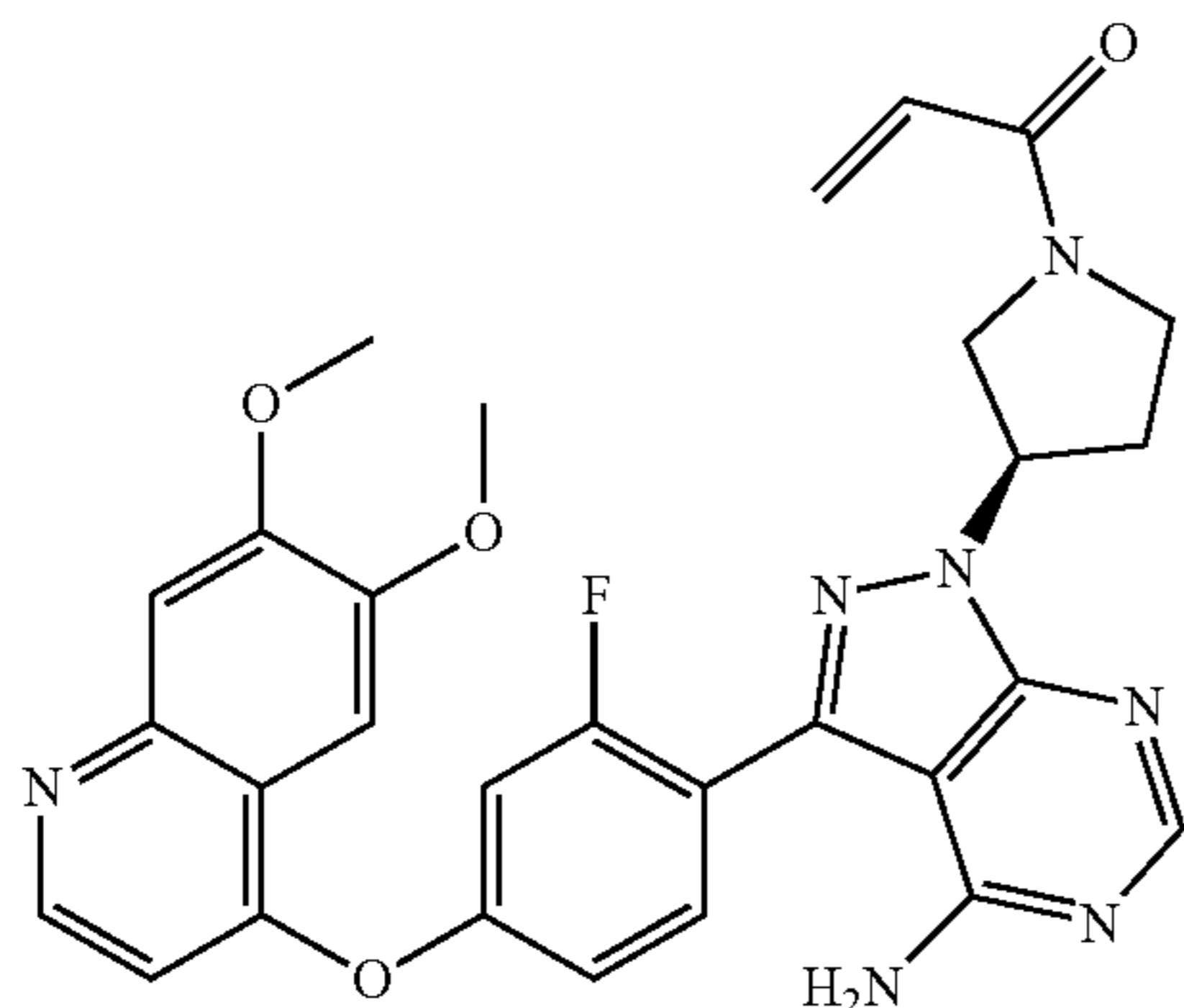
1-((R)-3-(4-amino-3-(4-(6,7-dimethoxyquinolin-4-yloxy)-2-fluorophenyl)-1H-pyrazolo[3,4-d]pyrimidin-1-yl)pyrrolidin-1-yl)prop-2-en-1-one
