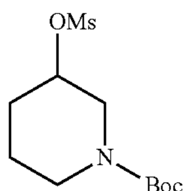
tert-butyl 3-(methylsulfonyloxy)piperidine-1-carboxylate
