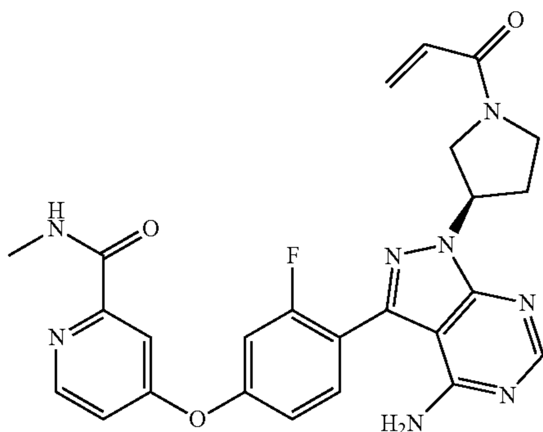
4-(4-(1-((R)-1-acryloylpyrrolidin-3-yl)-4-amino-1H-pyrazolo[3,4-d]pyrimidin-3-yl)-3-fluorophenoxy)-N-methylpicolinamide
