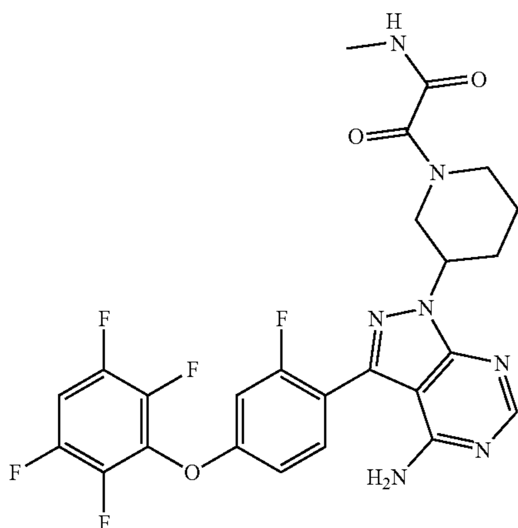
2-(3-(4-amino-3-(2-fluoro-4-(2,3,5,6-tetrafluorophenoxy)phenyl)-1H-pyrazolo[3,4-d]pyrimidin-1-yl)piperidin-1-yl)-N-methyl-2-oxoacetamide
