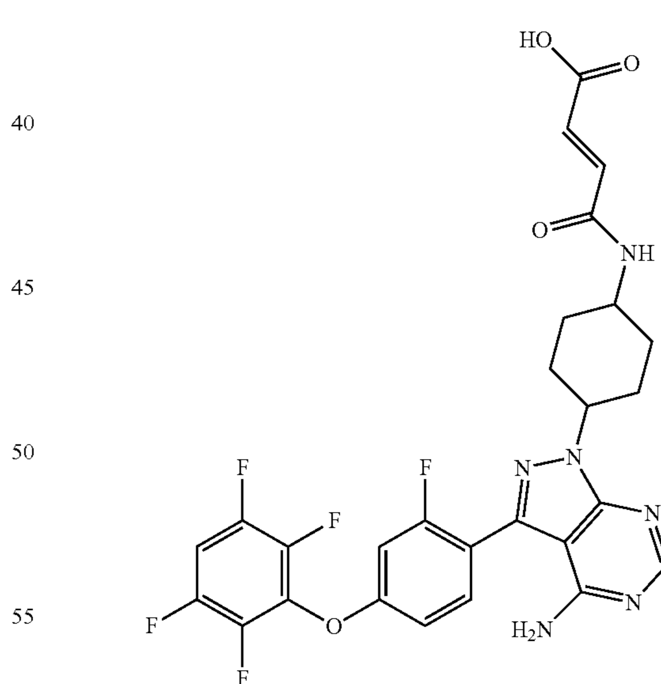
4-(4-(4-amino-3-(2-fluoro-4-(2,3,5,6-tetrafluorophenoxy)phenyl)-1H-pyrazolo[3,4-d]pyrimidin-1-yl)cyclohexylamino)-4-oxobut-2-enoic Acid
