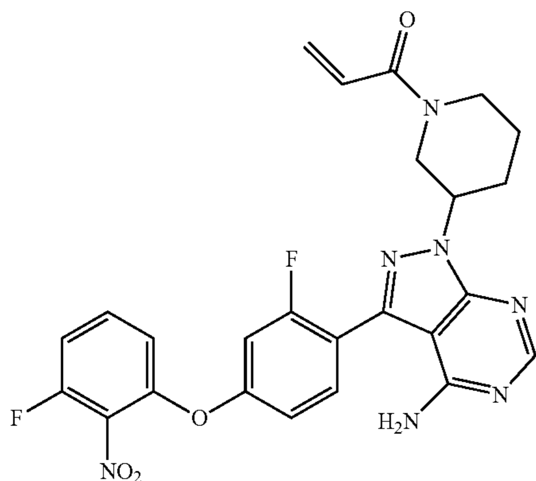
1-(3-(4-amino-3-(2-fluoro-4-(3-fluoro-2-nitro phenoxy)phenyl)-1H-pyrazolo[3,4-d]pyrimidin-1-yl)piperidin-1-yl)prop-2-en-1-one
