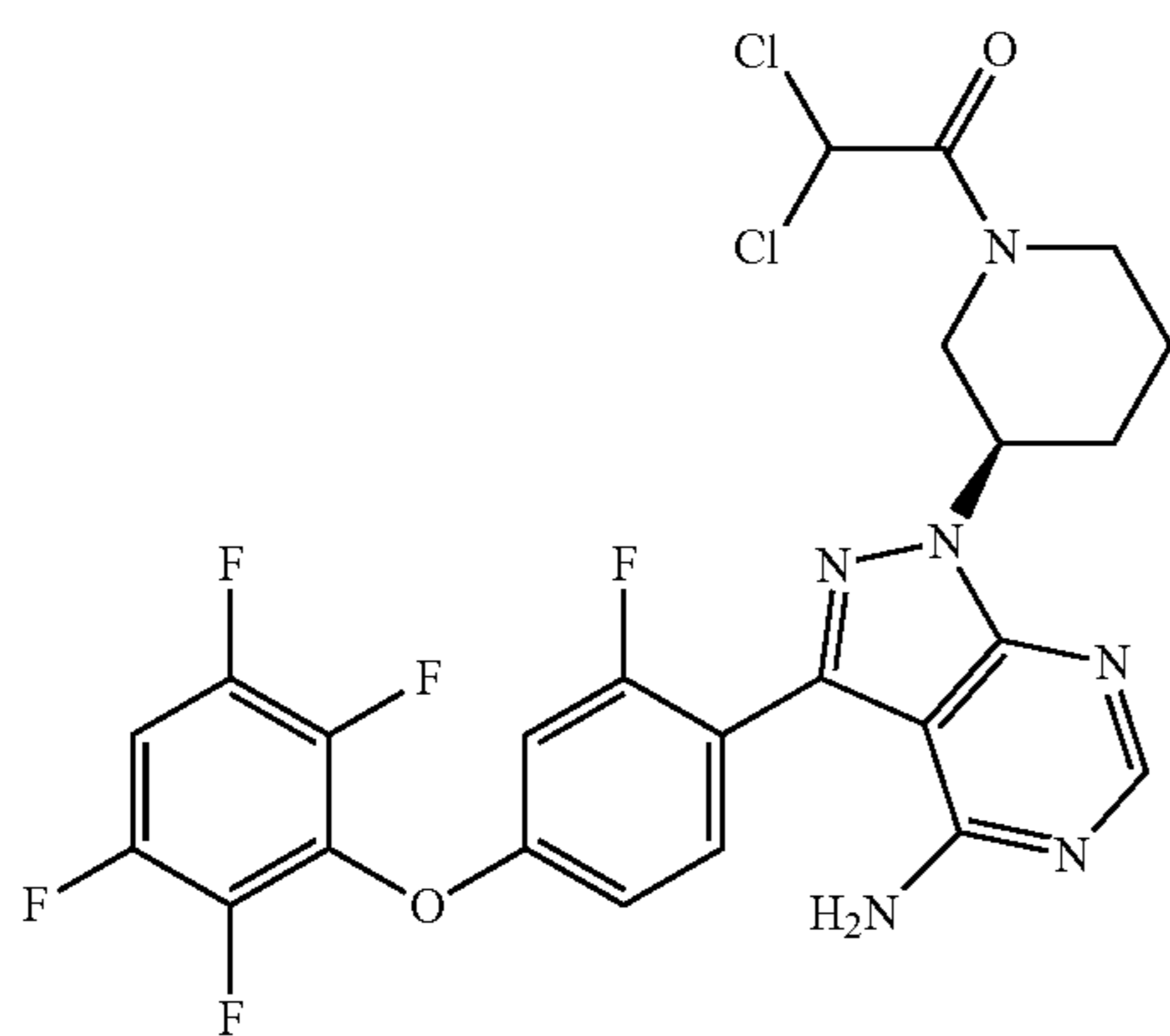
1-((R)-3-(4-amino-3-(2-fluoro-4-(2,3,5,6-tetrafluorophenoxy)phenyl)-1H-pyrazolo[3,4-d]pyrimidin-1-yl)piperidin-1-yl)-2,2-dichloroethanone
