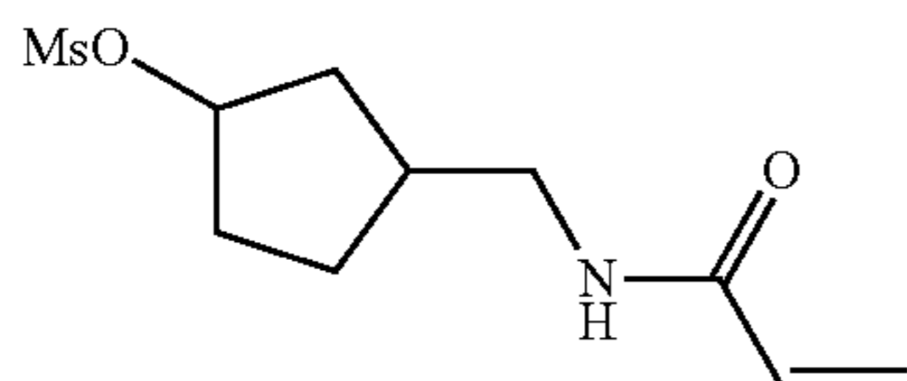
3-(acrylamidomethyl)cyclopentyl methanesulfonate
