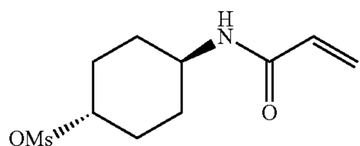
(1r,4r)-4-acrylamidocyclohexyl methanesulfonate
