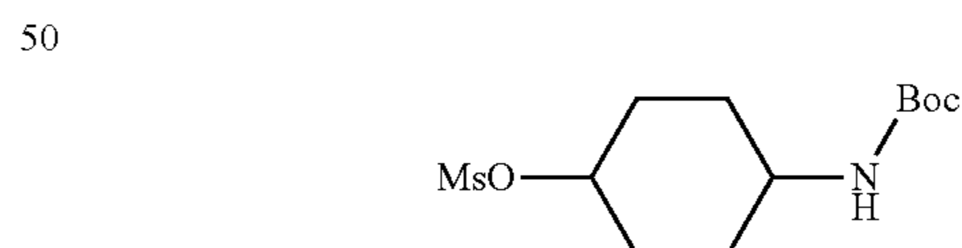
4-(tert-butoxycarbonyl)cyclohexyl methanesulfonate
