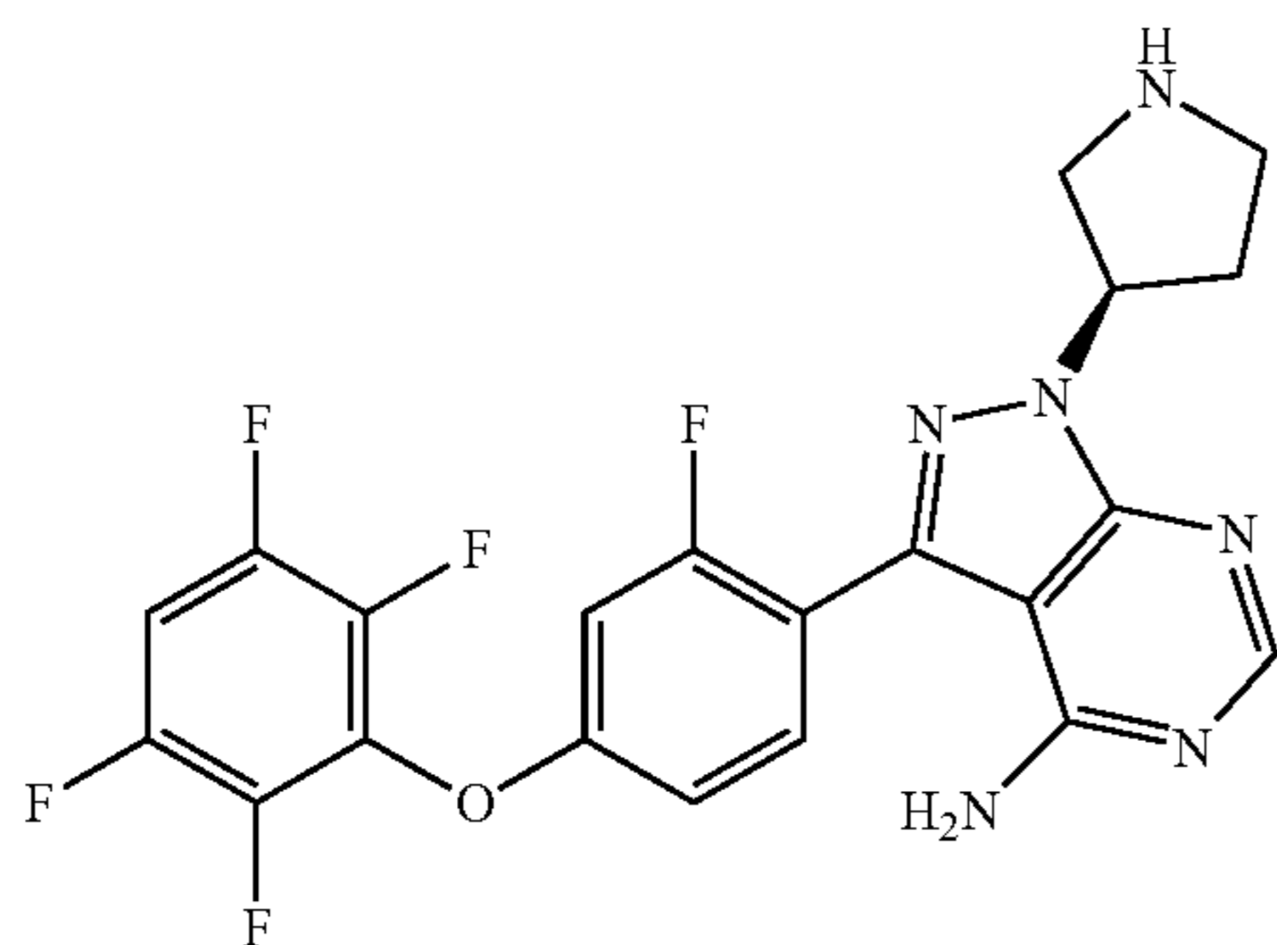
3-(2-fluoro-4-(2,3,5,6-tetrafluorophenoxy)phenyl)-1-((R)-pyrrolidin-3-yl)-1H-pyrazolo[3,4-d]pyrimidin-4-amine
