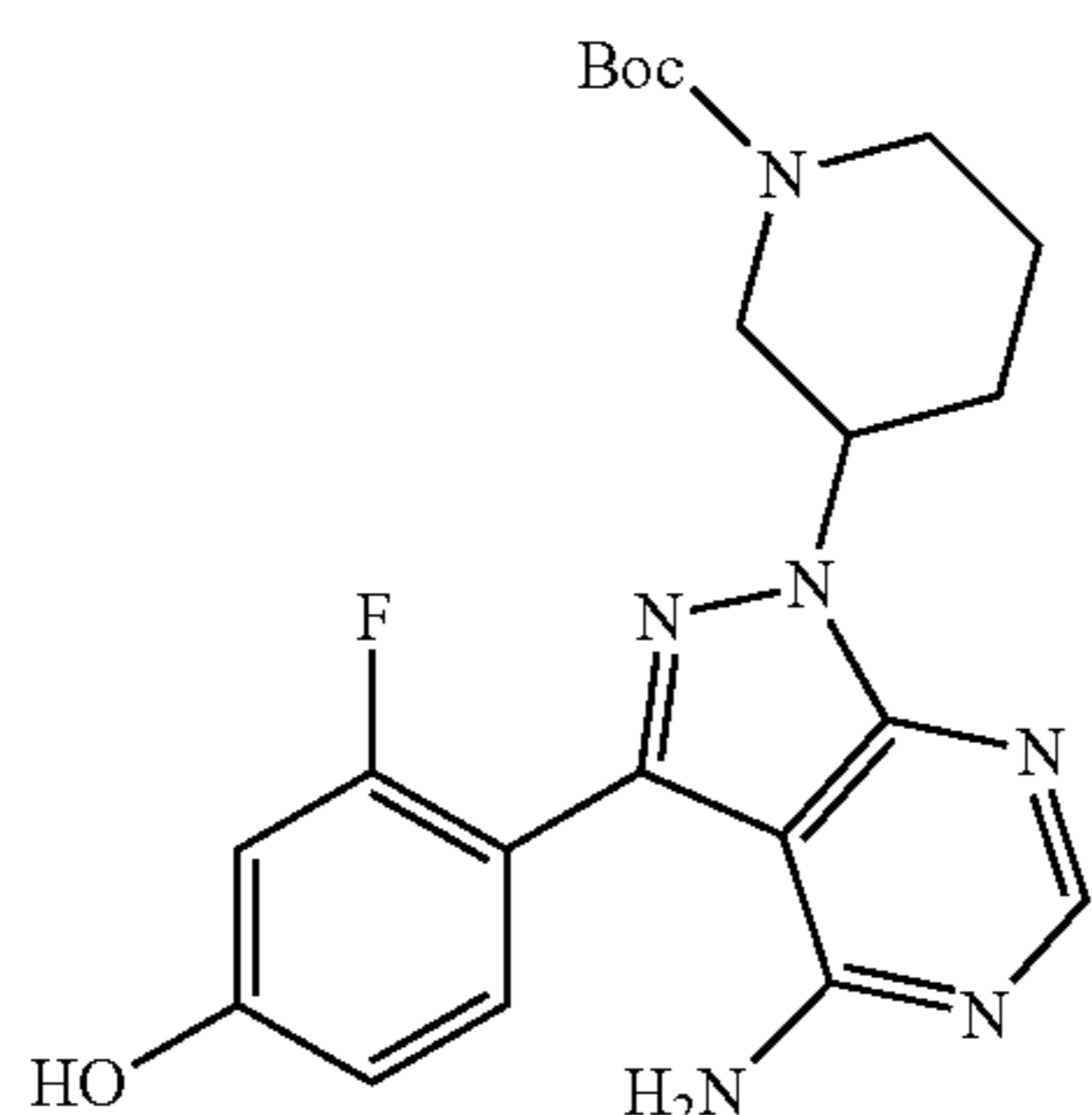
tert-butyl 3-(4-amino-3-(2-fluoro-4-hydroxyphenyl)-1H-pyrazolo[3,4-d]pyrimidin-1-yl)piperidine-1-carboxylate
