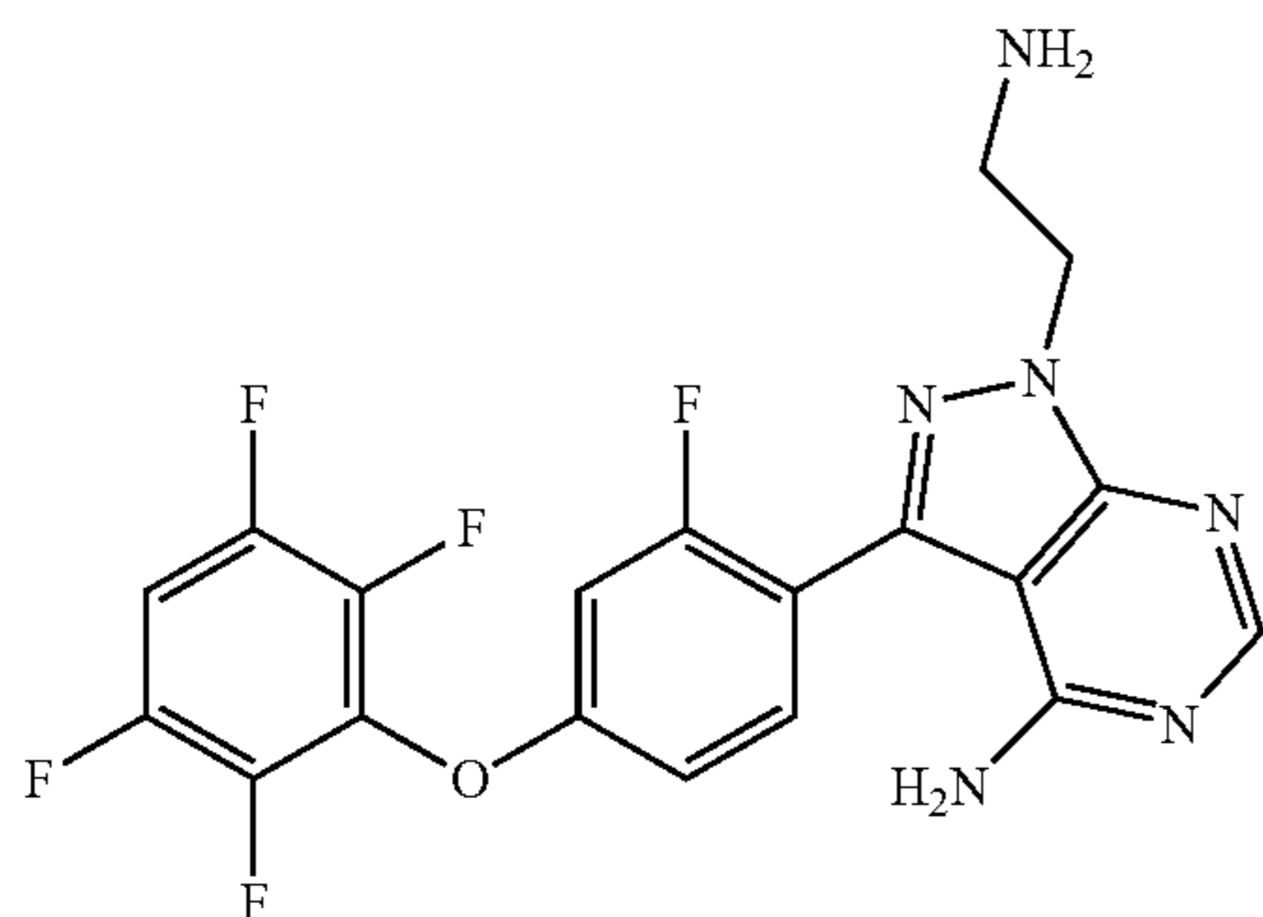
1-(2-aminoethyl)-3-(2-fluoro-4-(2,3,5,6-tetrafluorophenoxy)phenyl)-1H-pyrazolo[3,4-d]pyrimidin-4-amine
