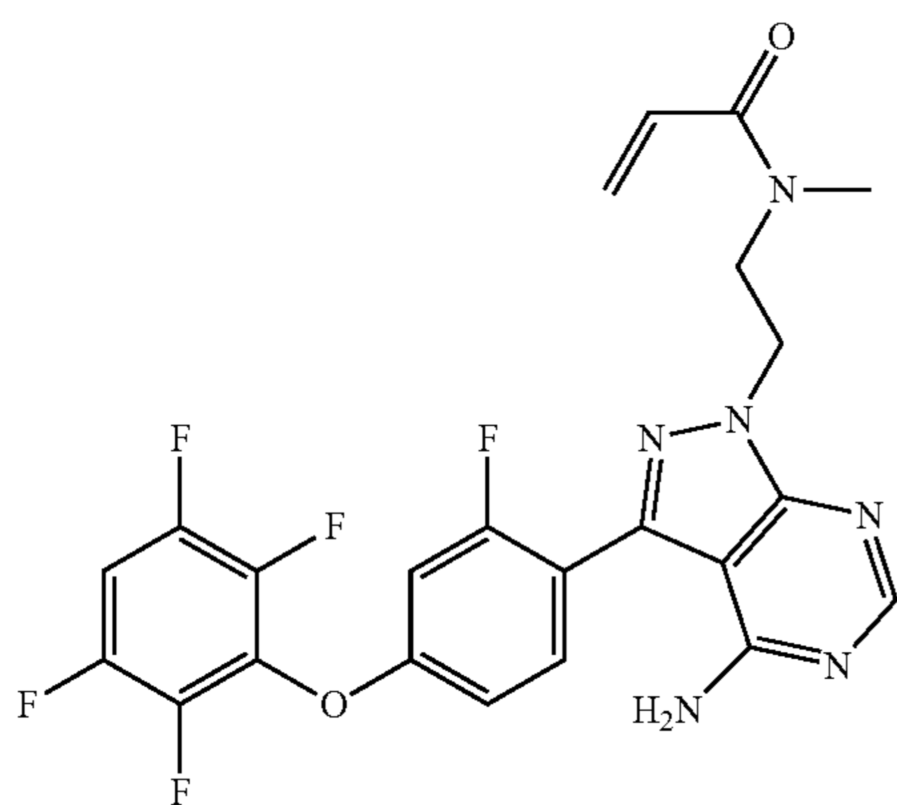
N-(2-(4-amino-3-(2-fluoro-4-(2,3,5,6-tetrafluorophenoxy)phenyl)-1H-pyrazolo[3,4-d]pyrimidin-1-yl)ethyl)-N-methylacrylamide
