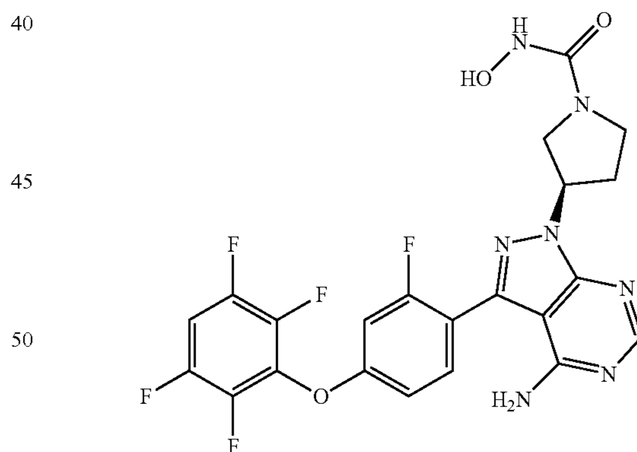
(3R)-3-(4-amino-3-(2-fluoro-4-(2,3,5,6-tetrafluorophenoxy)phenyl)-1H-pyrazolo[3,4-d]pyrimidin-1-yl)-N-hydroxypyrrolidine-1-carboxamide
