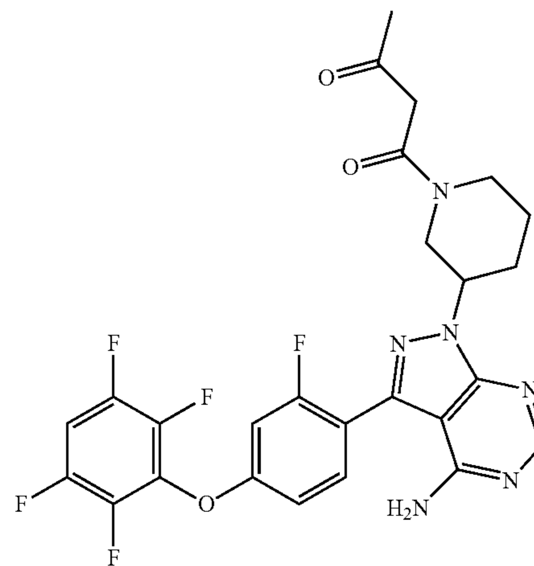
1-(3-(4-amino-3-(2-fluoro-4-(2,3,5,6-tetrafluorophenoxy)phenyl)-1H-pyrazolo[3,4-d]pyrimidin-1-yl)piperidin-1-yl)butane-1,3-dione
