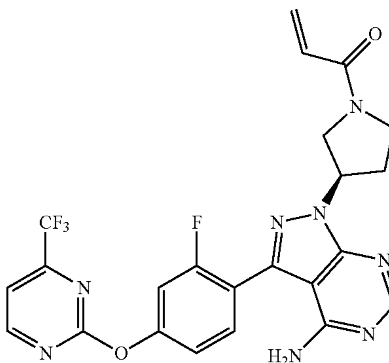
1-((R)-3-(4-amino-3-(2-fluoro-4-(4-(trifluoromethyl)pyrimidin-2-yloxy)phenyl)-1H-pyrazolo[3,4-d]pyrimidin-1-yl)pyrrolidin-1-yl)prop-2-en-1-one
