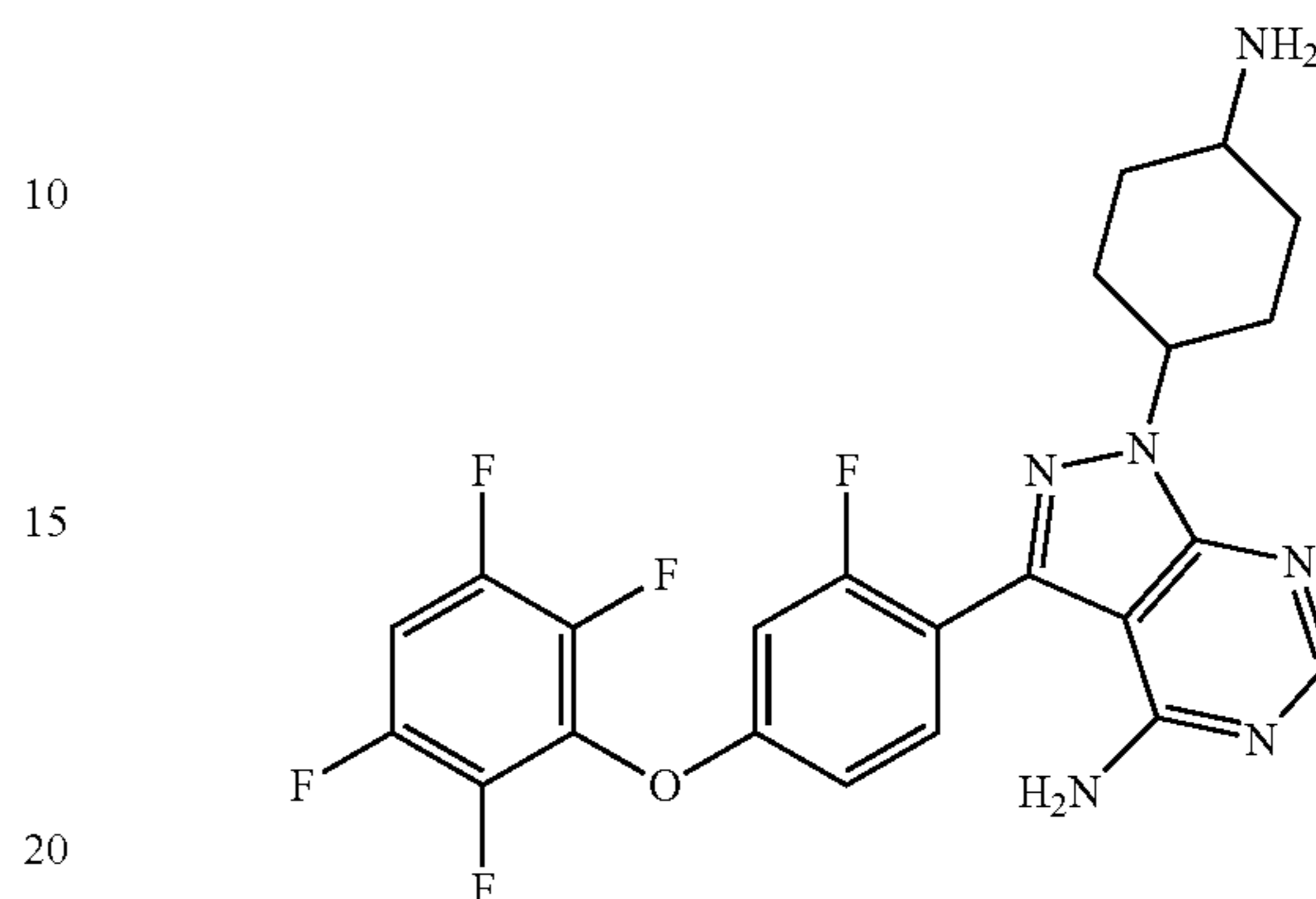
1-(4-aminocyclohexyl)-3-(2-fluoro-4-(2,3,5,6-tetrafluorophenoxy)phenyl)-1H-pyrazolo[3,4-d]pyrimidin-4-amine
