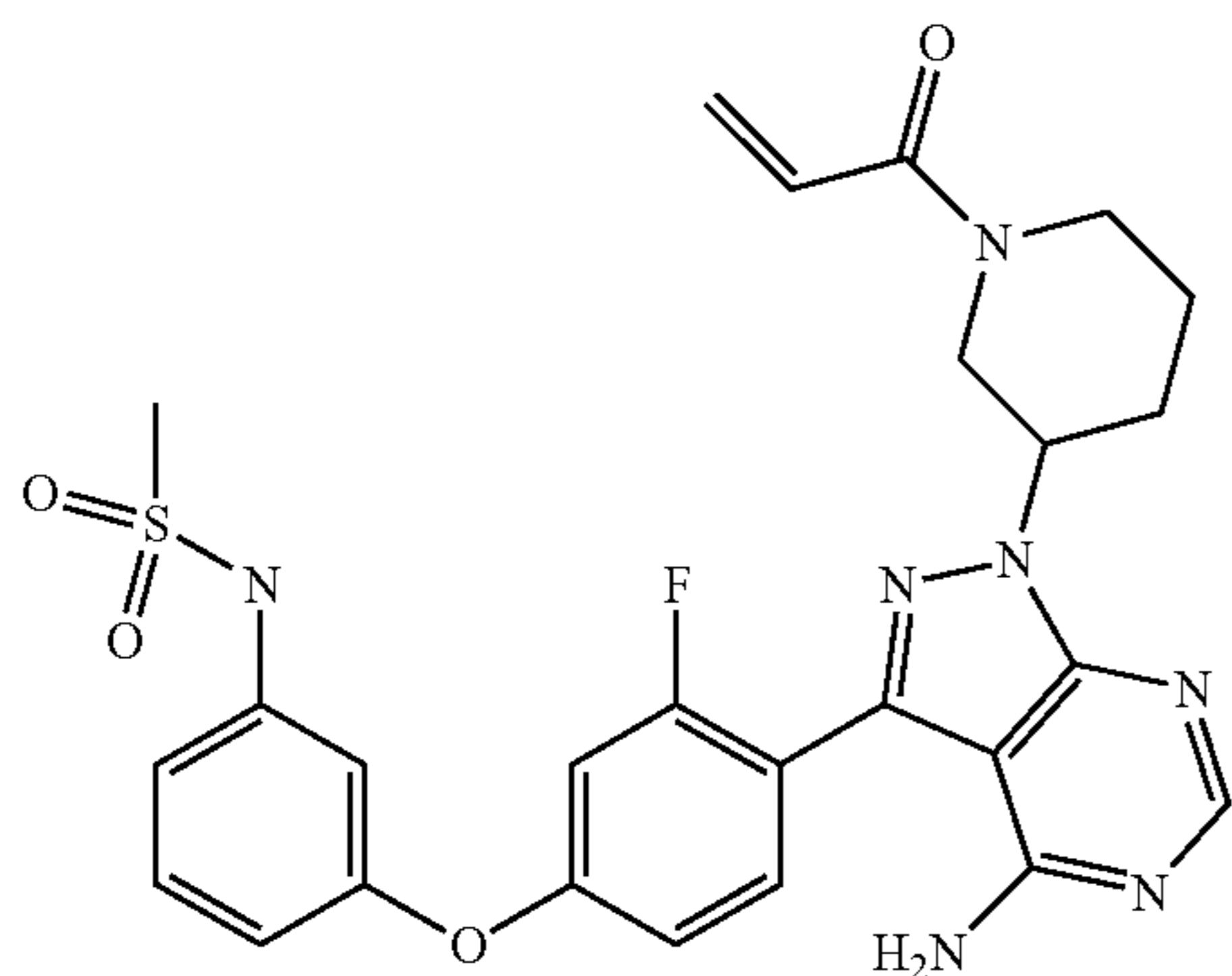
N-(3-(4-(1-(1-acryloylpiperidin-3-yl)-4-amino-1H-pyrazolo[3,4-d]pyrimidin-3-yl)-3-fluorophenoxy)phenyl)methanesulfonamide
