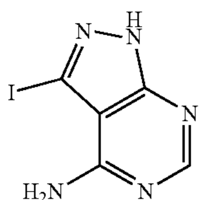
3-iodo-1H-pyrazolo[3,4-d]pyrimidin-4-amine
