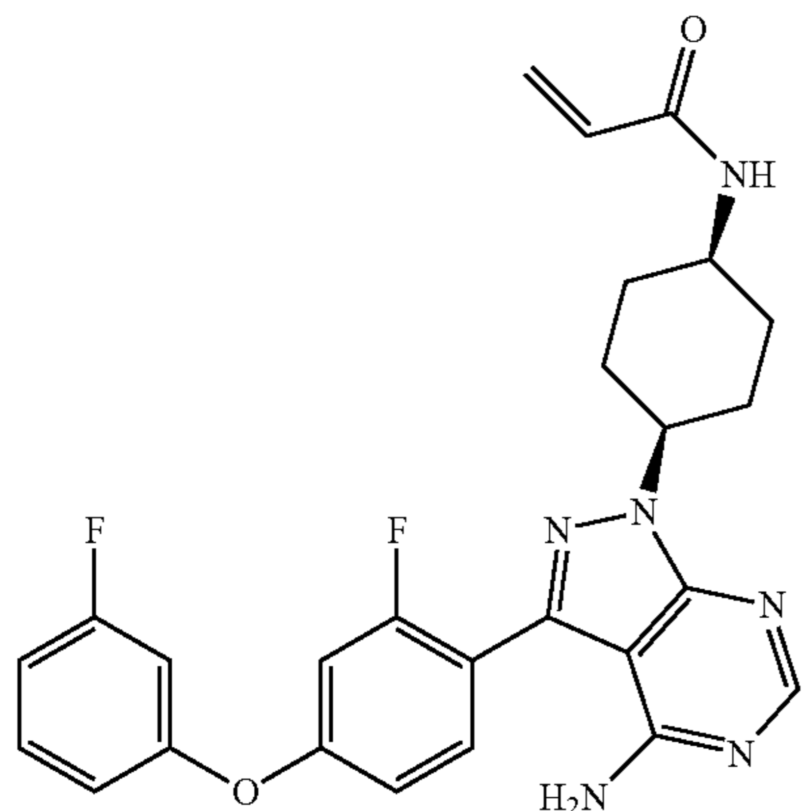
N-((1s,4s)-4-(4-amino-3-(2-fluoro-4-(3-fluorophenoxy)phenyl)-1H-pyrazolo[3,4-d]pyrimidin-1-yl)cyclohexyl)acrylamide
