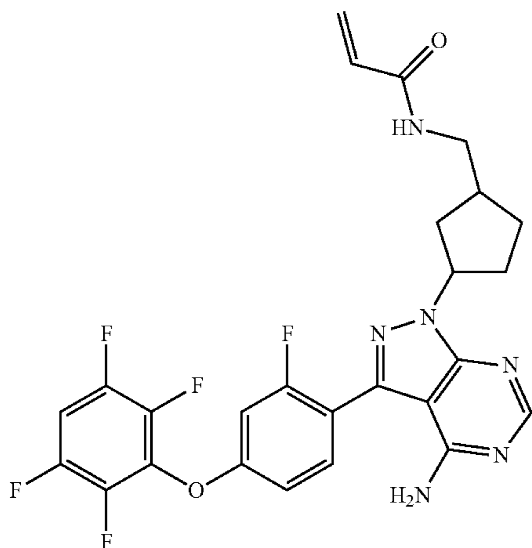
N-((3-(4-amino-3-(2-fluoro-4-(2,3,5,6-tetrafluorophenoxy)phenyl)-1H-pyrazolo[3,4-d]pyrimidin-1-yl)cyclopentyl)methyl)acrylamide
