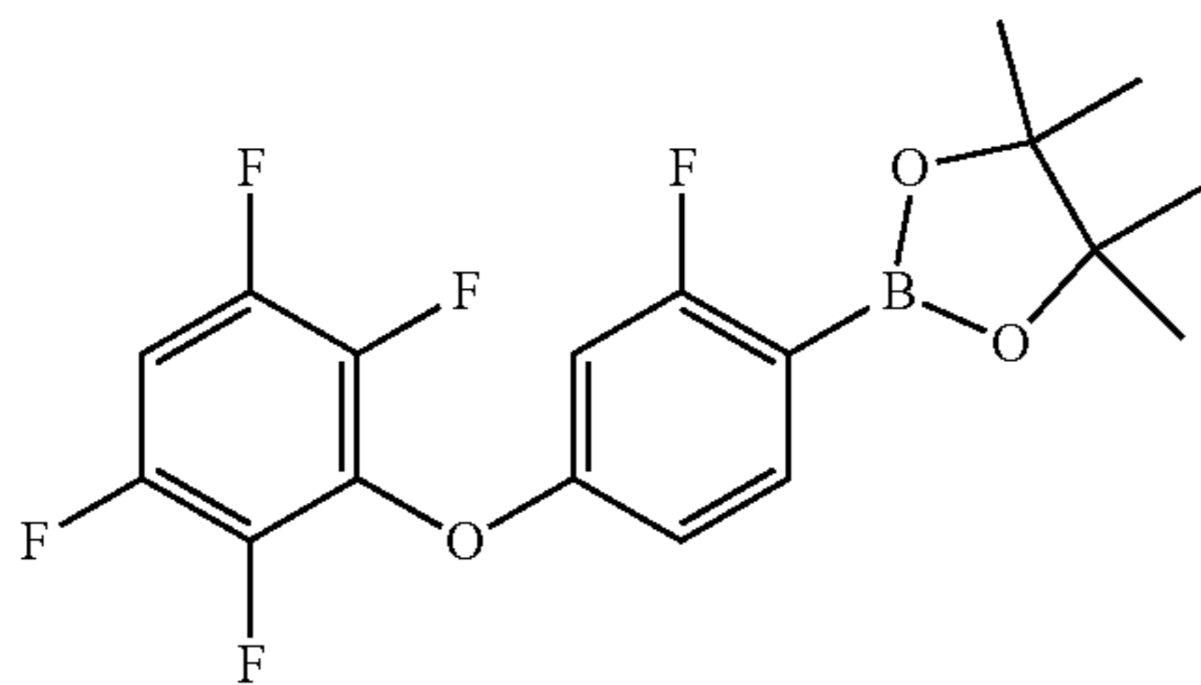
2-(2-fluoro-4-(2,3,5,6-tetrafluorophenoxy)phenyl)-4,4,5,5-tetramethyl-1,3,2-dioxaborolane
