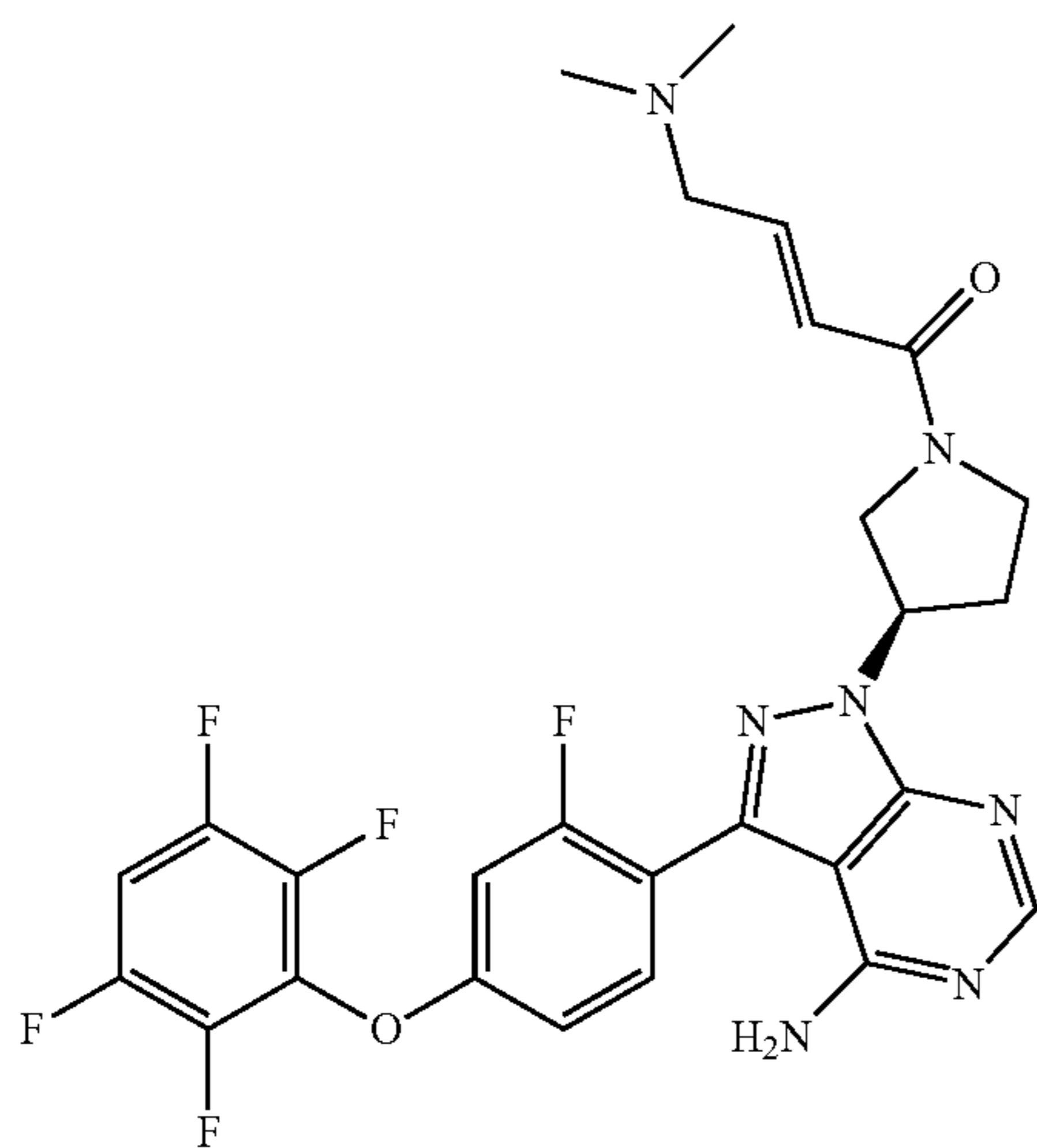
(E)-1-((R)-3-(4-amino-3-(2-fluoro-4-(2,3,5,6-tetrafluorophenoxy)phenyl)-1H-pyrazolo[3,4-d]pyrimidin-1-yl)pyrrolidin-1-yl)-4-(dimethylamino)but-2-en-1-one
