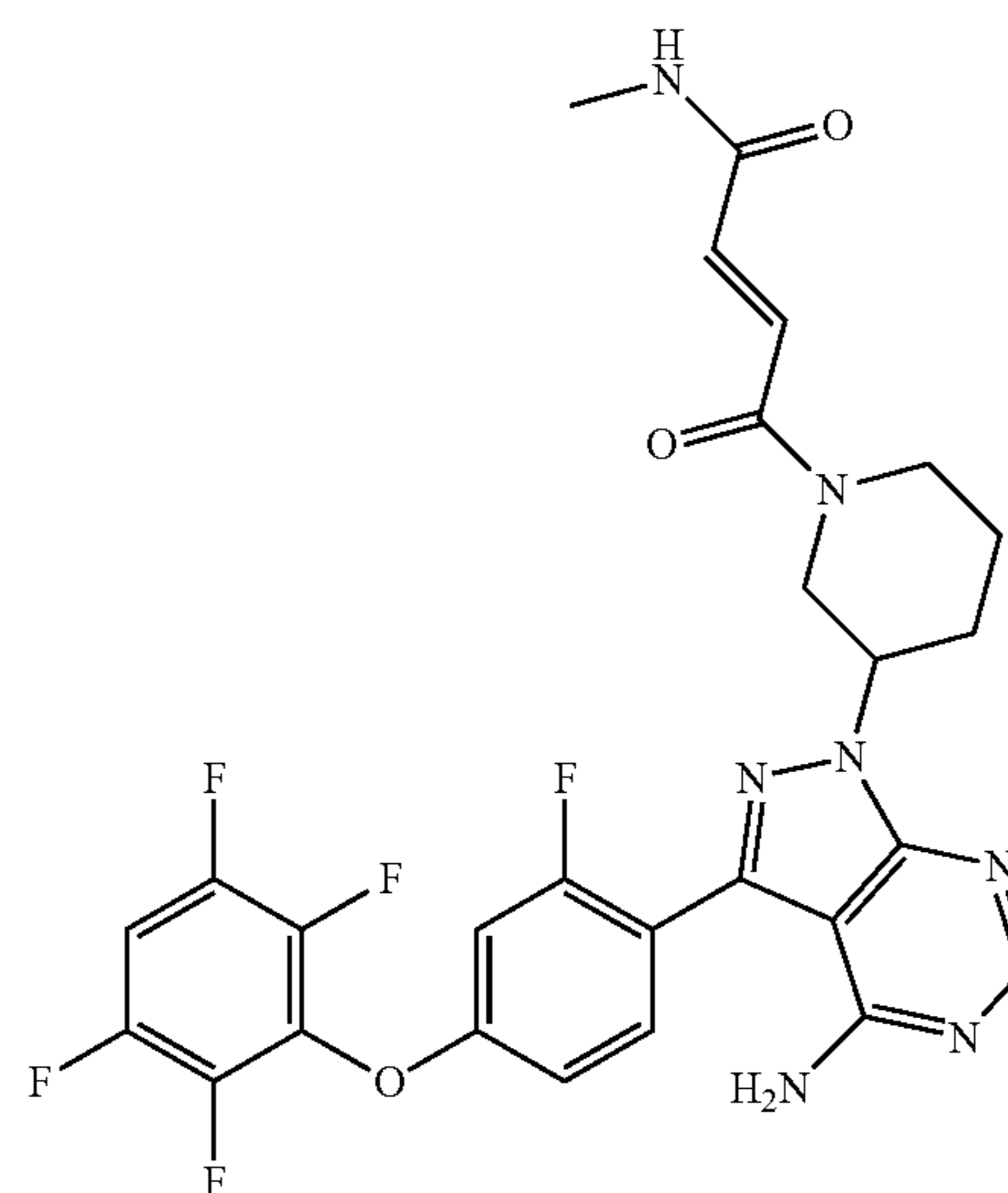
(E)-4-(3-(4-amino-3-(2-fluoro-4-(2,3,5,6-tetrafluorophenoxy)phenyl)-1H-pyrazolo[3,4-d]pyrimidin-1-yl)piperidin-1-yl)-N-methyl-4-oxobut-2-enamide
