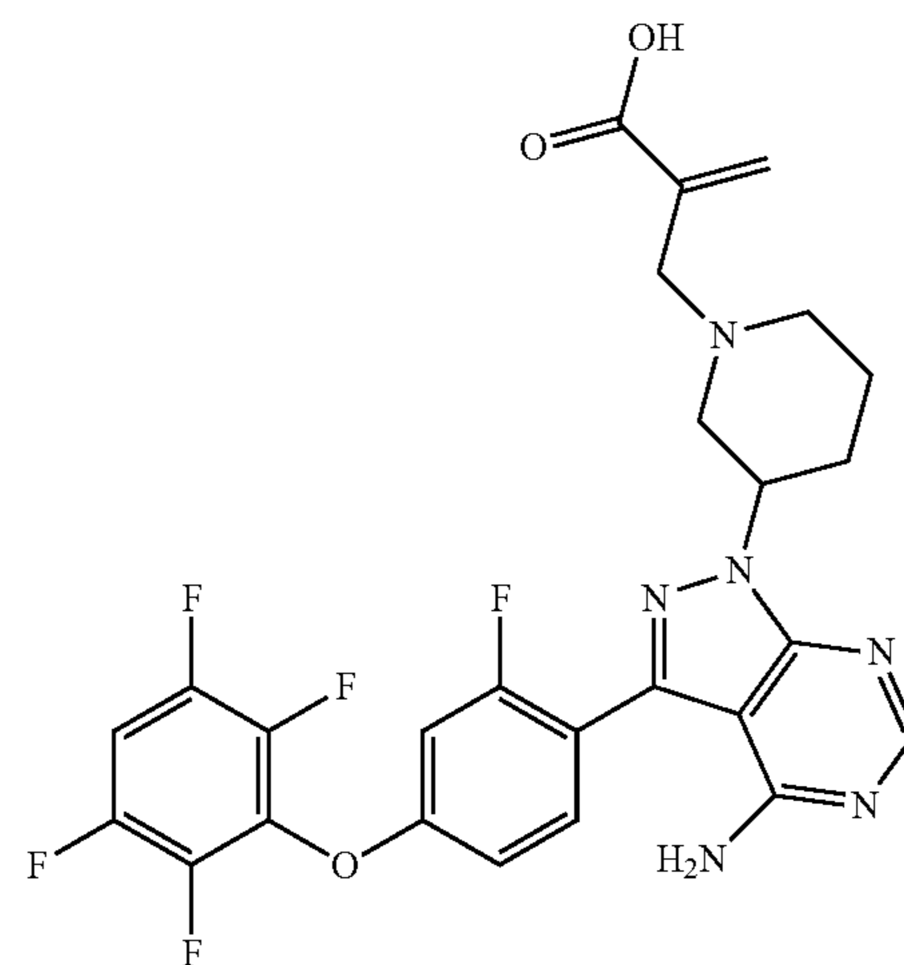
2-((3-(4-amino-3-(2-fluoro-4-(2,3,5,6-tetrafluorophenoxy)phenyl)-1H-pyrazolo[3,4-d]pyrimidin-1-yl)piperidin-1-yl)methyl)acrylic acid
