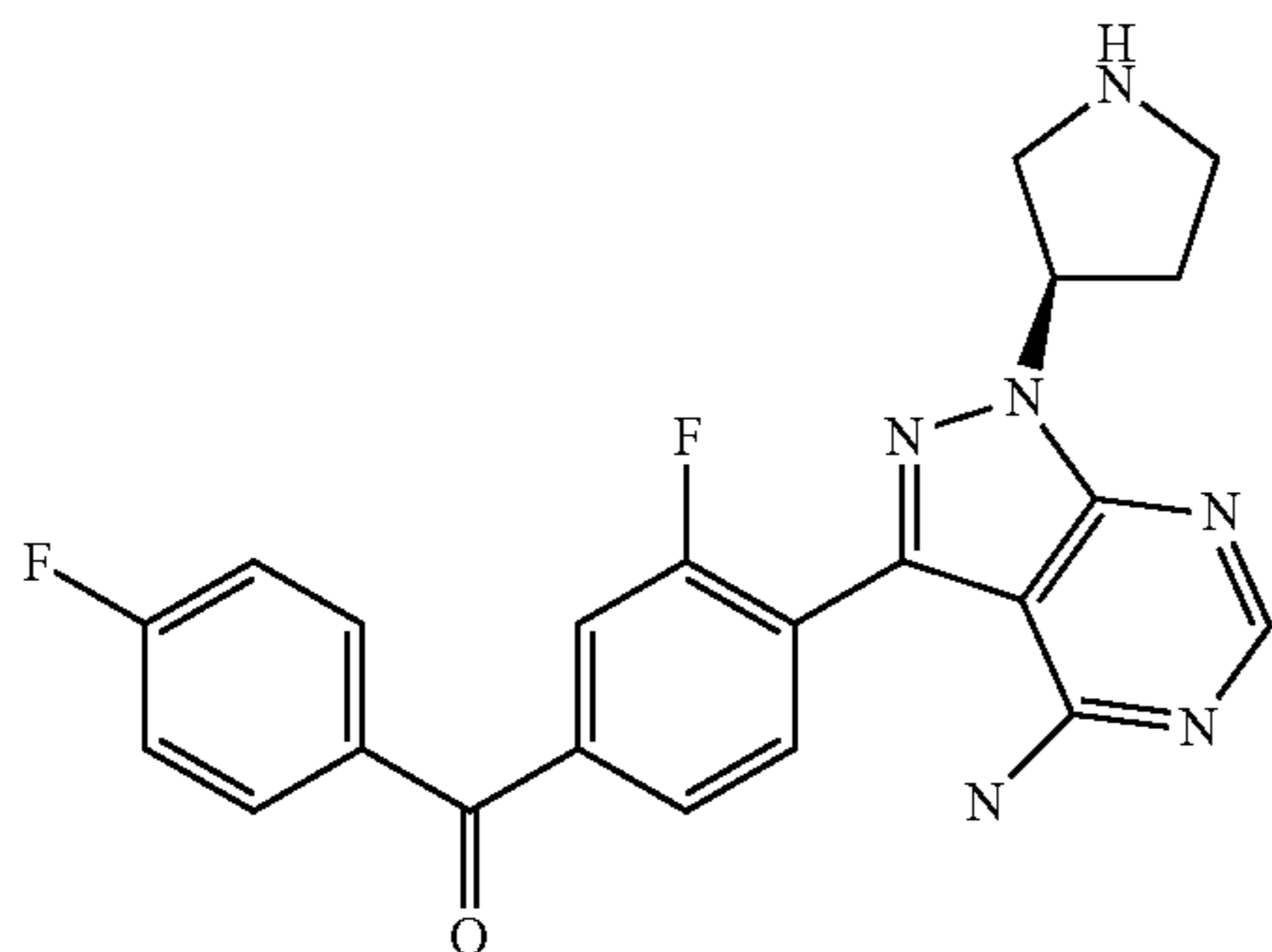
(4-(4-amino-1-((R)-pyrrolidin-3-yl)-1H-pyrazolo[3,4-d]pyrimidin-3-yl)-3-fluorophenyl)(4-fluorophenyl) methanone
