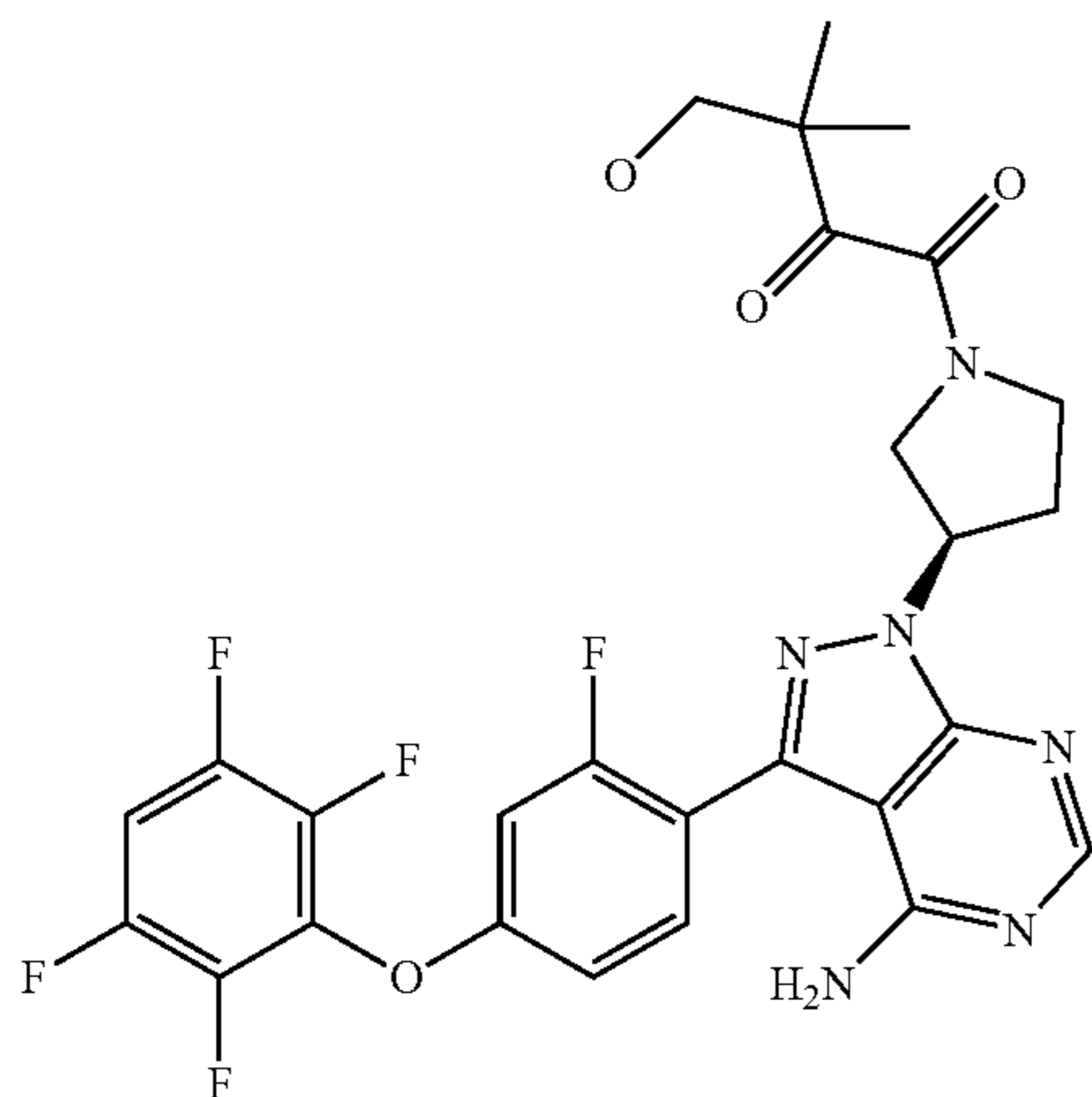
1-((R)-3-(4-amino-3-(2-fluoro-4-(2,3,5,6-tetrafluorophenoxy)phenyl)-1H-pyrazolo[3,4-d]pyrimidin-1-yl)pyrrolidin-1-yl)-4-hydroxy-3,3-dimethylbutane-1,2-dione
