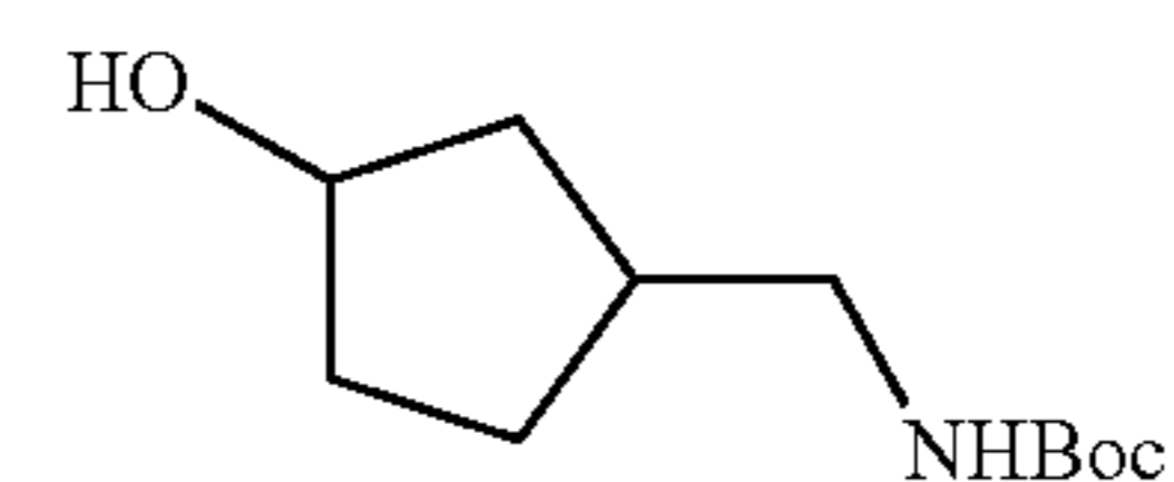
tert-butyl (3-hydroxycyclopentyl)methylcarbamate
