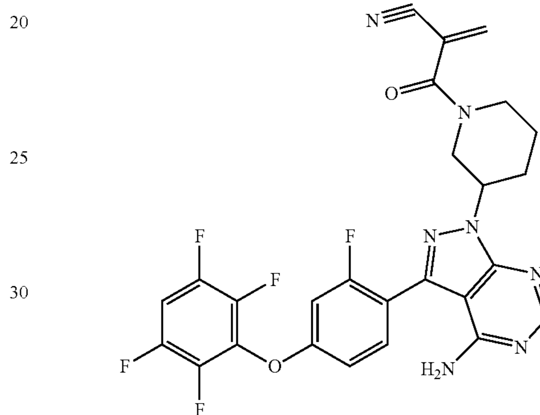
(Z)-methyl 2-(3-(4-amino-3-(2-fluoro-4-(2,3,5,6-tetrafluorophenoxy)phenyl)-1H-pyrazolo[3,4-d]pyrimidin-1-yl)piperidine-1-carbonyl)but-2-enoate
