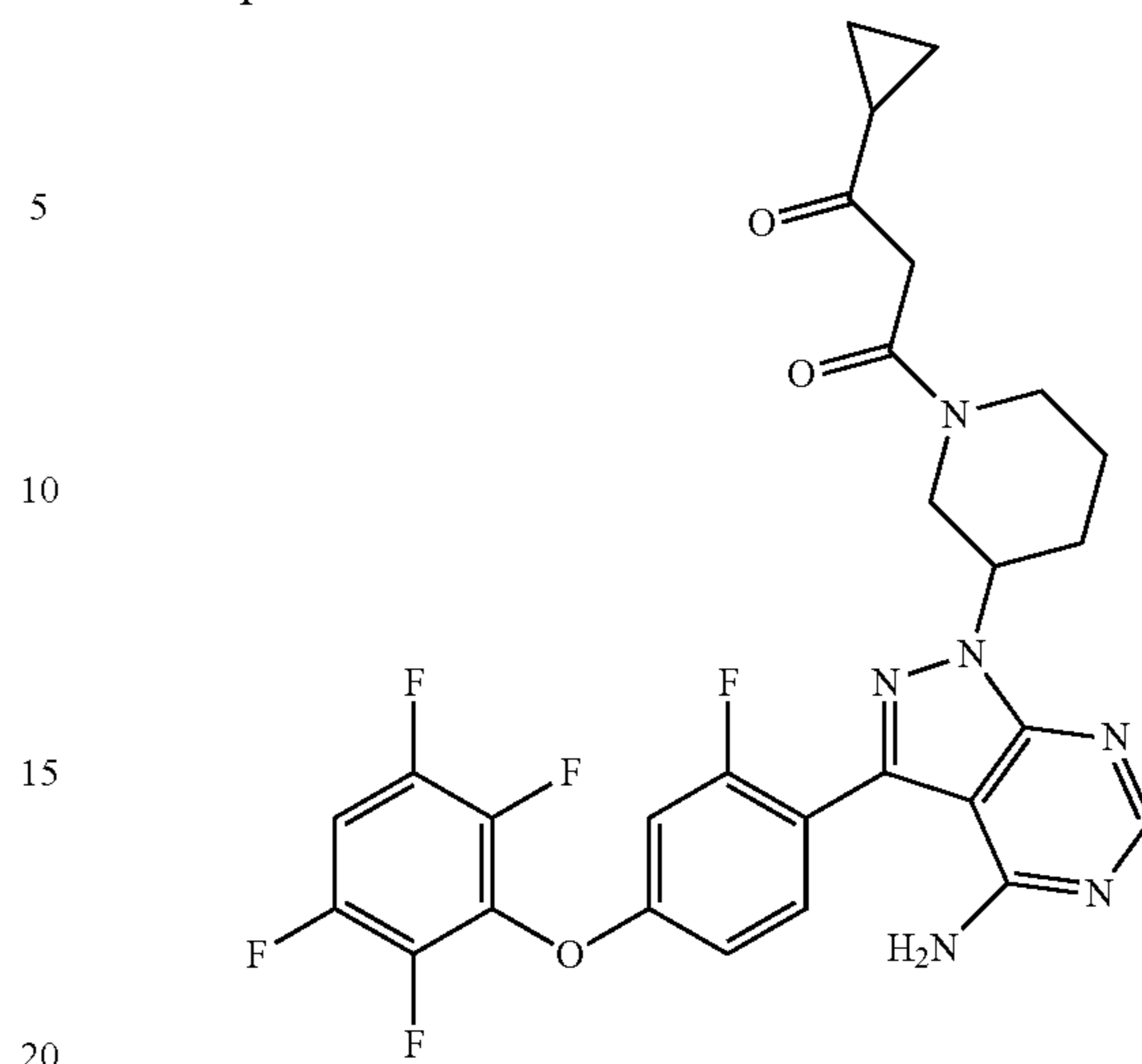
1-(3-(4-amino-3-(2-fluoro-4-(2,3,5,6-tetrafluorophenoxy)phenyl)-1H-pyrazolo[3,4-d]pyrimidin-1-yl)piperidin-1-yl)-3-cyclopropylpropane-1,3-dione
