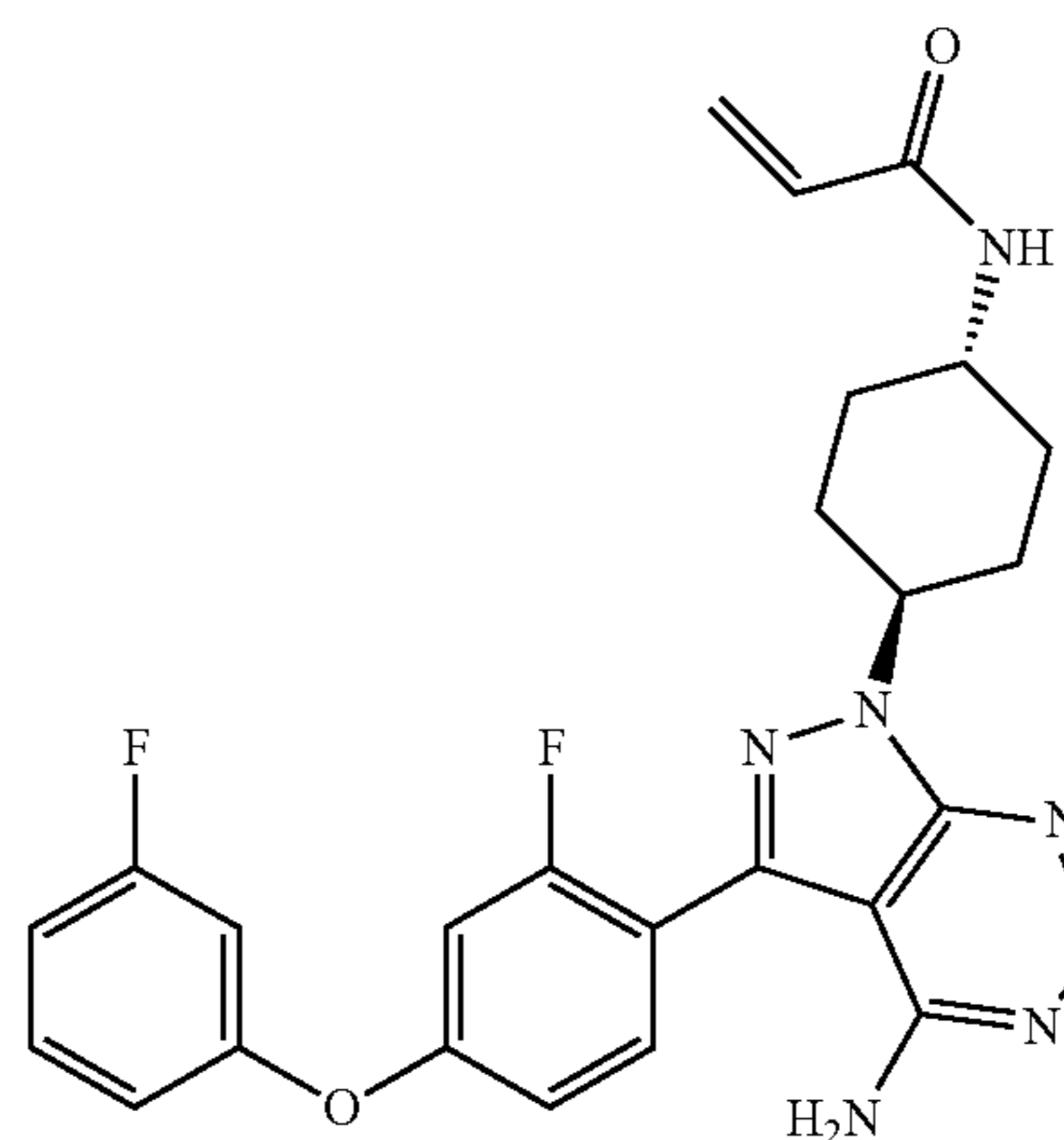
N-((1r,4r)-4-(4-amino-3-(2-fluoro-4-(3-fluorophenoxy)phenyl)-1H-pyrazolo[3,4-d]pyrimidin-1-yl)cyclohexyl)acrylamide
