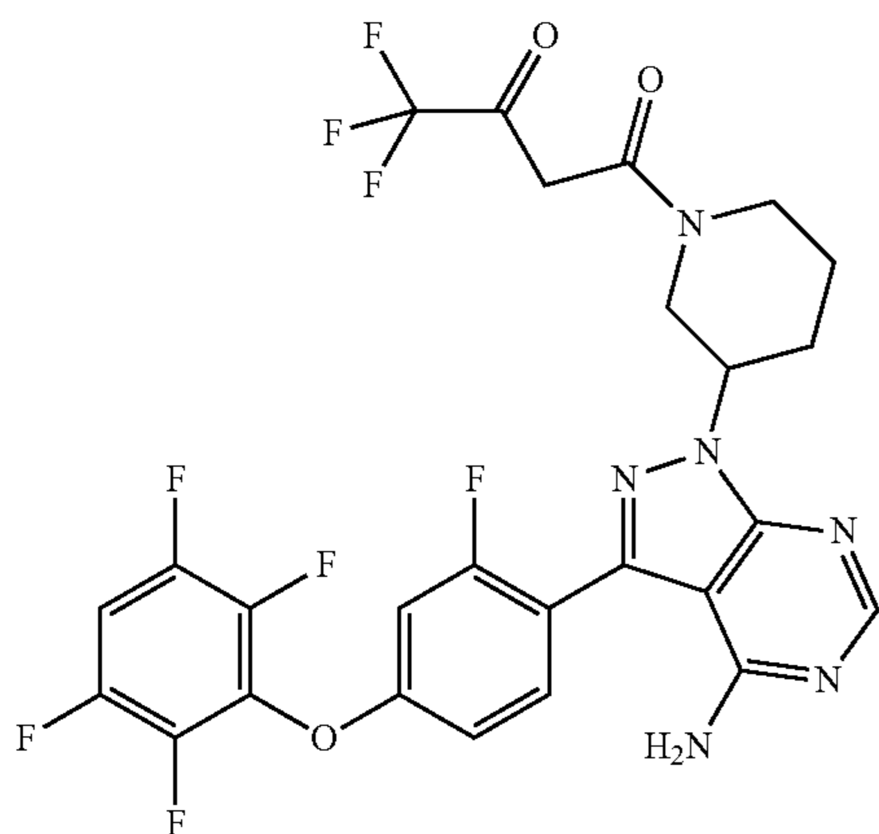
1-(3-(4-amino-3-(2-fluoro-4-(2,3,5,6-tetrafluorophenoxy)phenyl)-1H-pyrazolo[3,4-d]pyrimidin-1-yl)piperidin-1-yl)-4,4,4-trifluorobutane-1,3-dione
