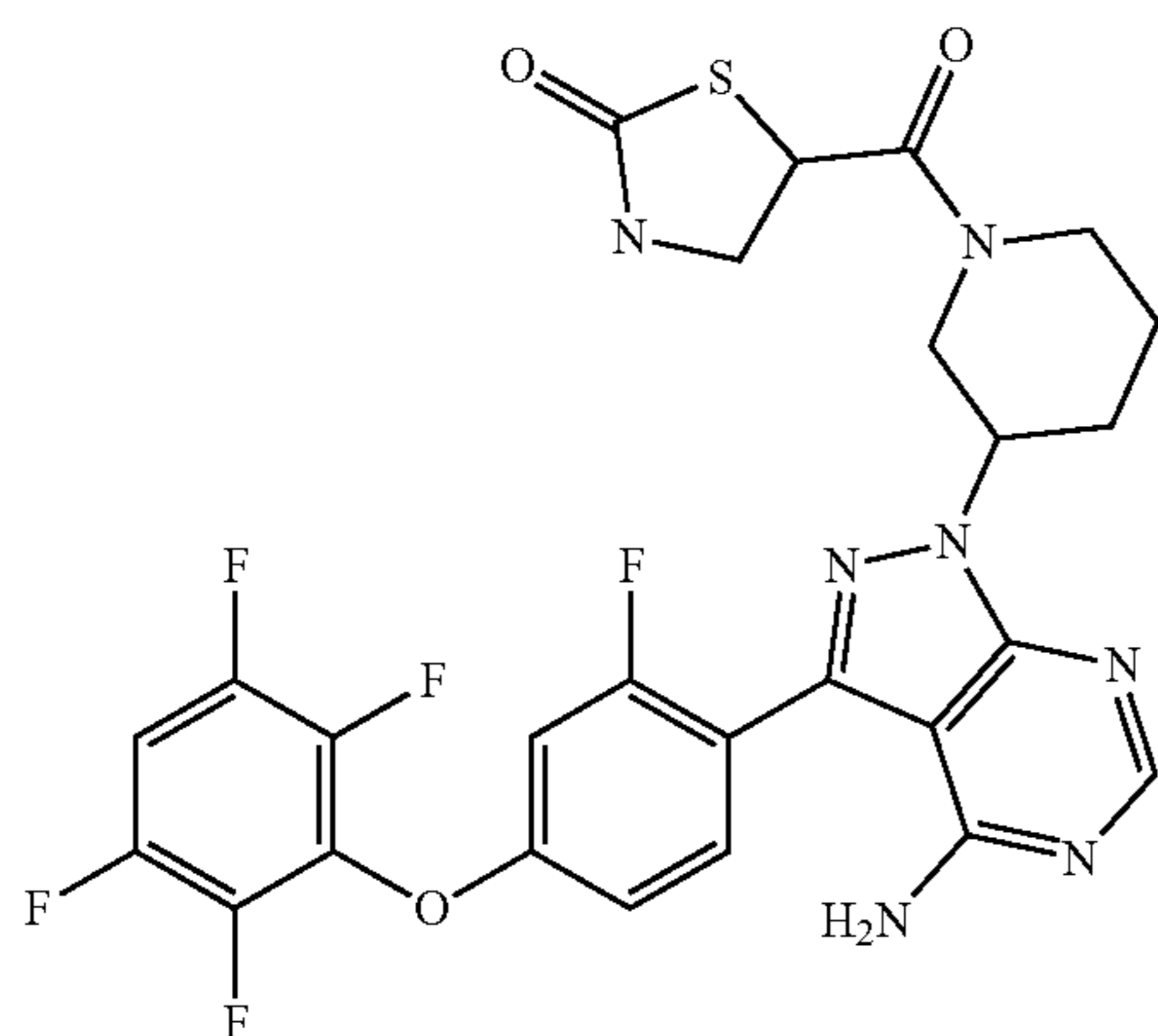
5-(3-(4-amino-3-(2-fluoro-4-(2,3,5,6-tetrafluorophenoxy)phenyl)-1H-pyrazolo[3,4-d]pyrimidin-1-yl)piperidine-1-carbonyl)thiazolidin-2-one
