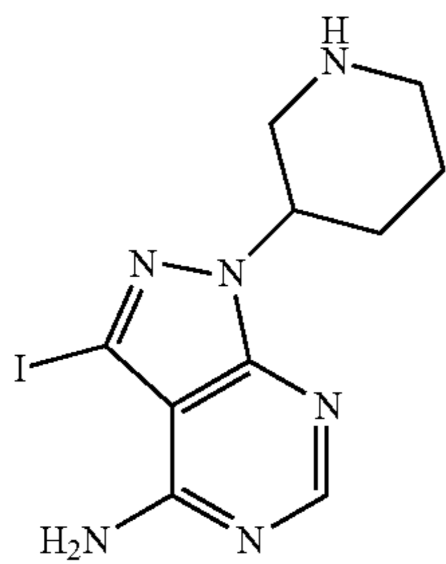
3-iodo-1-(piperidin-3-yl)-1H-pyrazolo[3,4-d]pyrimidin-4-amine
