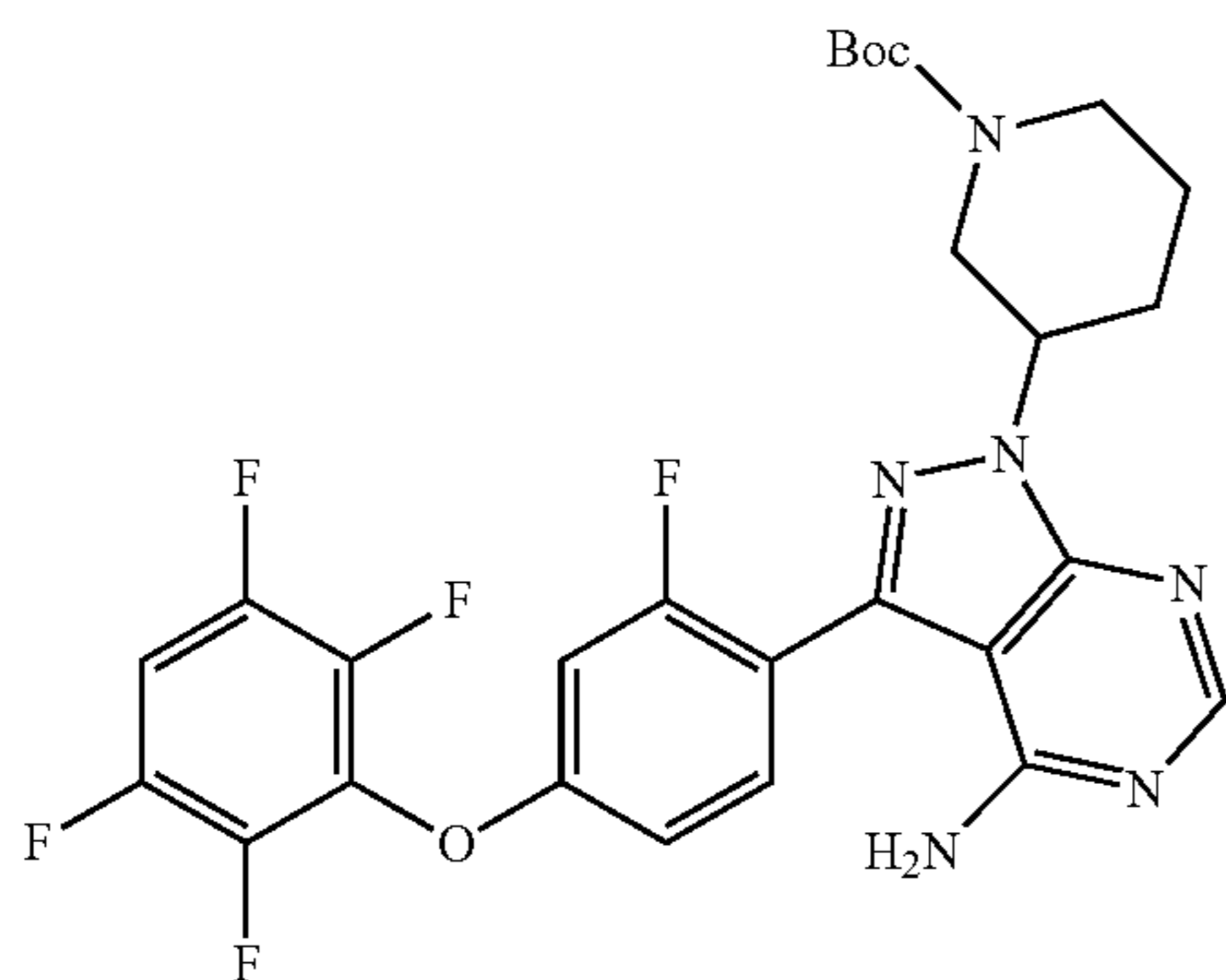
tert-butyl 3-(4-amino-3-(2-fluoro-4-(2,3,5,6-tetrafluorophenoxy)phenyl)-1H-pyrazolo[3,4-d]pyrimidin-1-yl)piperidine-1-carboxylate
