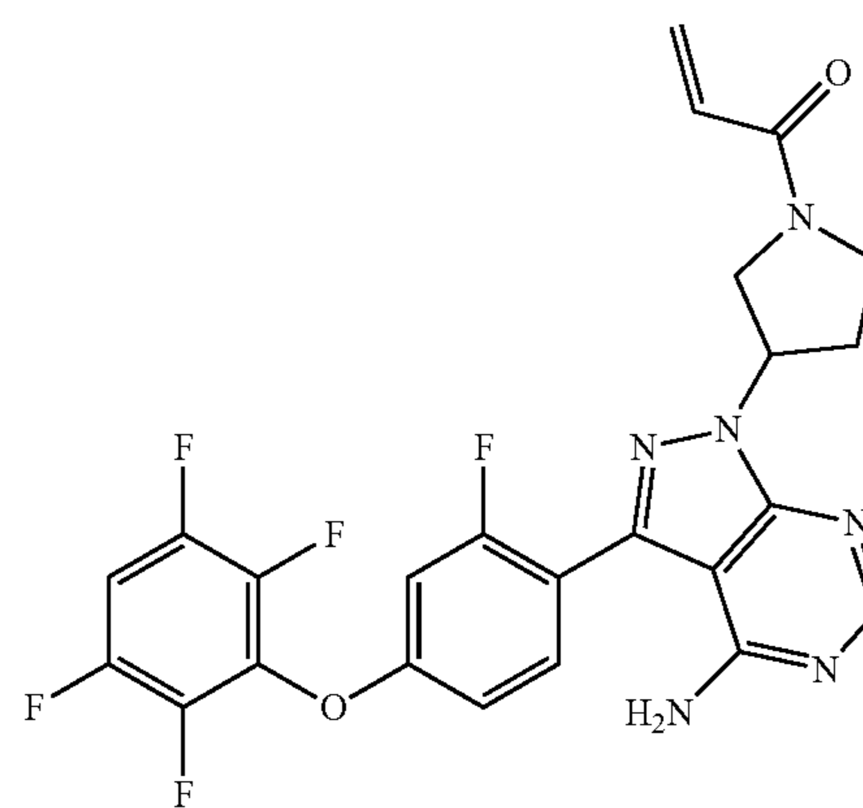
1-(3-(4-amino-3-(2-fluoro-4-(2,3,5,6-tetrafluorophenoxy)phenyl)-1H-pyrazolo[3,4-d]pyrimidin-1-yl)pyrrolidin-1-yl)prop-2-en-1-one
