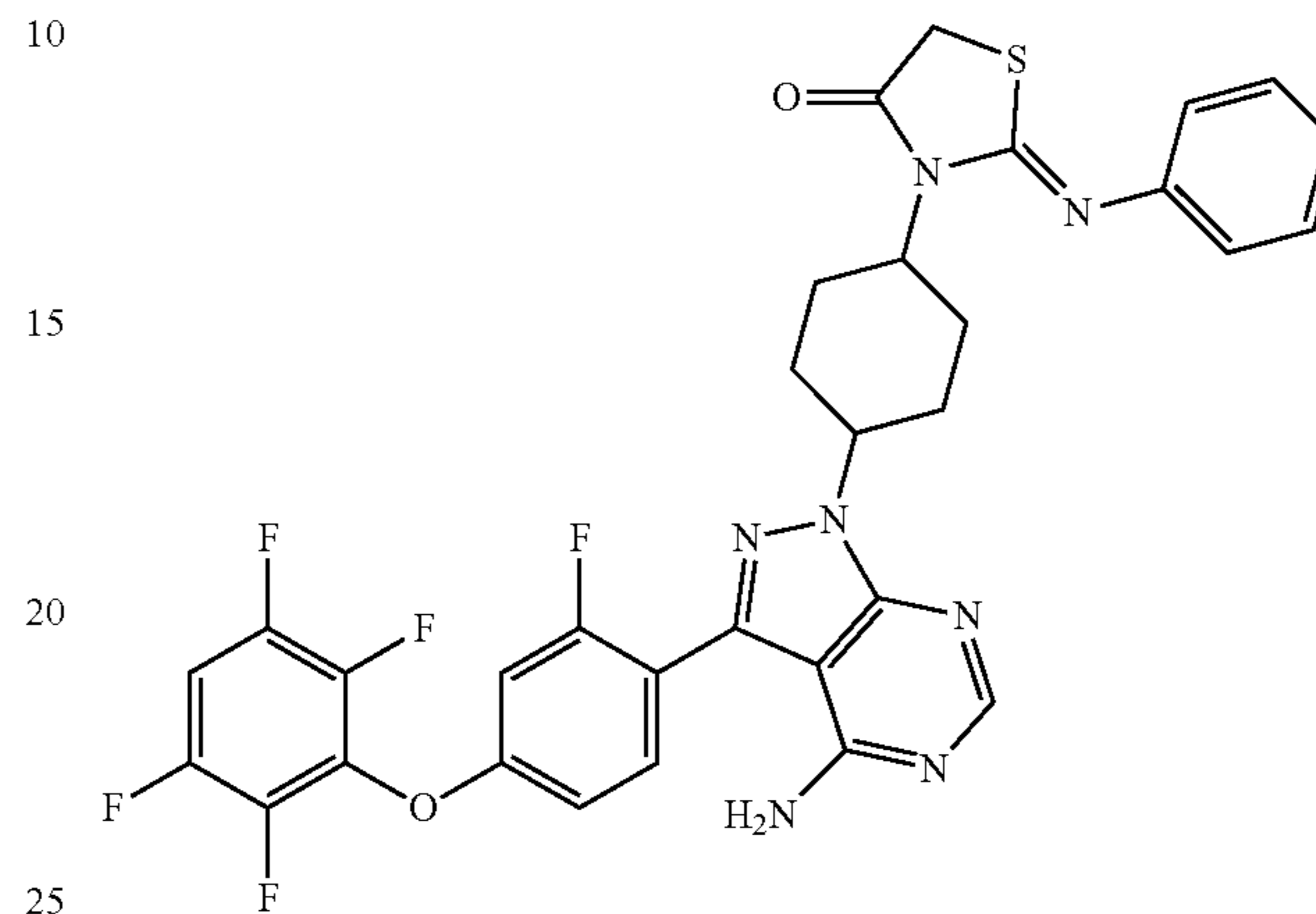
(Z)-3-(4-(4-amino-3-(2-fluoro-4-(2,3,5,6-tetrafluorophenoxy)phenyl)-1H-pyrazolo[3,4-d]pyrimidin-1-yl)cyclohexyl)-2-(phenylimino)thiazolidin-4-one
