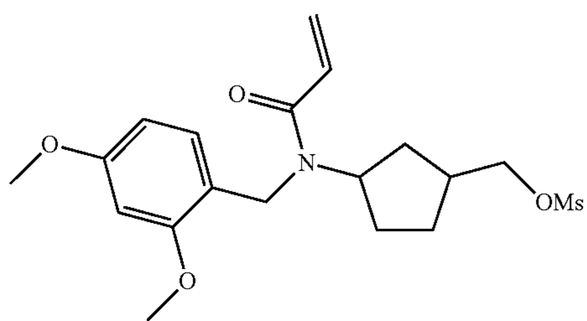
(3-(N-(2,4-dimethoxybenzyl)acrylamido)cyclopentyl)methyl methanesulfonate
