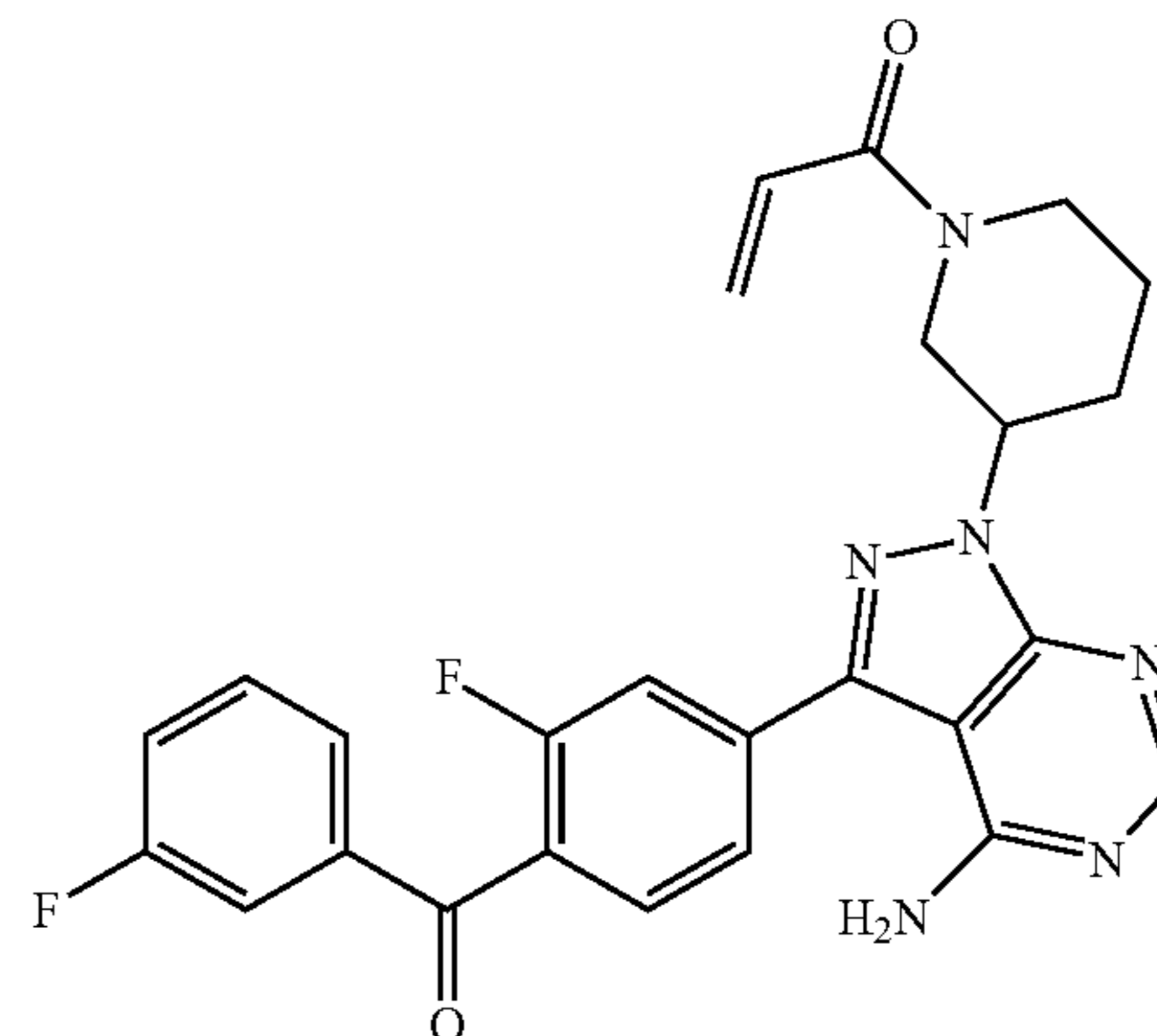
1-(3-(4-amino-3-(3-fluoro-4-(3-fluorobenzoyl)phenyl)-1H-pyrazolo[3,4-d]pyrimidin-1-yl)piperidin-1-yl)prop-2-en-1-one
