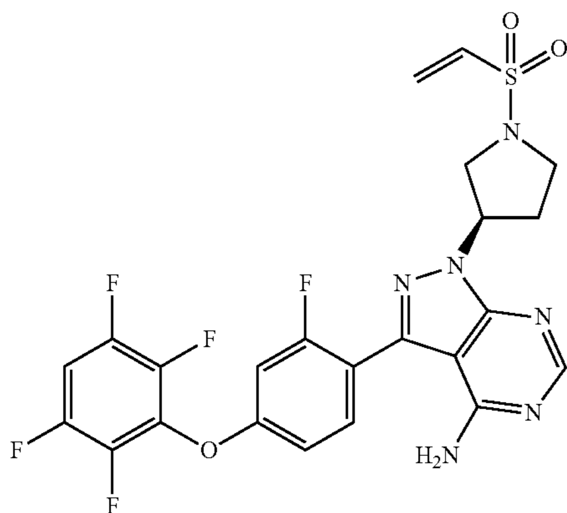
3-(2-fluoro-4-(2,3,5,6-tetrafluorophenoxy)phenyl)-1-((R)-1-(vinylsulfonyl)pyrrolidin-3-yl)-1H-pyrazolo[3,4-d]pyrimidin-4-amine
