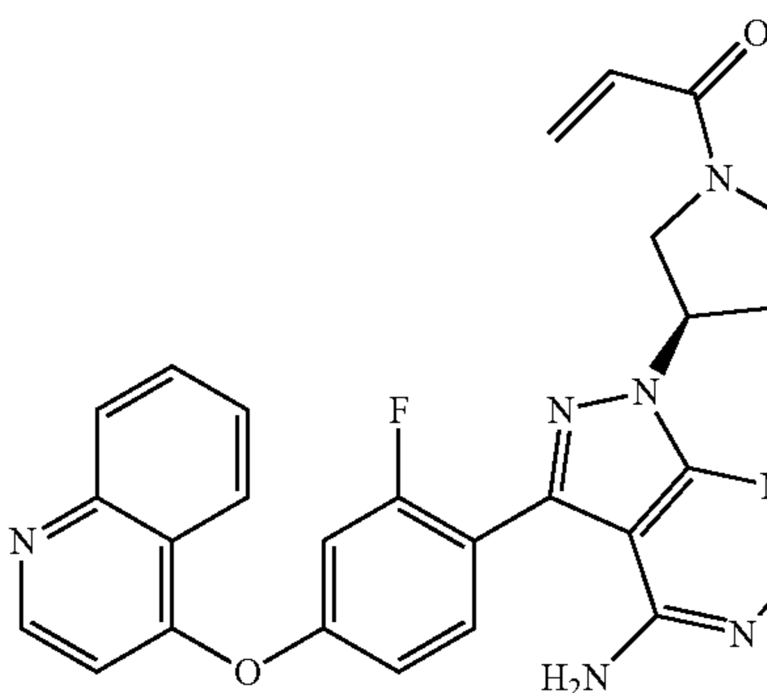
1-((R)-3-(4-amino-3-(2-fluoro-4-(quinolin-4-yloxy)phenyl)-1H-pyrazolo[3,4-d]pyrimidin-1-yl)pyrrolidin-1-yl)prop-2-en-1-one
