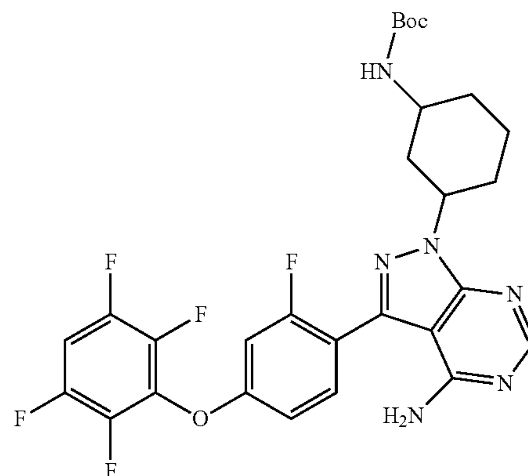
tert-butyl 3-(4-amino-3-(2-fluoro-4-(2,3,5,6-tetrafluorophenoxy)phenyl)-1H-pyrazolo[3,4-d]pyrimidin-1-yl)cyclohexylcarbamate
