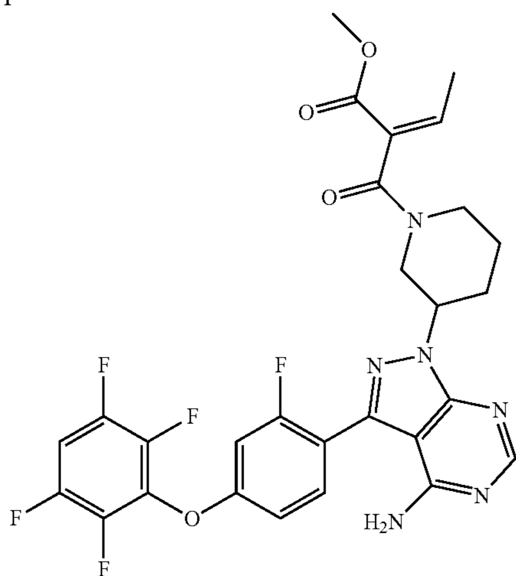
(Z)-methyl 2-(3-(4-amino-3-(2-fluoro-4-(2,3,5,6-tetrafluorophenoxy)phenyl)-1H-pyrazolo[3,4-d]pyrimidin-1-yl)piperidine-1-carbonyl)but-2-enoate
