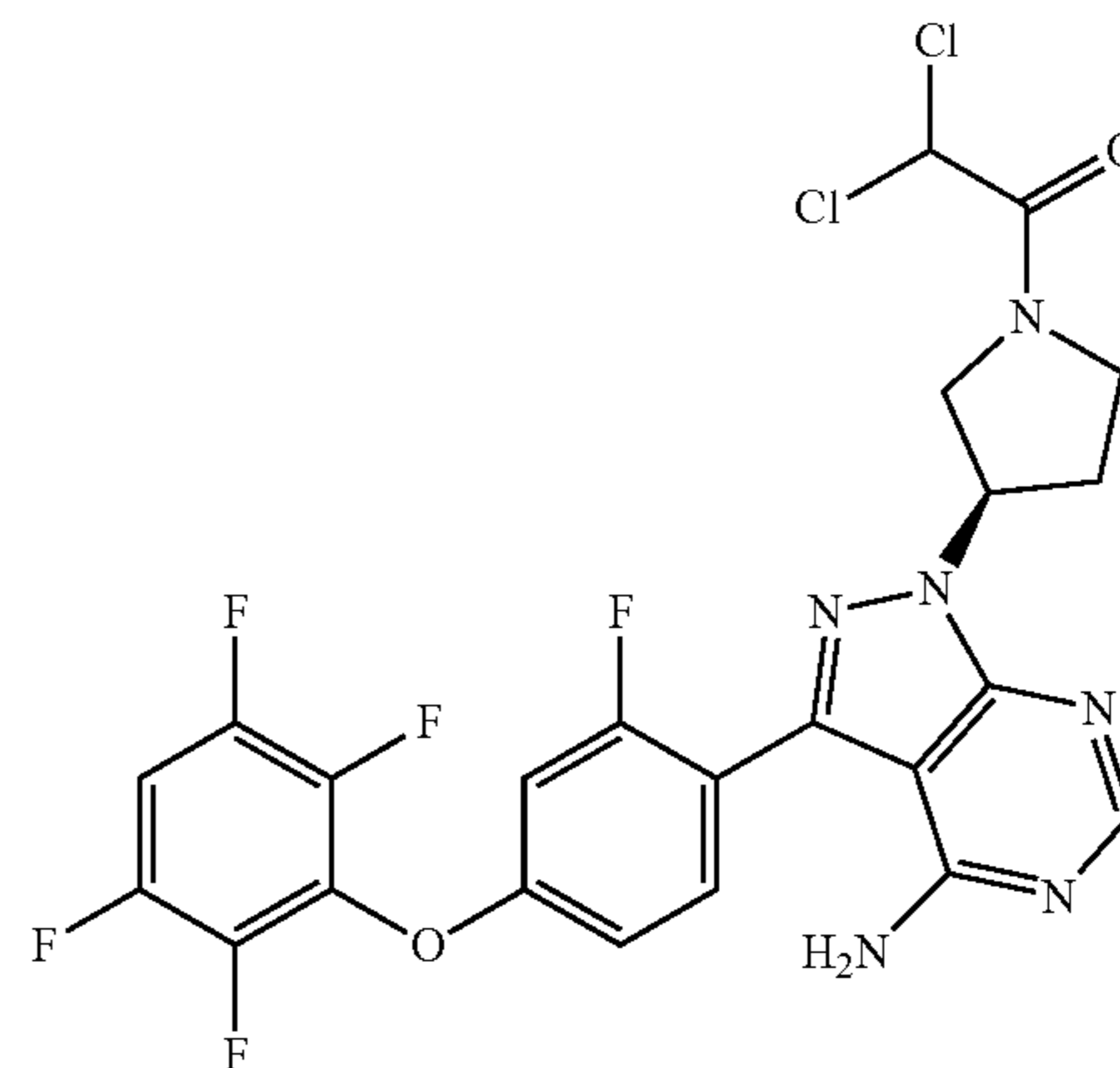
1-((R)-3-(4-amino-3-(2-fluoro-4-(2,3,5,6-tetrafluorophenoxy)phenyl)-1H-pyrazolo[3,4-d]pyrimidin-1-yl)pyrrolidin-1-yl)-2,2-dichloroethanone
