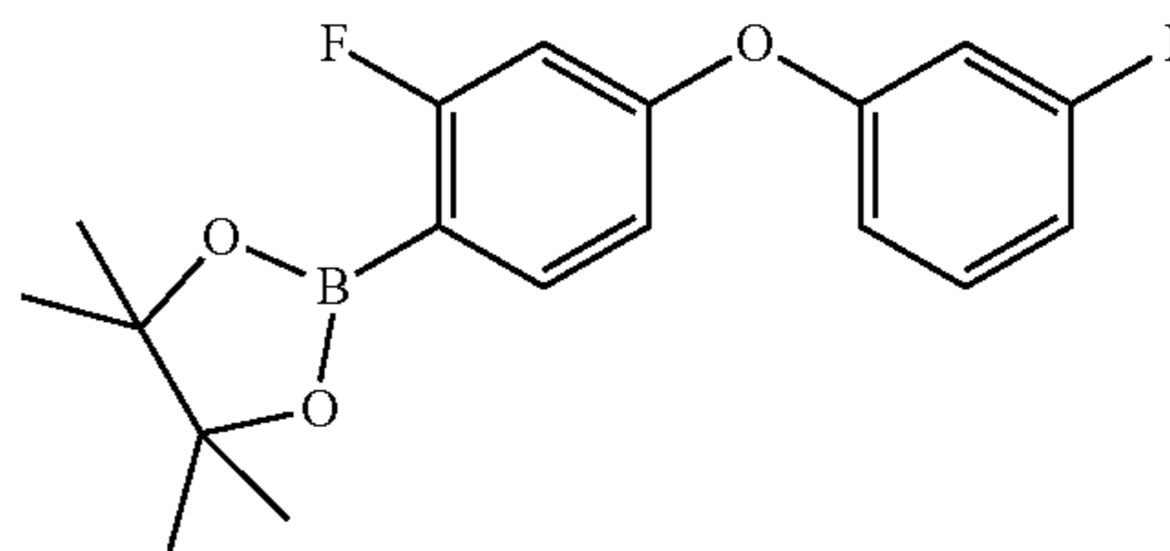
2-(2-fluoro-4-(3-fluorophenoxy)phenyl)-4,4,5,5-tetramethyl-1,3,2-dioxaborolane
