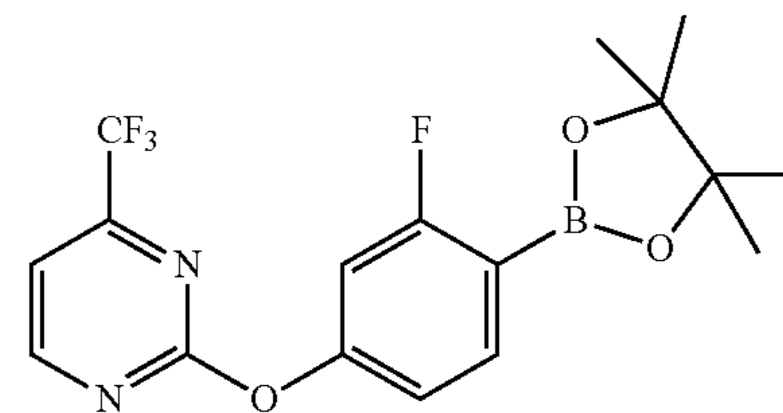
2-(3-fluoro-4-(4,4,5,5-tetramethyl-1,3,2-dioxaborolan-2-yl)phenoxy)-4-(trifluoromethyl)pyrimidine
