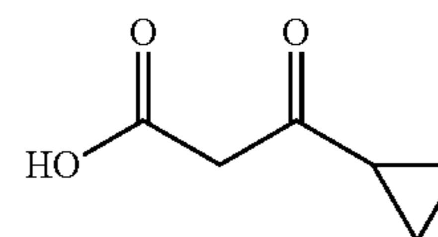
3-cyclopropyl-3-oxopropanoic Acid
