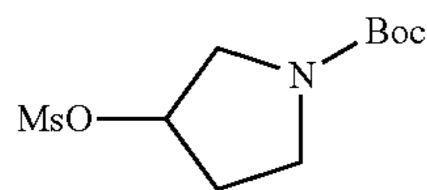
tert-butyl 3-(methylsulfonyloxy)pyrrolidine-1-carboxylate
