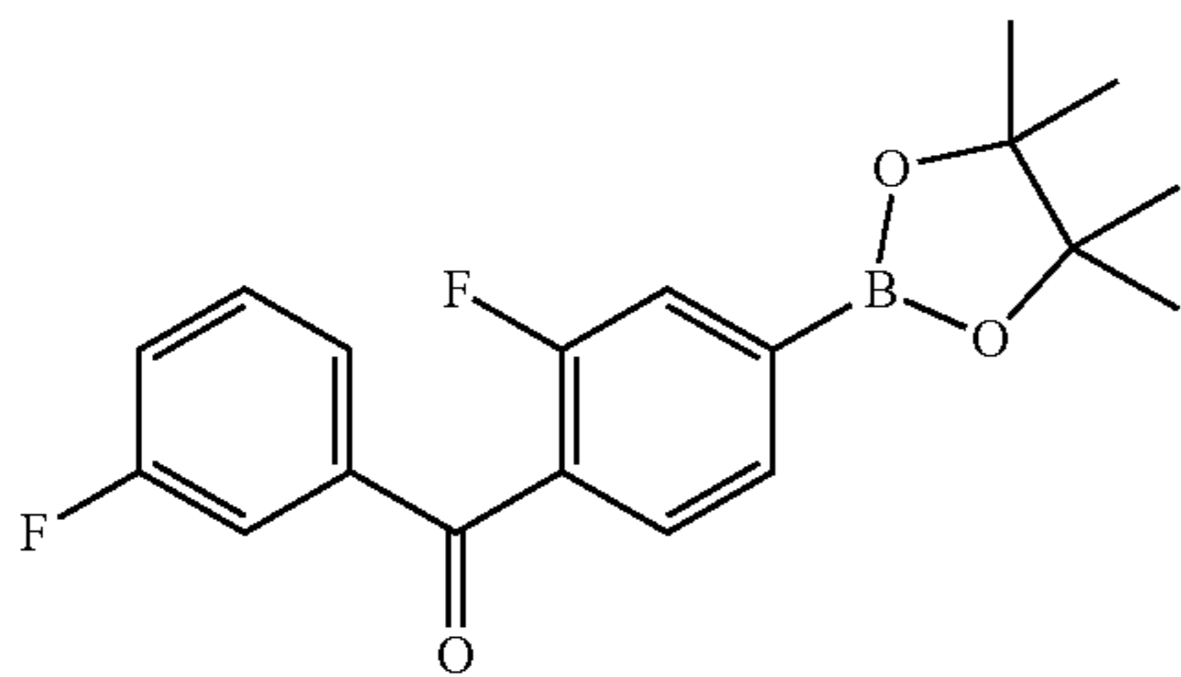
(2-fluoro-4-(4,4,5,5-tetramethyl-1,3,2-dioxaborolan-2-yl)phenyl)(3-fluorophenyl)methanone
