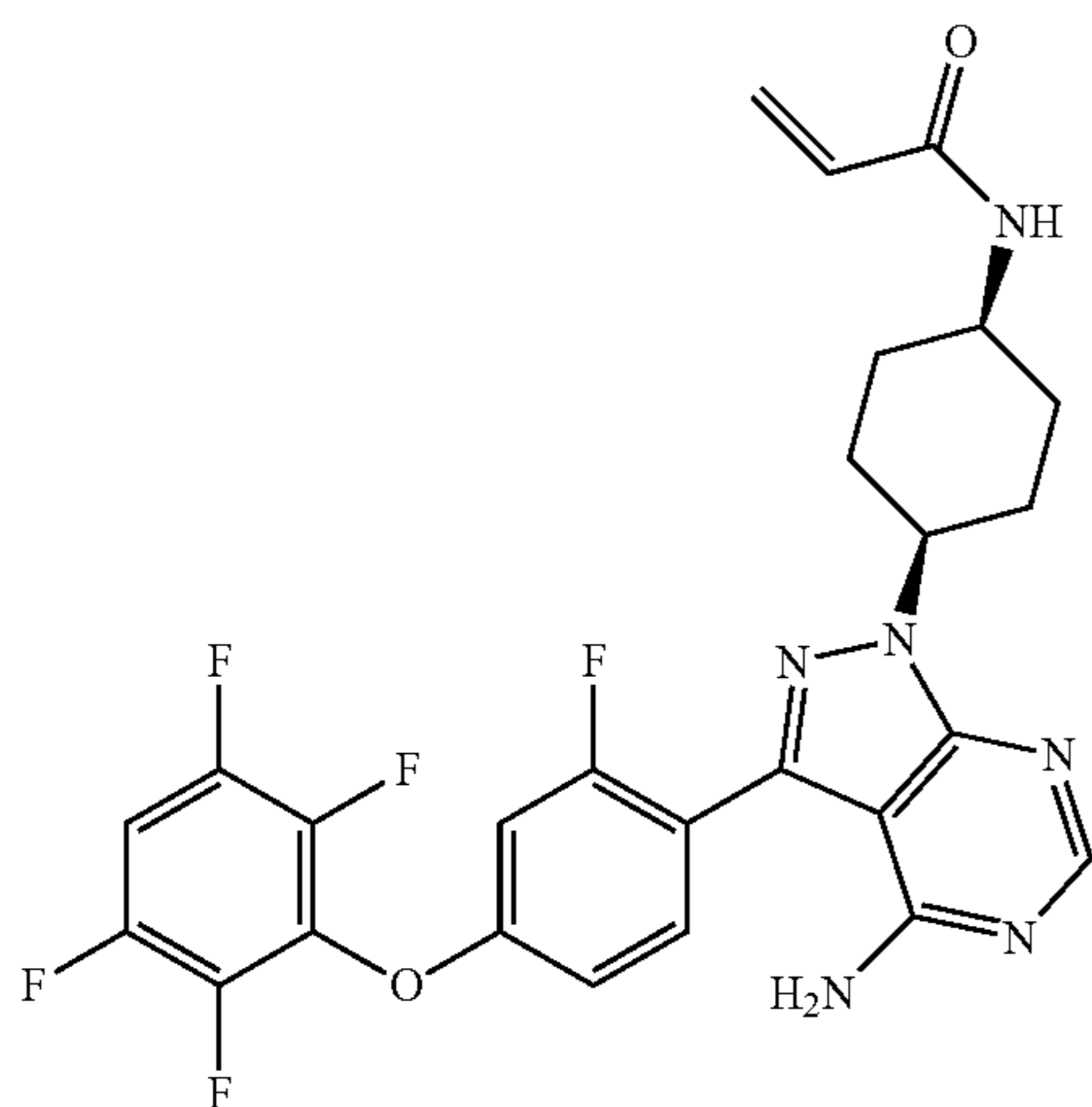
N-((1s,4s)-4-(4-amino-3-(2-fluoro-4-(2,3,5,6-tetrafluorophenoxy)phenyl)-1H-pyrazolo[3,4-d]pyrimidin-1-yl)cyclohexyl)acrylamide
