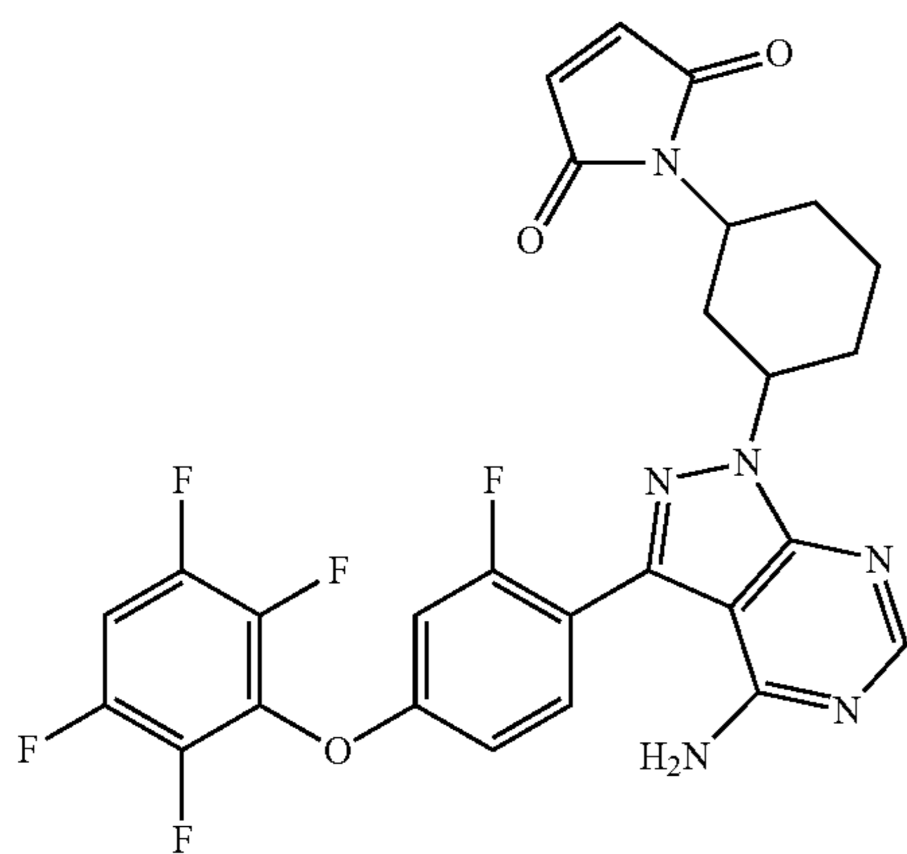
1-(3-(4-amino-3-(2-fluoro-4-(2,3,5,6-tetrafluorophenoxy)phenyl)-1H-pyrazolo[3,4-d]pyrimidin-1-yl)cyclohexyl)-1H-pyrrole-2,5-dione
