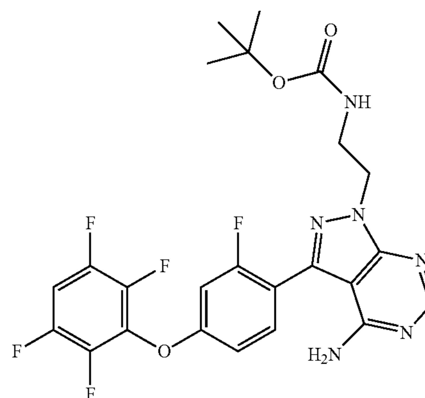
tert-butyl 2-(4-amino-3-(2-fluoro-4-(2,3,5,6-tetrafluorophenoxy)phenyl)-1H-pyrazolo[3,4-d]pyrimidin-1-yl)ethylcarbamate
