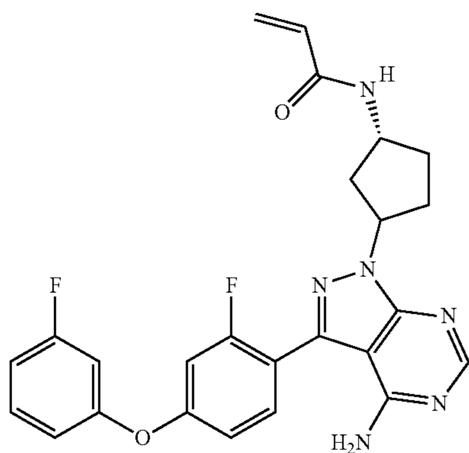
N-((1r,3r)-3-(4-amino-3-(2-fluoro-4-(3-fluorophenoxy)phenyl)-1H-pyrazolo[3,4-d]pyrimidin-1-yl)cyclopentyl)acrylamide
