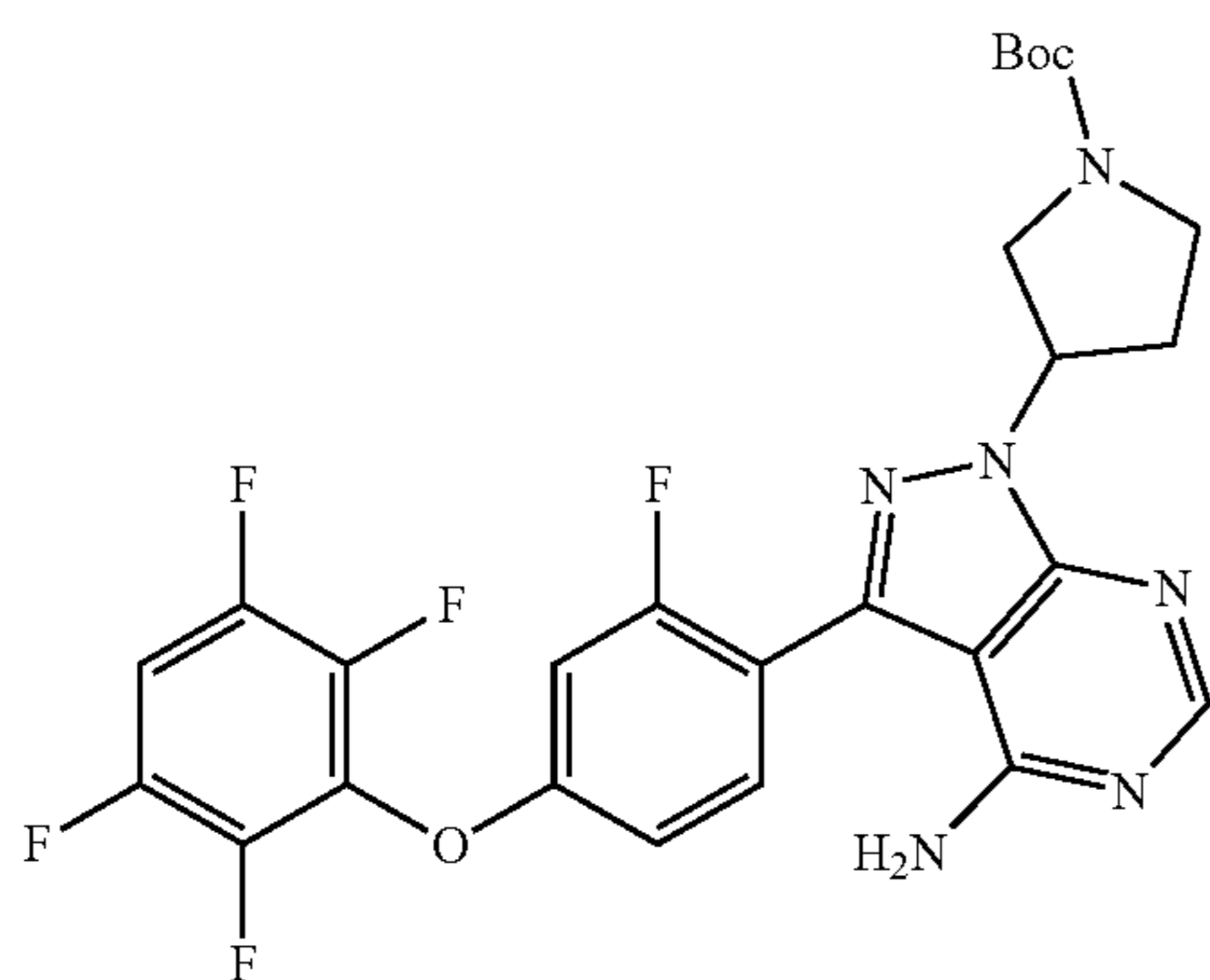
tert-butyl 3-(4-amino-3-(2-fluoro-4-(2,3,5,6-tetrafluorophenoxy)phenyl)-1H-pyrazolo[3,4-d]pyrimidin-1-yl)pyrrolidine-1-carboxylate
