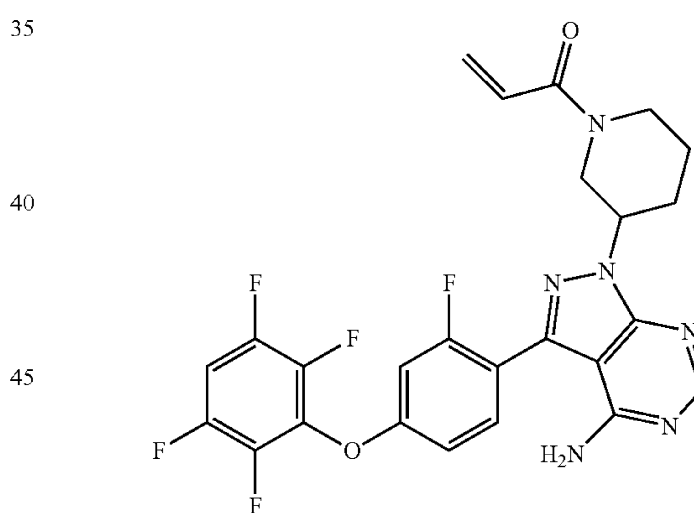
1-(3-(4-amino-3-(2-fluoro-4-(2,3,5,6-tetrafluorophenoxy)phenyl)-1H-pyrazolo[3,4-d]pyrimidin-1-yl)piperidin-1-yl)prop-2-en-1-one
