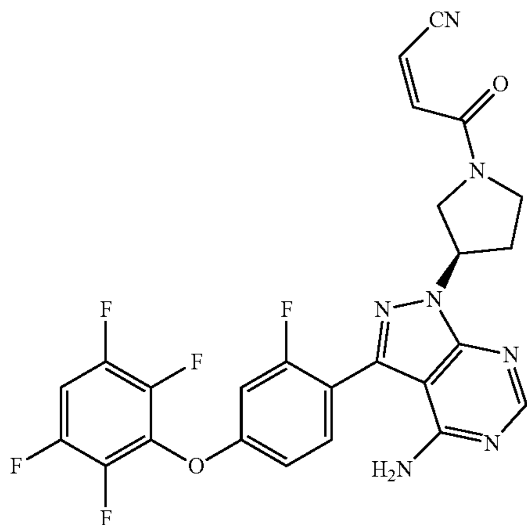
(Z)-4-((R)-3-(4-amino-3-(2-fluoro-4-(2,3,5,6-tetrafluorophenoxy)phenyl)-1H-pyrazolo[3,4-d]pyrimidin-1-yl)pyrrolidin-1-yl)-4-oxobut-2-enenitrile
