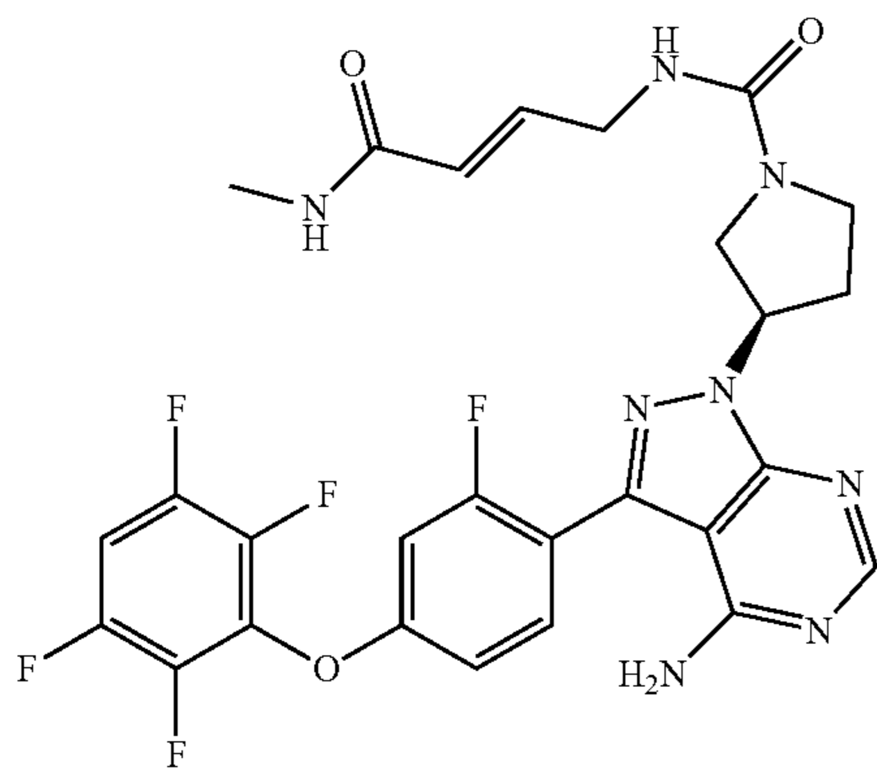
(3R)-3-(4-amino-3-(2-fluoro-4-(2,3,5,6-tetrafluorophenoxy)phenyl)-1H-pyrazolo[3,4-d]pyrimidin-1-yl)-N-(4-(methylamino)-4-oxobut-2-enyl)pyrrolidine-1-carboxamide
