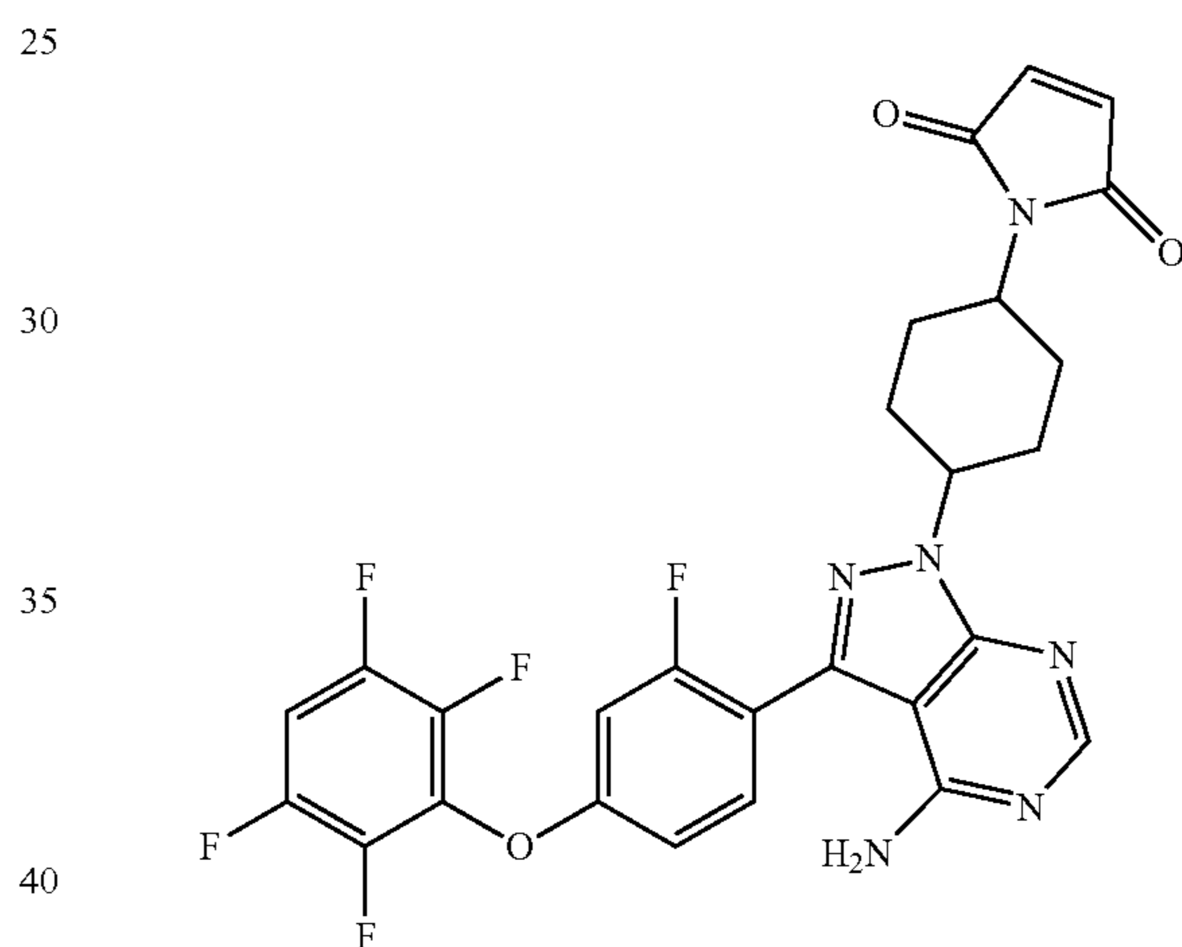
1-(4-(4-amino-3-(2-fluoro-4-(2,3,5,6-tetrafluorophenoxy)phenyl)-1H-pyrazolo[3,4-d]pyrimidin-1-yl)cyclohexyl)-1H-pyrrole-2,5-dione
