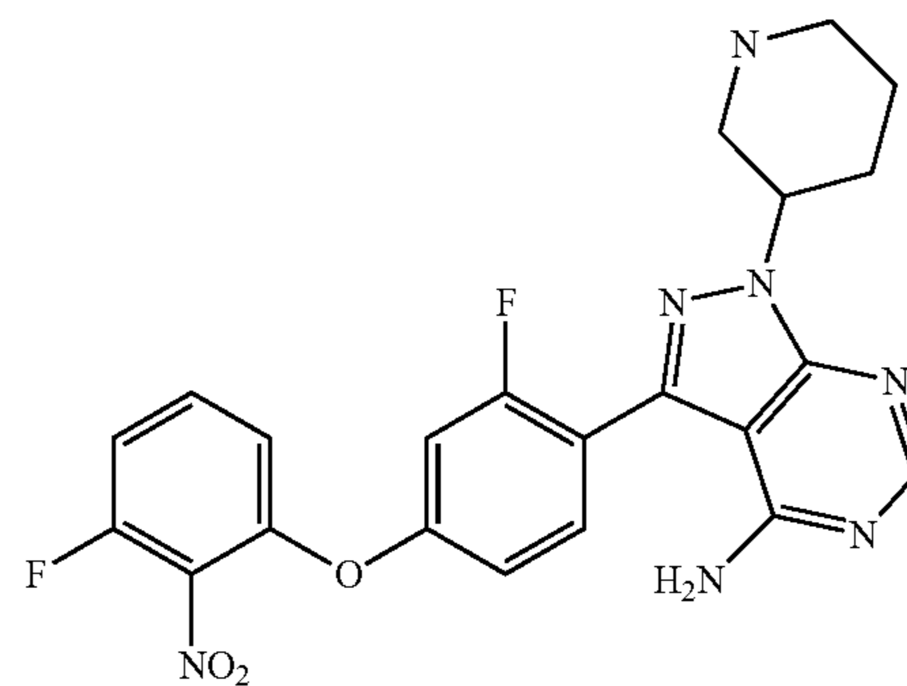
3-(2-fluoro-4-(3-fluoro-2-nitro phenoxy)phenyl)-1-(piperidin-3-yl)-1H-pyrazolo[3,4-d]pyrimidin-4-amine
