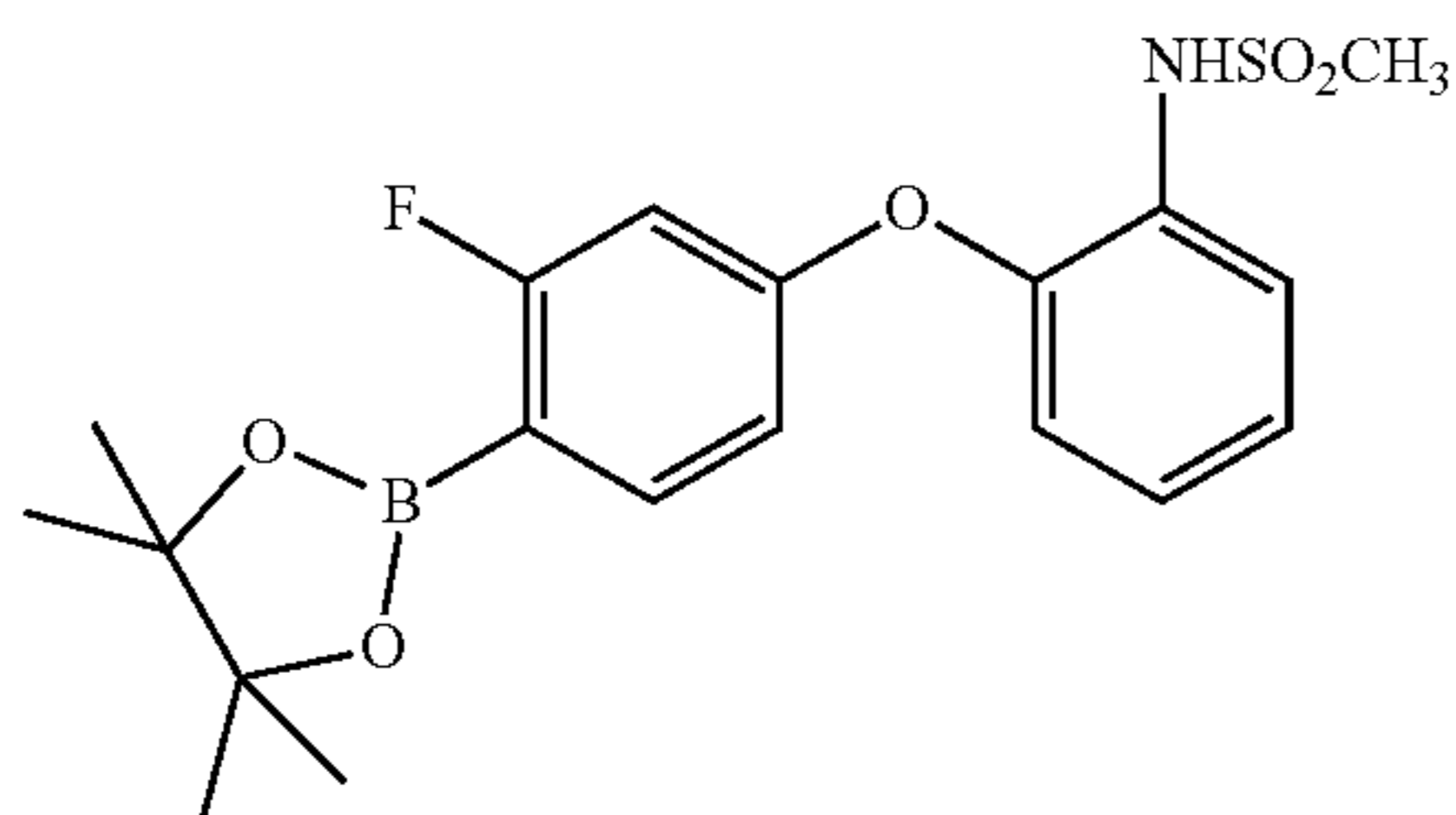
N-(2-(3-fluoro-4-(4,4,5,5-tetramethyl-1,3,2-dioxaborolan-2-yl)phenoxy)phenyl)methanesulfonamide
