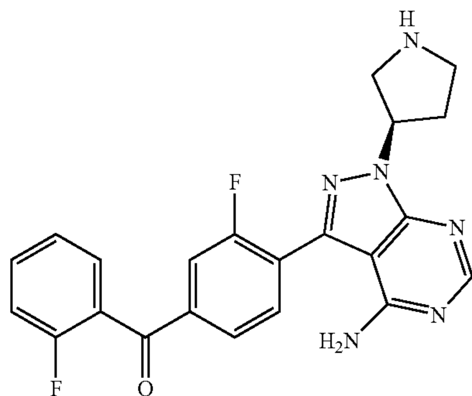
(4-(4-amino-1-((R)-pyrrolidin-3-yl)-1H-pyrazolo[3,4-d]pyrimidin-3-yl)-3-fluorophenyl)(2-fluorophenyl) methanone
