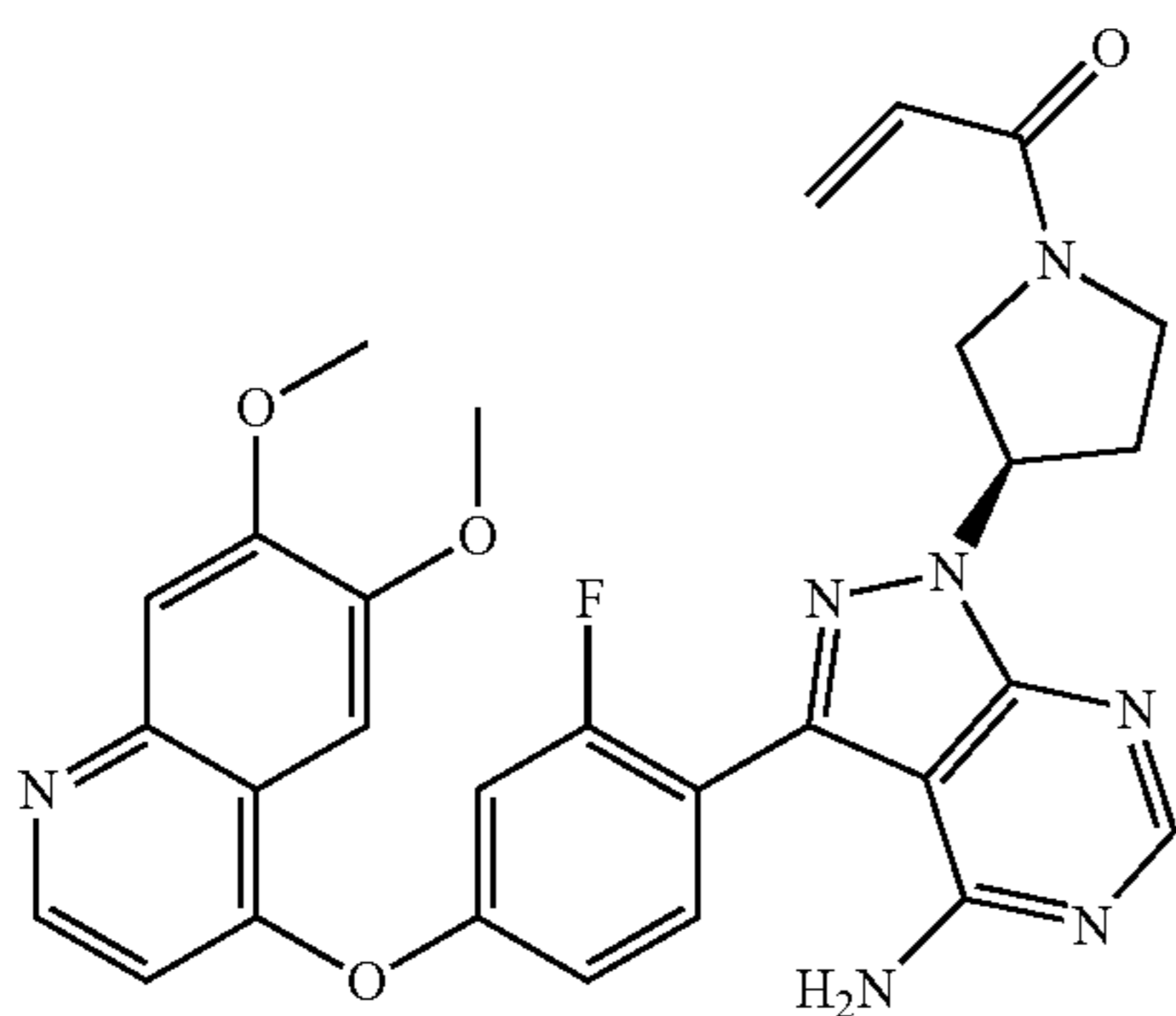
1-((R)-3-(4-amino-3-(4-(6,7-dimethoxyquinolin-4-yloxy)-2-fluorophenyl)-1H-pyrazolo[3,4-d]pyrimidin-1-yl)pyrrolidin-1-yl)prop-2-en-1-one
