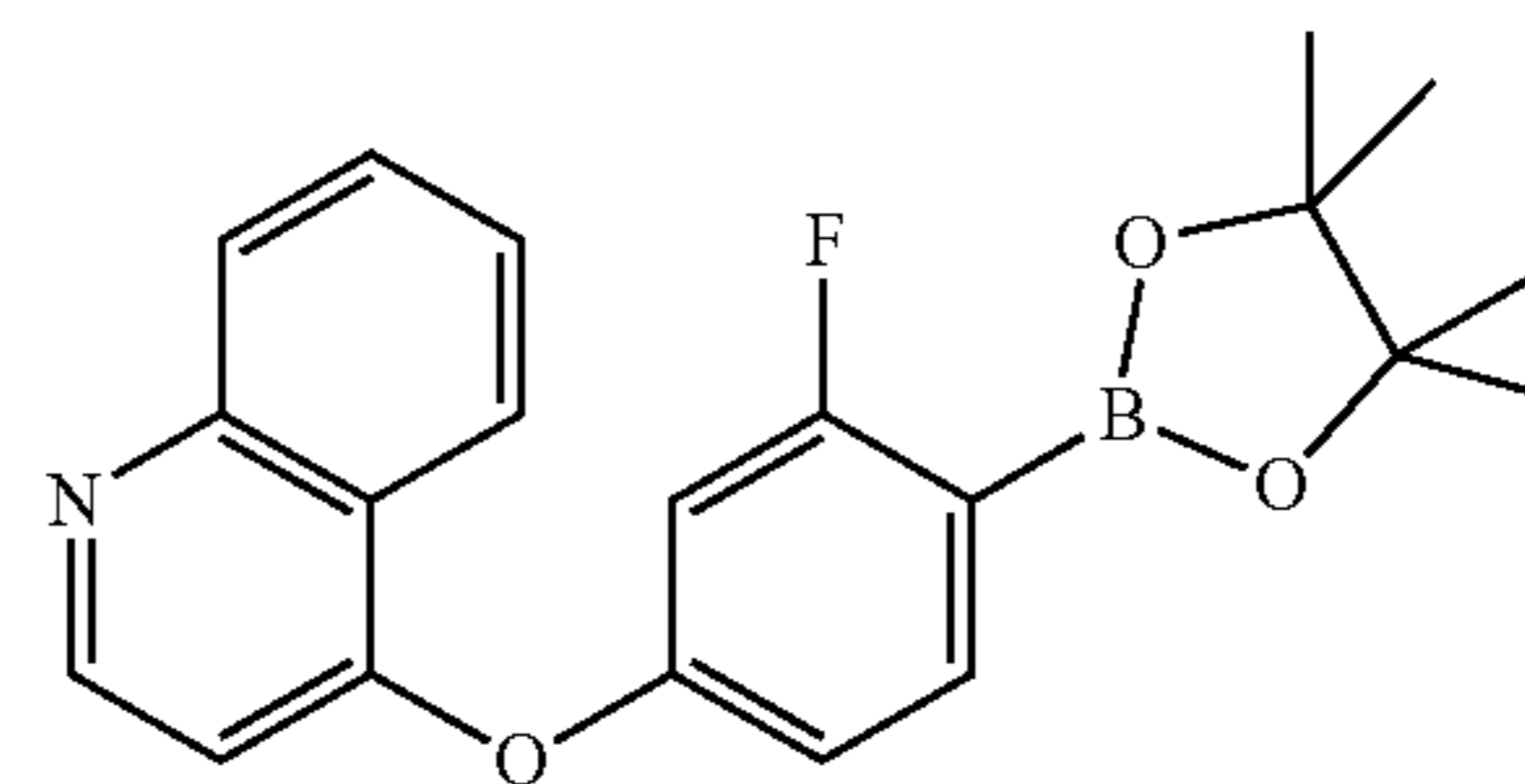
4-(3-fluoro-4-(4,4,5,5-tetramethyl-1,3,2-dioxaborolan-2-yl)phenoxy)quinoline
