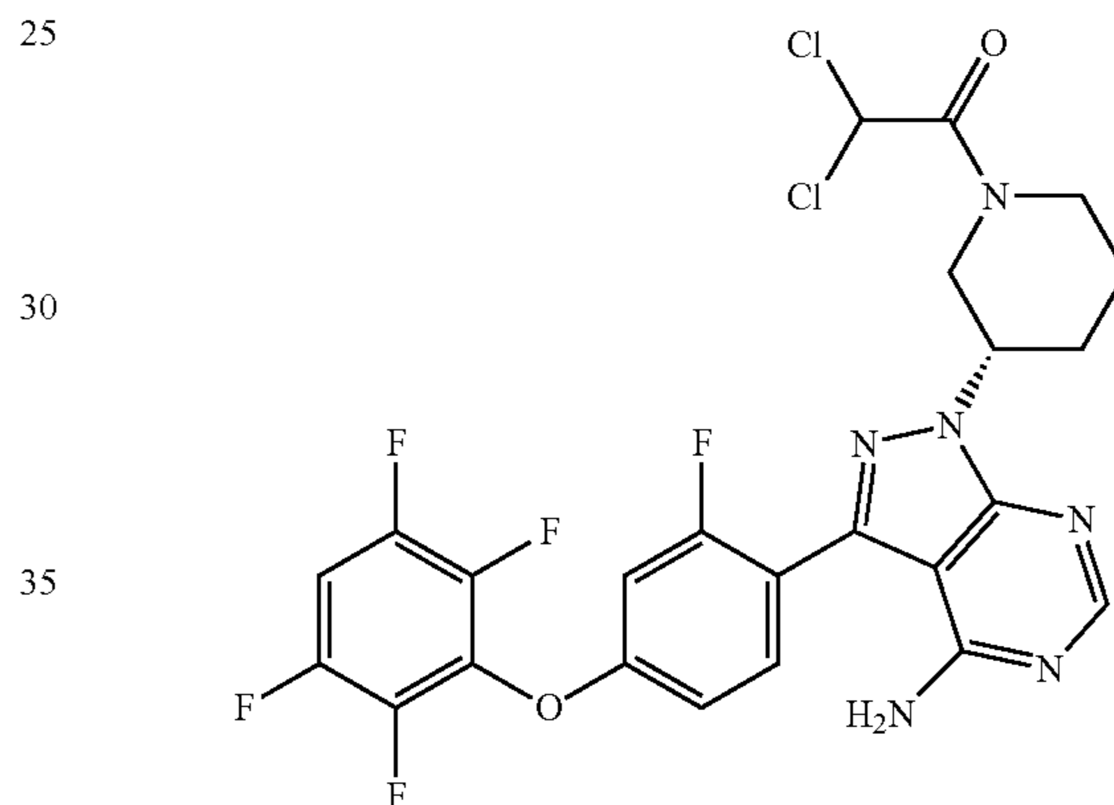
1-((S)-3-(4-amino-3-(2-fluoro-4-(2,3,5,6-tetrafluorophenoxy)phenyl)-1H-pyrazolo[3,4-d]pyrimidin-1-yl)piperidin-1-yl)-2,2-dichloroethanone
