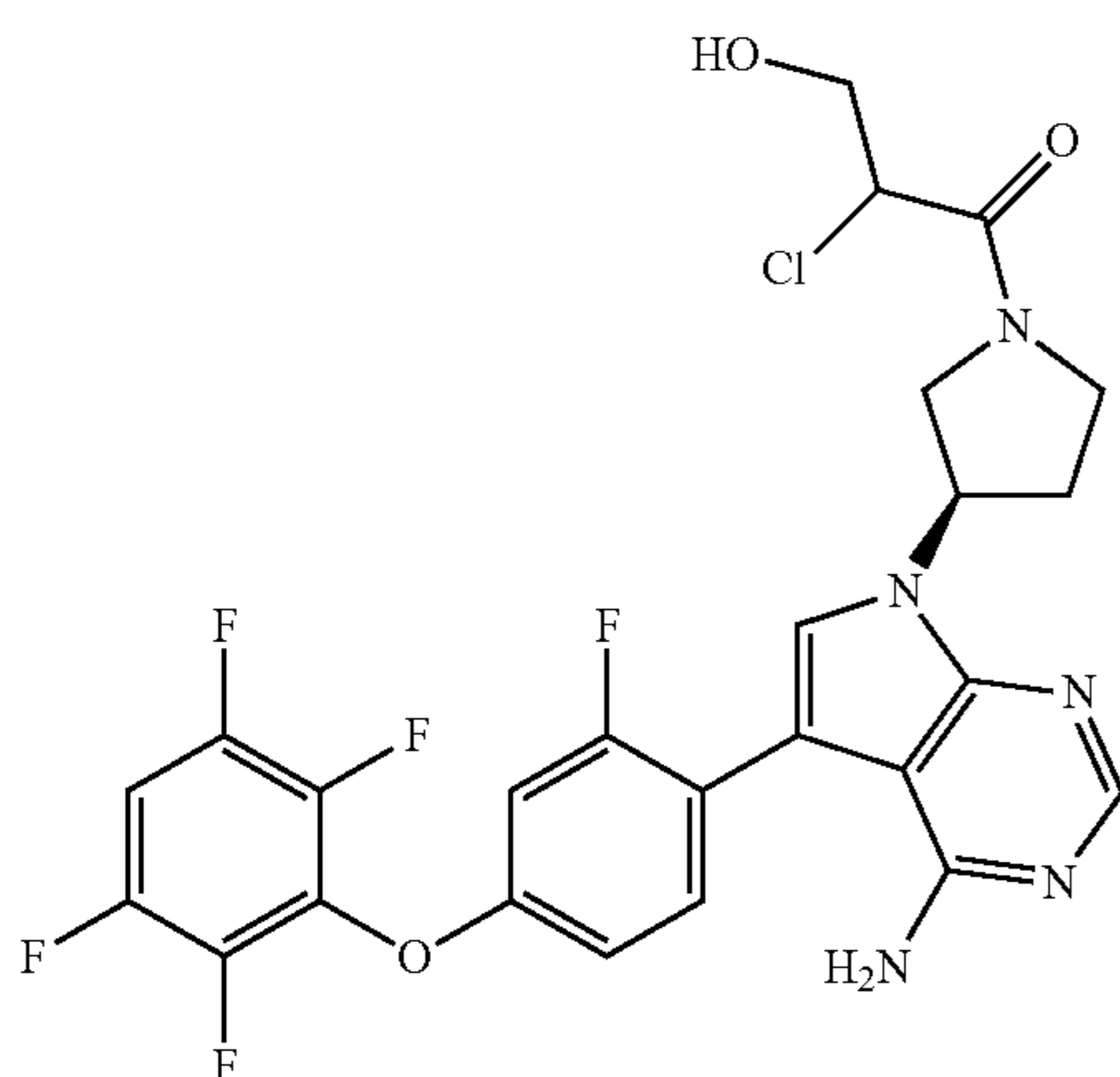
1-((R)-3-(4-amino-3-(2-fluoro-4-(2,3,5,6-tetrafluorophenoxy)phenyl)-1H-pyrrolo[2,3-d]pyrimidin-1-yl)pyrrolidin-1-yl)-2-chloro-3-hydroxypropan-1-one
