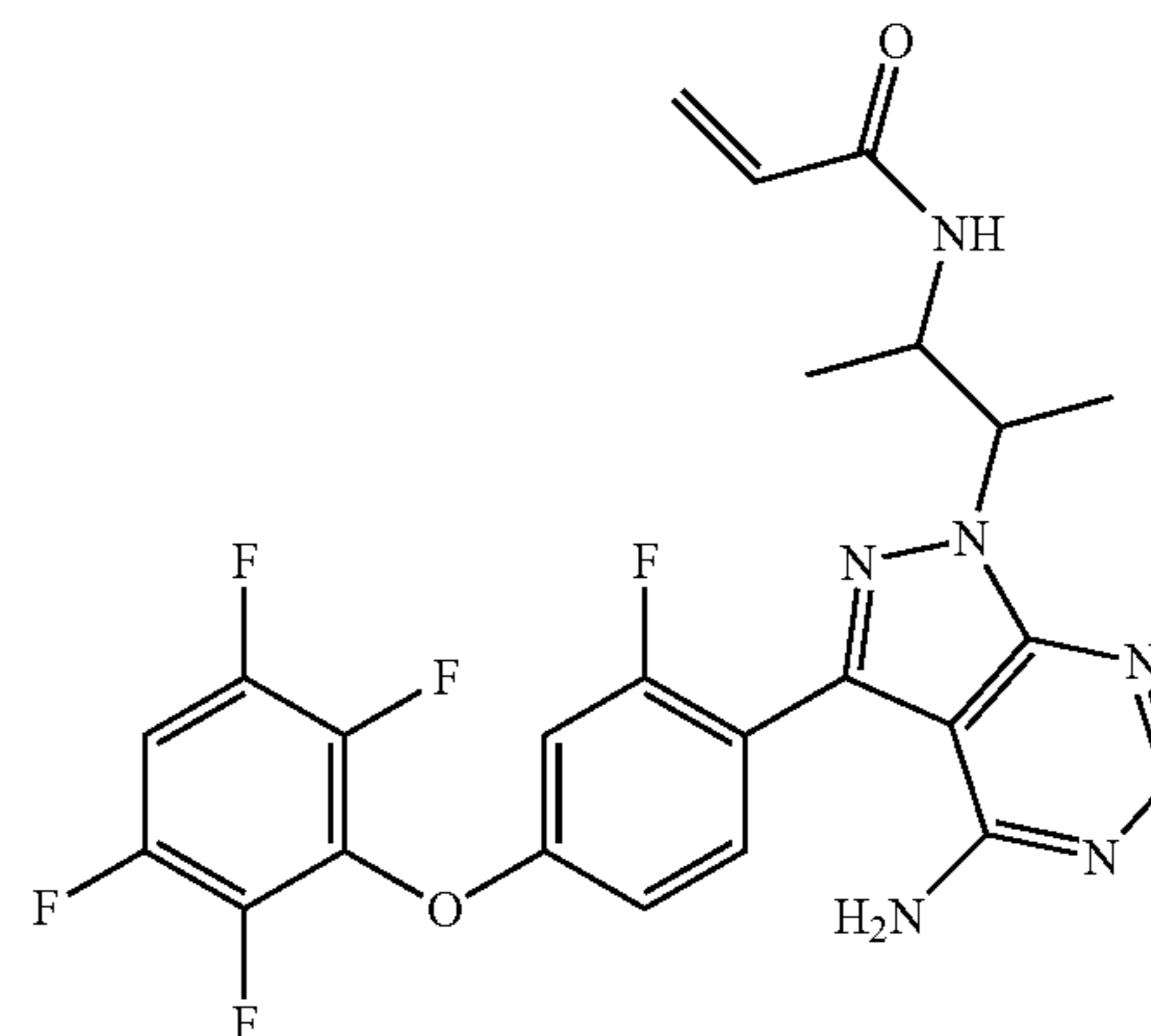
N-(3-(4-amino-3-(2-fluoro-4-(2,3,5,6-tetrafluorophenoxy)phenyl)-1H-pyrazolo[3,4-d]pyrimidin-1-yl)butan-2-yl)acrylamide
