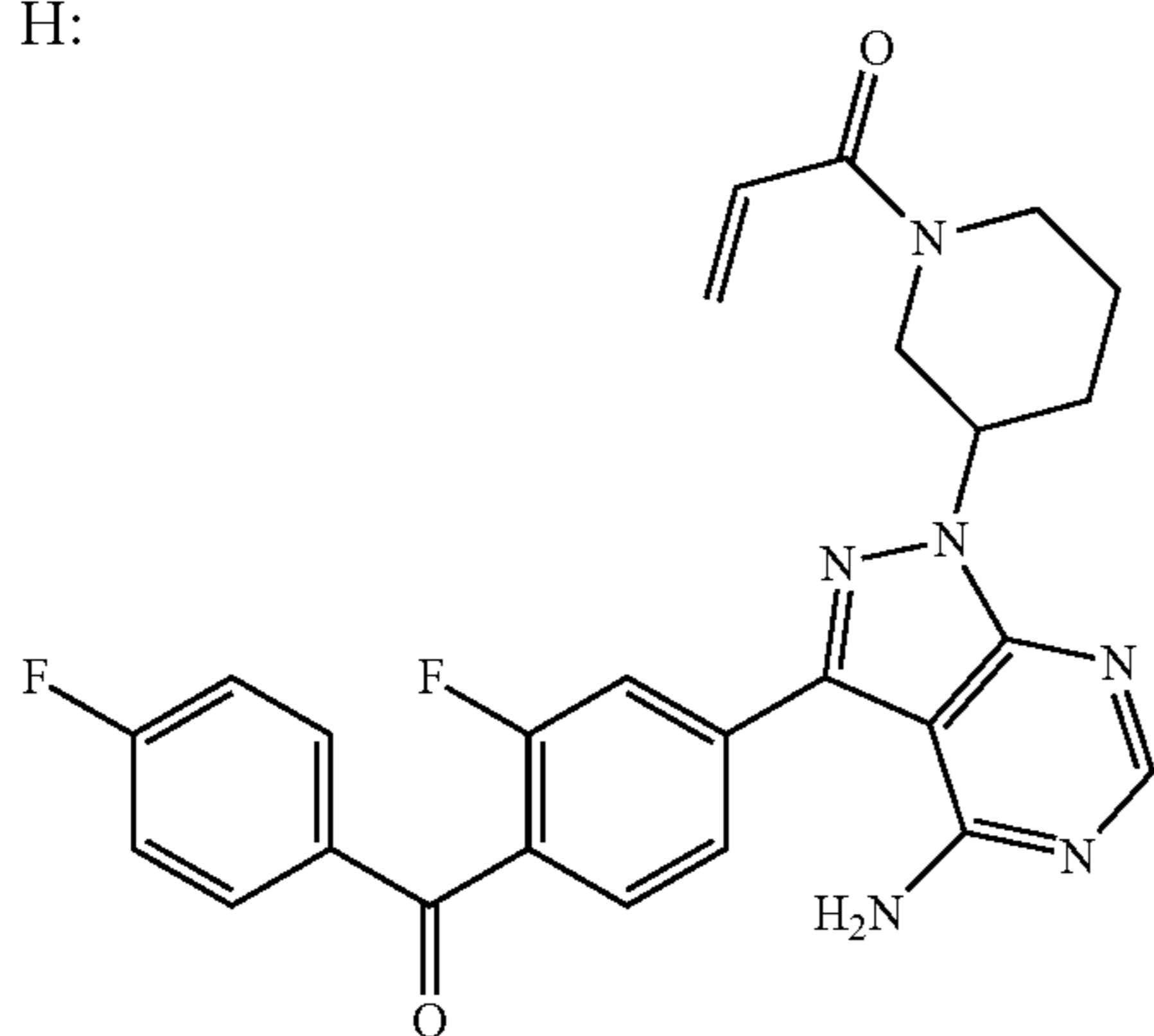
1-(3-(4-amino-3-(3-fluoro-4-(4-fluorobenzoyl)phenyl)-1H-pyrazolo[3,4-d]pyrimidin-1-yl)piperidin-1-yl)prop-2-en-1-one
