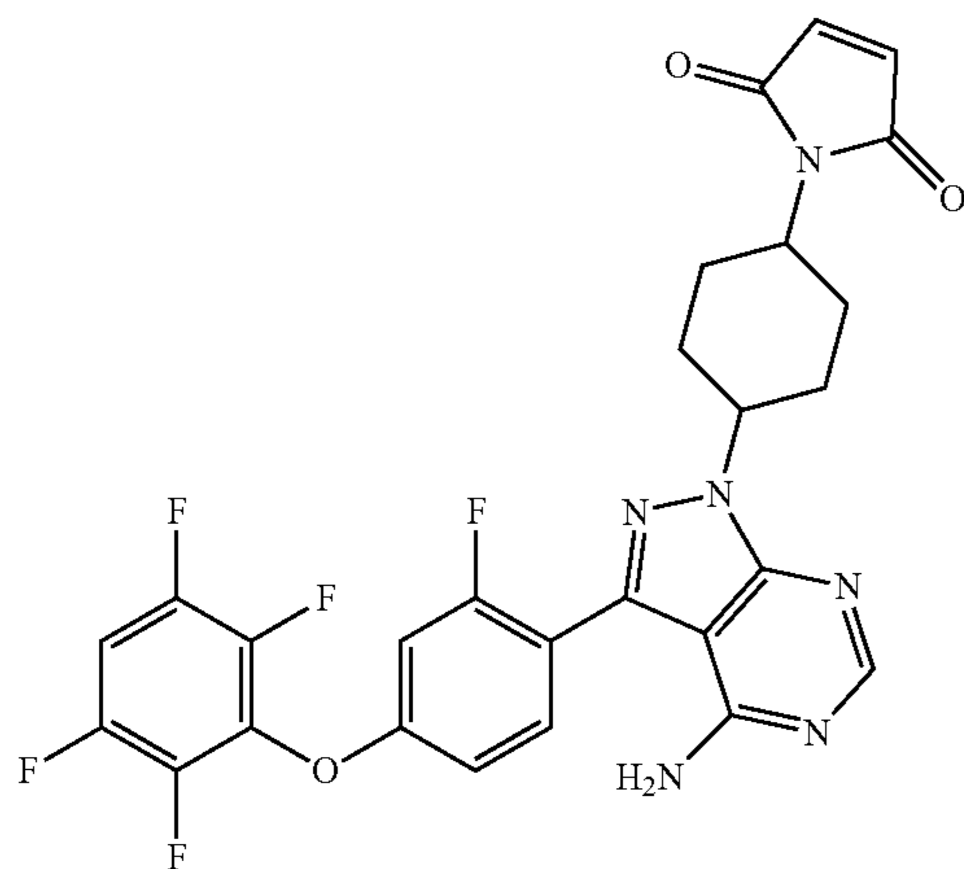
1-(4-(4-amino-3-(2-fluoro-4-(2,3,5,6-tetrafluorophenoxy)phenyl)-1H-pyrazolo[3,4-d]pyrimidin-1-yl)cyclohexyl)-1H-pyrrole-2,5-dione
