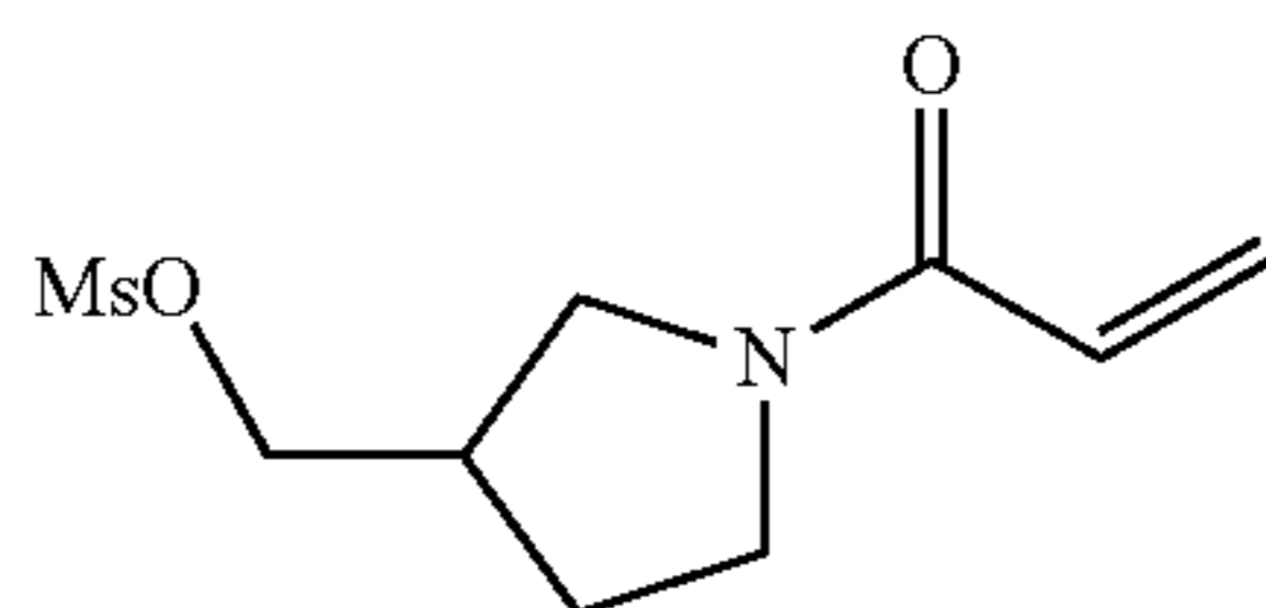
(1-acryloylpyrrolidin-3-yl)methyl methanesulfonate
