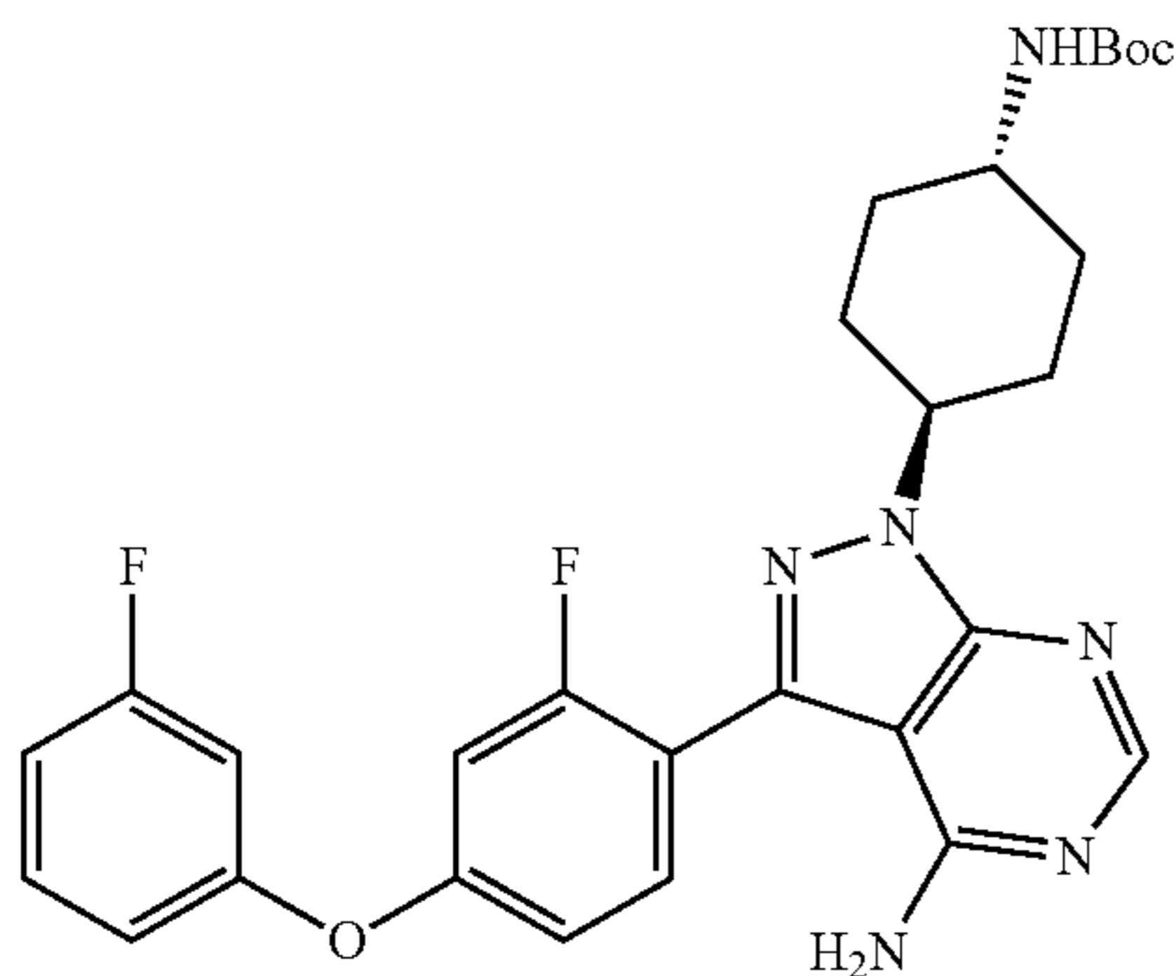
tert-butyl (1r,4r)-4-(4-amino-3-(2-fluoro-4-(3-fluorophenoxy)phenyl)-1H-pyrazolo[3,4-d]pyrimidin-1-yl)cyclohexylcarbamate
