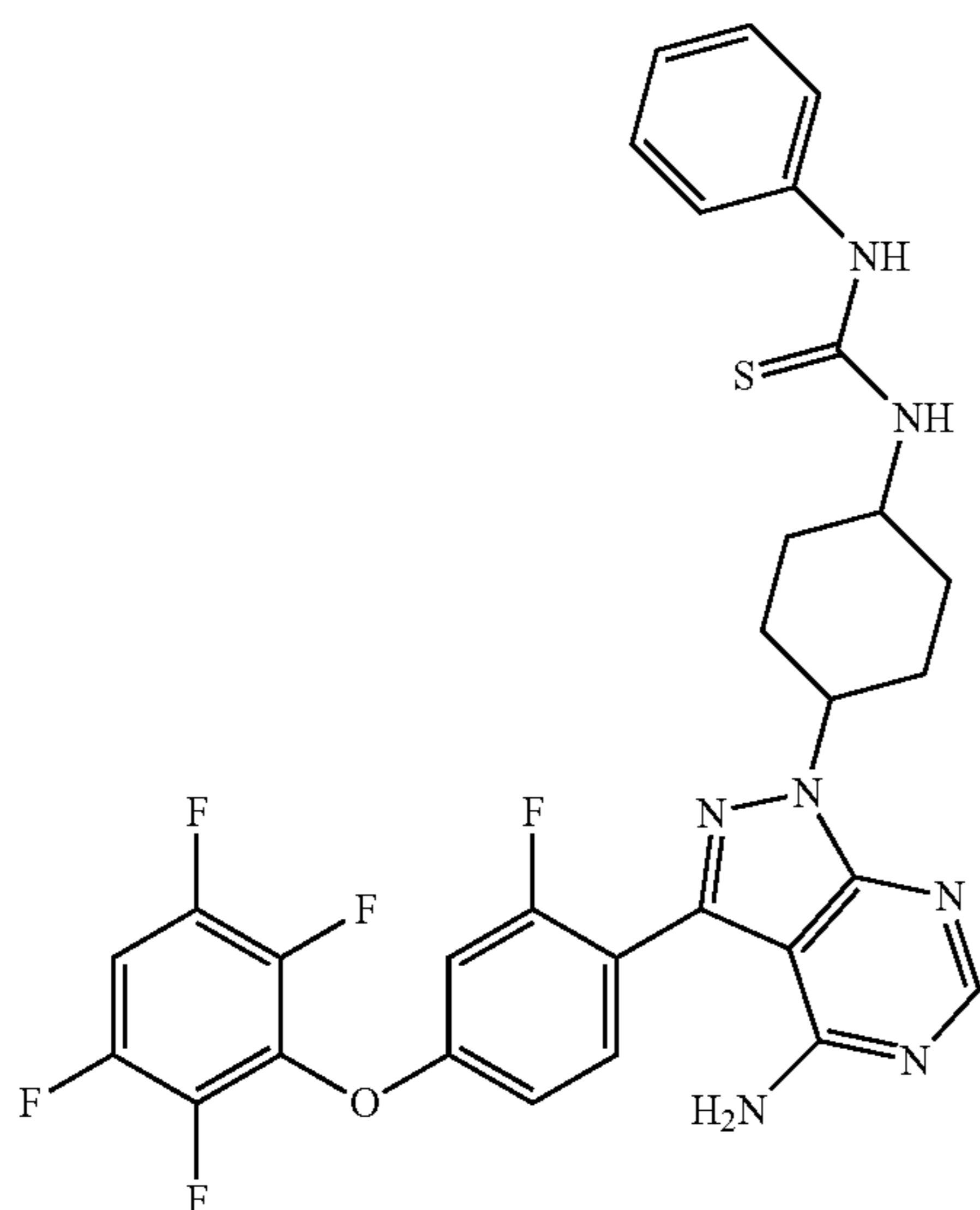
1-(4-(4-amino-3-(2-fluoro-4-(2,3,5,6-tetrafluorophenoxy)phenyl)-1H-pyrazolo[3,4-d]pyrimidin-1-yl)cyclohexyl)-3-phenylthiourea
