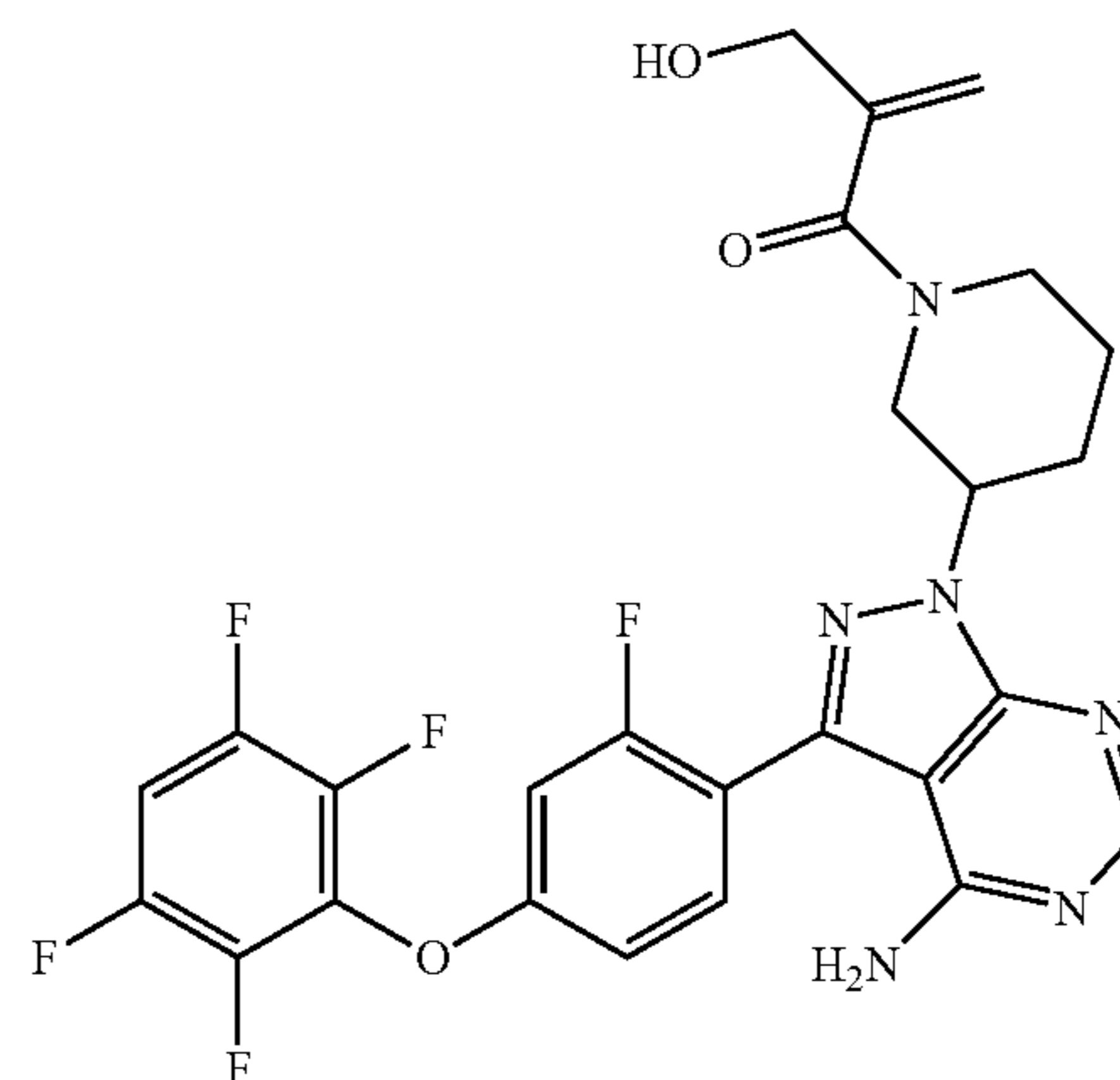
1-(3-(4-amino-3-(2-fluoro-4-(2,3,5,6-tetrafluorophenoxy)phenyl)-1H-pyrazolo[3,4-d]pyrimidin-1-yl)piperidin-1-yl)-2-(hydroxymethyl)prop-2-en-1-one
