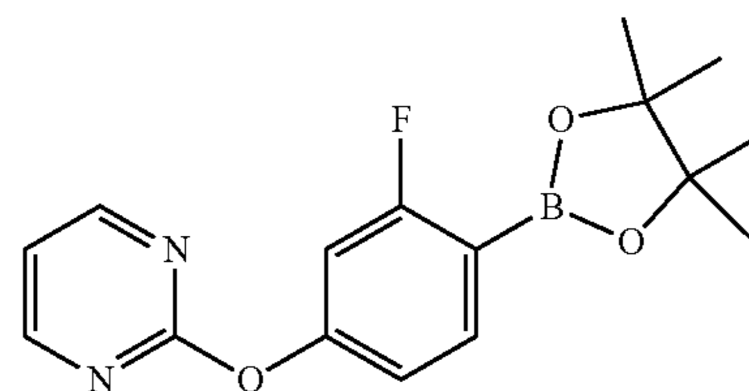
2-(3-fluoro-4-(4,4,5,5-tetramethyl-1,3,2-dioxaborolan-2-yl)phenoxy)pyrimidine
