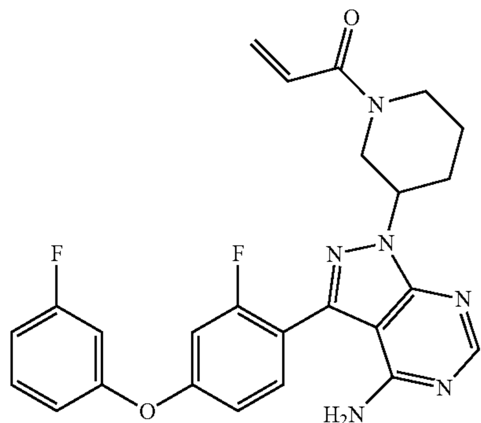
1-(3-(4-amino-3-(2-fluoro-4-(3-fluorophenoxy)phenyl)-1H-pyrazolo[3,4-d]pyrimidin-1-yl)piperidin-1-yl)prop-2-en-1-one
