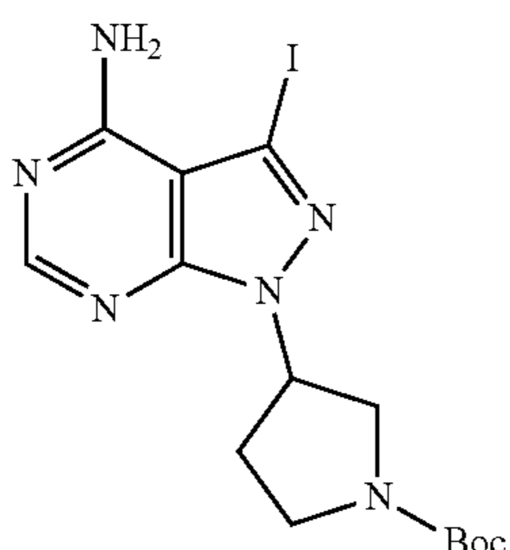
tert-butyl 3-(4-amino-3-iodo-1H-pyrazolo[3,4-d]pyrimidin-1-yl)pyrrolidine-1-carboxylate
