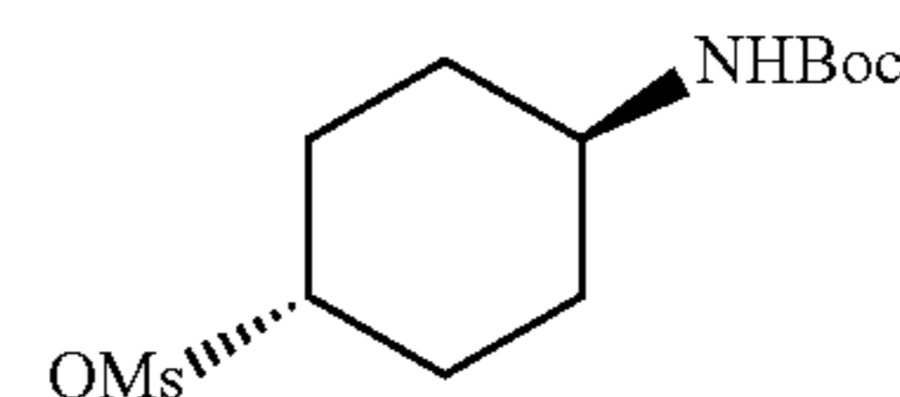
(1r,4r)-4-(tert-butoxycarbonyl)cyclohexyl methanesulfonate
