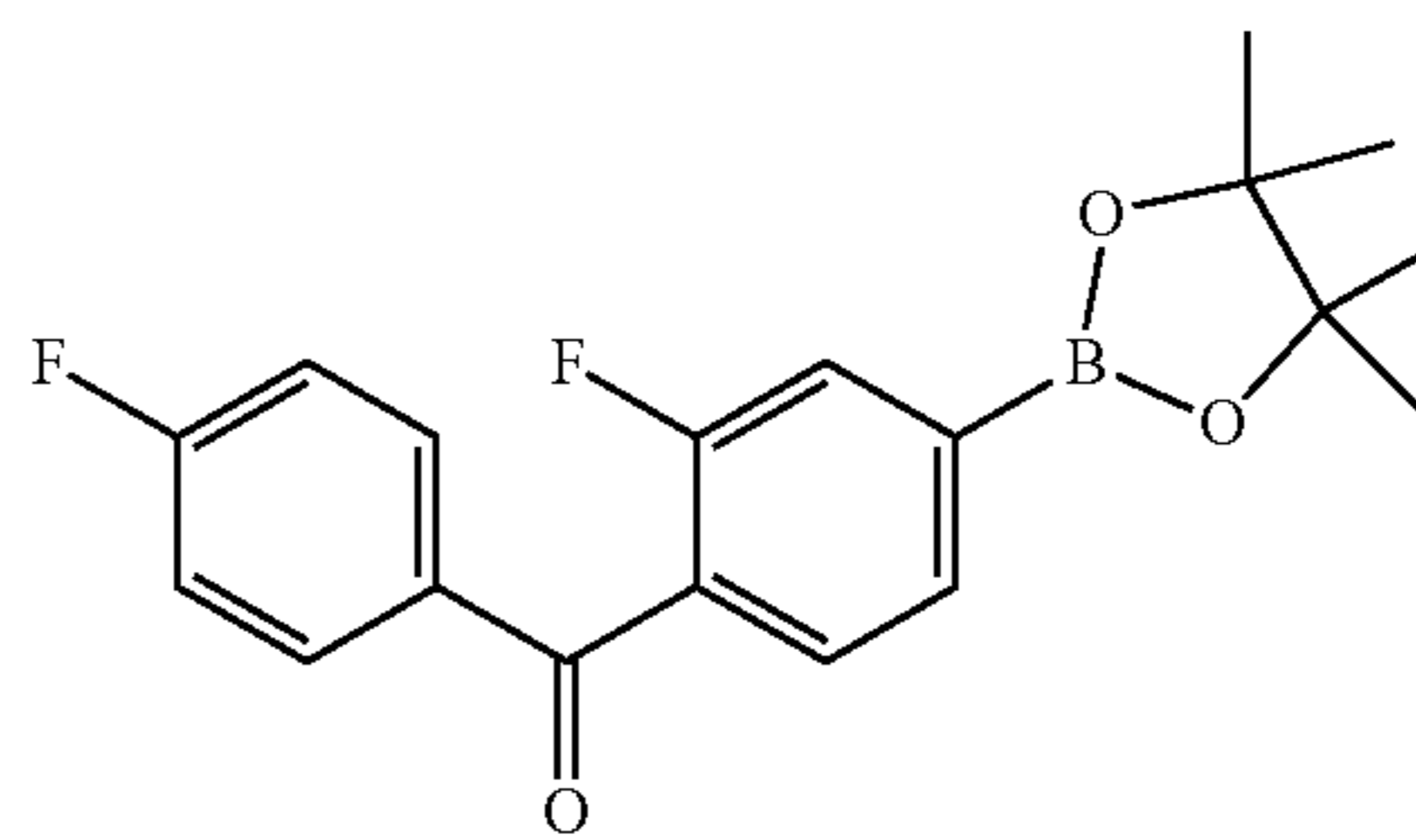
(2-fluoro-4-(4,4,5,5-tetramethyl-1,3,2-dioxaborolan-2-yl)phenyl)(4-fluorophenyl)methanone
