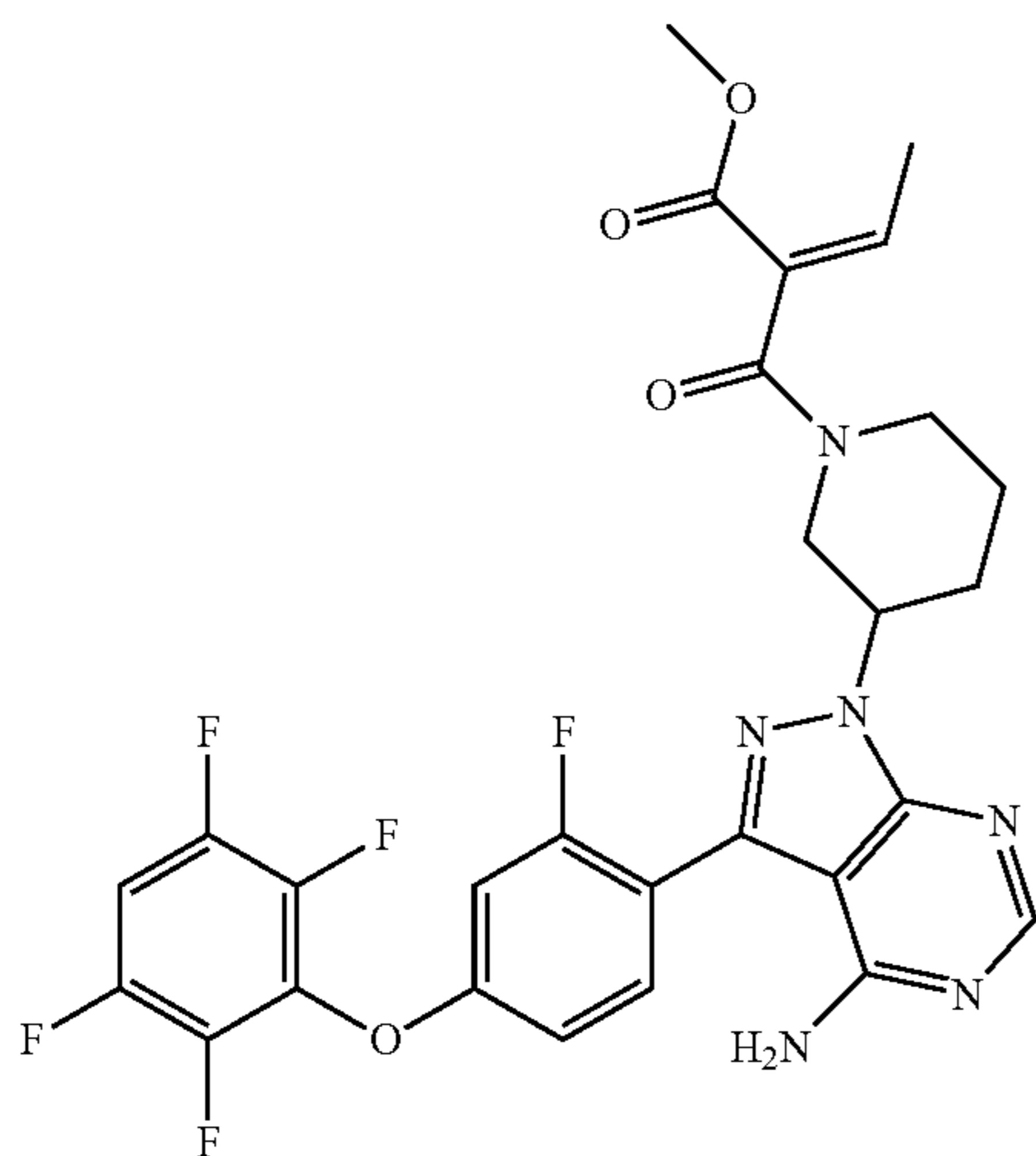
(Z)-methyl 2-(3-(4-amino-3-(2-fluoro-4-(2,3,5,6-tetrafluorophenoxy)phenyl)-1H-pyrazolo[3,4-d]pyrimidin-1-yl)piperidine-1-carbonyl)but-2-enoate
