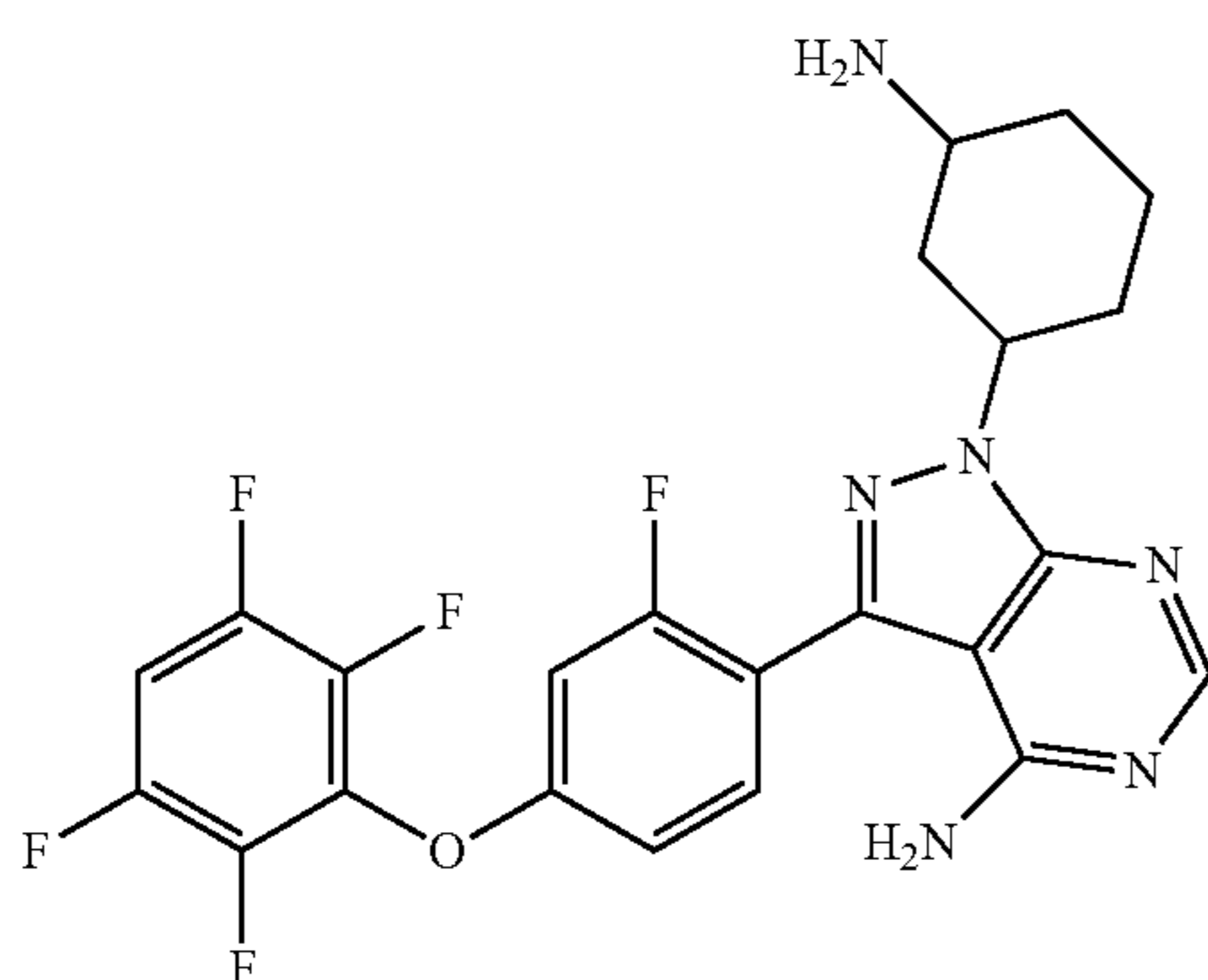
1-(3-(aminocyclohexyl)-3-(2-fluoro-4-(2,3,5,6-tetrafluorophenoxy)phenyl)-1H-pyrazolo[3,4-d]pyrimidin-4-amine
