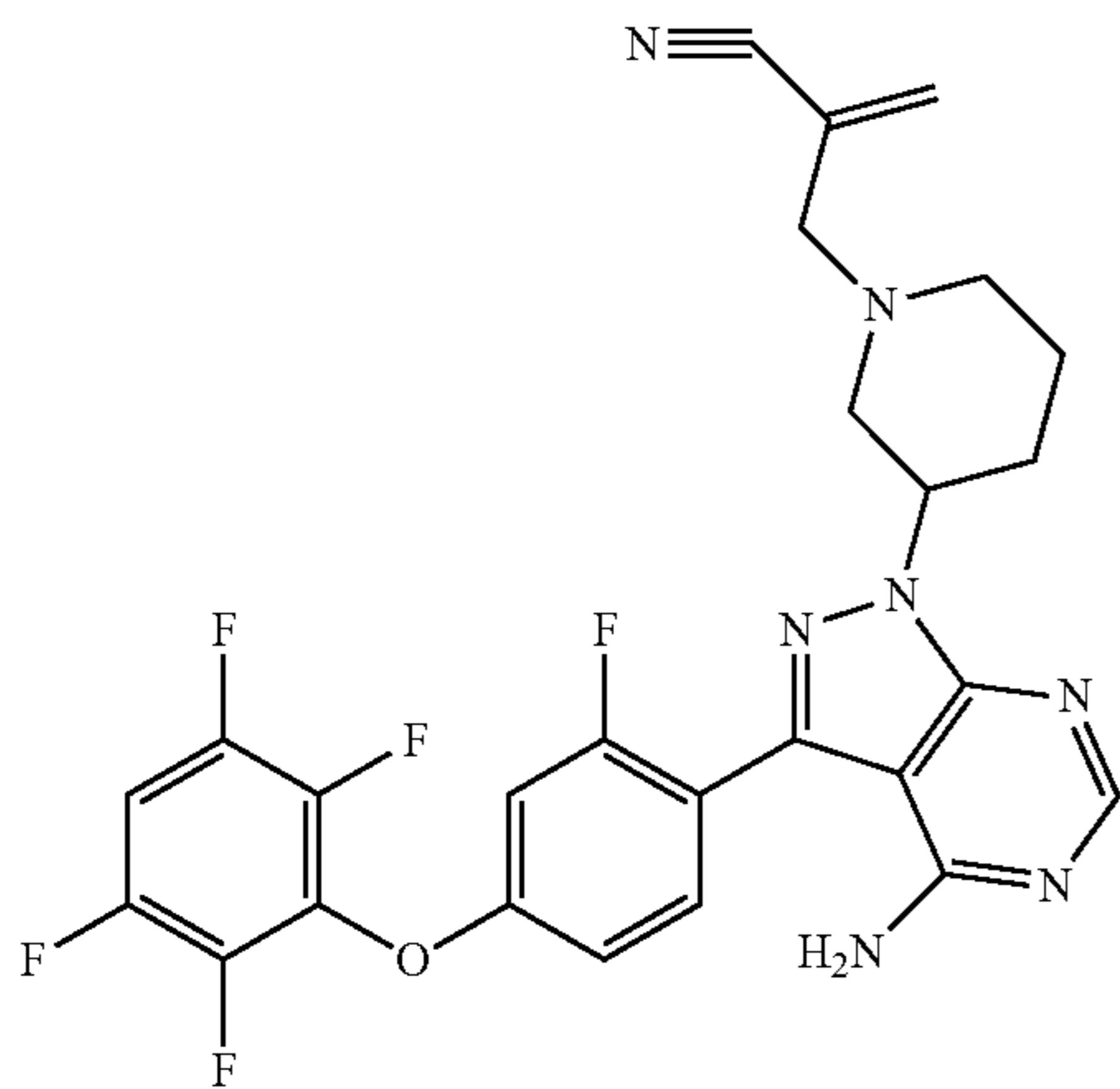
2-((3-(4-amino-3-(2-fluoro-4-(2,3,5,6-tetrafluorophenoxy)phenyl)-1H-pyrazolo[3,4-d]pyrimidin-1-yl)piperidin-1-yl)methyl)acrylonitrile
