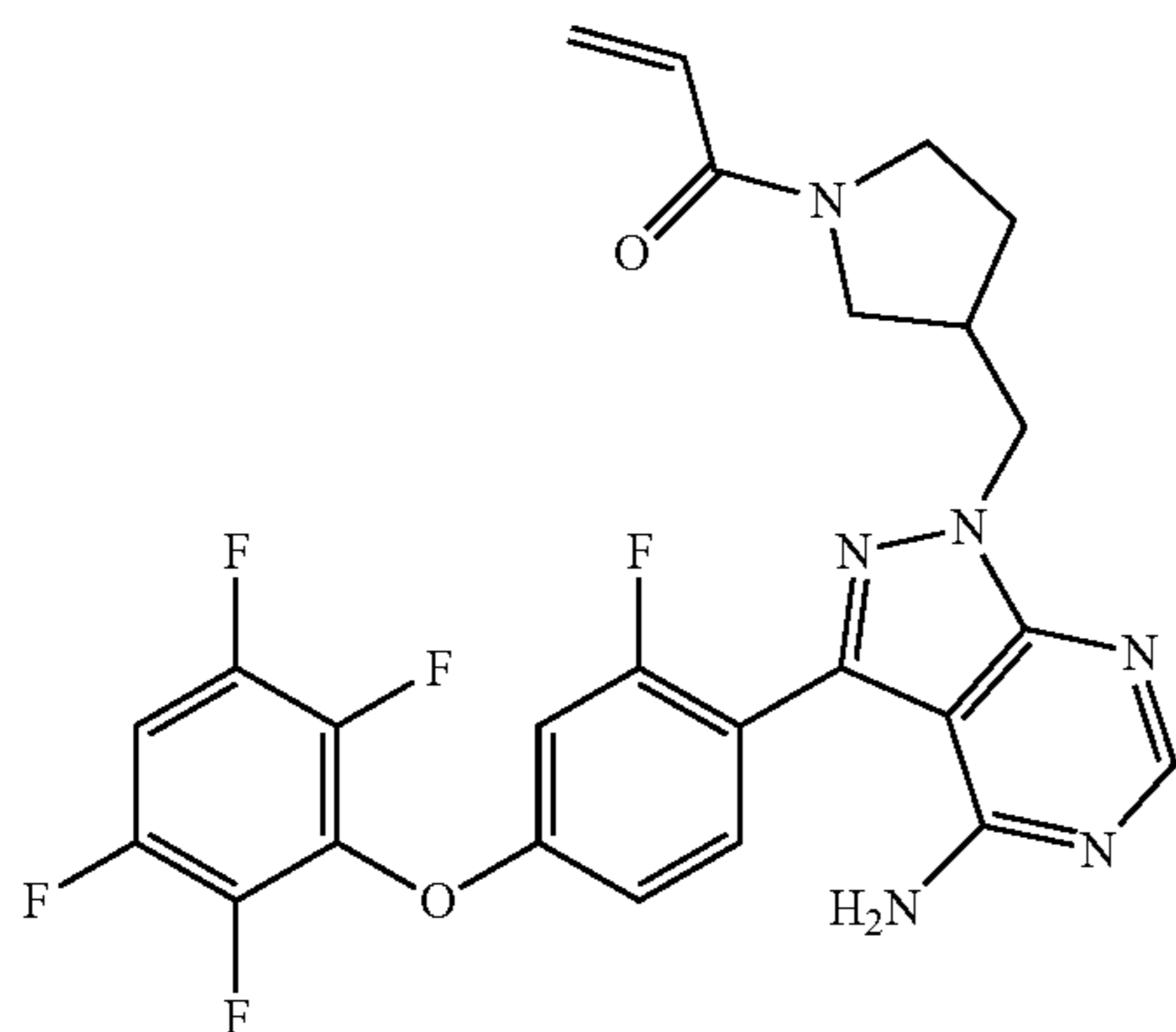
1-(3-((4-amino-3-(2-fluoro-4-(2,3,5,6-tetrafluorophenoxy)phenyl)-1H-pyrazolo[3,4-d]pyrimidin-1-yl)methyl)pyrrolidin-1-yl)prop-2-en-1-one
