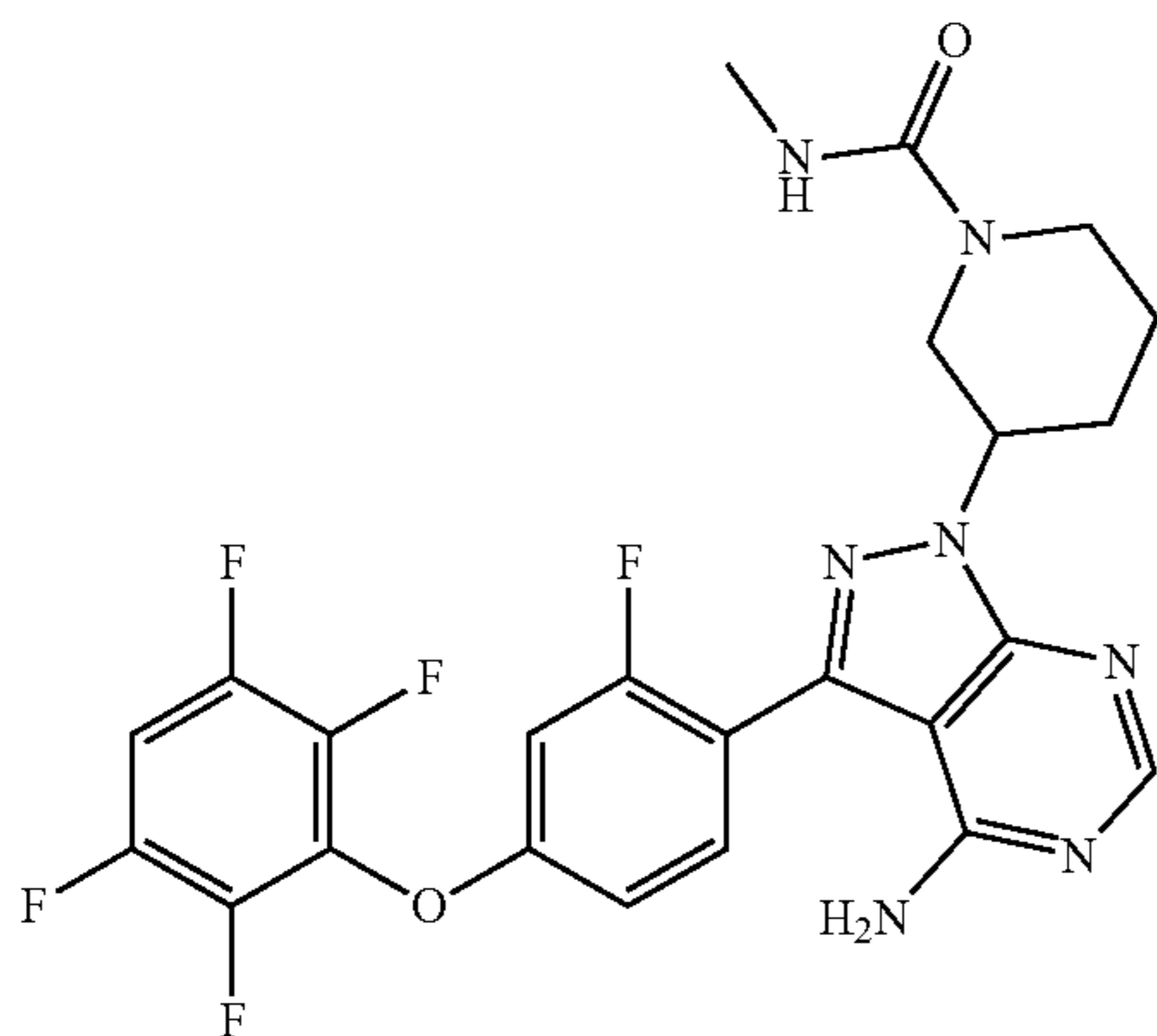
3-(4-amino-3-(2-fluoro-4-(2,3,5,6-tetrafluorophenoxy)phenyl)-1H-pyrazolo[3,4-d]pyrimidin-1-yl)-N-methylpiperidine-1-carboxamide
