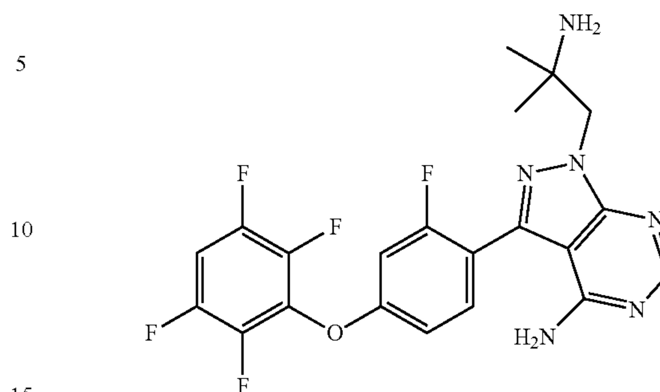
1-(2-amino-2-methylpropyl)-3-(2-fluoro-4-(2,3,5,6-tetrafluorophenoxy)phenyl)-1H-pyrazolo[3,4-d]pyrimidin-4-amine
