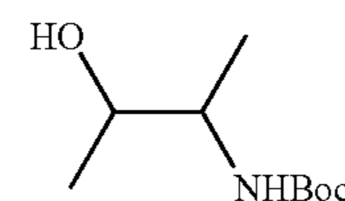
tert-butyl 3-hydroxybutan-2-ylcarbamate
