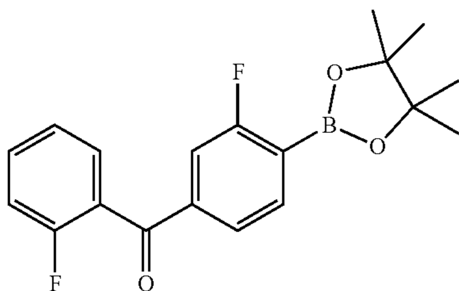
(3-fluoro-4-(4,4,5,5-tetramethyl-1,3,2-dioxaborolan-2-yl)phenyl)(2-fluorophenyl)methanone
