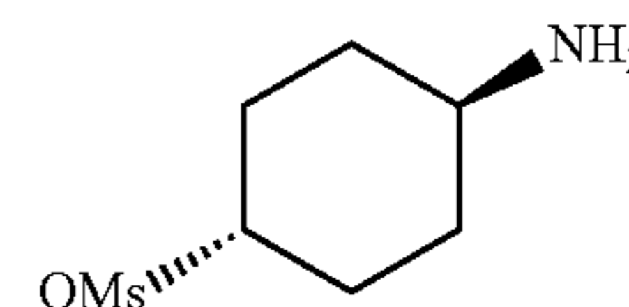
(1r,4r)-4-aminocyclohexyl methanesulfonate
