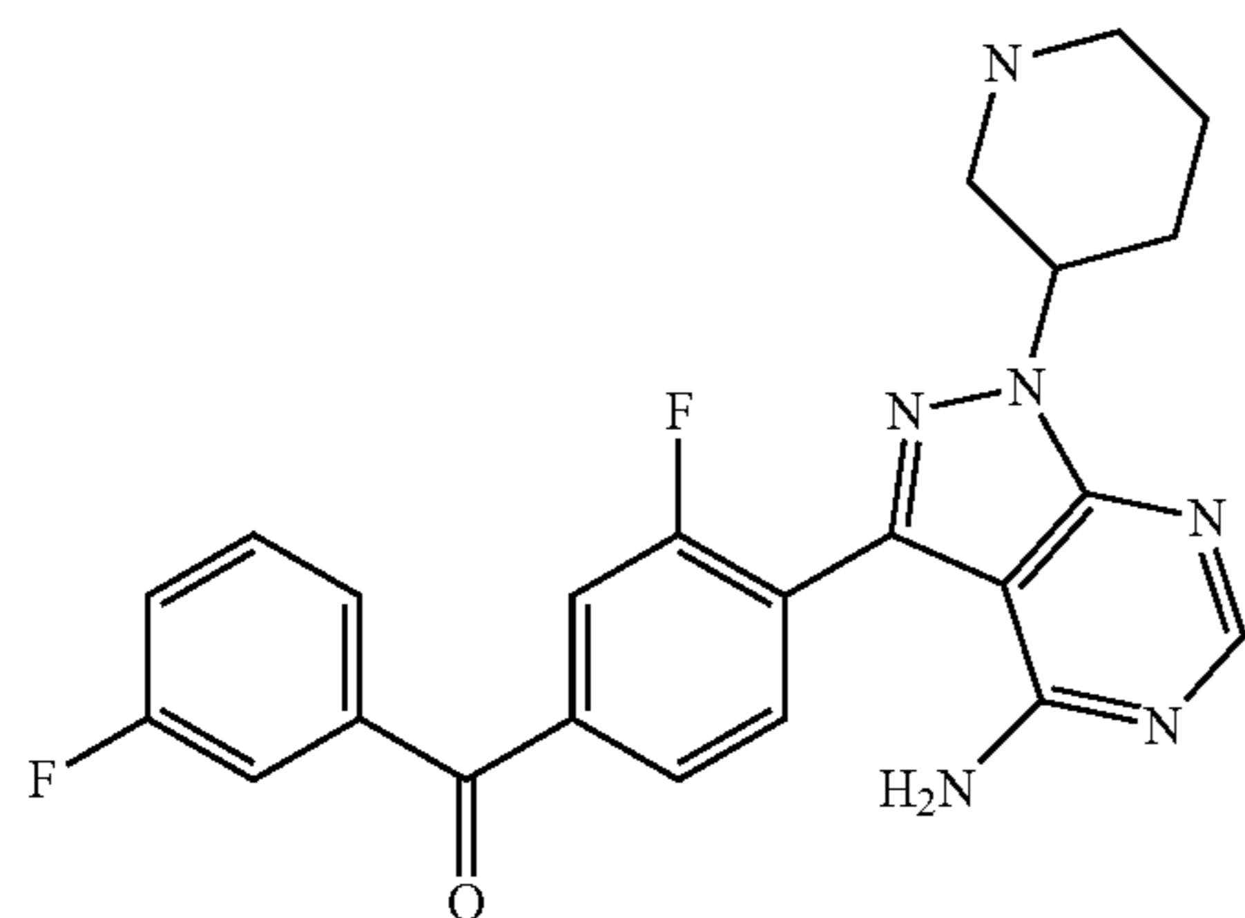
(4-(4-amino-1-(piperidin-3-yl)-1H-pyrazolo[3,4-d]pyrimidin-3-yl)-3-fluorophenyl)(3-fluorophenyl)methanone
