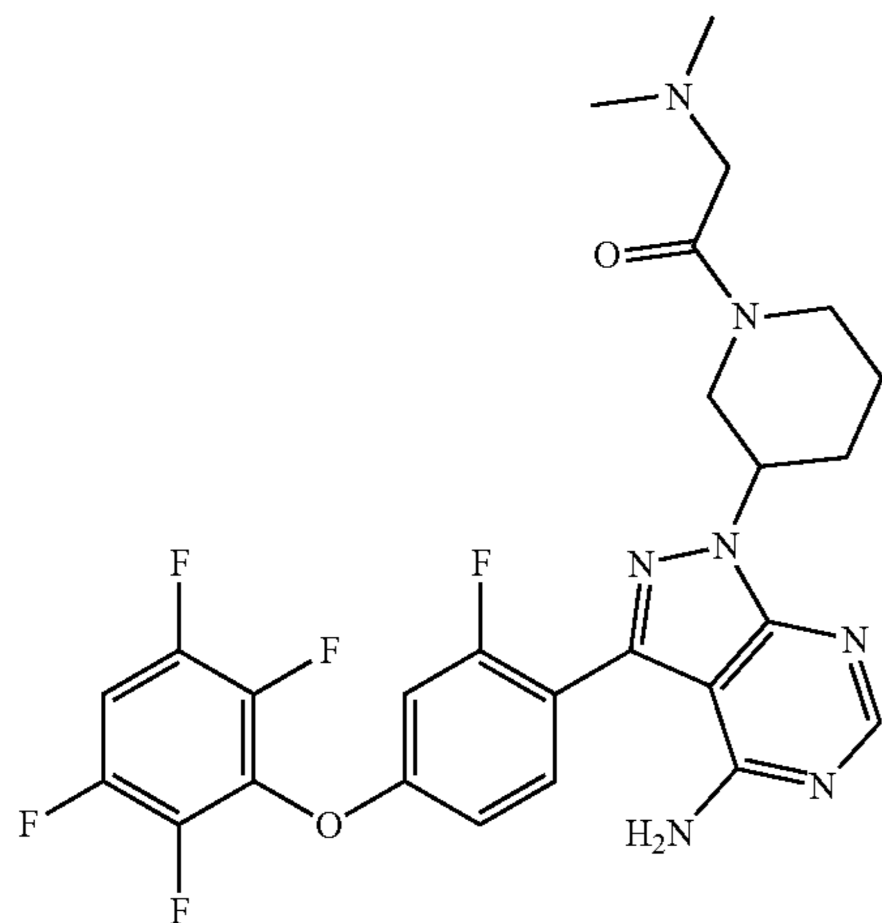
1-(3-(4-amino-3-(2-fluoro-4-(2,3,5,6-tetrafluorophenoxy)phenyl)-1H-pyrazolo[3,4-d]pyrimidin-1-yl)piperidin-1-yl)-2-(dimethylamino)ethanone
