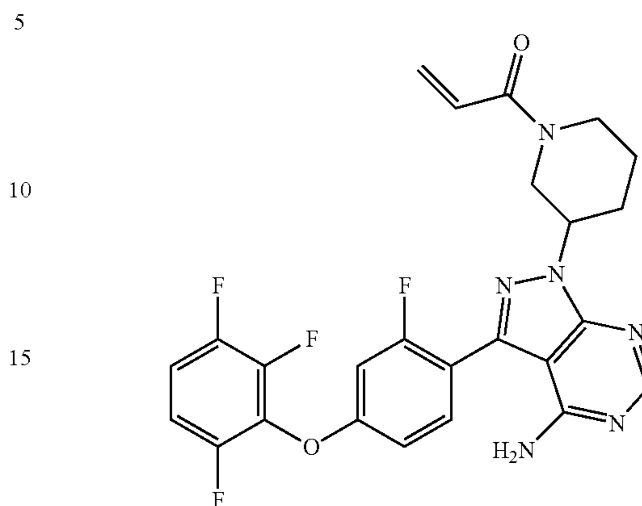
1-(3-(4-amino-3-(2-fluoro-4-(2,3,6-trifluorophenoxy)phenyl)-1H-pyrazolo[3,4-d]pyrimidin-1-yl)piperidin-1-yl)prop-2-en-1-one
