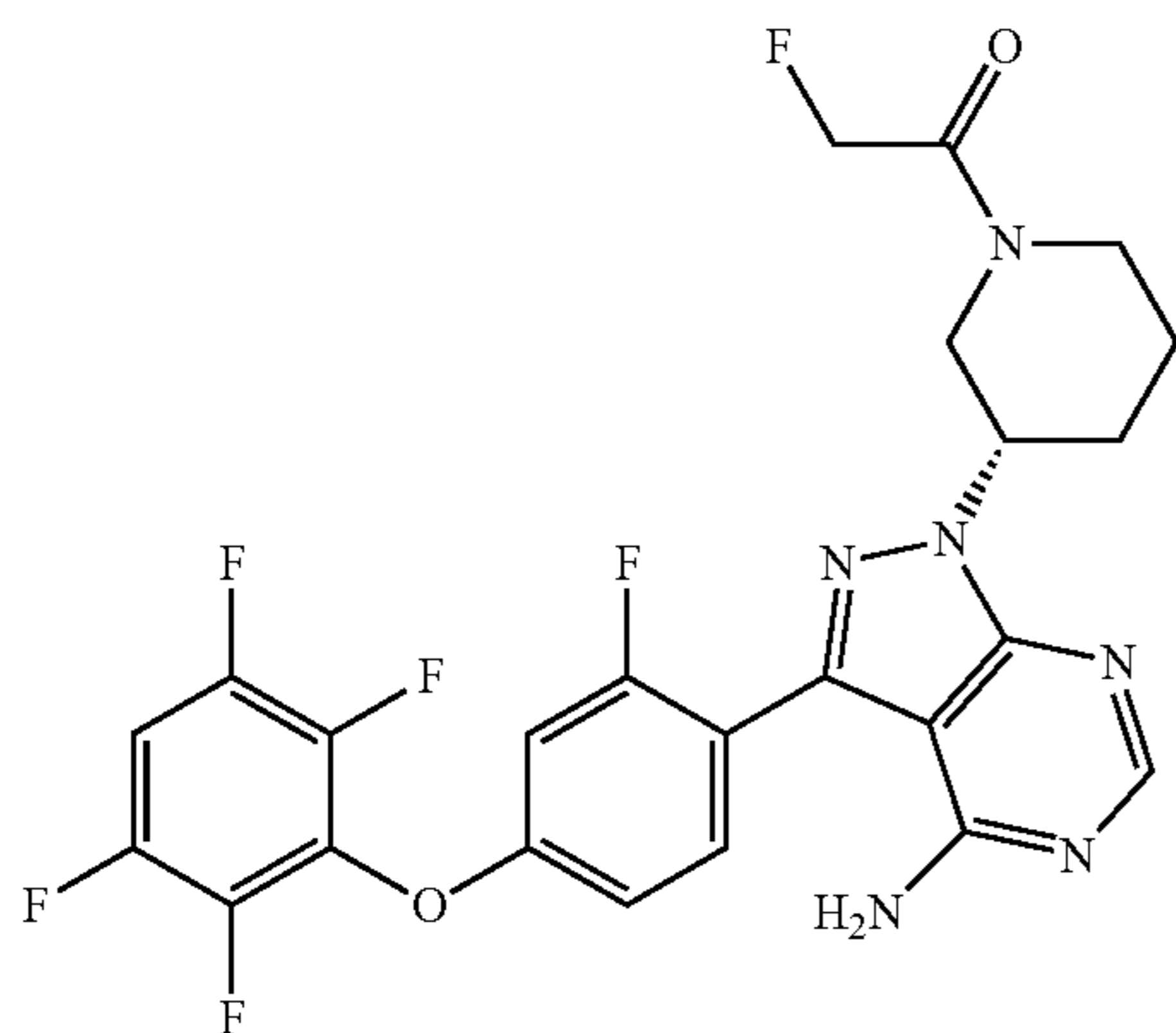
1-((S)-3-(4-amino-3-(2-fluoro-4-(2,3,5,6-tetrafluorophenoxy)phenyl)-1H-pyrazolo[3,4-d]pyrimidin-1-yl) piperidin-1-yl)-2-fluoroethanone
