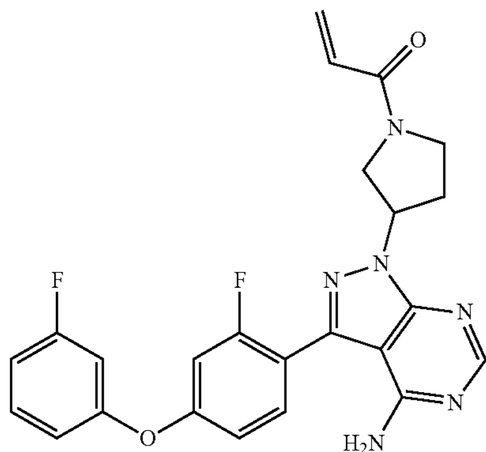
1-(3-(4-amino-3-(2-fluoro-4-(3-fluorophenoxy)phenyl)-1H-pyrazolo[3,4-d]pyrimidin-1-yl)pyrrolidin-1-yl)prop-2-en-1-one
