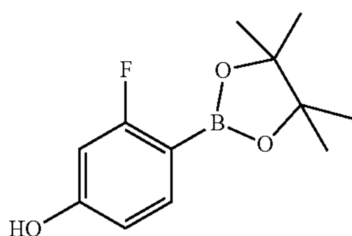
3-fluoro-4-(4,4,5,5-tetramethyl-1,3,2-dioxaborolan-2-yl)phenol
