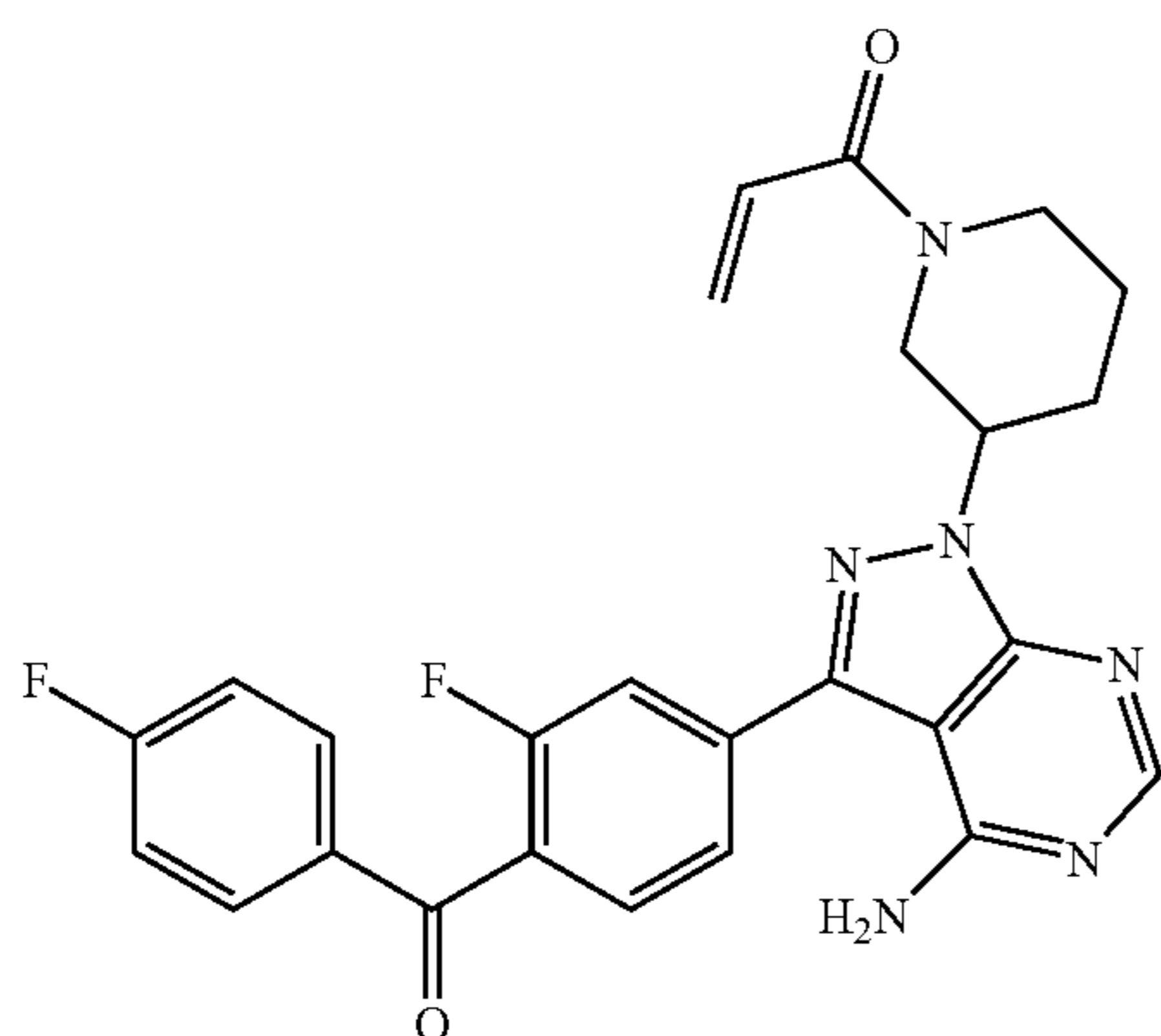
1-(3-(4-amino-3-(3-fluoro-4-(4-fluorobenzoyl)phenyl)-1H-pyrazolo[3,4-d]pyrimidin-1-yl)piperidin-1-yl)prop-2-en-1-one
