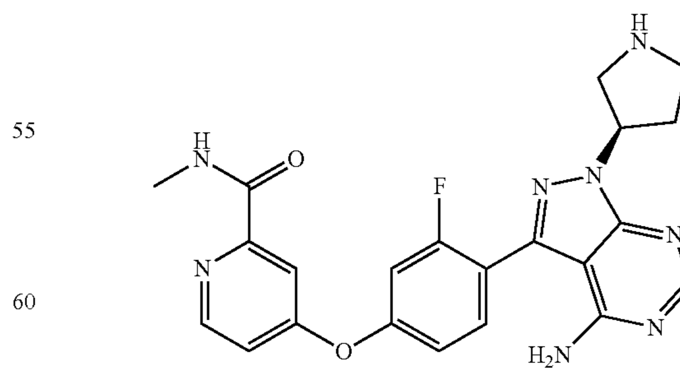
4-(4-(4-amino-1-((R)-pyrrolidin-3-yl)-1H-pyrazolo[3,4-d]pyrimidin-3-yl)-3-fluorophenoxy)-N-methylpicolinamide
