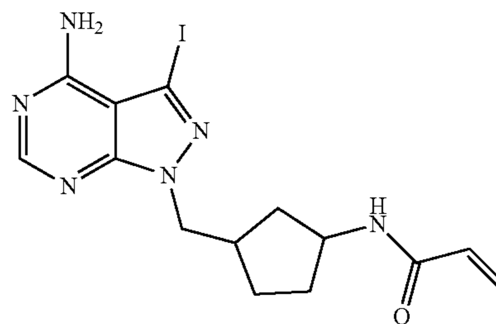
N-(3-((4-amino-3-iodo-1H-pyrazolo[3,4-d]pyrimidin-1-yl)methyl)cyclopentyl)acrylamide
