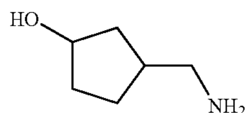
3-(aminomethyl)cyclopentanol
