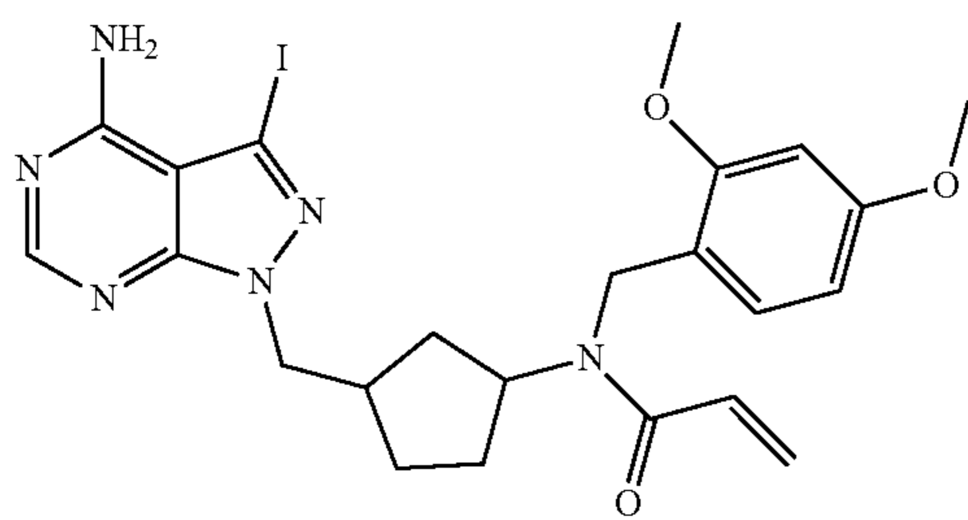
N-(2,4-dimethoxybenzyl)-N-(3-((4-amino-3-iodo-1H-pyrazolo[3,4-d]pyrimidin-1-yl)methyl)cyclopentyl)acrylamide
