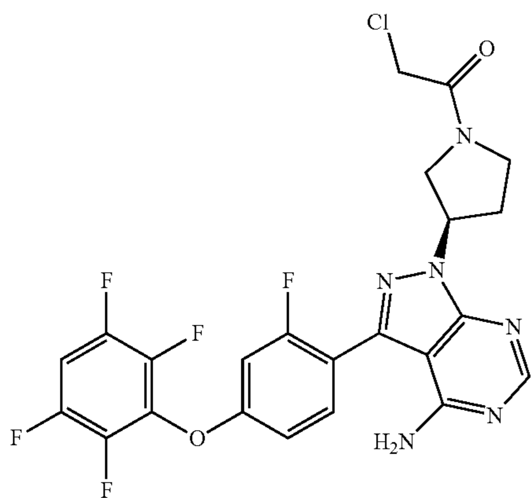
1-((R)-3-(4-amino-3-(2-fluoro-4-(2,3,5,6-tetrafluorophenoxy)phenyl)-1H-pyrazolo[3,4-d]pyrimidin-1-yl)pyrrolidin-1-yl)-2-chloroethanone
