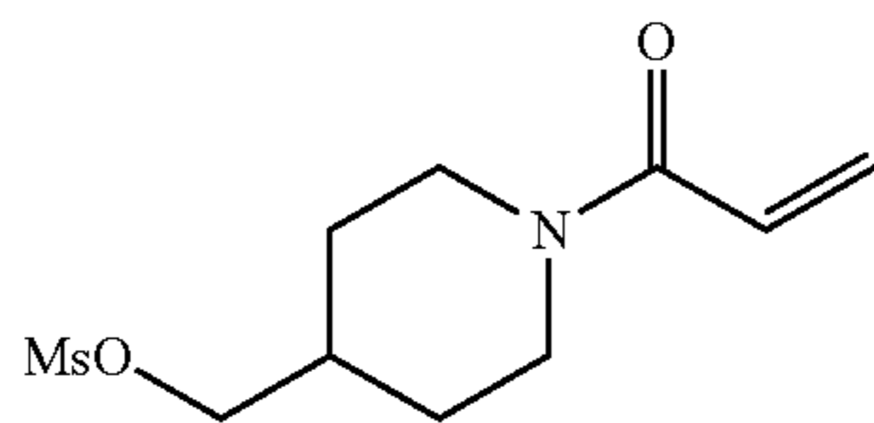
(1-acryloylpiperidin-4-yl)methyl methanesulfonate
