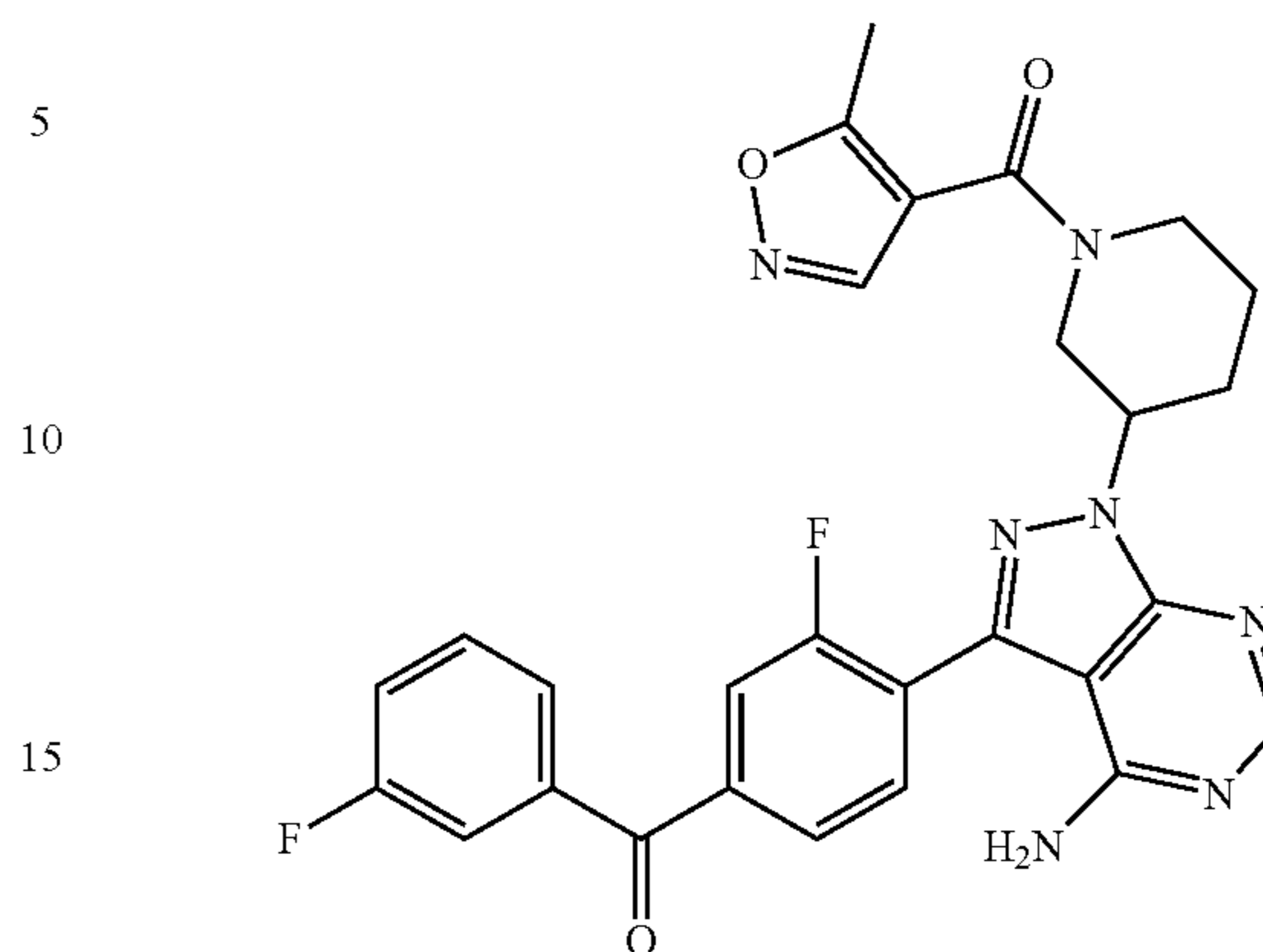
(3-(4-amino-3-(2-fluoro-4-(3-fluorobenzoyl)phenyl)-1H-pyrazolo[3,4-d]pyrimidin-1-yl)piperidin-1-yl)(5-methylisoxazol-4-yl)methanone
