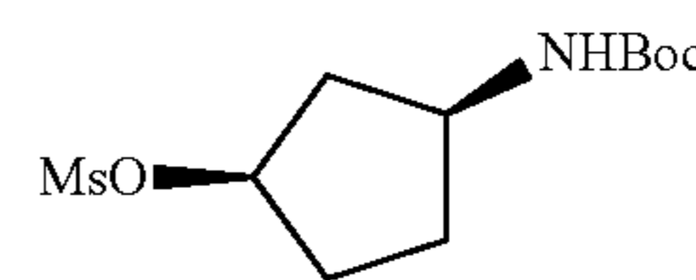
(1r,3s)-3-(tert-butoxycarbonyl)cyclopentyl methanesulfonate
