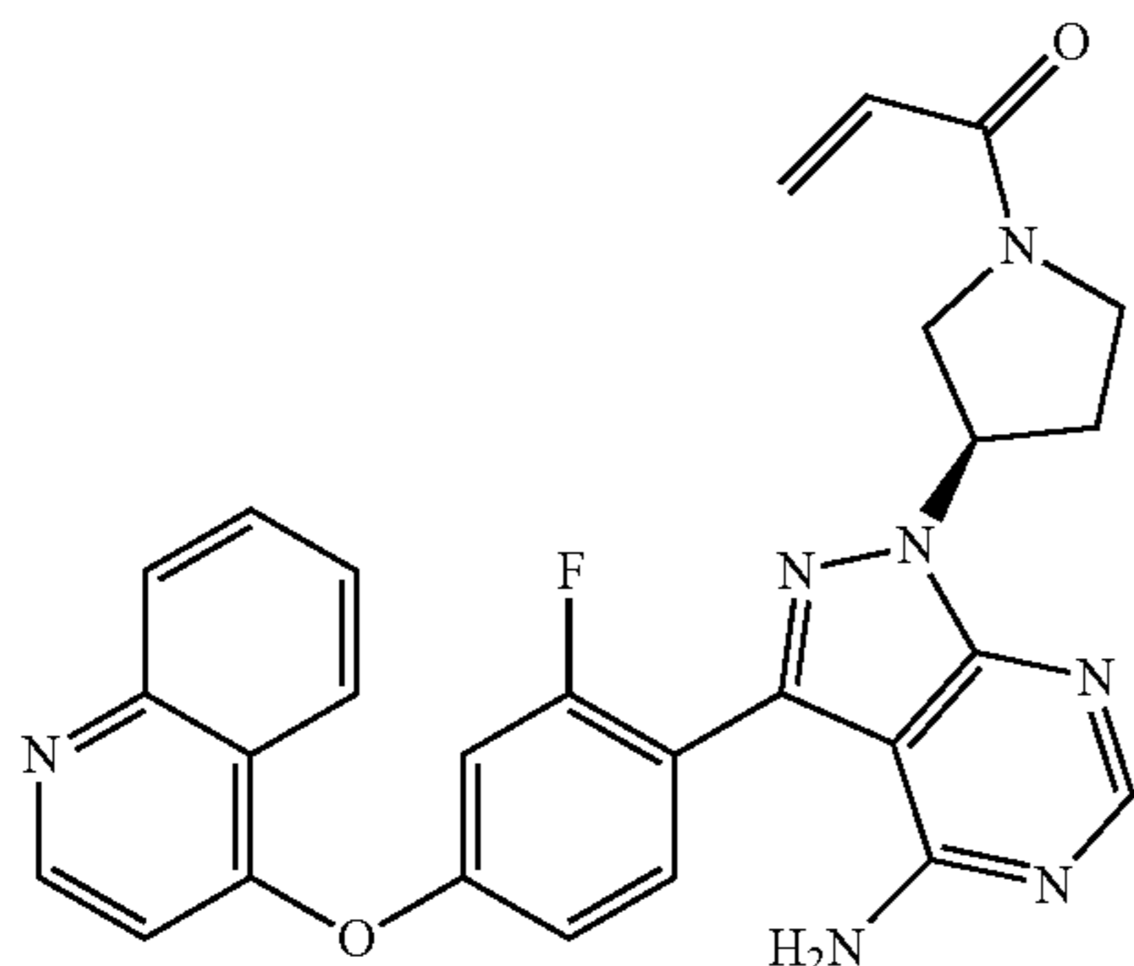
1-((R)-3-(4-amino-3-(2-fluoro-4-(quinolin-4-yloxy)phenyl)-1H-pyrazolo[3,4-d]pyrimidin-1-yl)pyrrolidin-1-yl)prop-2-en-1-one
