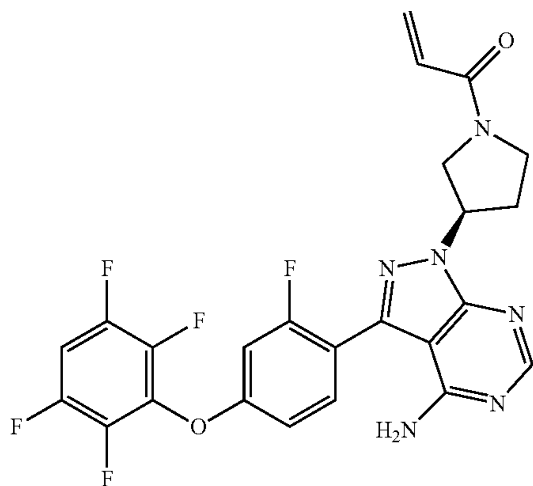
1-((R)-3-(4-amino-3-(2-fluoro-4-(2,3,5,6-tetrafluorophenoxy)phenyl)-1H-pyrazolo[3,4-d]pyrimidin-1-yl)pyrrolidin-1-yl)prop-2-en-1-one
