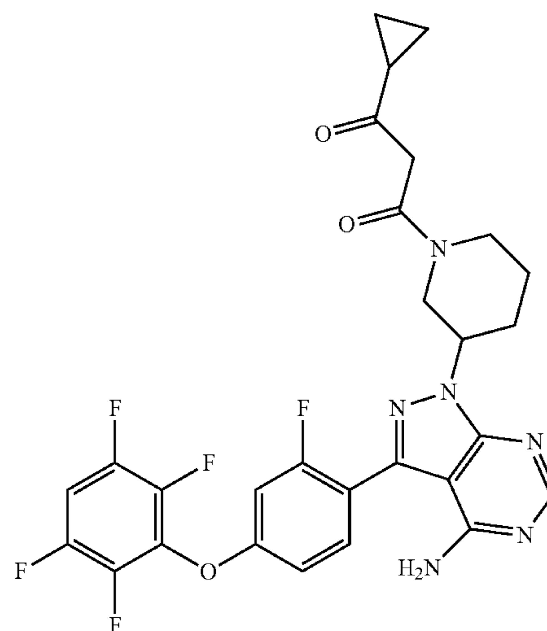
1-(3-(4-amino-3-(2-fluoro-4-(2,3,5,6-tetrafluorophenoxy)phenyl)-1H-pyrazolo[3,4-d]pyrimidin-1-yl)piperidin-1-yl)-3-cyclopropylpropane-1,3-dione
