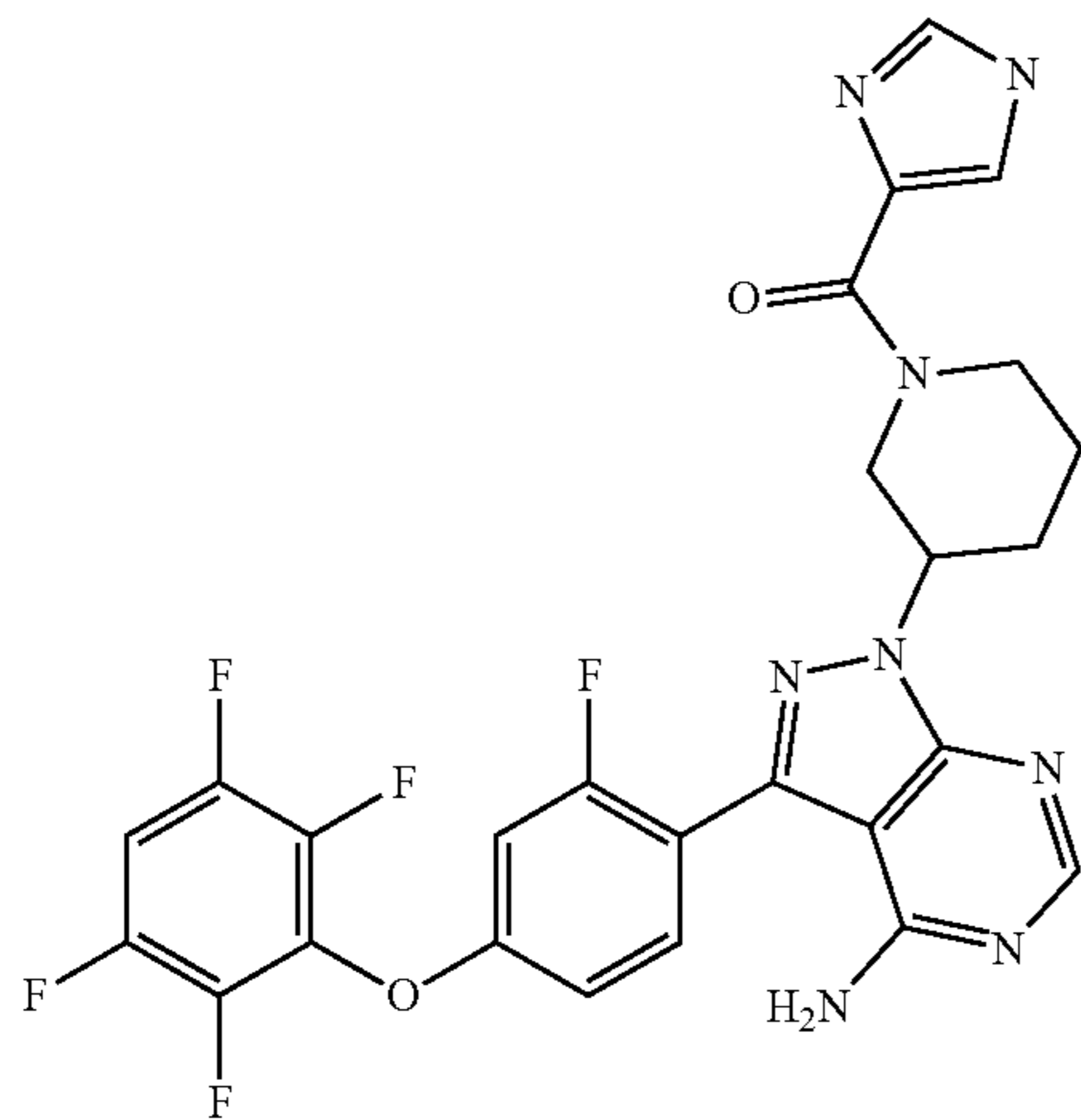
(3-(4-amino-3-(2-fluoro-4-(2,3,5,6-tetrafluorophenoxy)phenyl)-1H-pyrazolo[3,4-d]pyrimidin-1-yl)piperidin-1-yl)(1H-imidazol-4-yl)methanone
