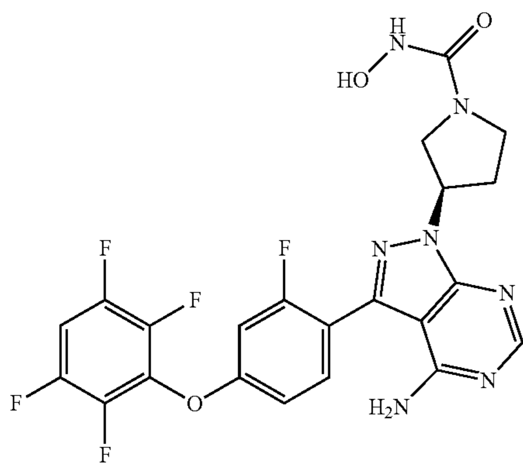
(3R)-3-(4-amino-3-(2-fluoro-4-(2,3,5,6-tetrafluorophenoxy)phenyl)-1H-pyrazolo[3,4-d]pyrimidin-1-yl)-N-hydroxypyrrolidine-1-carboxamide
