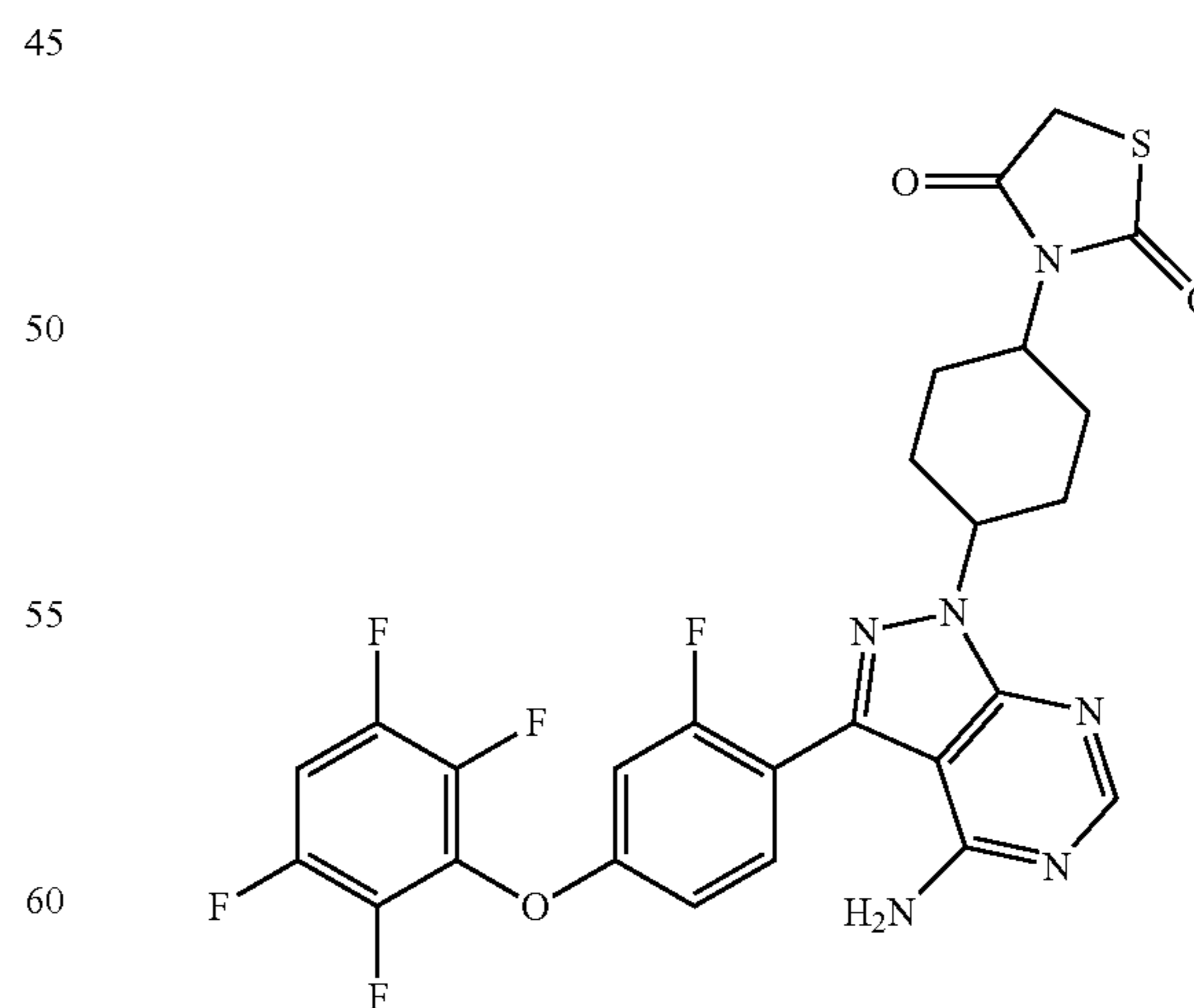
3-(4-(4-amino-3-(2-fluoro-4-(2,3,5,6-tetrafluorophenoxy)phenyl)-1H-pyrazolo[3,4-d]pyrimidin-1-yl)cyclohexyl)thiazolidine-2,4-dione
