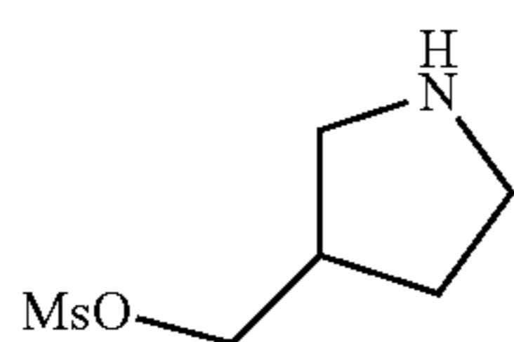
pyrrolidin-3-ylmethyl methanesulfonate
