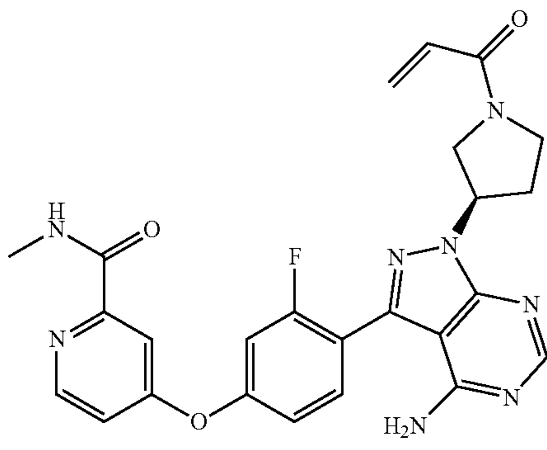
4-(4-(1-((R)-1-acryloylpyrrolidin-3-yl)-4-amino-1H-pyrazolo[3,4-d]pyrimidin-3-yl)-3-fluorophenoxy)-N-methylpicolinamide
