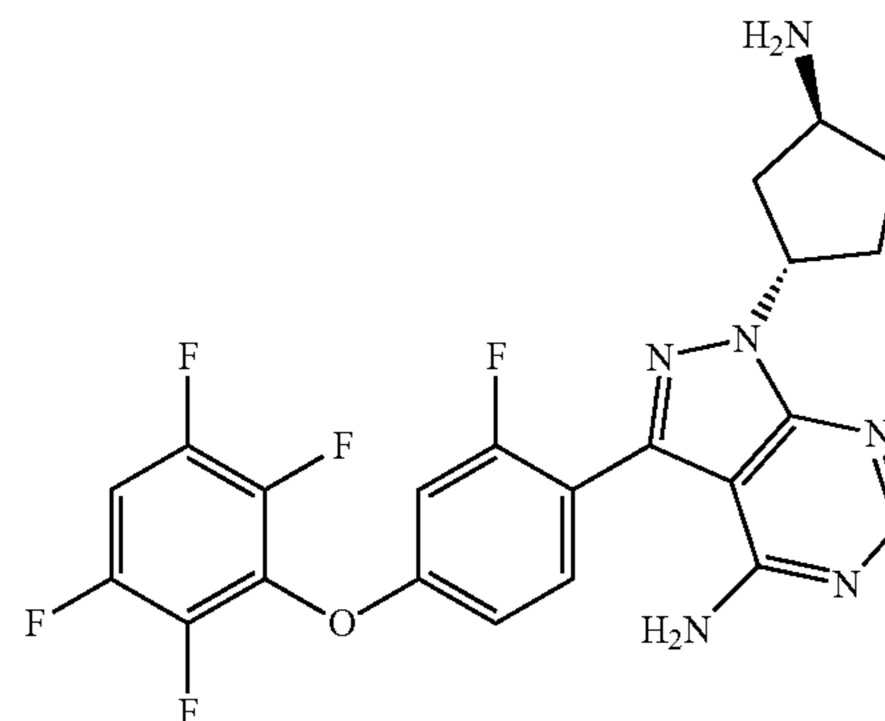
1-((1s,3 s)-3-aminocyclopentyl)-3-(2-fluoro-4-(2,3,5,6-tetrafluorophenoxy)phenyl)-1H-pyrazolo[3,4-d]pyrimidin-4-amine
