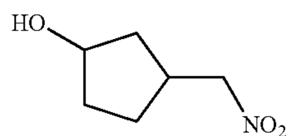
3-(nitromethyl)cyclopentanol
