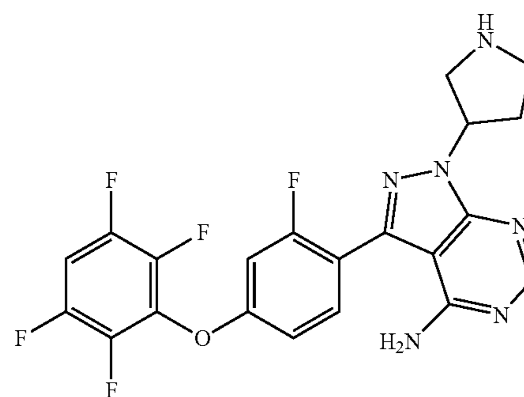
3-(2-fluoro-4-(2,3,5,6-tetrafluorophenoxy)phenyl)-1-(pyrrolidin-3-yl)-1H-pyrazolo[3,4-d]pyrimidin-4-amine
