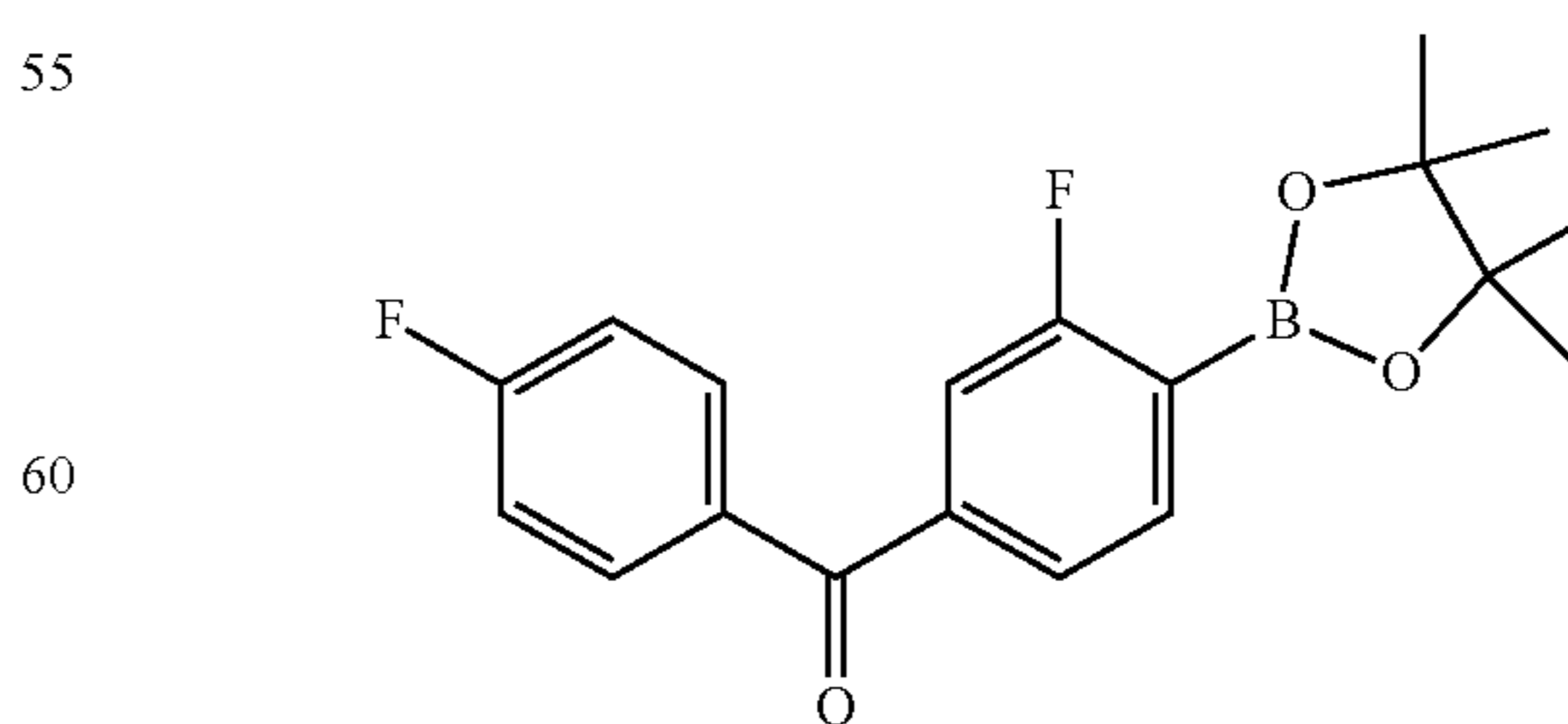
(3-fluoro-4-(4,4,5,5-tetramethyl-1,3,2-dioxaborolan-2-yl)phenyl)(4-fluorophenyl)methanone
