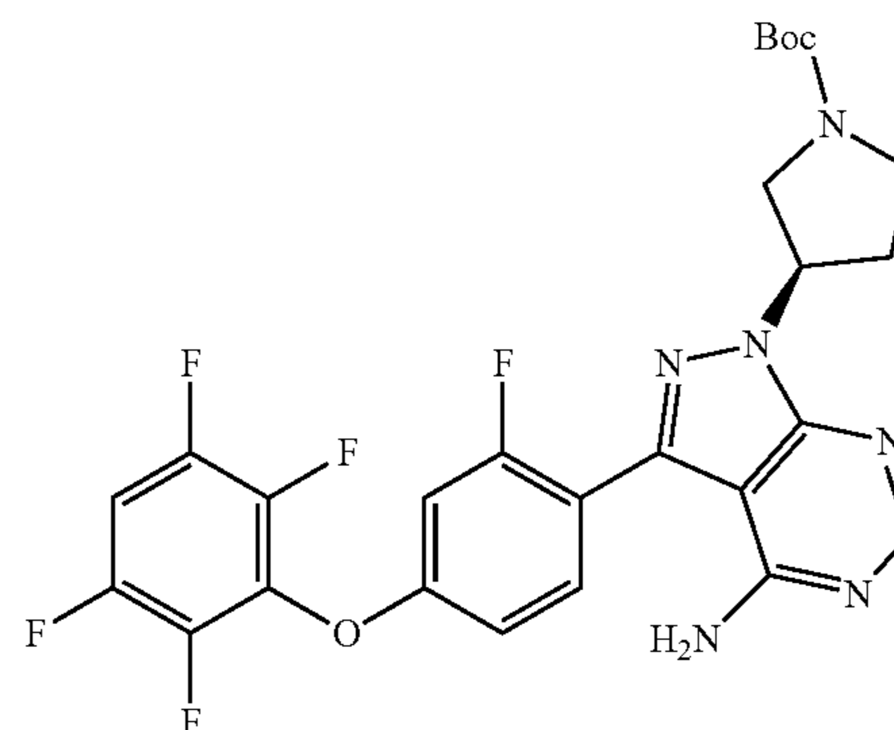
(3R)-tert-butyl 3-(4-amino-3-(2-fluoro-4-(2,3,5,6-tetrafluorophenoxy)phenyl)-1H-pyrazolo[3,4-d]pyrimidin-1-yl)pyrrolidine-1-carboxylate
