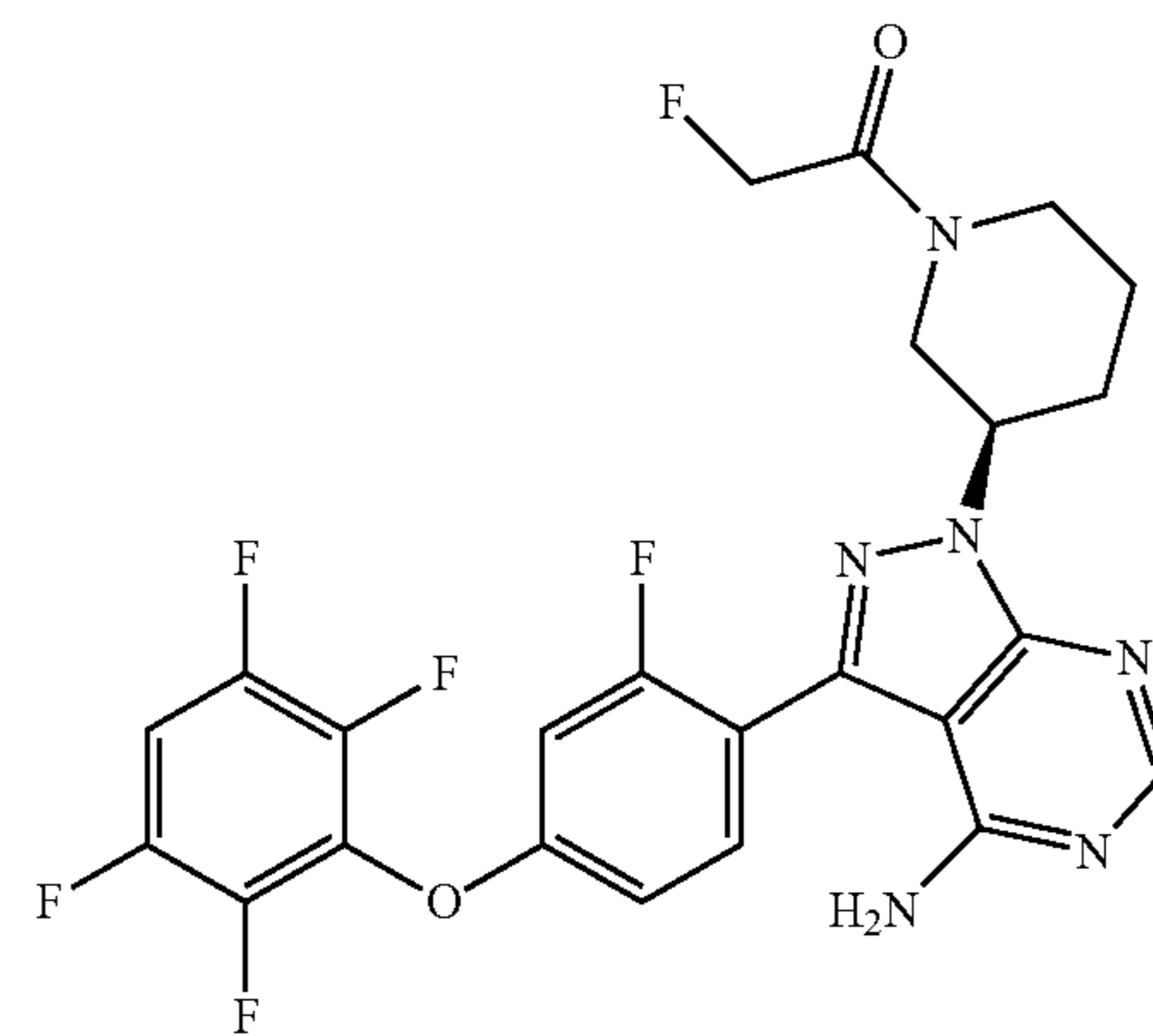
1-((R)-3-(4-amino-3-(2-fluoro-4-(2,3,5,6-tetrafluorophenoxy)phenyl)-1H-pyrazolo[3,4-d]pyrimidin-1-yl)piperidin-1-yl)-2-fluoroethanone
