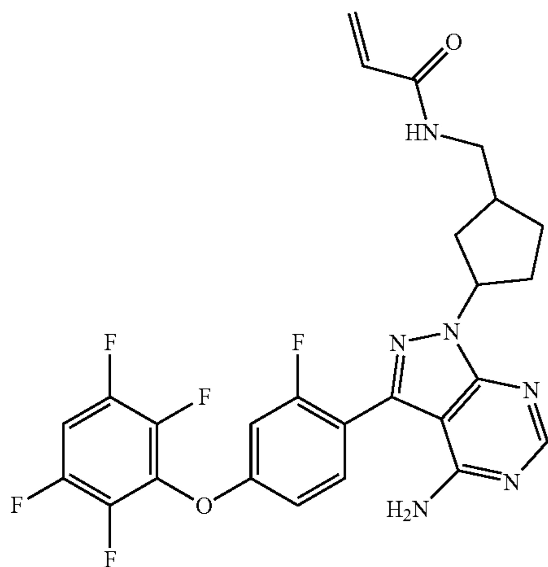
N-((3-(4-amino-3-(2-fluoro-4-(2,3,5,6-tetrafluorophenoxy)phenyl)-1H-pyrazolo[3,4-d]pyrimidin-1-yl)cyclopentyl)methyl)acrylamide
