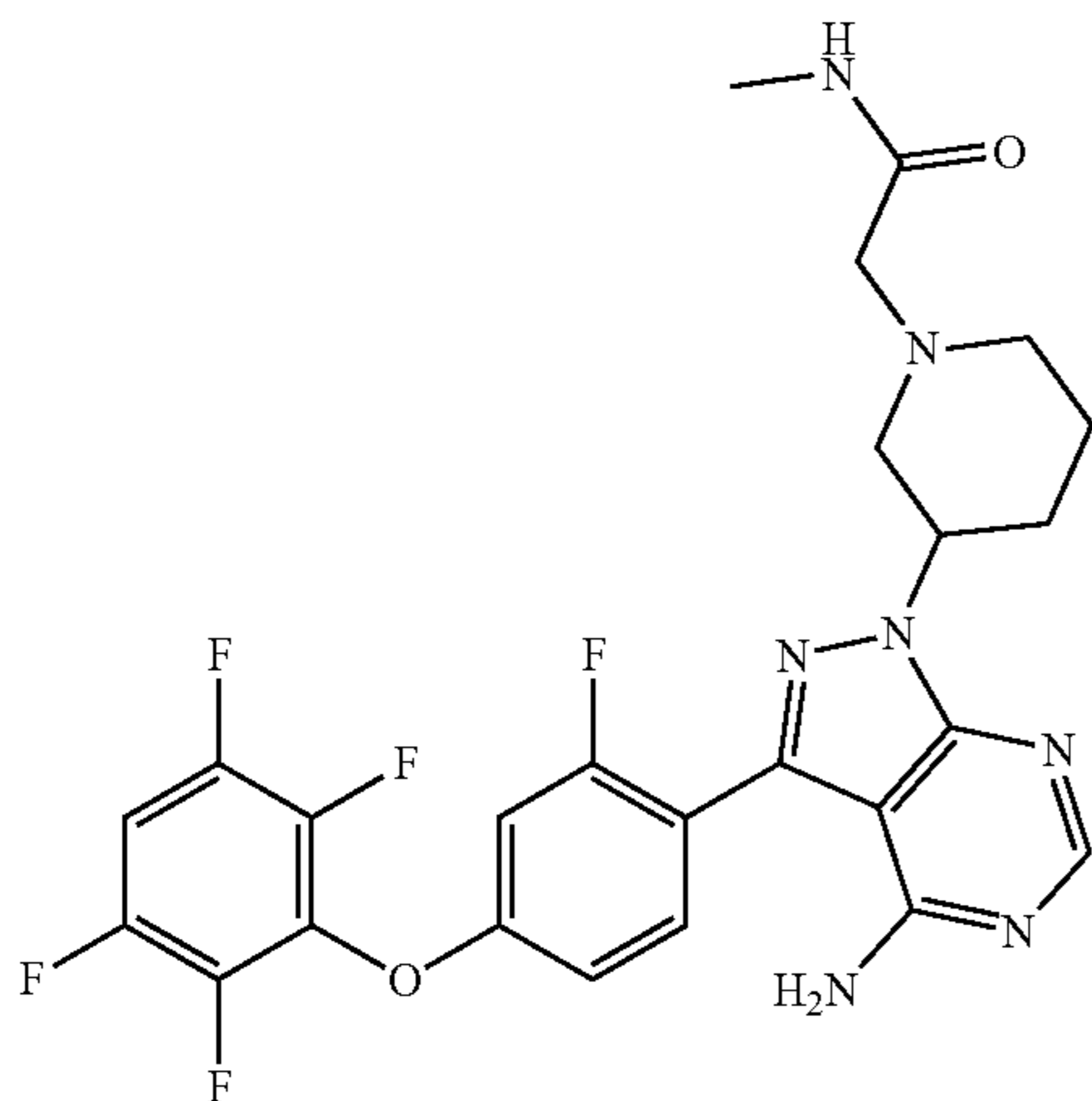
2-(3-(4-amino-3-(2-fluoro-4-(2,3,5,6-tetrafluorophenoxy)phenyl)-1H-pyrazolo[3,4-d]pyrimidin-1-yl)piperidin-1-yl)-N-methylacetamide
