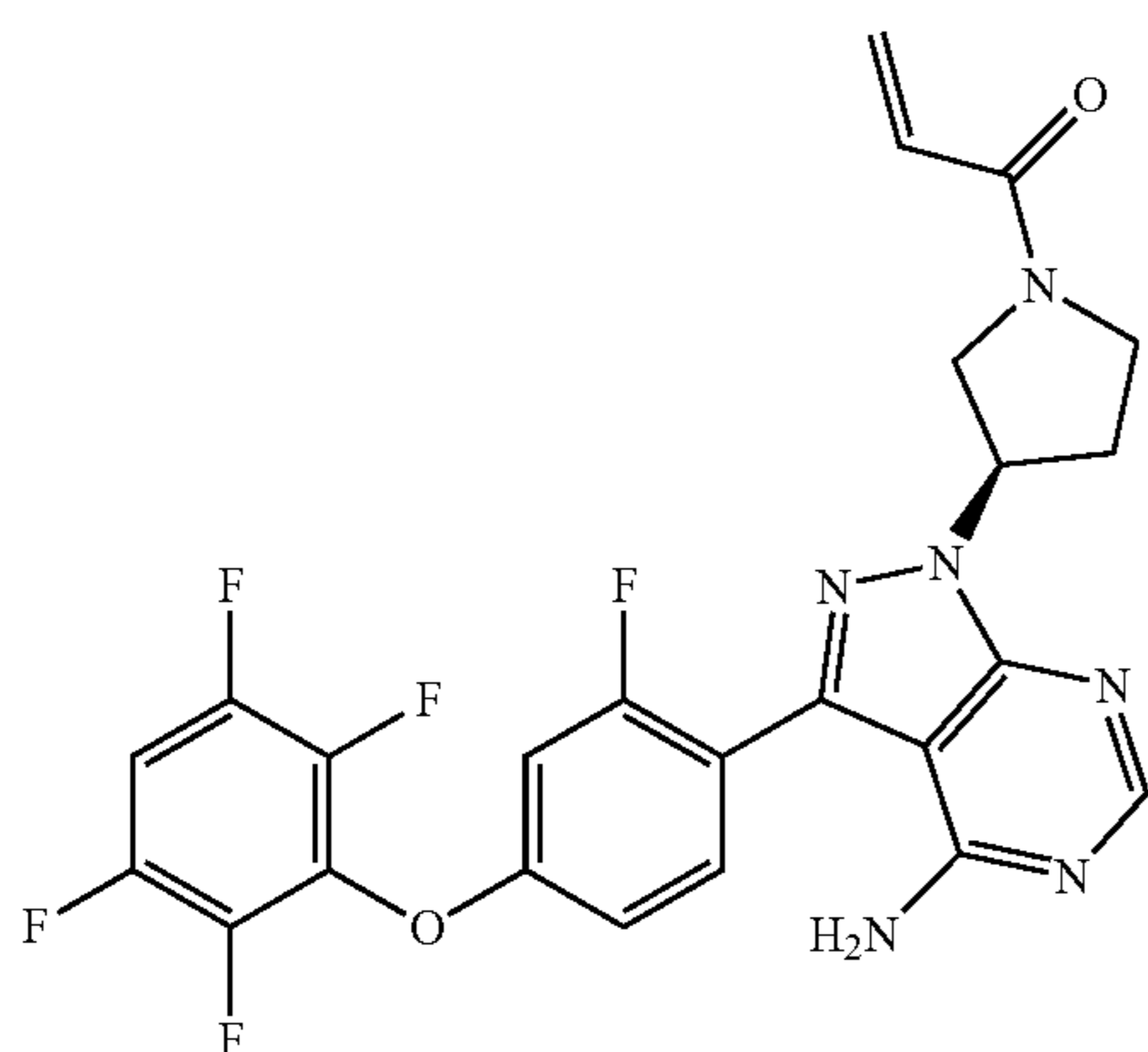
1-((R)-3-(4-amino-3-(2-fluoro-4-(2,3,5,6-tetrafluorophenoxy)phenyl)-1H-pyrazolo[3,4-d]pyrimidin-1-yl)pyrrolidin-1-yl)prop-2-en-1-one
