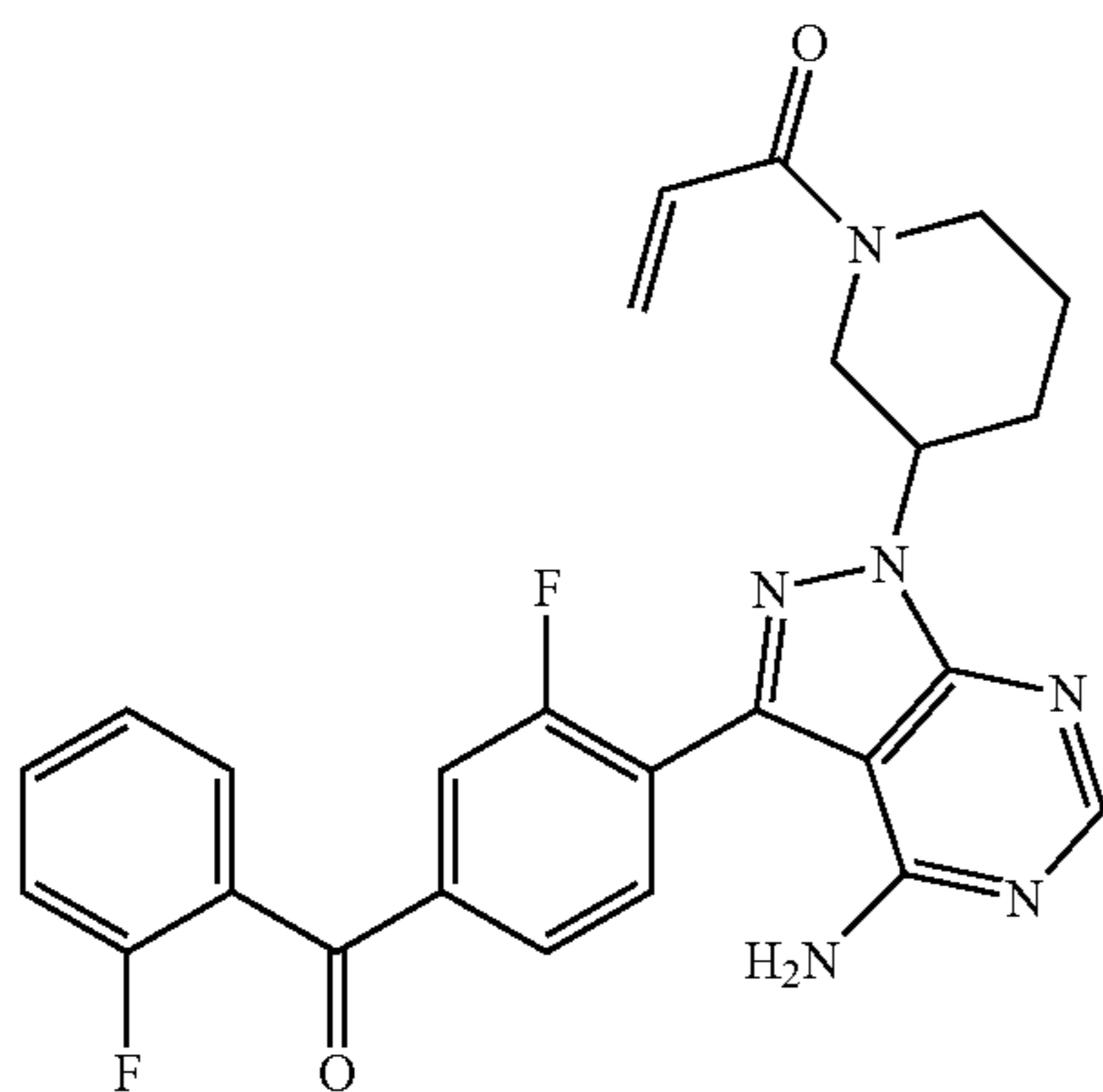
1-(3-(4-amino-3-(2-fluoro-4-(2-fluorobenzoyl)phenyl)-1H-pyrazolo[3,4-d]pyrimidin-1-yl)piperidin-1-yl)prop-2-en-1-one
