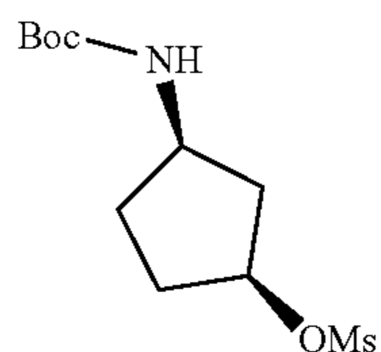
(1s,3r)-3-(tert-butoxycarbonyl)cyclopentyl methanesulfonate
