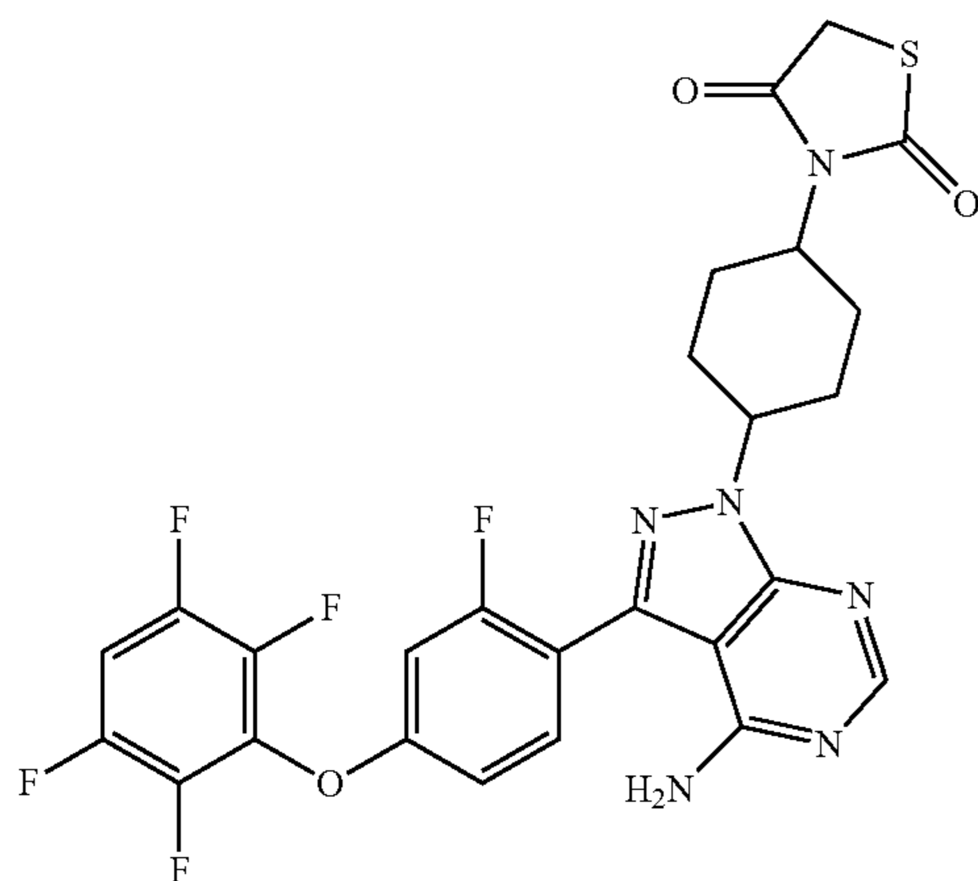
3-(4-(4-amino-3-(2-fluoro-4-(2,3,5,6-tetrafluorophenoxy)phenyl)-1H-pyrazolo[3,4-d]pyrimidin-1-yl)cyclohexyl)thiazolidine-2,4-dione
