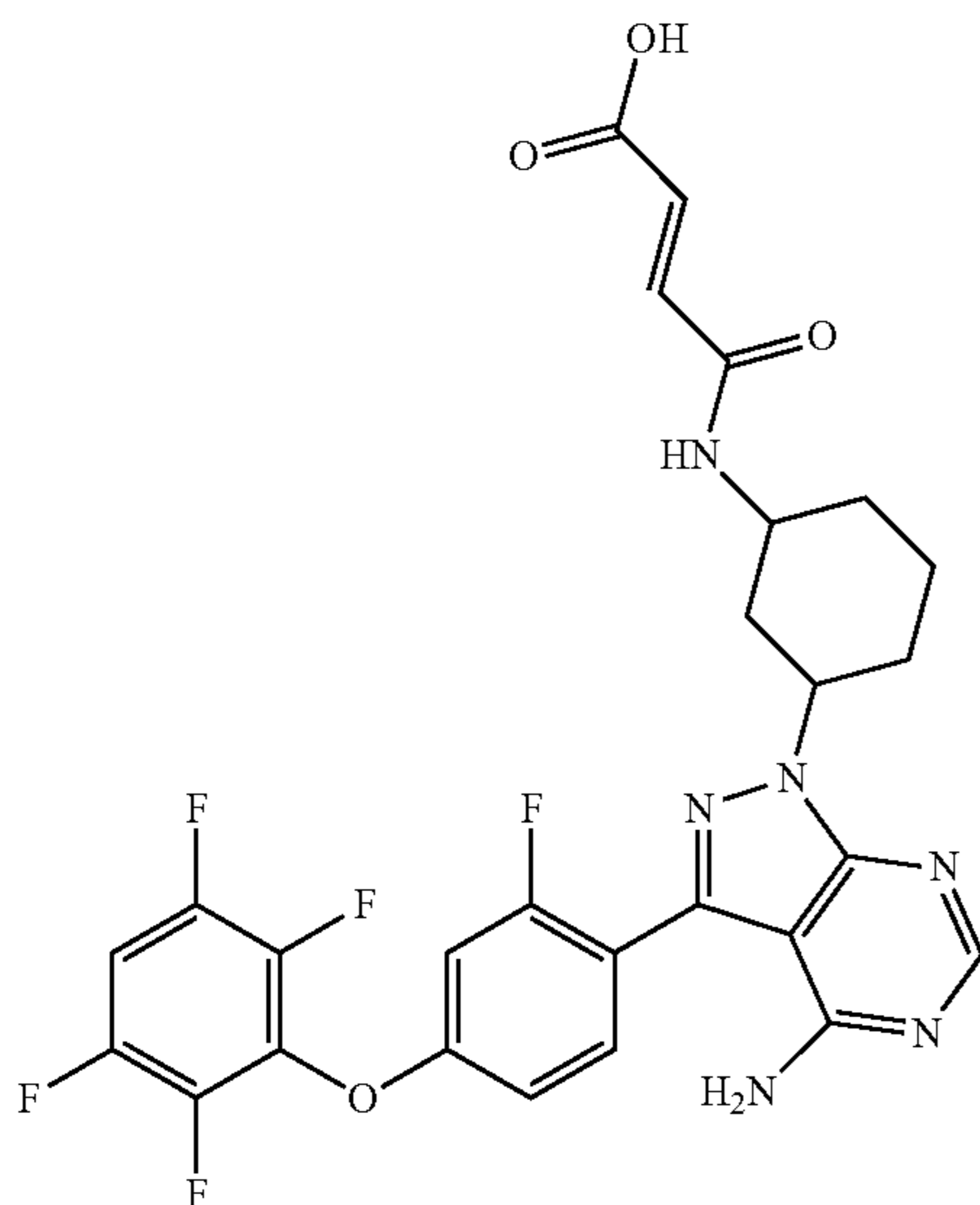
(E)-4-(3-(4-amino-3-(2-fluoro-4-(2,3,5,6-tetrafluorophenoxy)phenyl)-1H-pyrazolo[3,4-d]pyrimidin-1-yl)cyclohexylamino)-4-oxobut-2-enoic Acid
