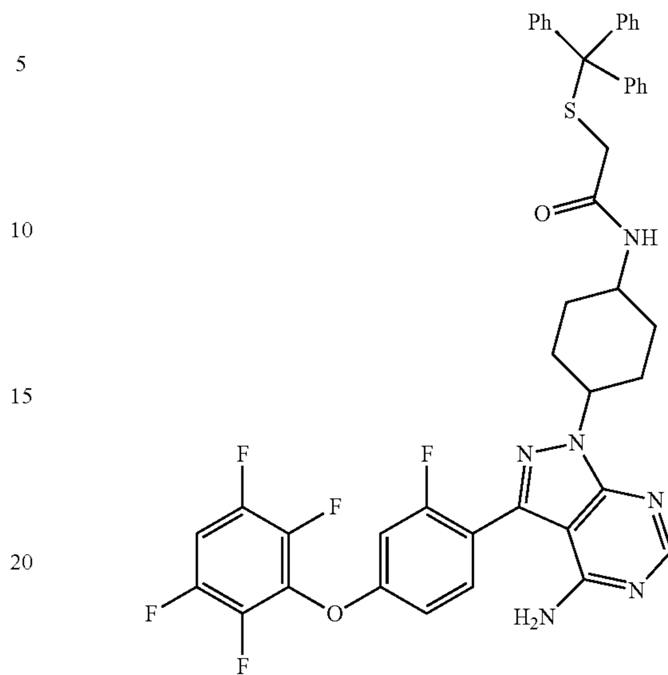
N-(4-(4-amino-3-(2-fluoro-4-(2,3,5,6-tetrafluorophenoxy)phenyl)-1H-pyrazolo[3,4-d]pyrimidin-1-yl)cyclohexyl)-2-(tritylthio)acetamide
