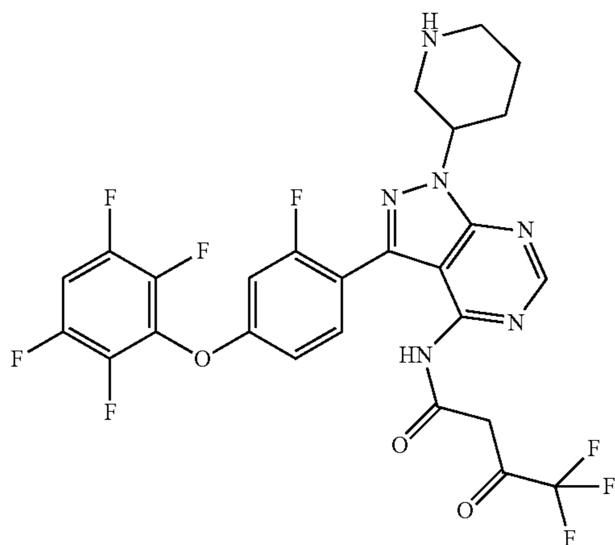
4,4,4-trifluoro-N-(3-(2-fluoro-4-(2,3,5,6-tetrafluorophenoxy)phenyl)-1-(piperidin-3-yl)-1H-pyrazolo[3,4-d]pyrimidin-4-yl)-3-oxobutanamide
