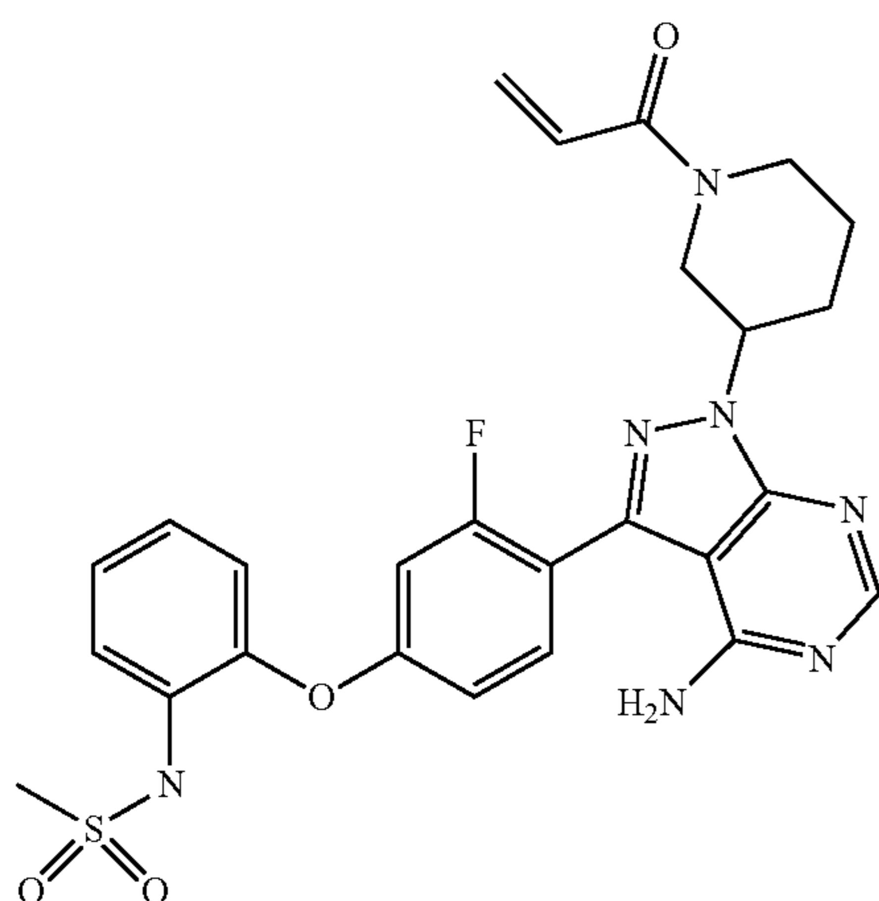
N-(2-(4-(1-(1-acryloylpiperidin-3-yl)-4-amino-1H-pyrazolo[3,4-d]pyrimidin-3-yl)-3-fluorophenoxy)phenyl)methanesulfonamide
