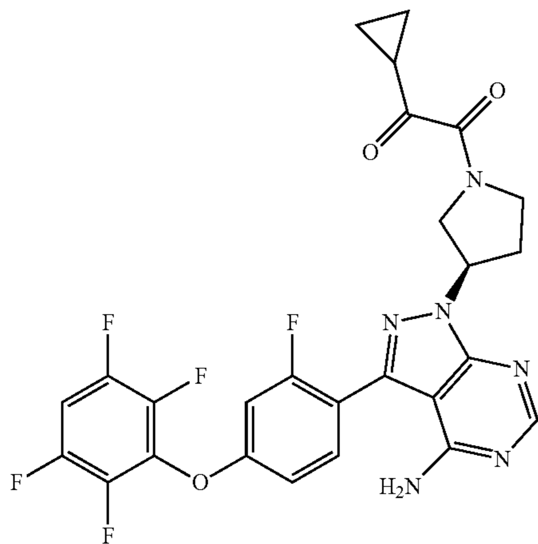
1-((R)-3-(4-amino-3-(2-fluoro-4-(2,3,5,6-tetrafluoro-phenoxy)phenyl)-1H-pyrazolo[3,4-d]pyrimidin-1-yl)pyrrolidin-1-yl)-2-cyclopropylethane-1,2-dione
