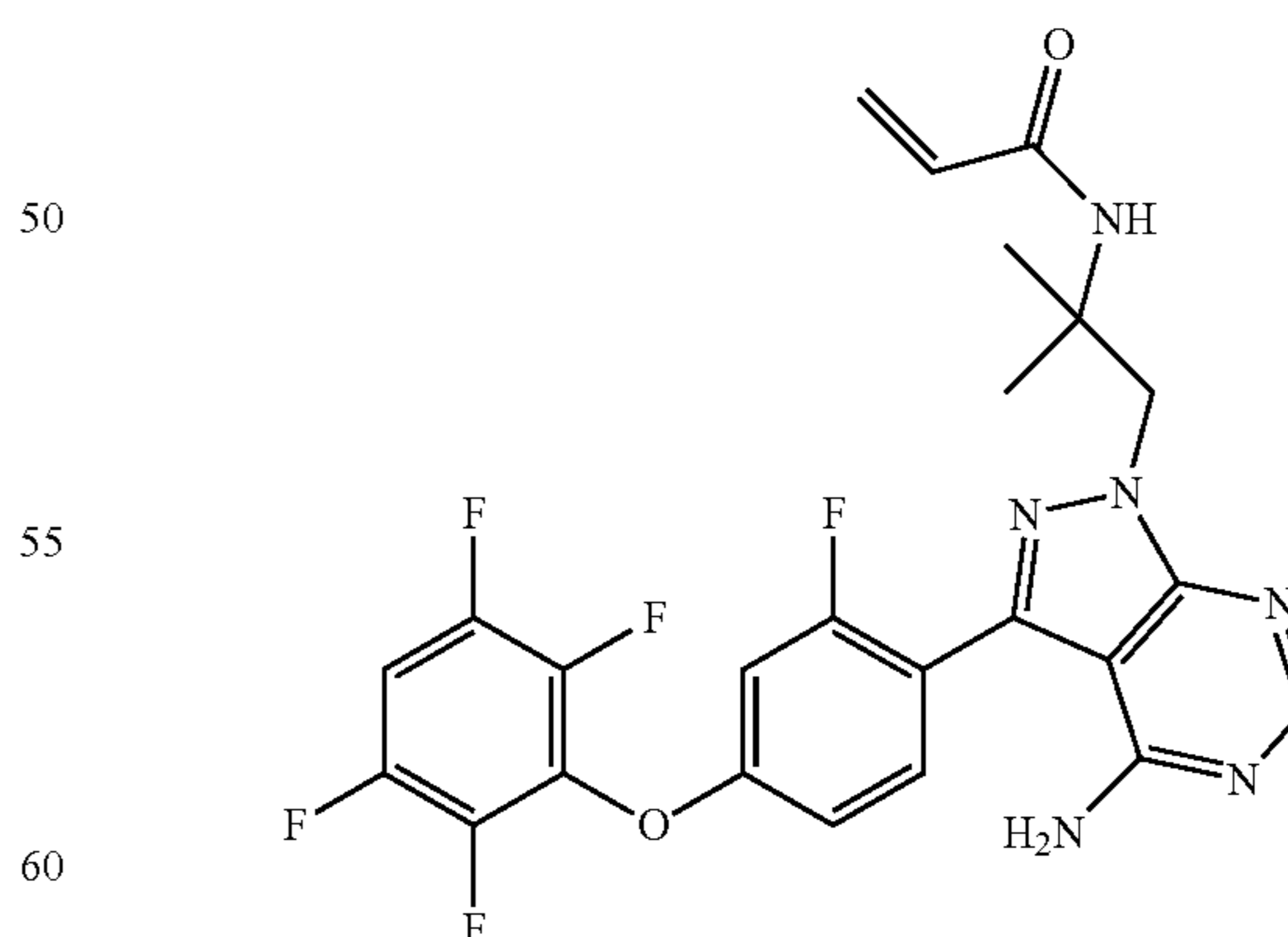
3-(2-fluoro-4-(2,3,5,6-tetrafluorophenoxy)phenyl)-1-(3-(methylamino)propyl)-1H-pyrazolo[3,4-d]pyrimidin-4-amine
