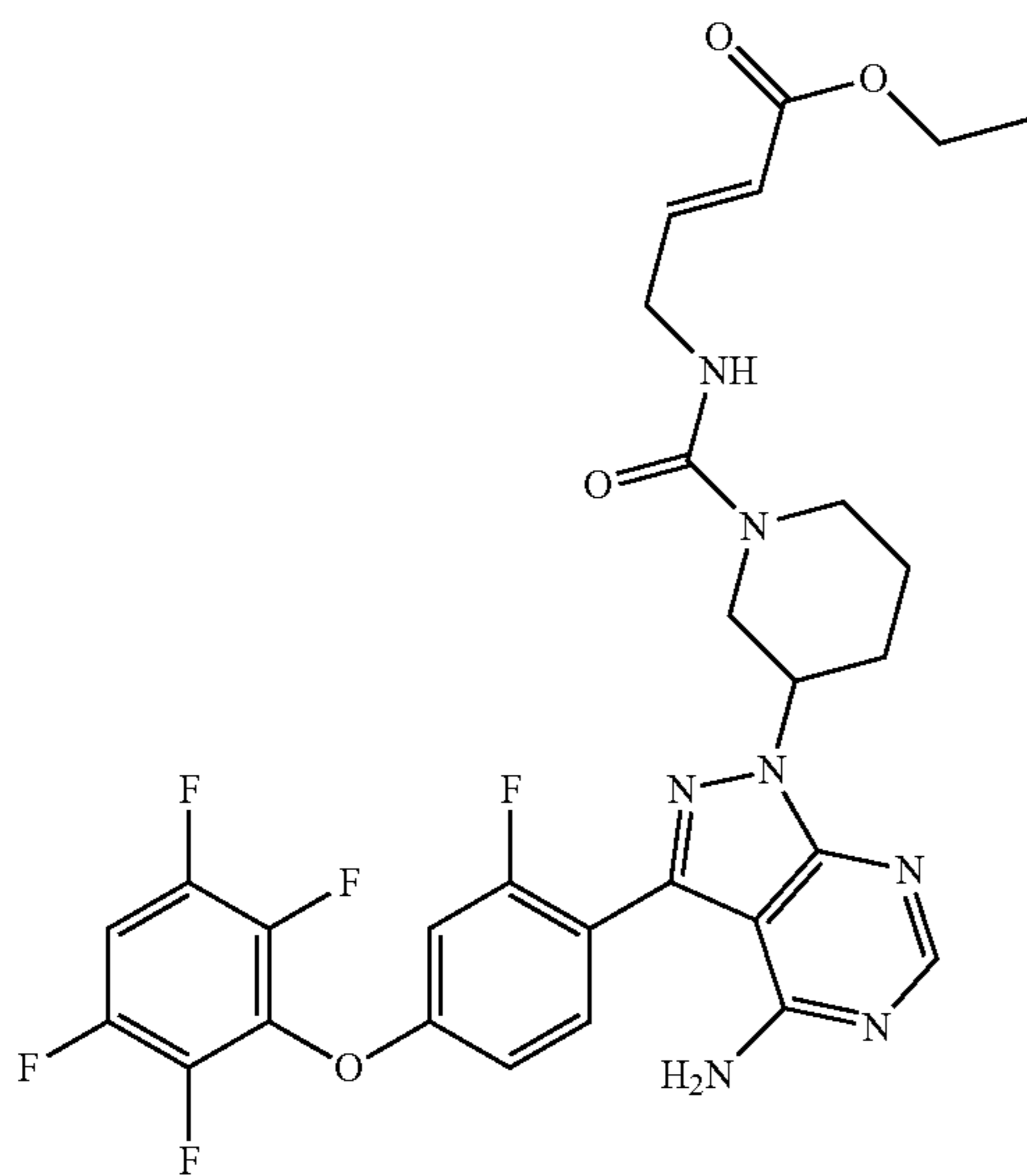
(E)-ethyl 4-(3-(4-amino-3-(2-fluoro-4-(2,3,5,6-tetrafluorophenoxy)phenyl)-1H-pyrazolo[3,4-d]pyrimidin-1-yl)piperidine-1-carboxamido)but-2-enoate
