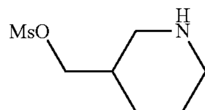
piperidin-3-ylmethyl methanesulfonate
