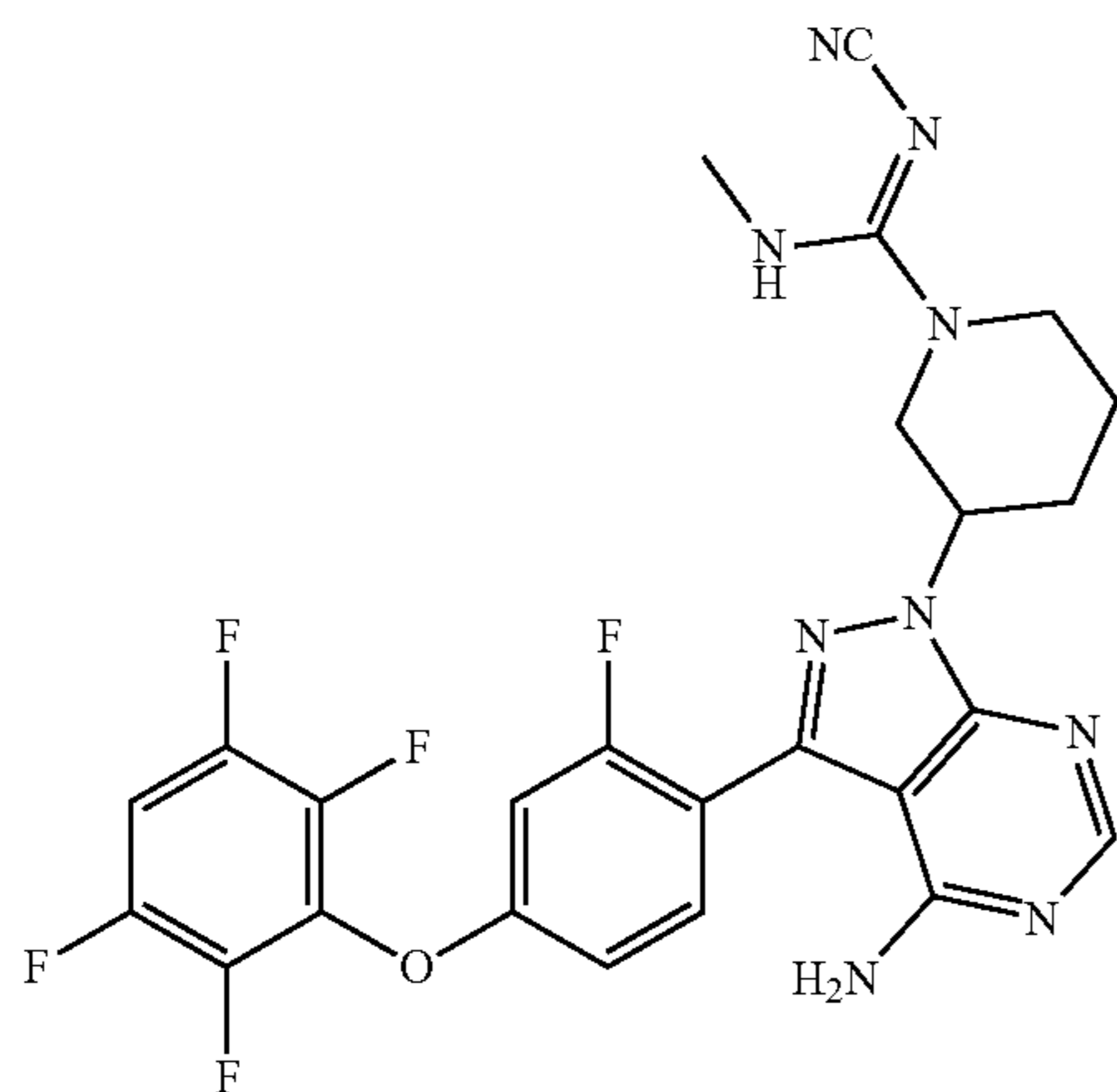
3-[4-amino-3-[2-fluoro-4-(2,3,5,6-fluorophenoxy)phenyl]-1H-pyrazolo[3,4-d]pyrimidin-1-yl]-N'-cyano-N-methyl-piperidine-1-carboxamide
