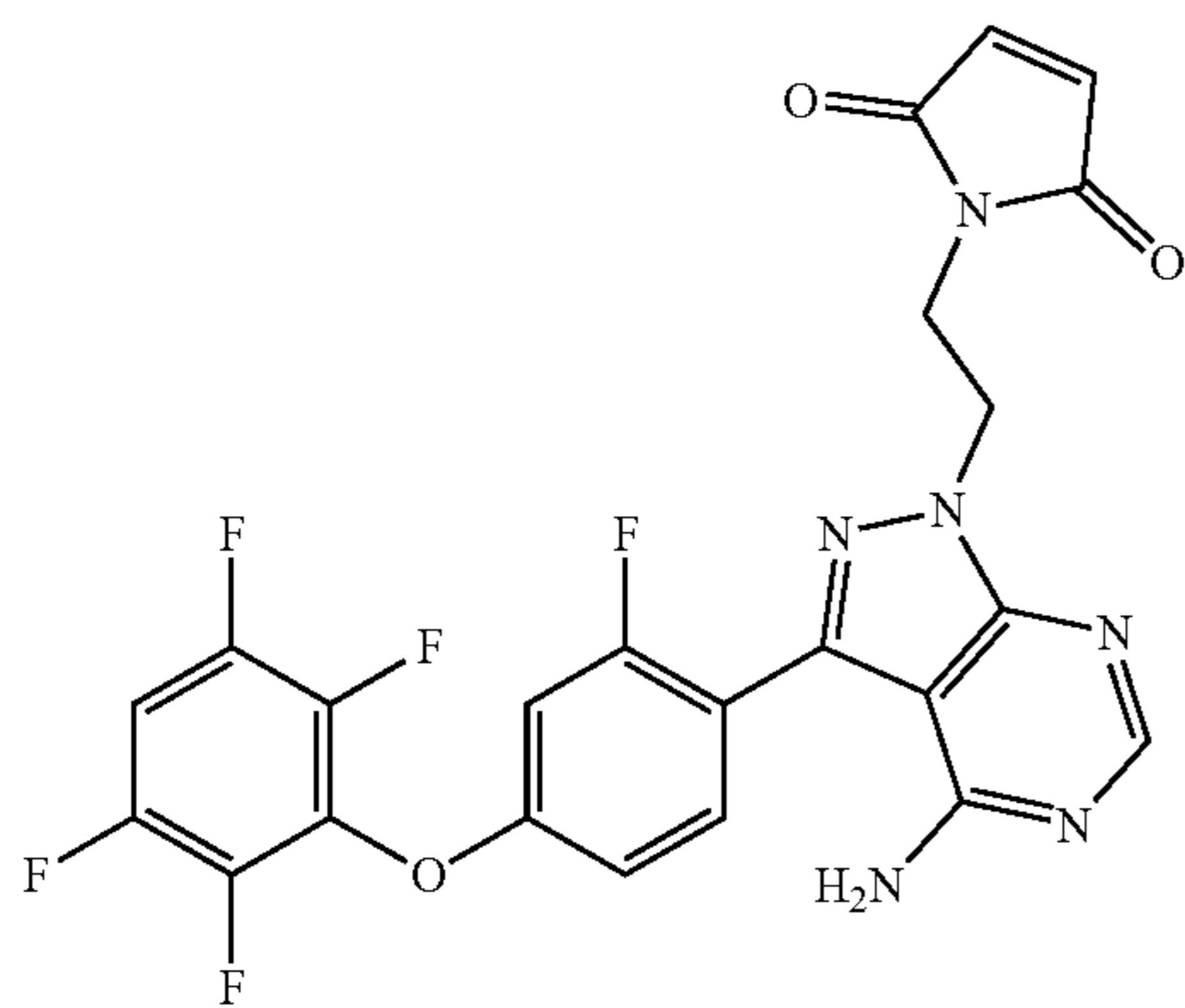
1-(2-(4-amino-3-(2-fluoro-4-(2,3,5,6-tetrafluorophenoxy)phenyl)-1H-pyrazolo[3,4-d]pyrimidin-1-yl)ethyl)-1H-pyrrole-2,5-dione
