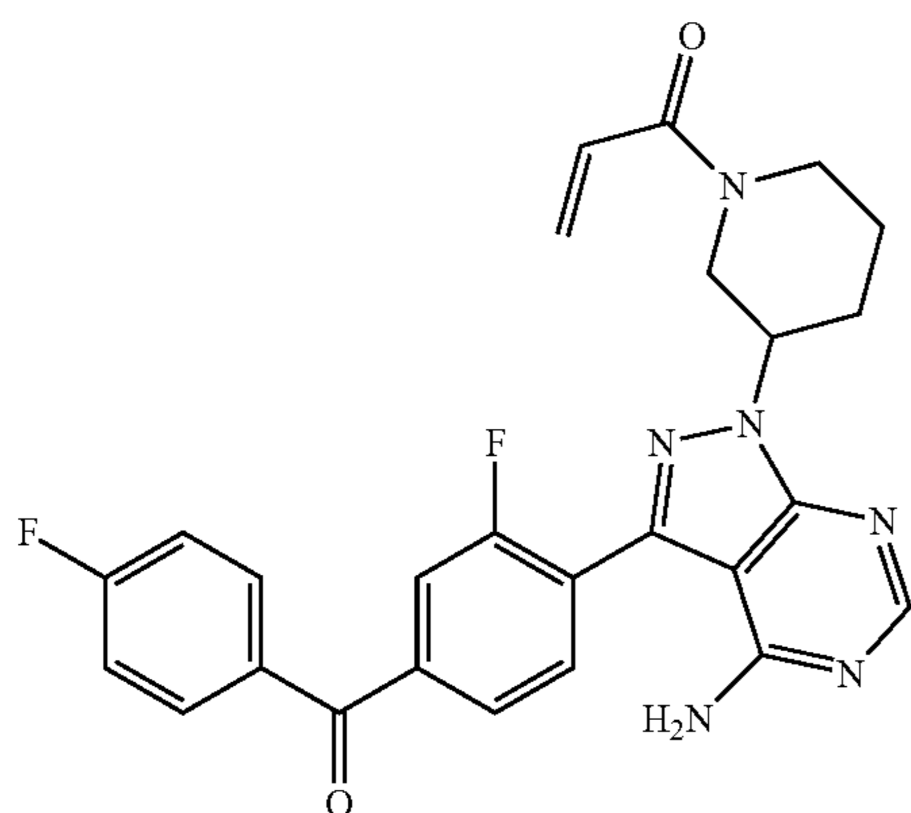
1-(3-(4-amino-3-(2-fluoro-4-(4-fluorobenzoyl)phenyl)-1H-pyrazolo[3,4-d]pyrimidin-1-yl)piperidin-1-yl)prop-2-en-1-one
