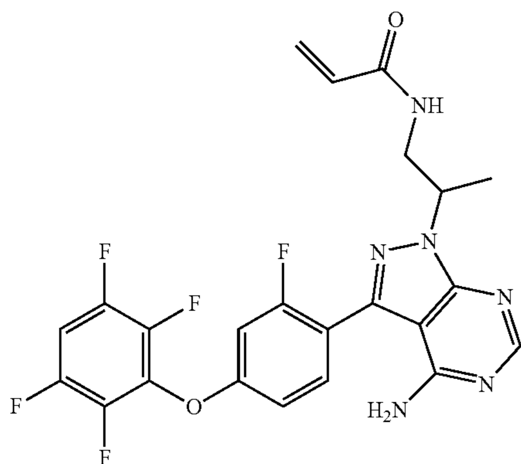
N-(2-(4-amino-3-(2-fluoro-4-(2,3,5,6-tetrafluorophenoxy)phenyl)-1H-pyrazolo[3,4-d]pyrimidin-1-yl)propyl)acrylamide
