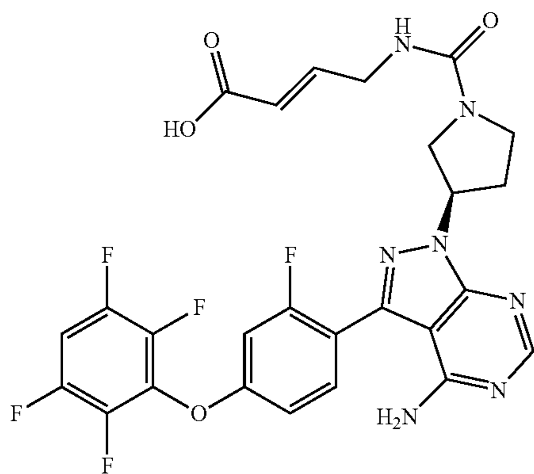
(E)-4-((R)-3-(4-amino-3-(2-fluoro-4-(2,3,5,6-tetrafluorophenoxy)phenyl)-1H-pyrazolo[3,4-d]pyrimidin-1-yl)pyrrolidine-1-carboxamido)but-2-enoic Acid
