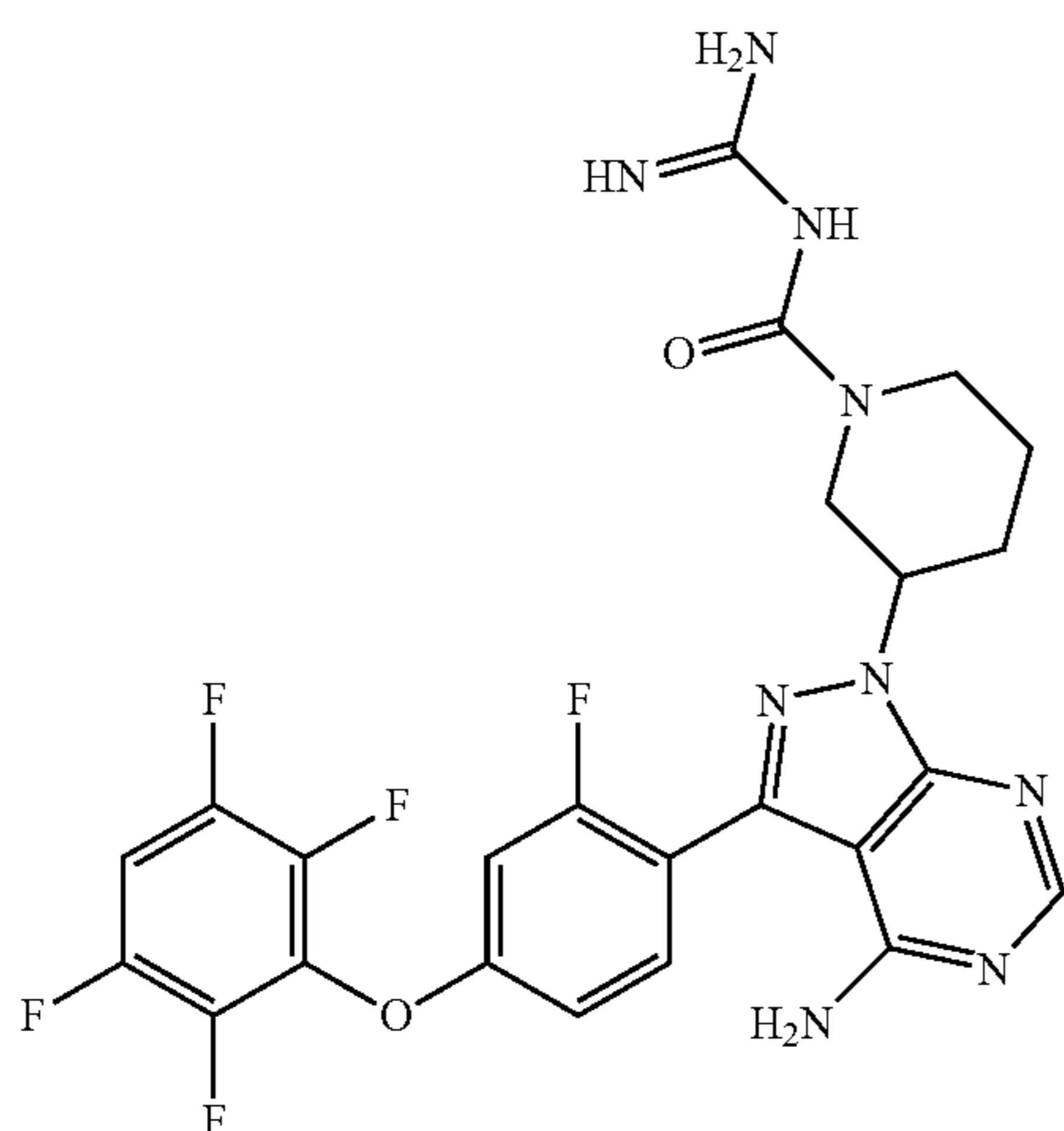
N-[3-[4-amino-3-[2-fluoro-4-(2,3,5,6-trifluorophenoxy)phenyl]-1H-pyrazolo[3,4-d]pyrimidin-1-yl]piperidine-1-carbonyl] formamide
