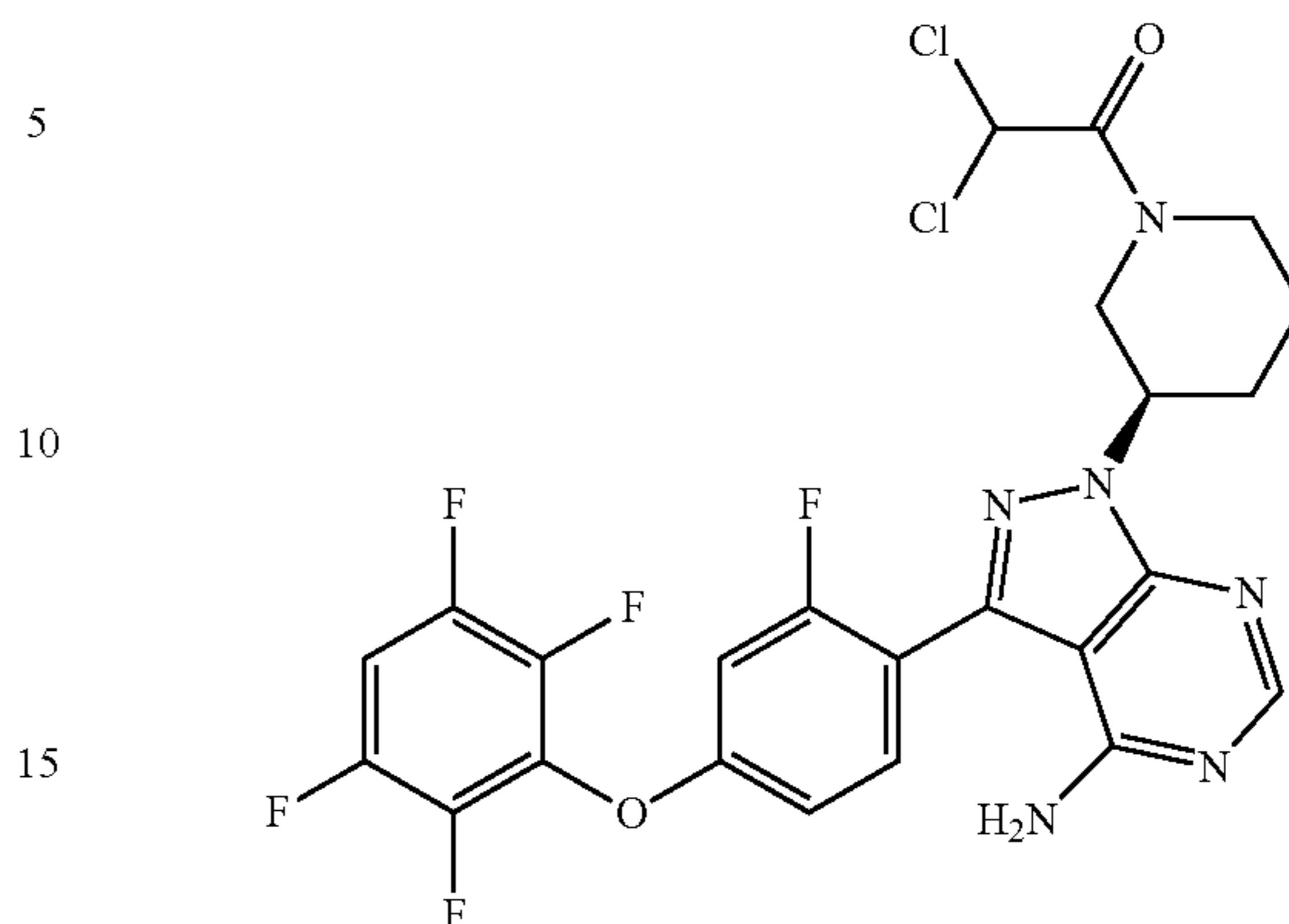
1-((R)-3-(4-amino-3-(2-fluoro-4-(2,3,5,6-tetrafluorophenoxy)phenyl)-1H-pyrazolo[3,4-d]pyrimidin-1-yl)piperidin-1-yl)-2,2-dichloroethanone
