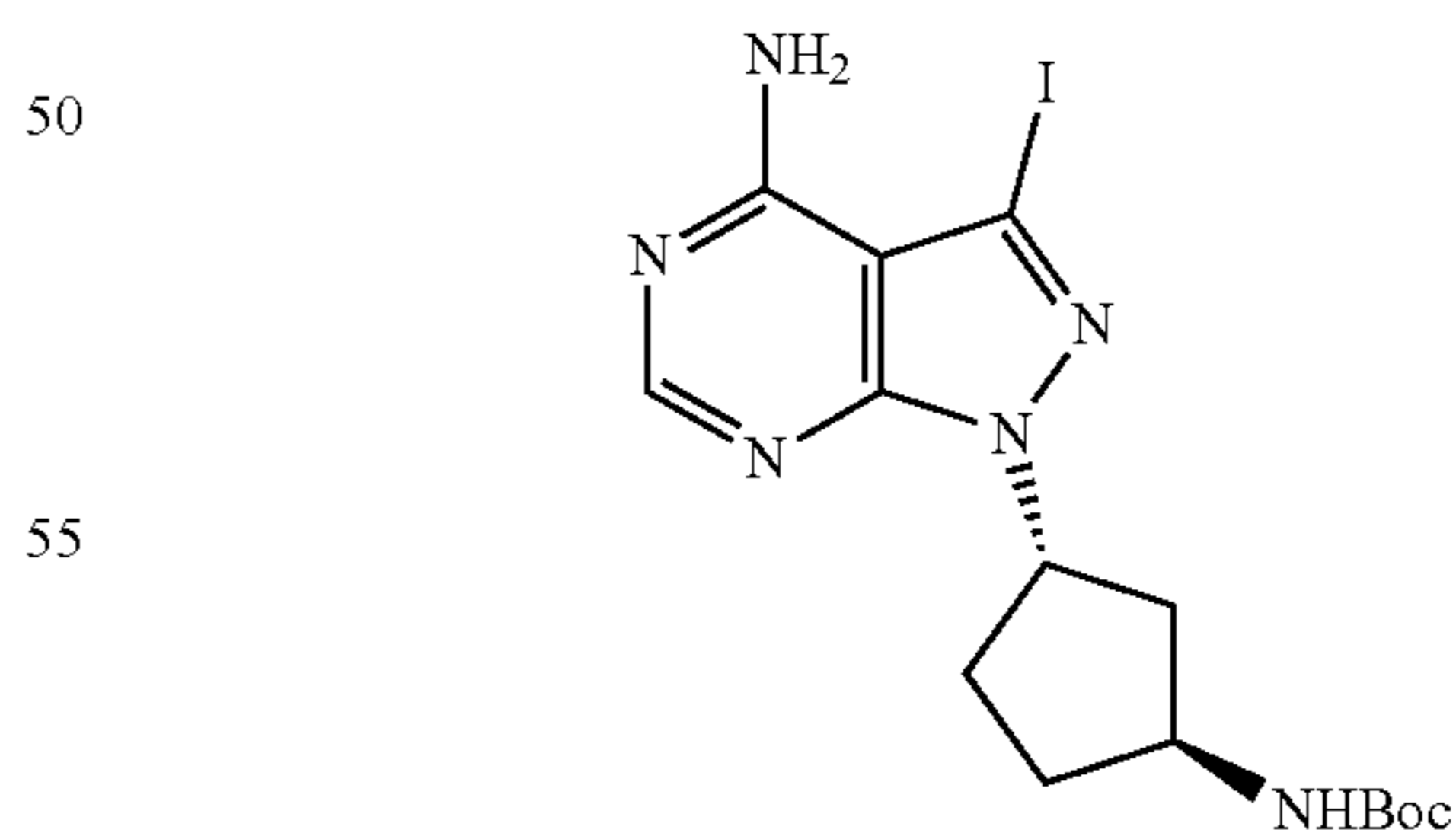
tert-butyl (1S,3S)-3-(4-amino-3-iodo-1H-pyrazolo[3,4-d]pyrimidin-1-yl)cyclopentylcarbamate
