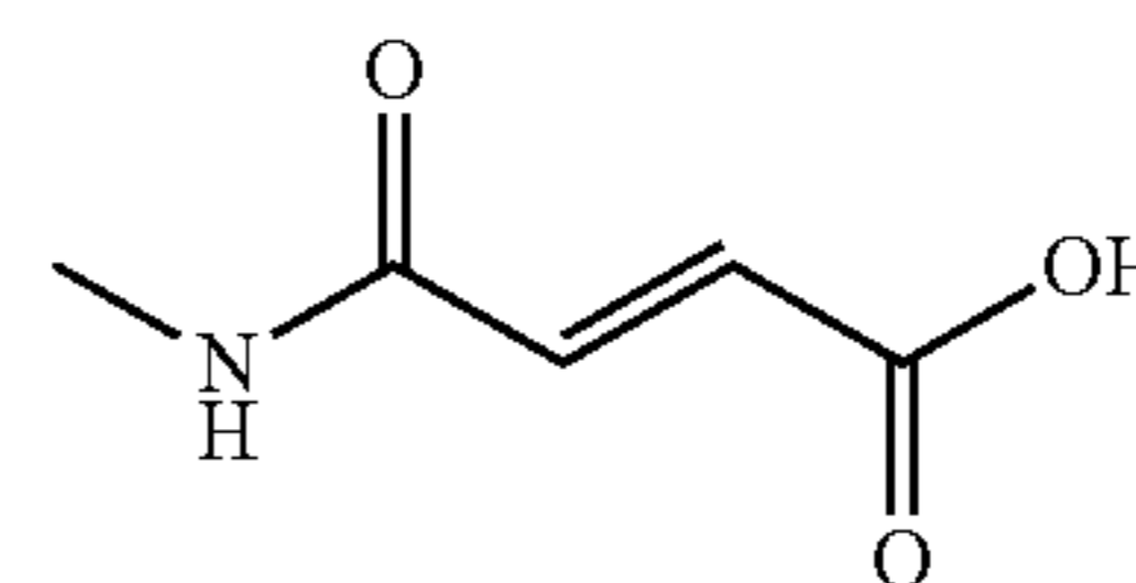
(E)-4-(methylamino)-4-oxobut-2-enoic Acid
