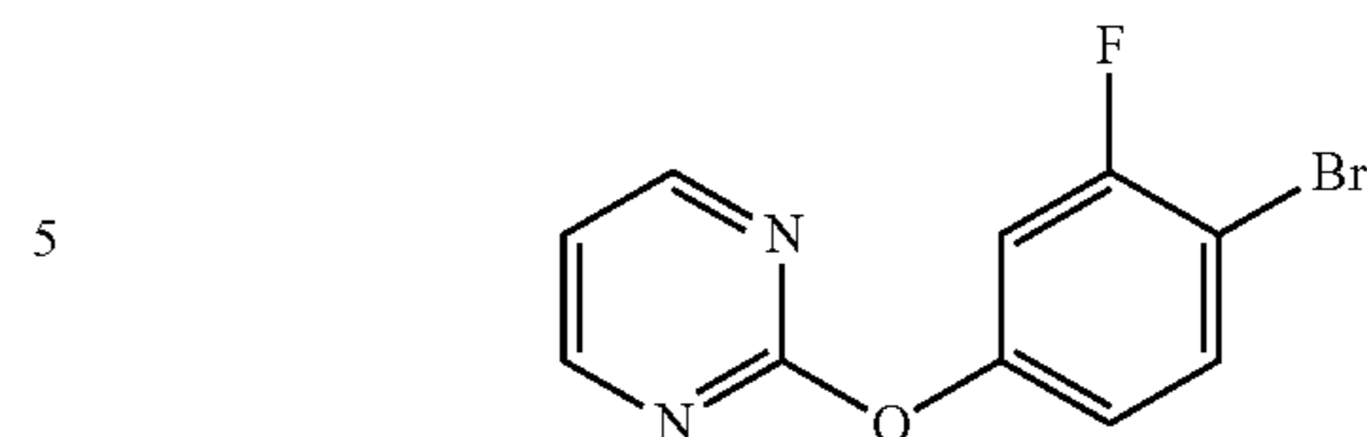
2-(4-bromo-3-fluorophenoxy)pyrimidine
