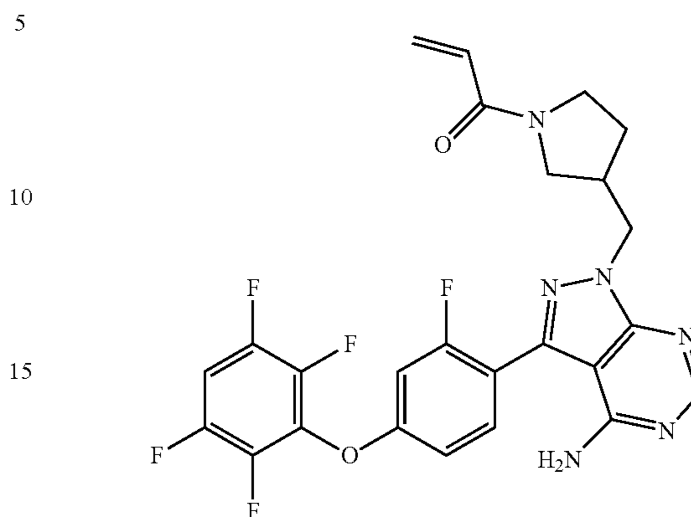
1-(3-((4-amino-3-(2-fluoro-4-(2,3,5,6-tetrafluorophenoxy)phenyl)-1H-pyrazolo[3,4-d]pyrimidin-1-yl)methyl)pyrrolidin-1-yl)prop-2-en-1-one
