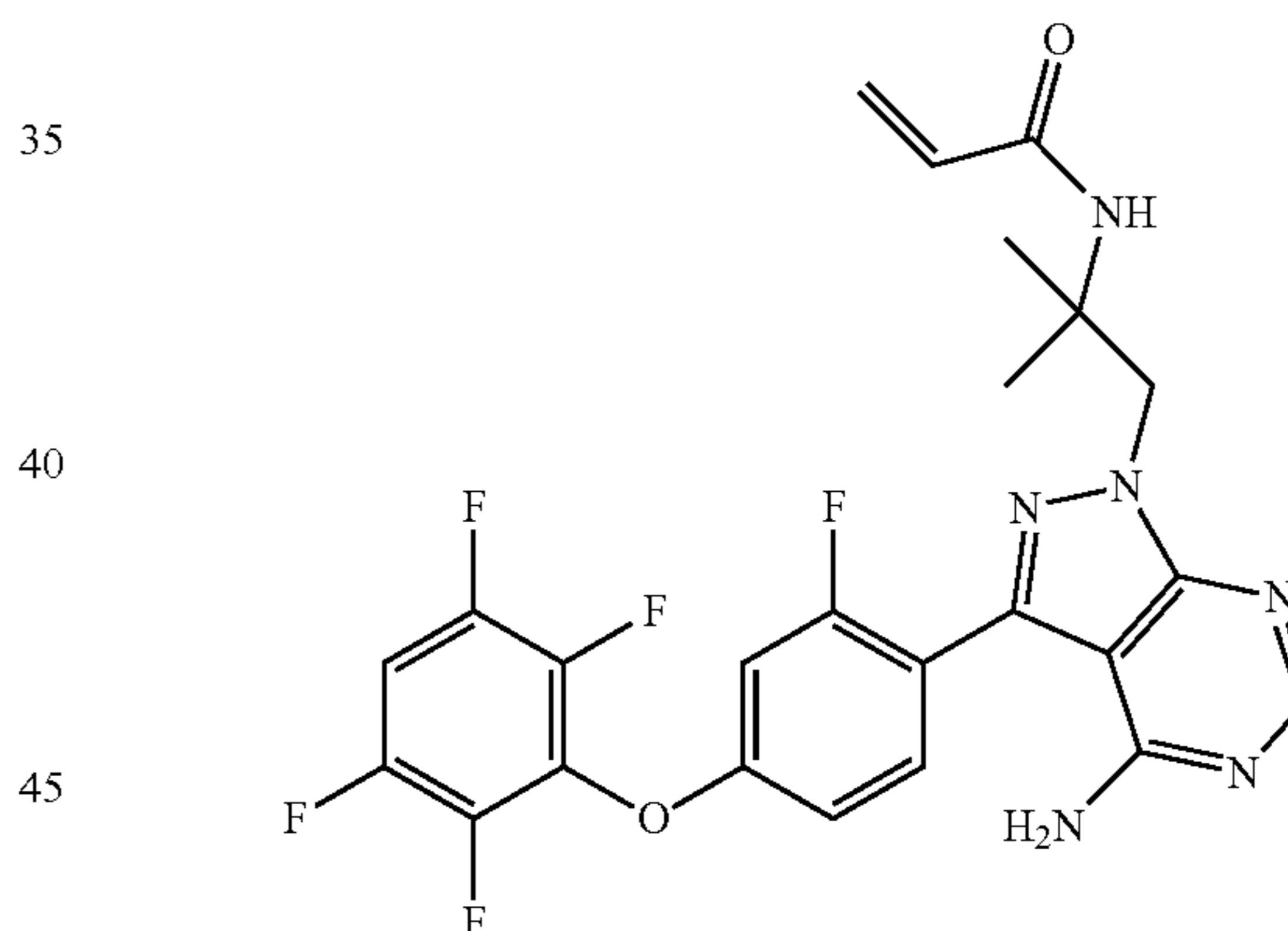
N-(1-(4-amino-3-(2-fluoro-4-(2,3,5,6-tetrafluorophenoxy)phenyl)-1H-pyrazolo[3,4-d]pyrimidin-1-yl)-2-methylpropan-2-yl)acrylamide
