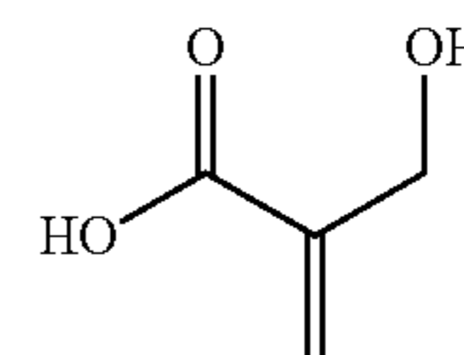
2-(hydroxymethyl)acrylic Acid
