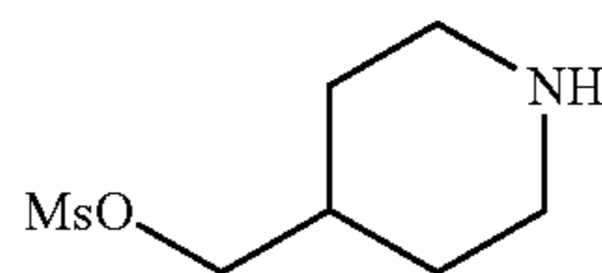
piperidin-4-ylmethyl methanesulfonate
