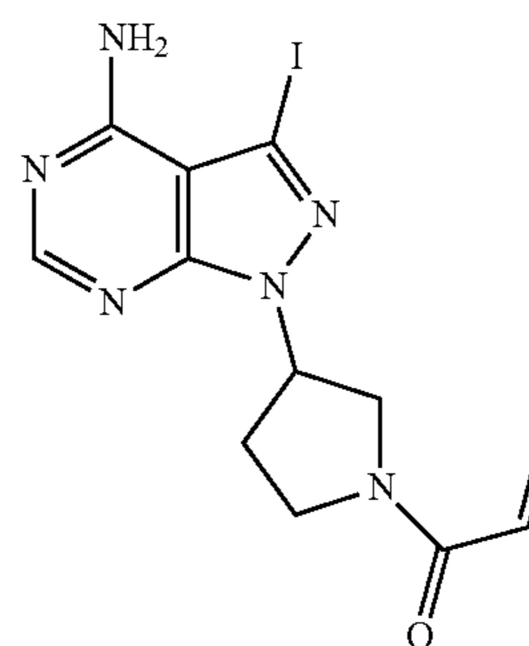
1-(3-(4-amino-3-iodo-1H-pyrazolo[3,4-d]pyrimidin-1-yl)pyrrolidin-1-yl)prop-2-en-1-one
