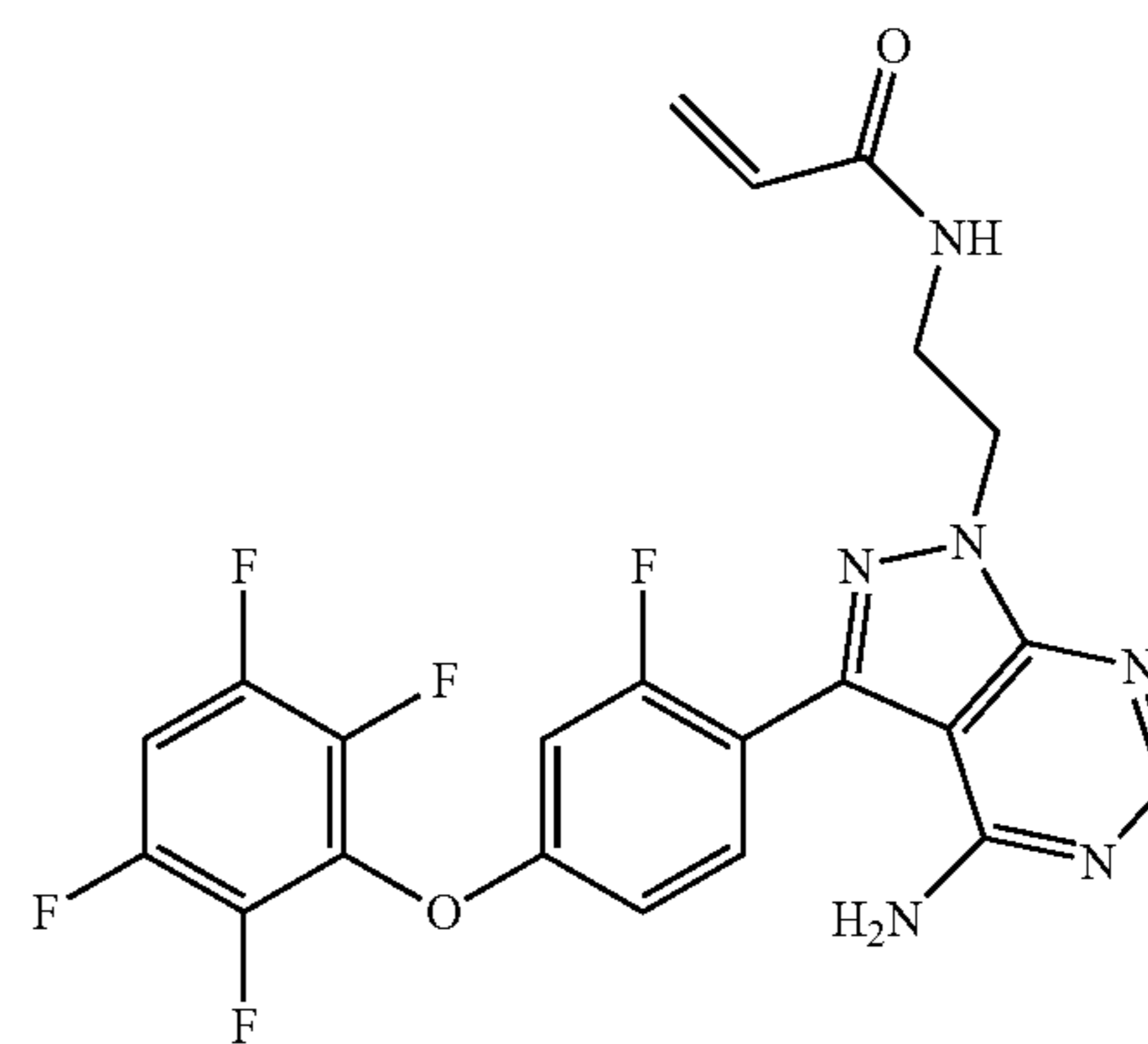
N-(2-(4-amino-3-(2-fluoro-4-(2,3,5,6-tetrafluorophenoxy)phenyl)-1H-pyrazolo[3,4-d]pyrimidin-1-yl)ethyl)acrylamide
