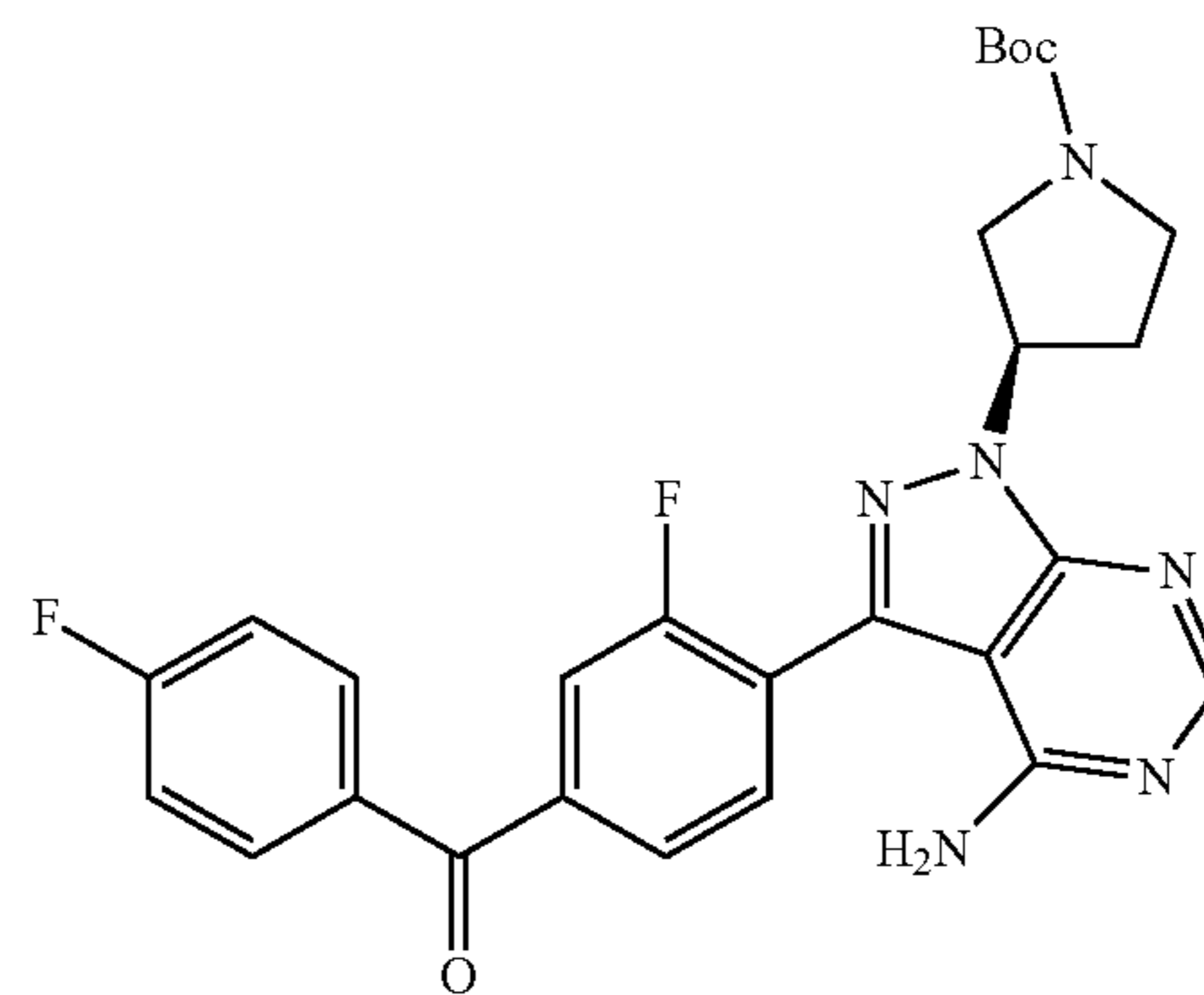
(3R)-tert-butyl 3-(4-amino-3-(2-fluoro-4-(4-fluorobenzoyl)phenyl)-1H-pyrazolo[3,4-d]pyrimidin-1-yl)pyrrolidine-1-carboxylate
