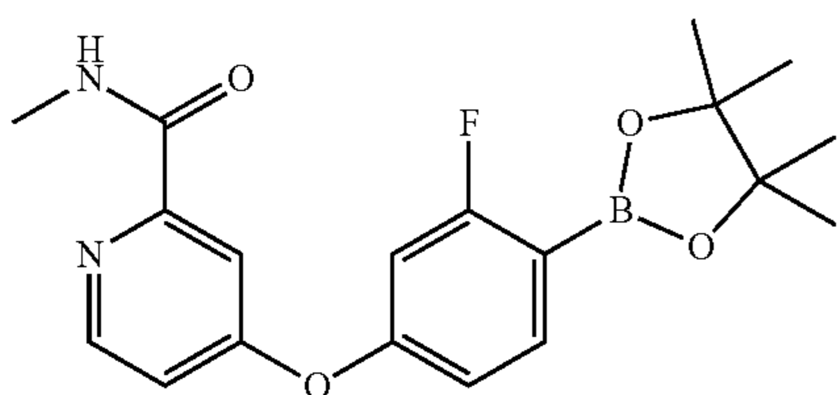
4-(3-fluoro-4-(4,4,5,5-tetramethyl-1,3,2-dioxaborolan-2-yl)phenoxy)-N-methylpicolinamide
