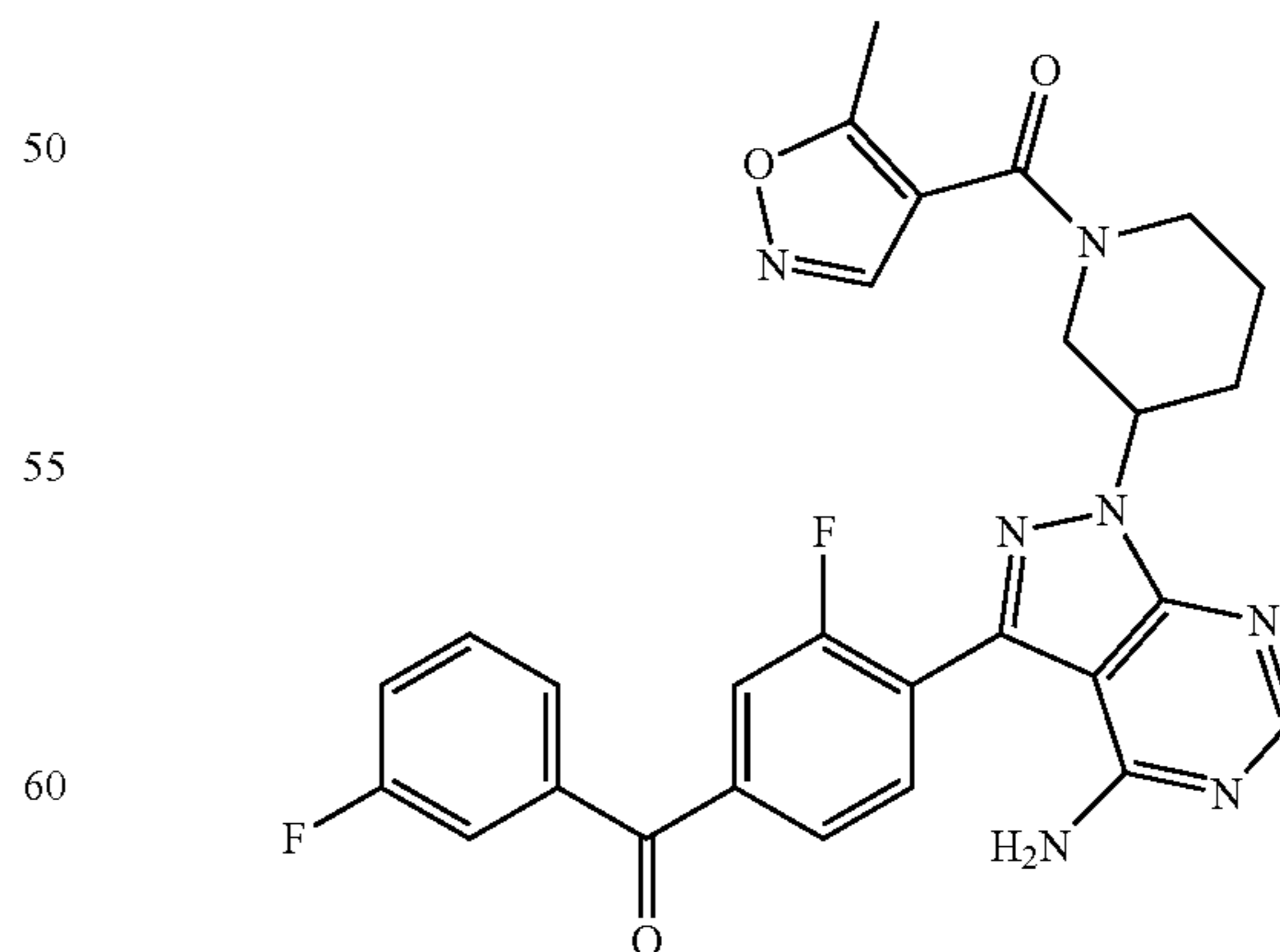
(3-(4-amino-3-(2-fluoro-4-(3-fluorobenzoyl)phenyl)-1H-pyrazolo[3,4-d]pyrimidin-1-yl)piperidin-1-yl)(5-methylisoxazol-4-yl)methanone
