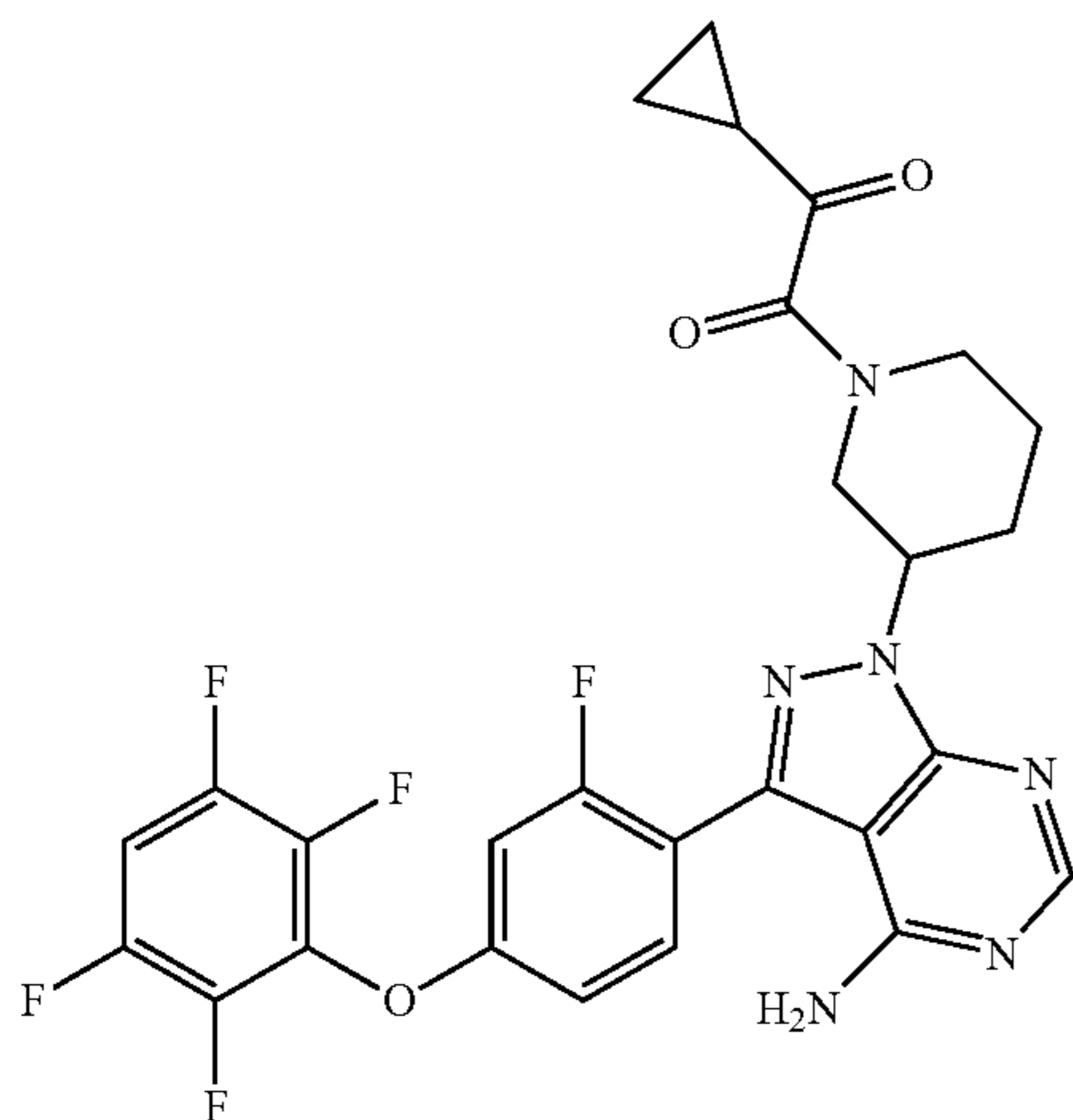
1-(3-(4-amino-3-(2-fluoro-4-(2,3,5,6-tetrafluorophenoxy)phenyl)-1H-pyrazolo[3,4-d]pyrimidin-1-yl)piperidin-1-yl)-2-cyclopropylethane-1,2-dione
