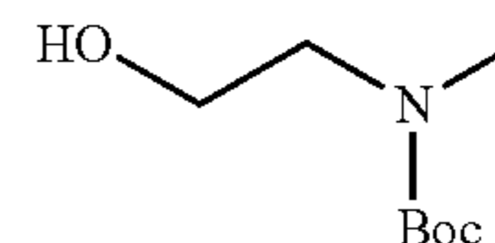
tert-butyl 2-hydroxyethyl(methyl)carbamate
