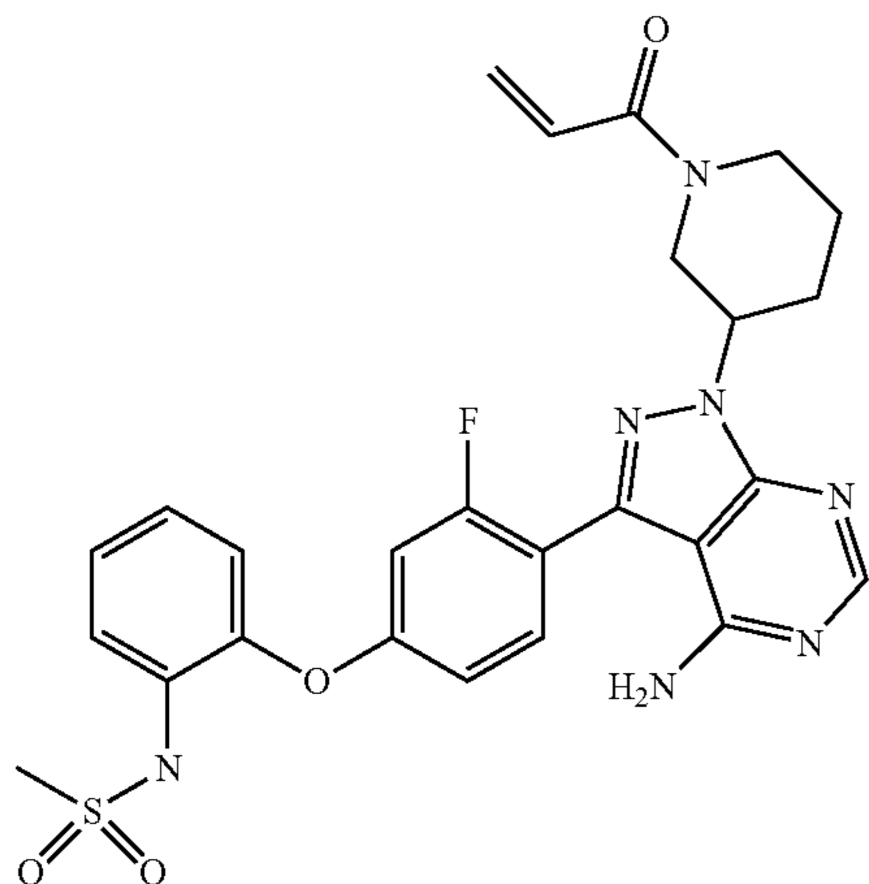
N-(2-(4-(1-(1-acryloylpiperidin-3-yl)-4-amino-1H-pyrazolo[3,4-d]pyrimidin-3-yl)-3-fluorophenoxy)phenyl)methanesulfonamide
