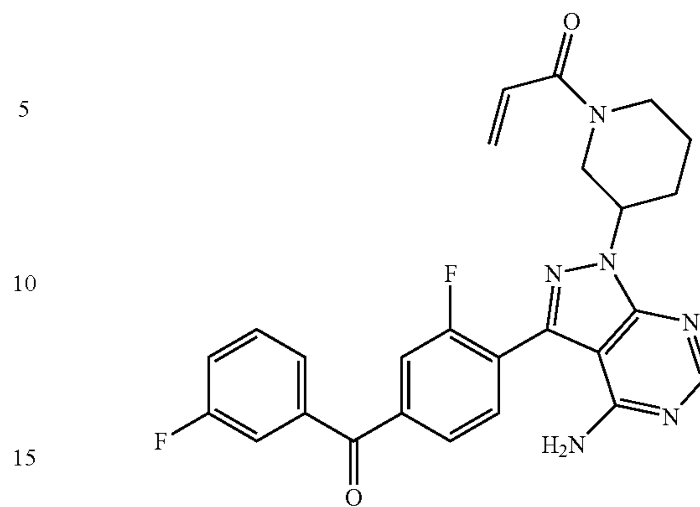
1-(3-(4-amino-3-(2-fluoro-4-(3-fluorobenzoyl)phenyl)-1H-pyrazolo[3,4-d]pyrimidin-1-yl)piperidin-1-yl)prop-2-en-1-one
