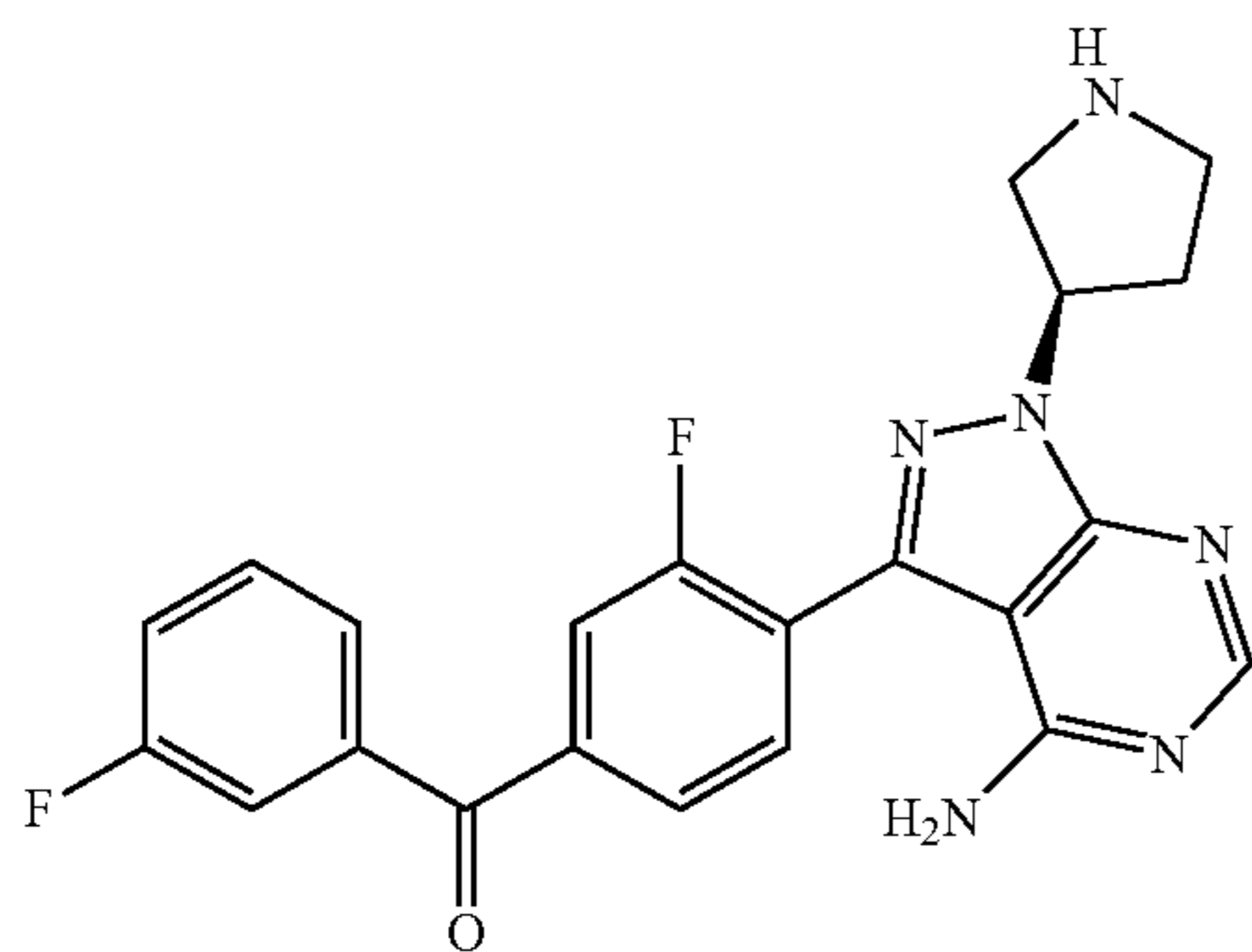
(4-(4-amino-1-((R)-pyrrolidin-3-yl)-1H-pyrazolo[3,4-d]pyrimidin-3-yl)-3-fluorophenyl)(3-fluorophenyl)methanone
