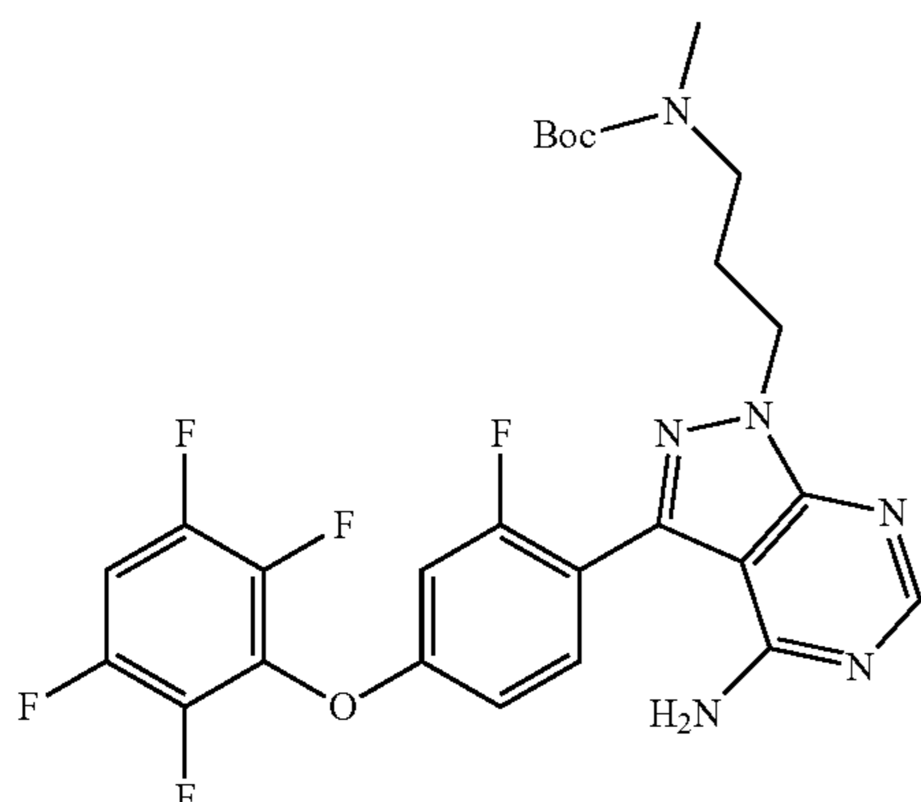
tert-butyl 3-(4-amino-3-(2-fluoro-4-(2,3,5,6-tetrafluorophenoxy)phenyl)-1H-pyrazolo[3,4-d]pyrimidin-1-yl)propyl(methyl)carbamate
