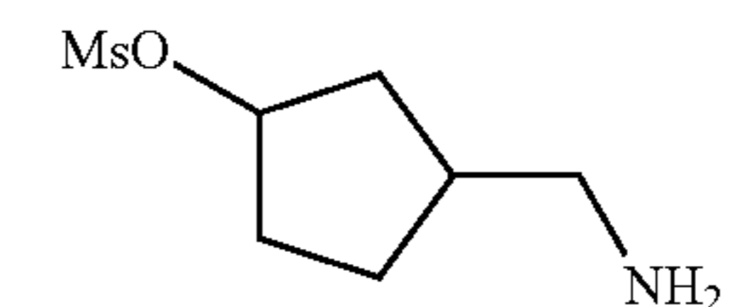
3-(aminomethyl)cyclopentyl methanesulfonate
