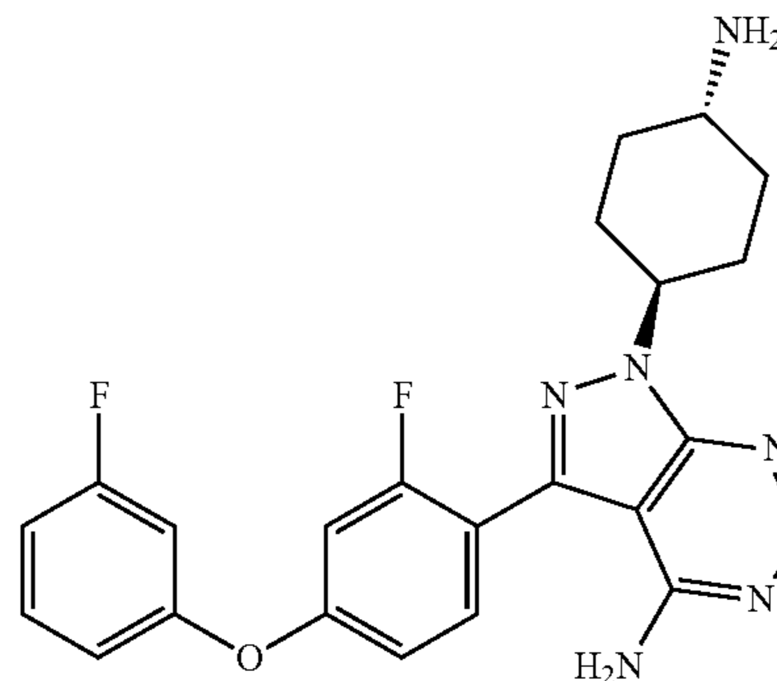
1-((1r,4r)-4-aminocyclohexyl)-3-(2-fluoro-4-(3-fluorophenoxy)phenyl)-1H-pyrazolo[3,4-d]pyrimidin-4-amine
