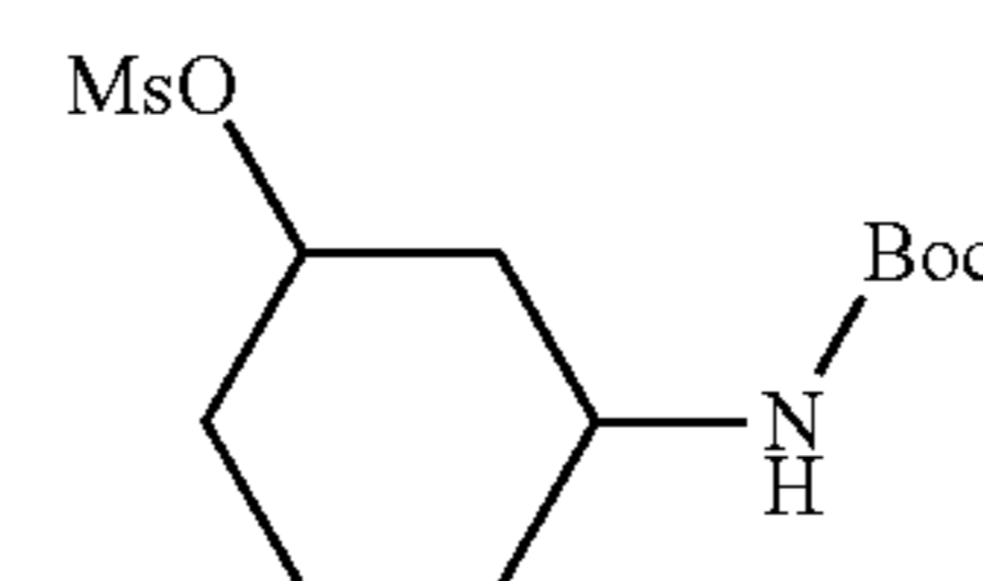
3-(tert-butoxycarbonyl)cyclohexyl methanesulfonate
