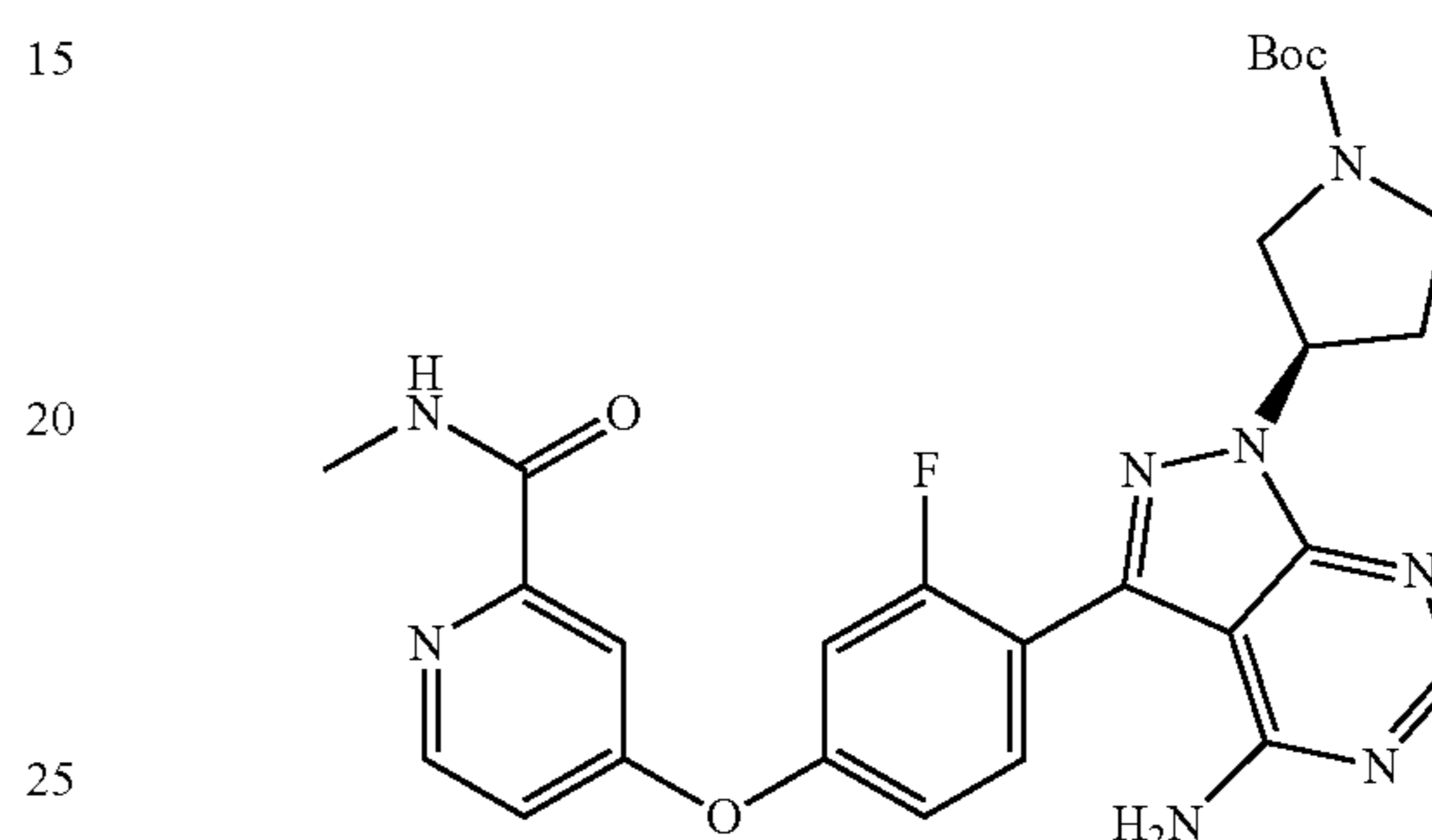
(3R)-tert-butyl 3-(4-amino-3-(2-fluoro-4-(2-(methylcarbamoyl)pyridin-4-yloxy)phenyl)-1H-pyrazolo[3,4-d]pyrimidin-1-yl)pyrrolidine-1-carboxylate
