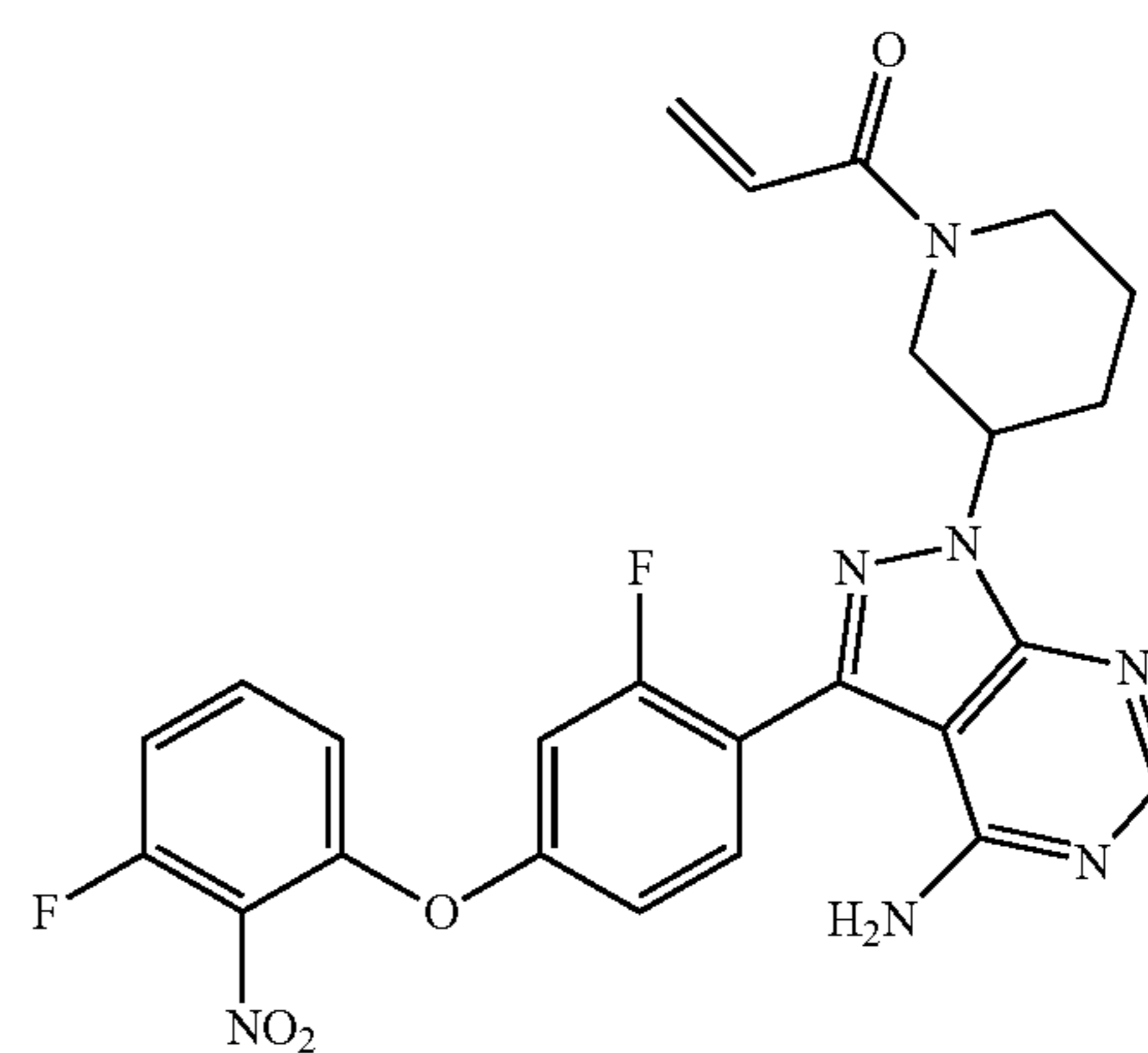
1-(3-(4-amino-3-(2-fluoro-4-(3-fluoro-2-nitro phenoxy)phenyl)-1H-pyrazolo[3,4-d]pyrimidin-1-yl)piperidin-1-yl)prop-2-en-1-one
