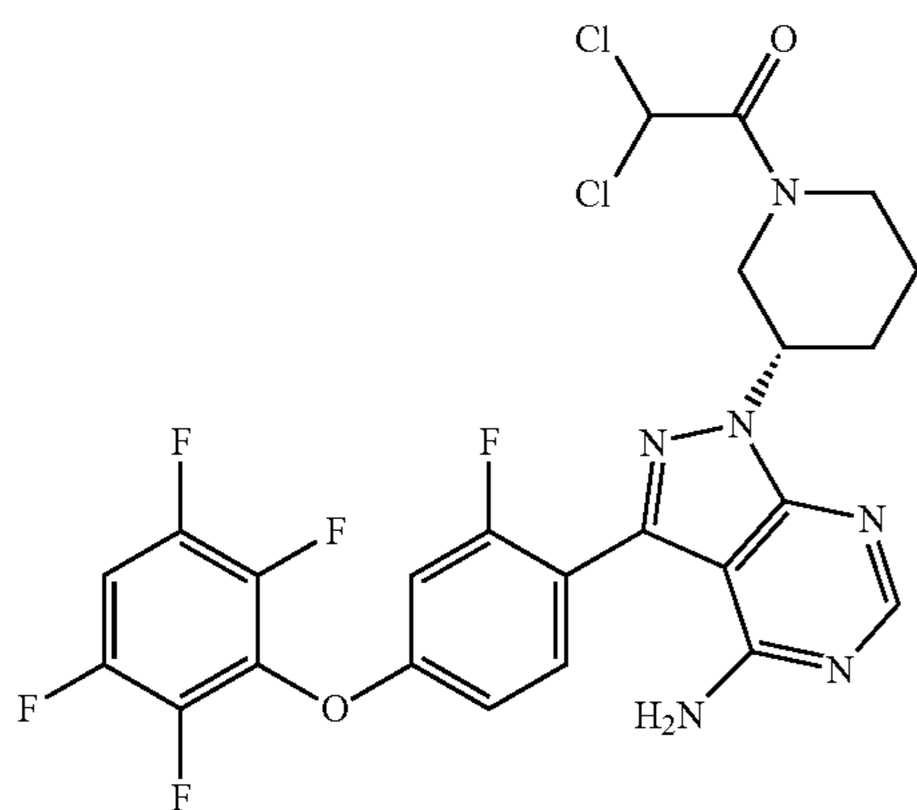
1-((S)-3-(4-amino-3-(2-fluoro-4-(2,3,5,6-tetrafluorophenoxy)phenyl)-1H-pyrazolo[3,4-d]pyrimidin-1-yl)piperidin-1-yl)-2,2-dichloroethanone
