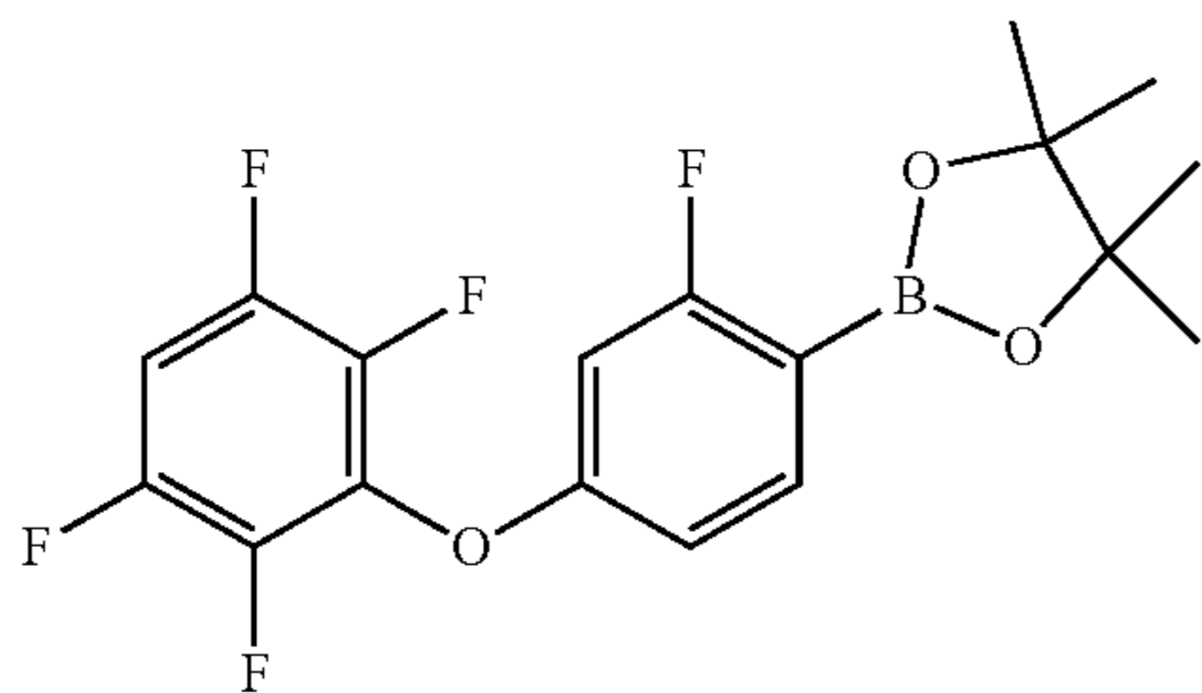
2-(2-fluoro-4-(2,3,5,6-tetrafluorophenoxy)phenyl)-4,4,5,5-tetramethyl-1,3,2-dioxaborolane
