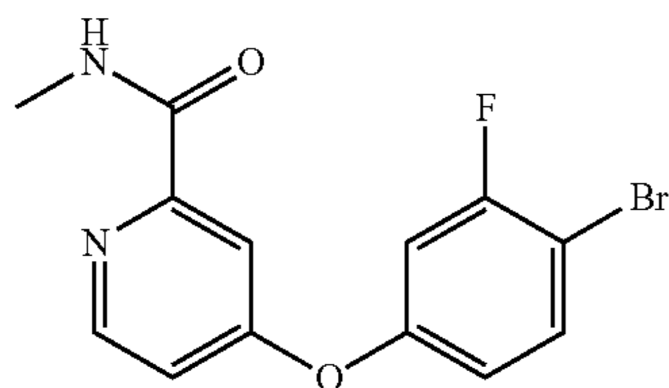
4-(4-bromo-3-fluorophenoxy)-N-methylpicolinamide
