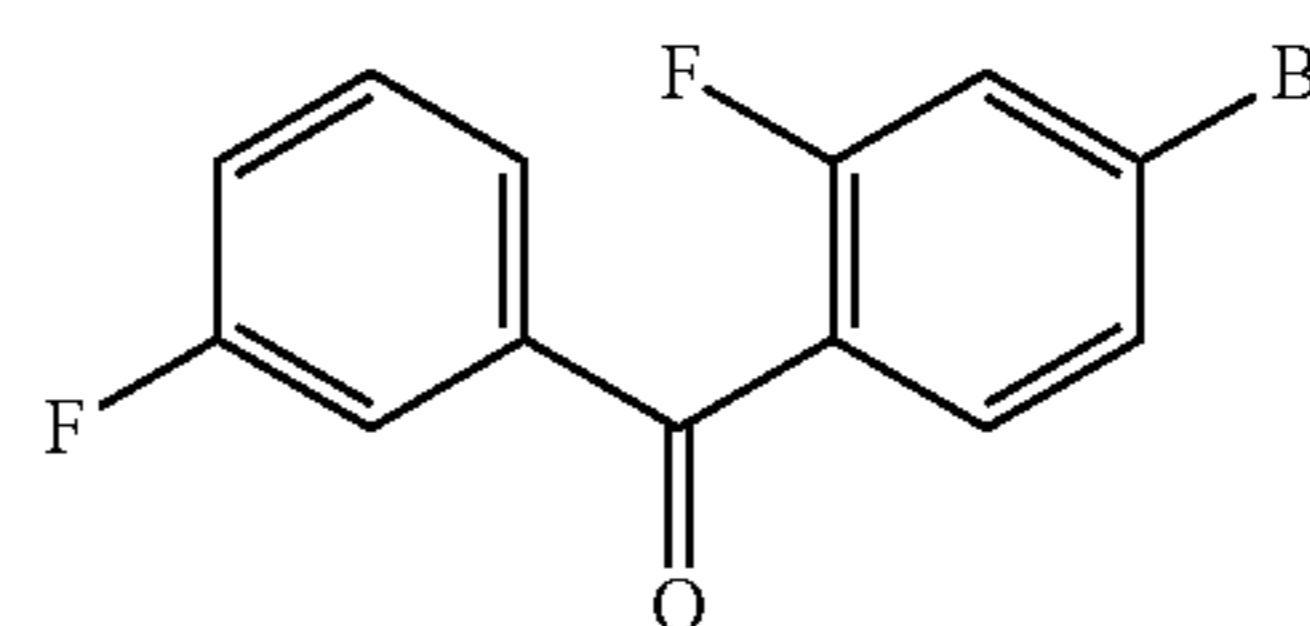
(4-bromo-2-fluorophenyl)(3-fluorophenyl)methanone
