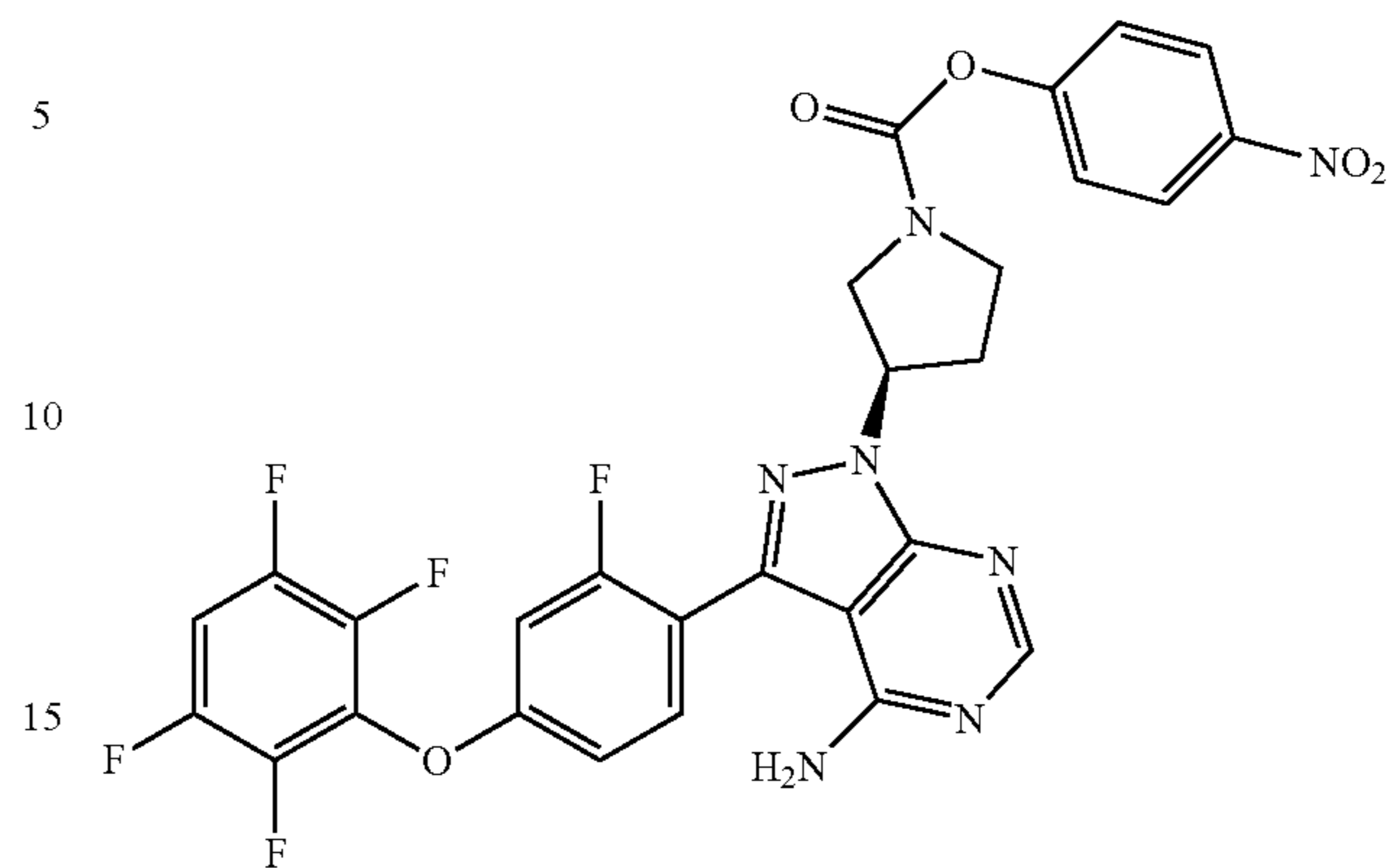
(3R)-4-nitrophenyl 3-(4-amino-3-(2-fluoro-4-(2,3,5,6-tetrafluorophenoxy)phenyl)-1H-pyrazolo[3,4-d]pyrimidin-1-yl)pyrrolidine-1-carboxylate
