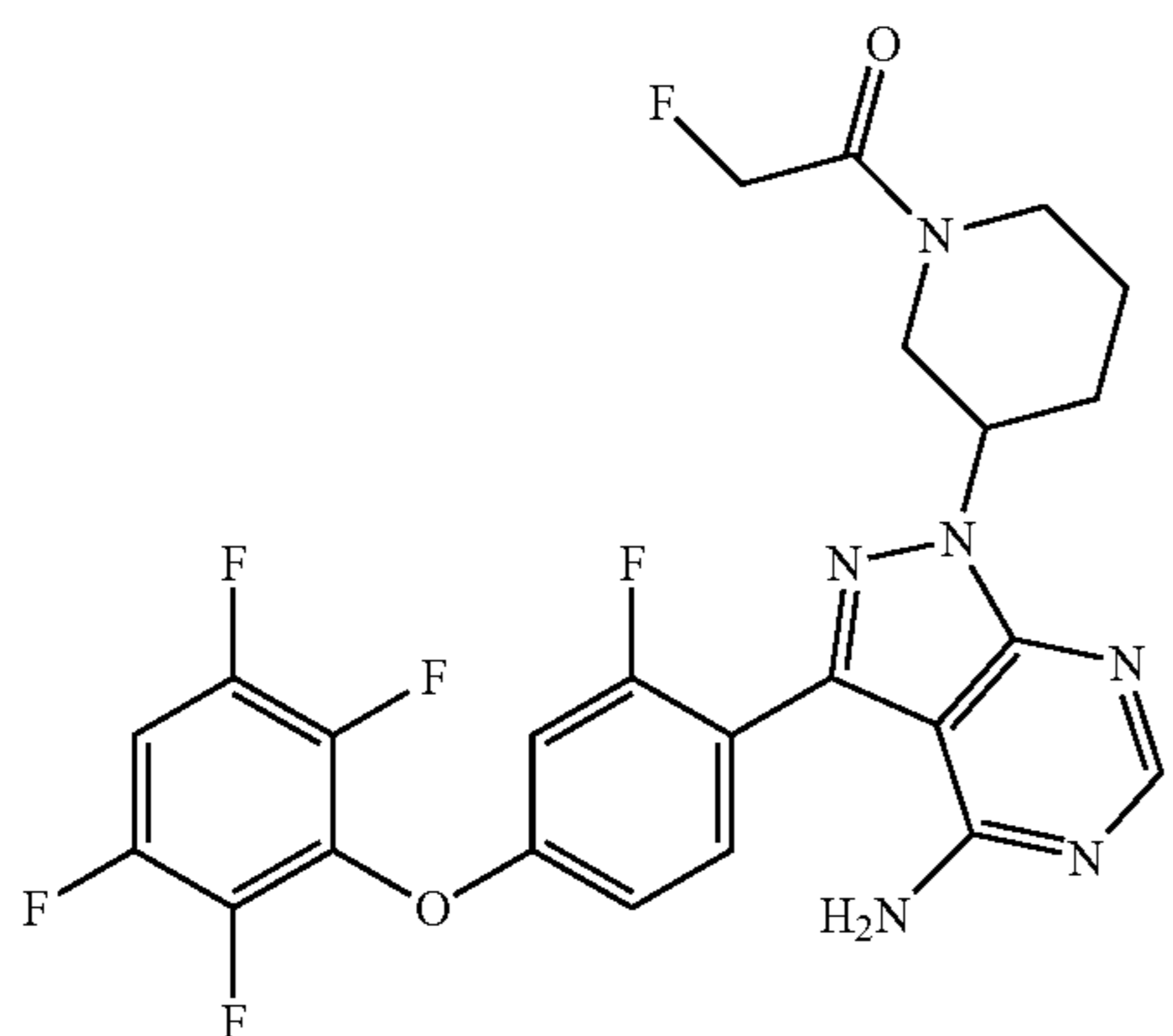
1-(3-(4-amino-3-(2-fluoro-4-(2,3,5,6-tetrafluorophenoxy)phenyl)-1H-pyrazolo[3,4-d]pyrimidin-1-yl) piperidin-1-yl)-2-fluoroethanone
