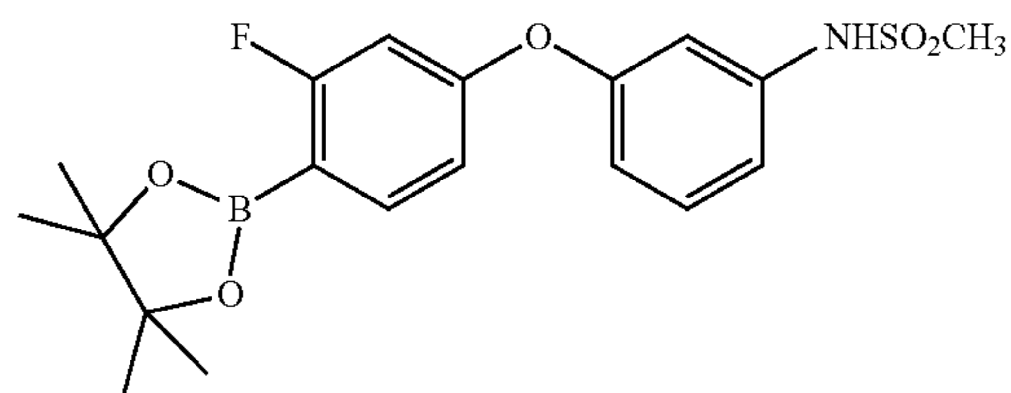
N-(3-(3-fluoro-4-(4,4,5,5-tetramethyl-1,3,2-dioxaborolan-2-yl)phenoxy)phenyl)methanesulfonamide
