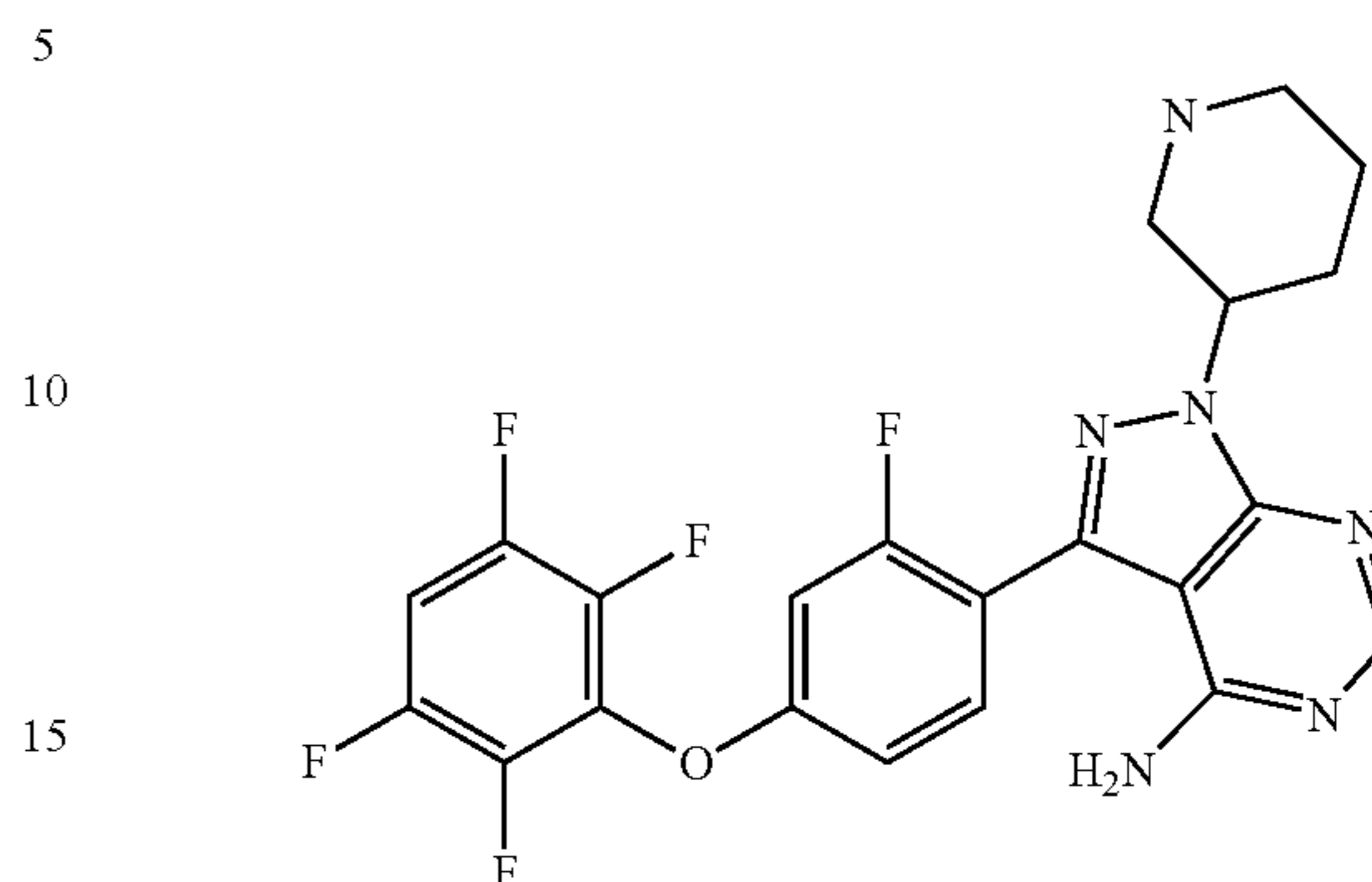
3-(2-fluoro-4-(2,3,5,6-tetrafluorophenoxy)phenyl)-1-(piperidin-3-yl)-1H-pyrazolo[3,4-d]pyrimidin-4-amine
