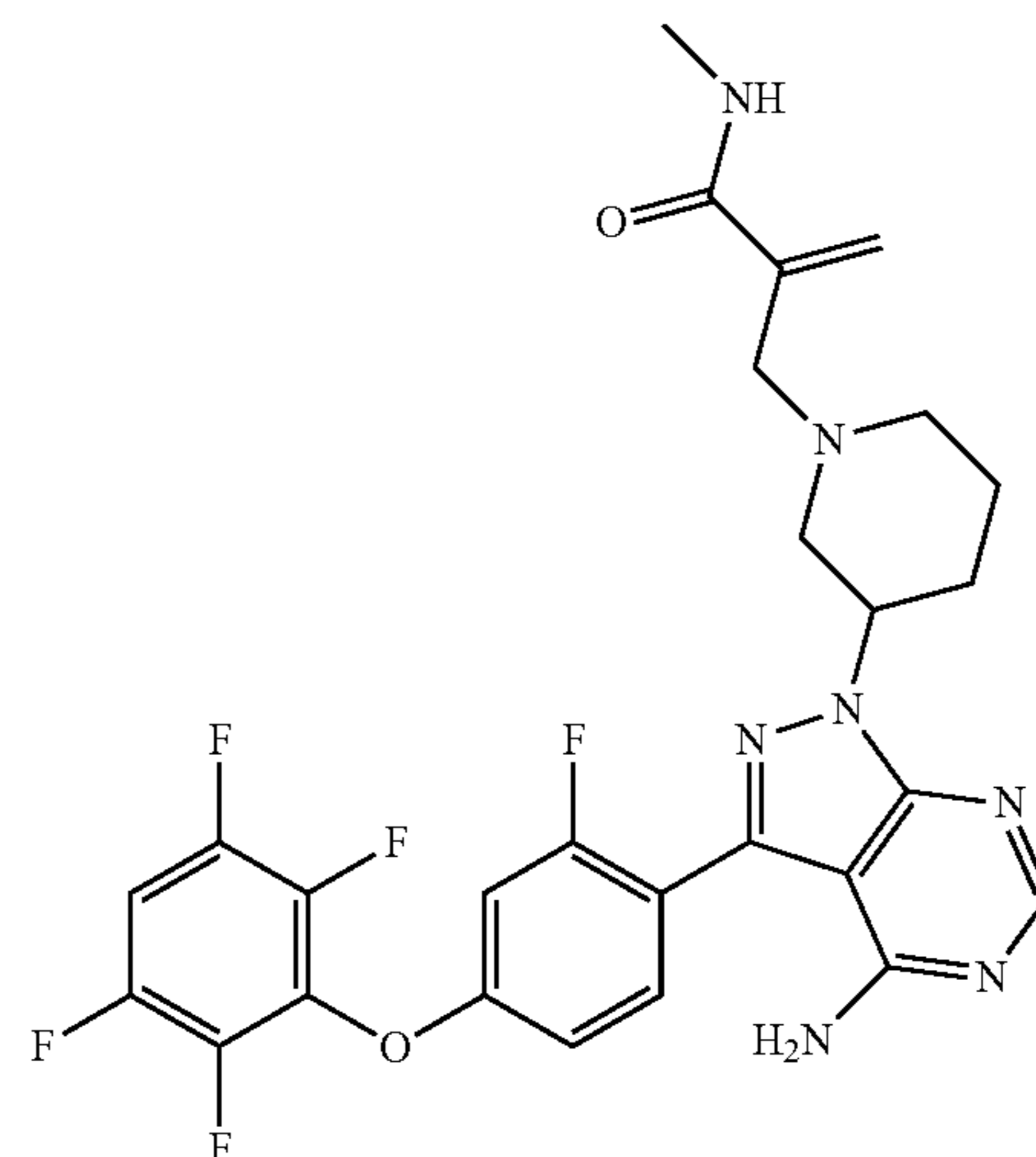
2-((3-(4-amino-3-(2-fluoro-4-(2,3,5,6-tetrafluorophenoxy)phenyl)-1H-pyrazolo[3,4-d]pyrimidin-1-yl)piperidin-1-yl)methyl)-N-methylacrylamide
