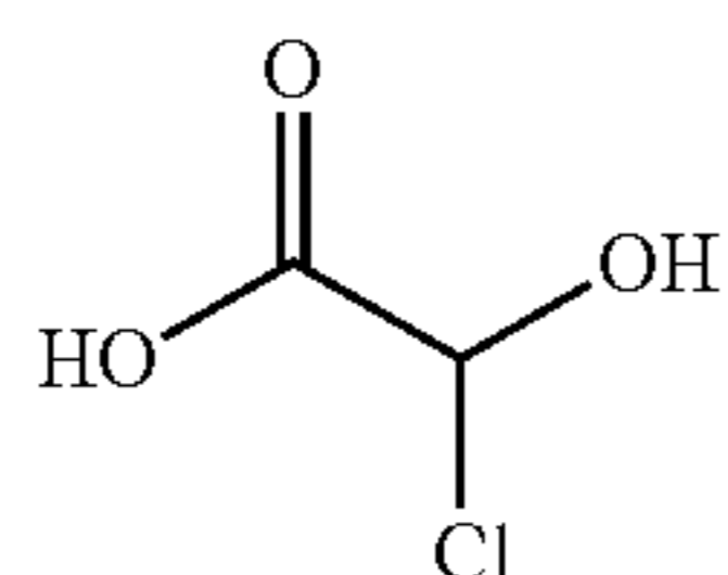
2-chloro-2-hydroxyacetic Acid
