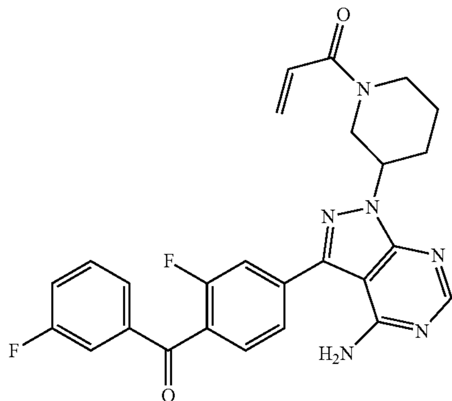
1-(3-(4-amino-3-(3-fluoro-4-(3-fluorobenzoyl)phenyl)-1H-pyrazolo[3,4-d]pyrimidin-1-yl)piperidin-1-yl)prop-2-en-1-one
