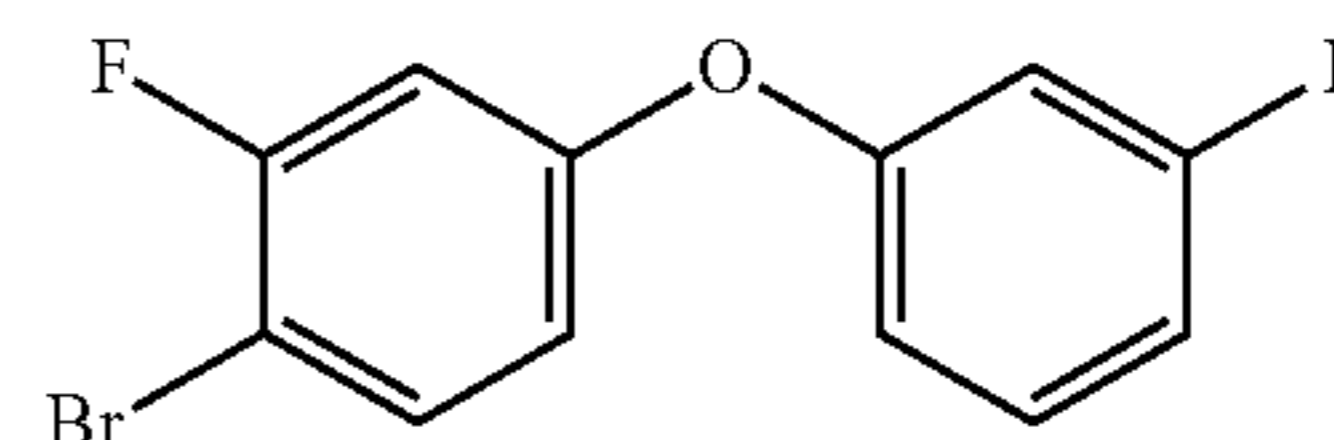
1-bromo-2-fluoro-4-(3-fluorophenoxy)benzene
