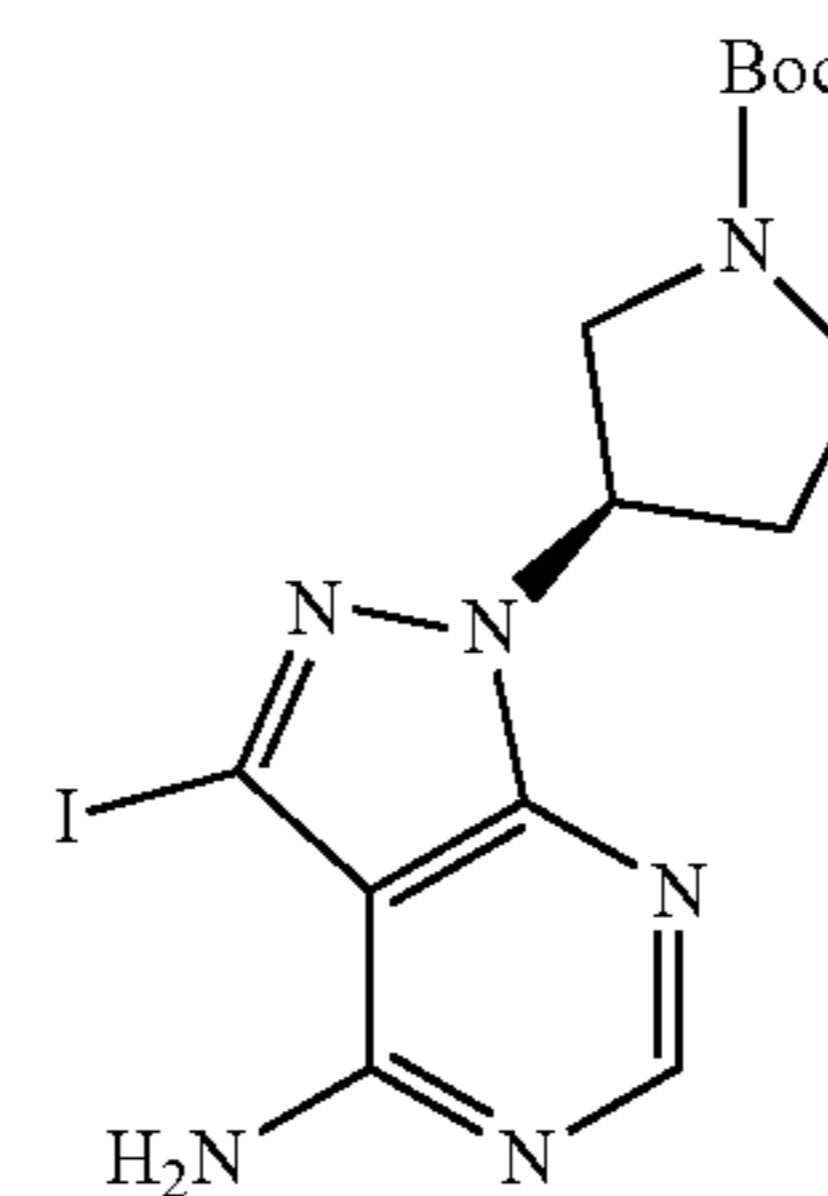
(R)-tert-butyl 3-(4-amino-3-iodo-1H-pyrazolo[3,4-d]pyrimidin-1-yl)pyrrolidine-1-carboxylate
