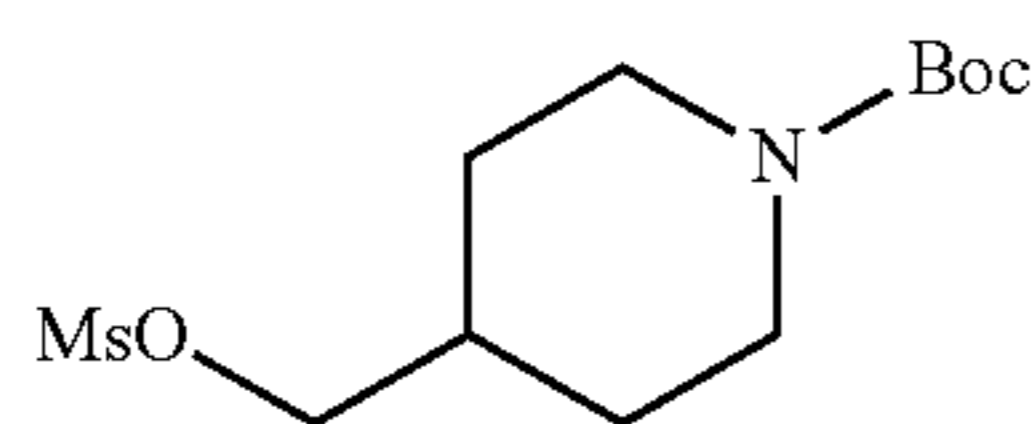
tert-butyl 4-((methylsulfonyloxy)methyl)piperidine-1-carboxylate
