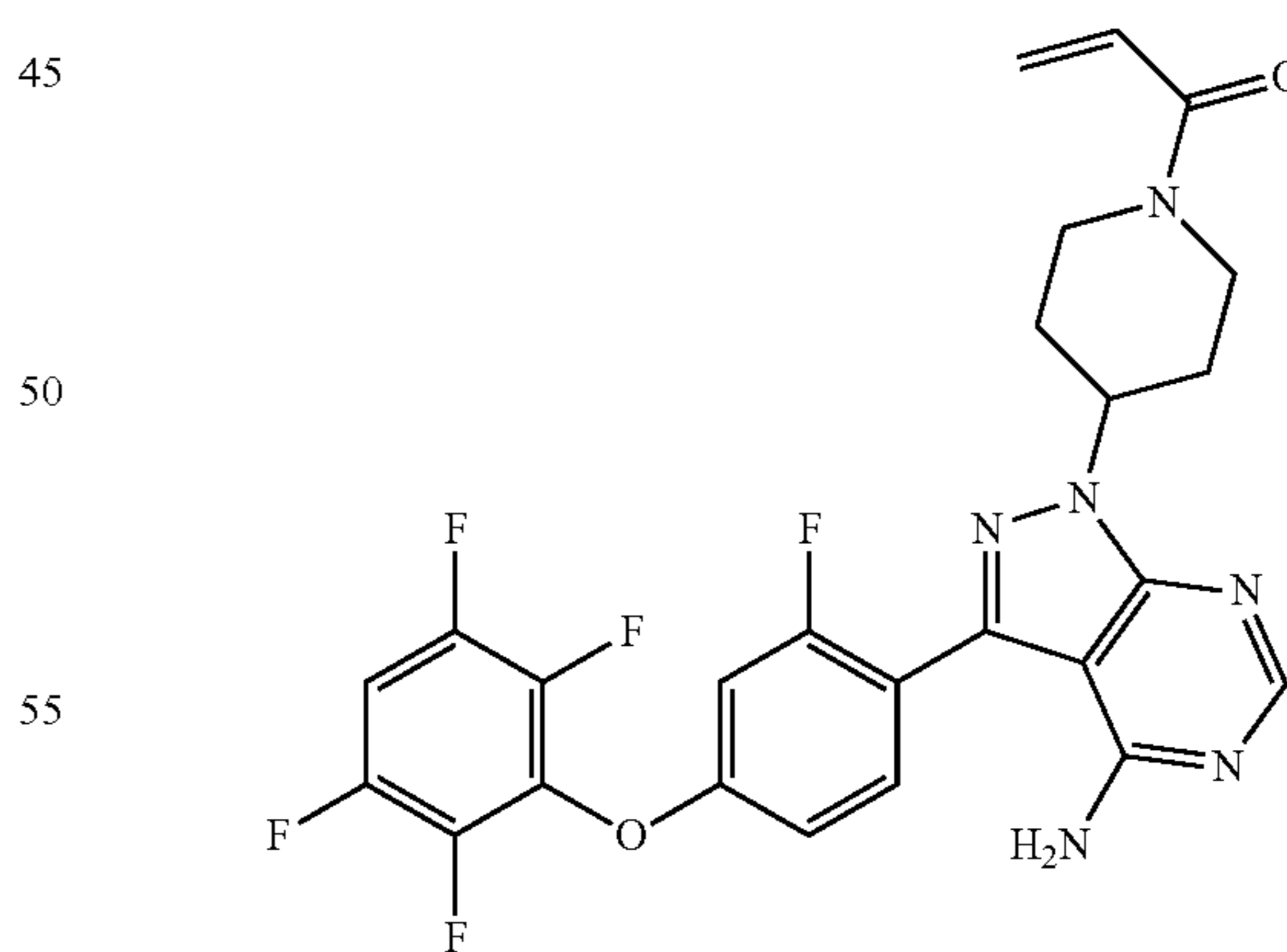
1-(4-(4-amino-3-(2-fluoro-4-(2,3,5,6-tetrafluorophenoxy)phenyl)-1H-pyrazolo[3,4-d]pyrimidin-1-yl)piperidin-1-yl)prop-2-en-1-one
