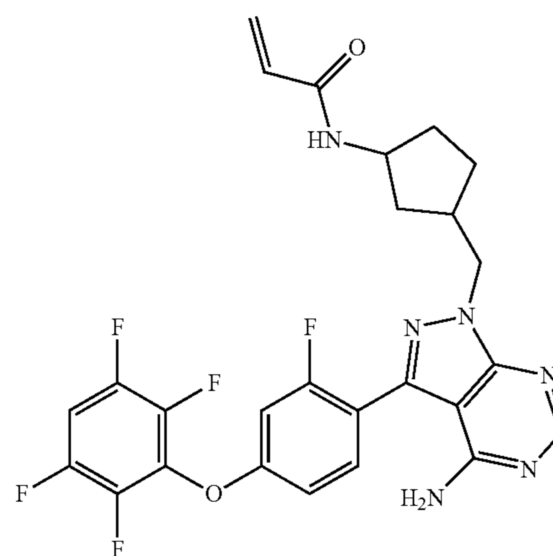
N-(3-((4-amino-3-(2-fluoro-4-(2,3,5,6-tetrafluorophenoxy)phenyl)-1H-pyrazolo[3,4-d]pyrimidin-1-yl)methyl)cyclopentyl)acrylamide
