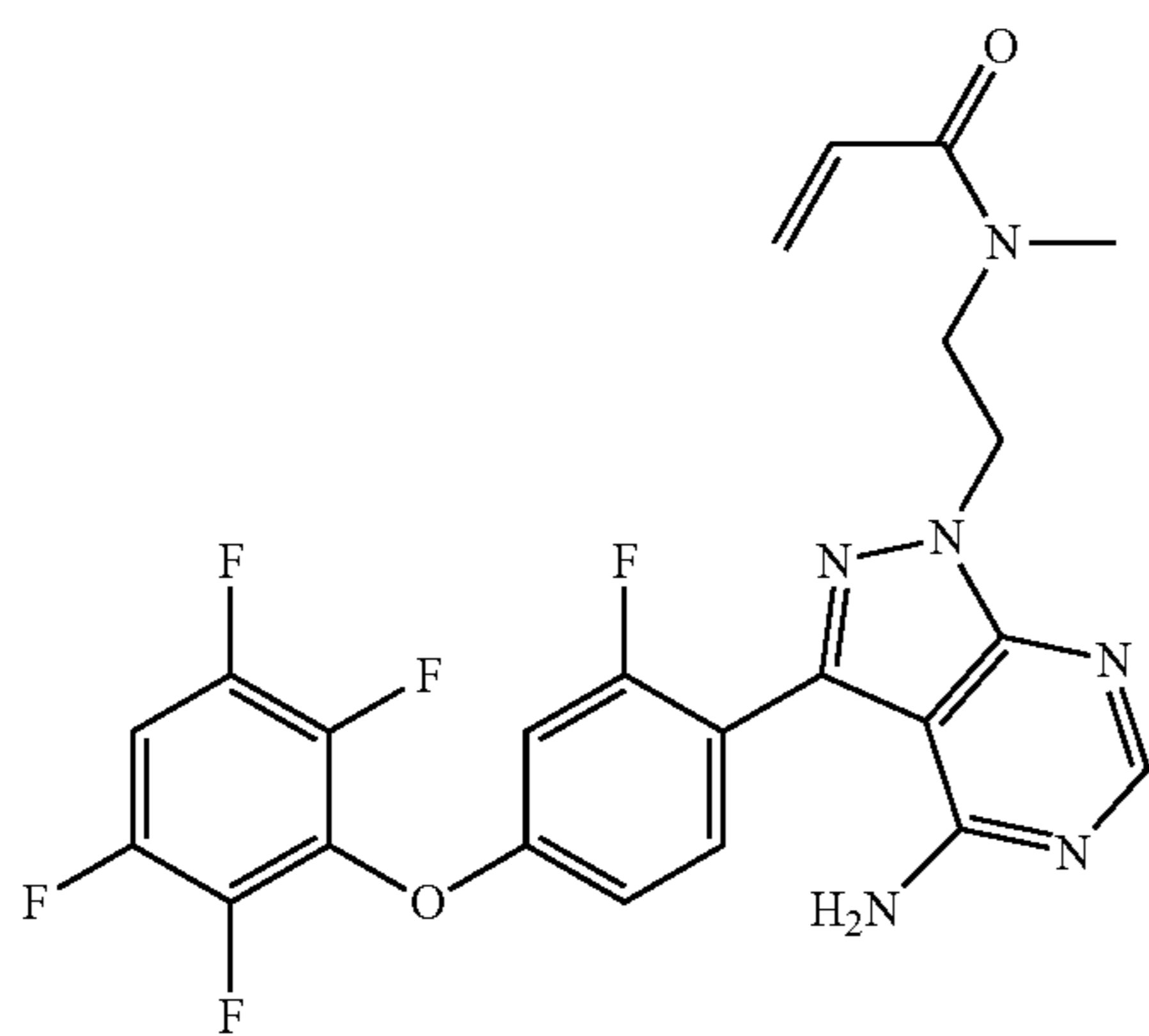
N-(2-(4-amino-3-(2-fluoro-4-(2,3,5,6-tetrafluorophenoxy)phenyl)-1H-pyrazolo[3,4-d]pyrimidin-1-yl)ethyl)-N-methylacrylamide
