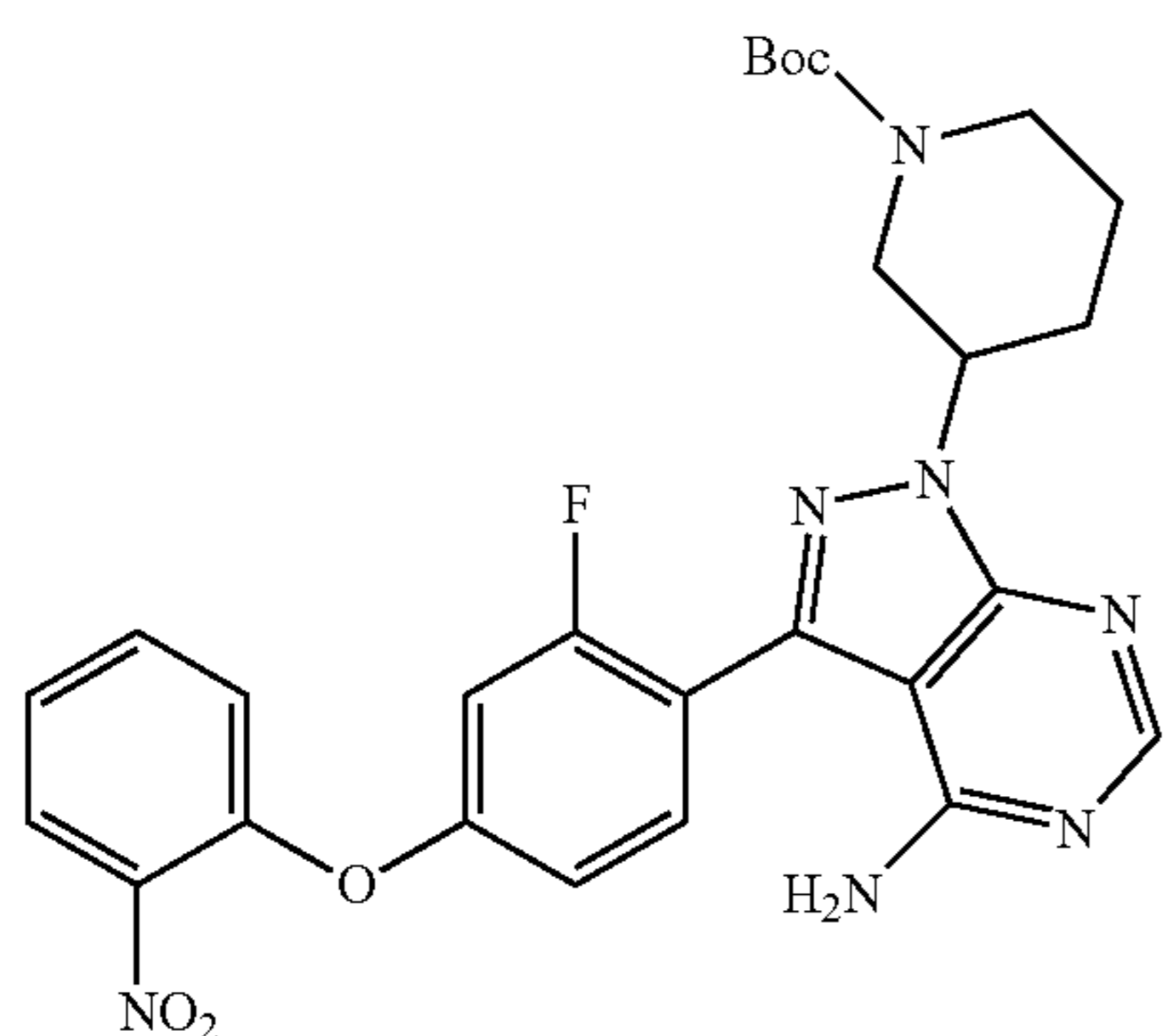
tert-butyl 3-(4-amino-3-(2-fluoro-4-(2-nitrophenoxy)phenyl)-1H-pyrazolo[3,4-d]pyrimidin-1-yl)piperidine-1-carboxylate
