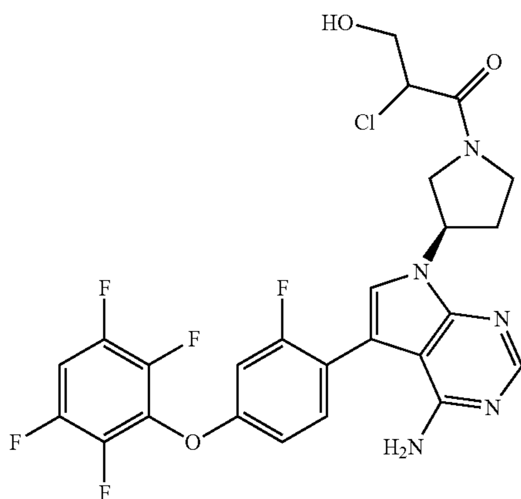
1-((R)-3-(4-amino-3-(2-fluoro-4-(2,3,5,6-tetrafluorophenoxy)phenyl)-1H-pyrrolo[2,3-d]pyrimidin-1-yl)pyrrolidin-1-yl)-2-chloro-3-hydroxypropan-1-one
