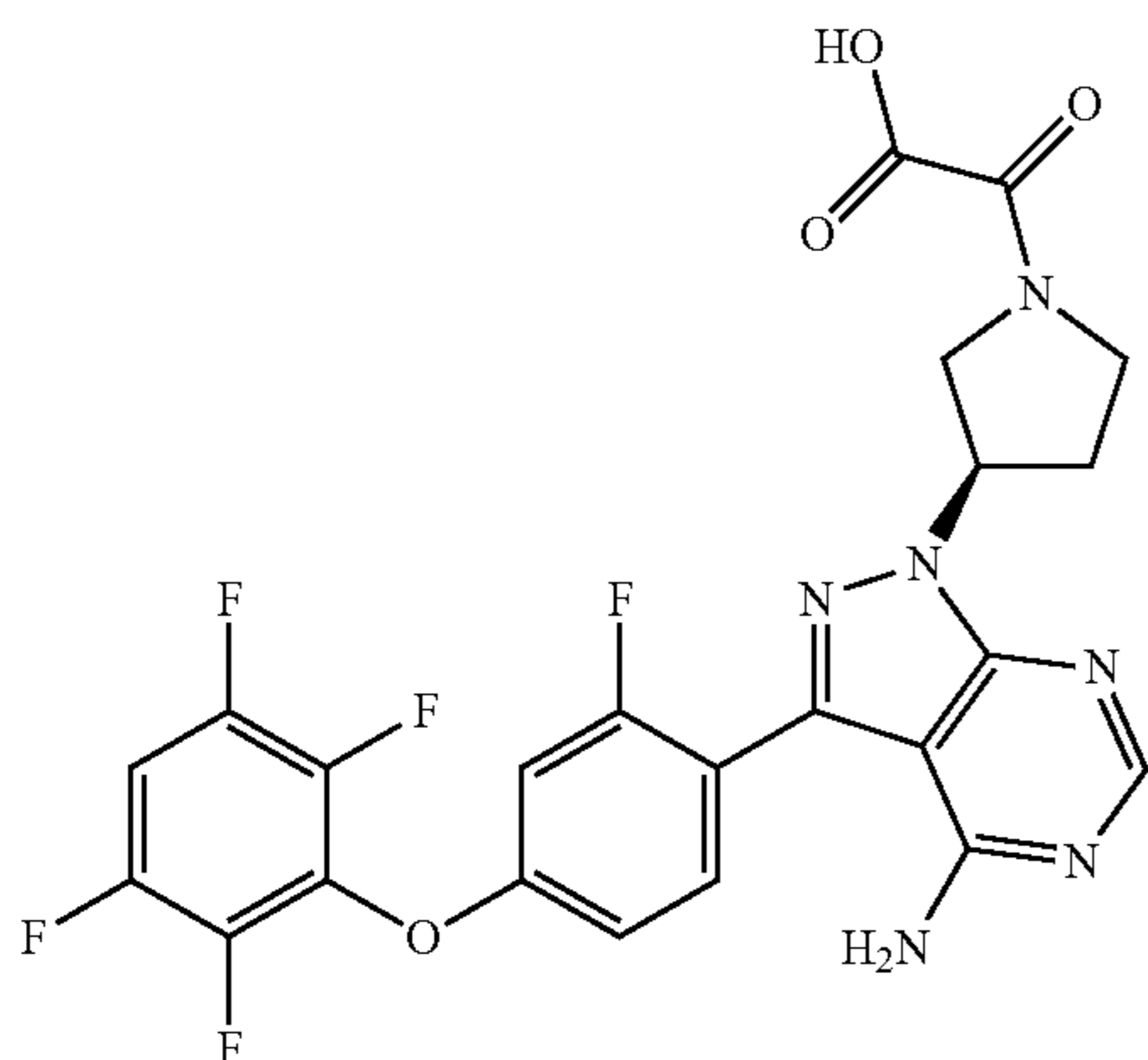
2-((R)-3-(4-amino-3-(2-fluoro-4-(2,3,5,6-tetrafluorophenoxy)phenyl)-1H-pyrazolo[3,4-d]pyrimidin-1-yl)pyrrolidin-1-yl)-2-oxoacetic Acid
