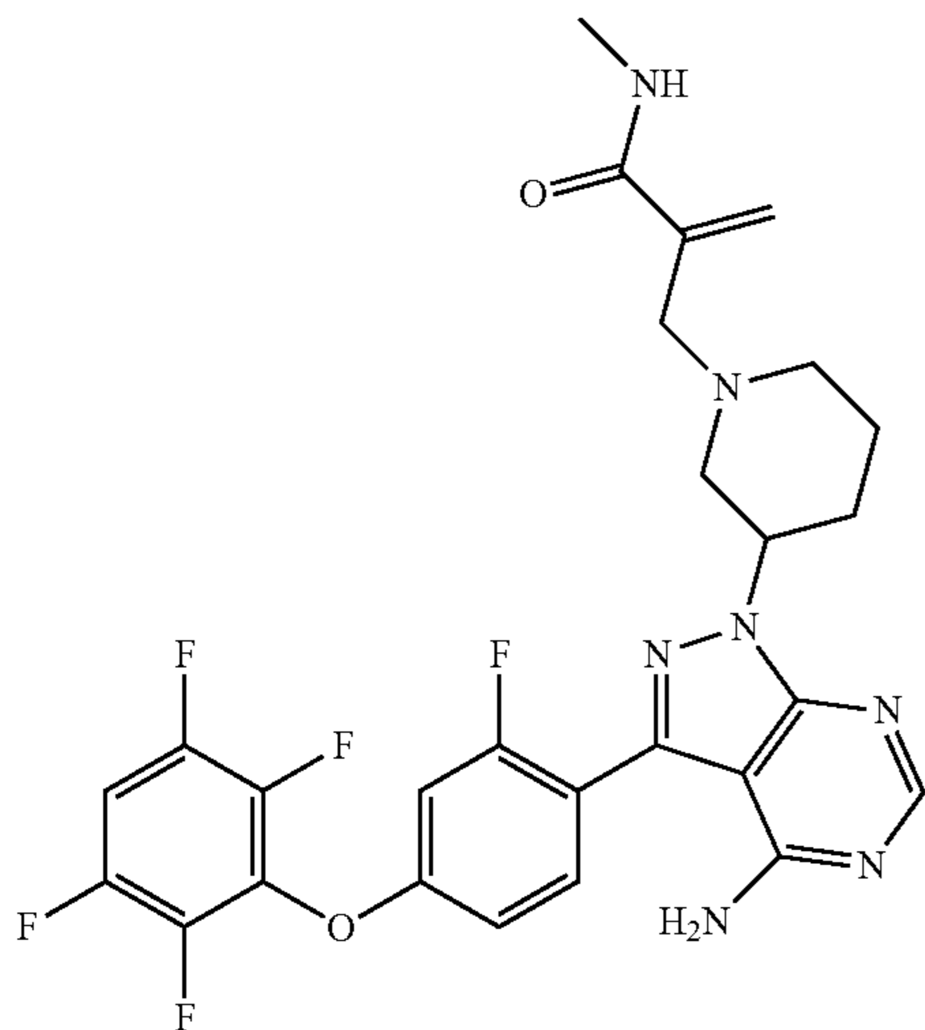
2-((3-(4-amino-3-(2-fluoro-4-(2,3,5,6-tetrafluorophenoxy)phenyl)-1H-pyrazolo[3,4-d]pyrimidin-1-yl)piperidin-1-yl)methyl)-N-methylacrylamide
