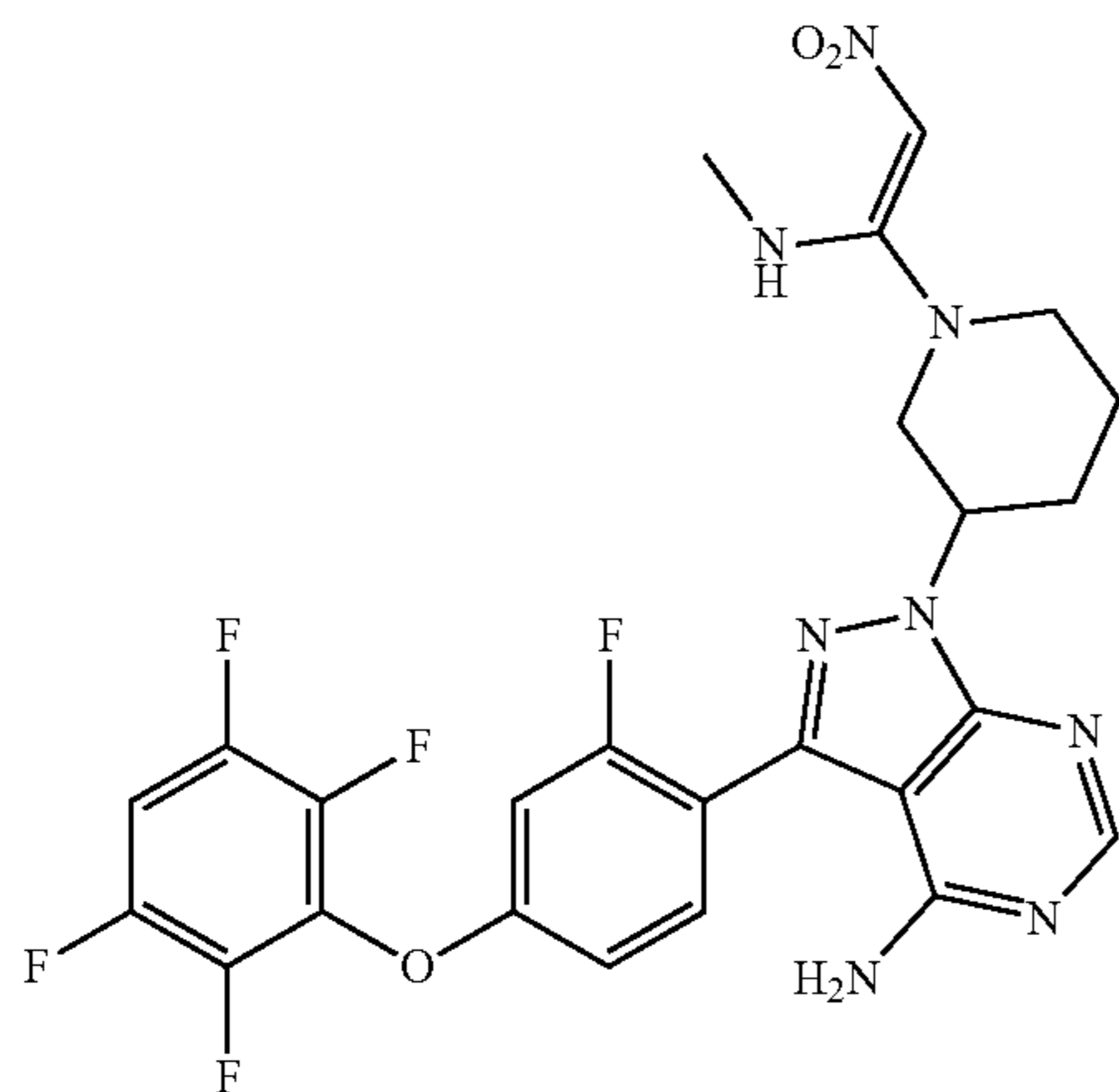
1-[3-[4-amino-3-[2-fluoro-4-(2,3,5,6-trifluorophenoxy)phenyl]-1H-pyrazolo[3,4-d]pyrimidin-1-yl]-1-piperidinyl]-1-(methylamino)-2-nitro ethylene
