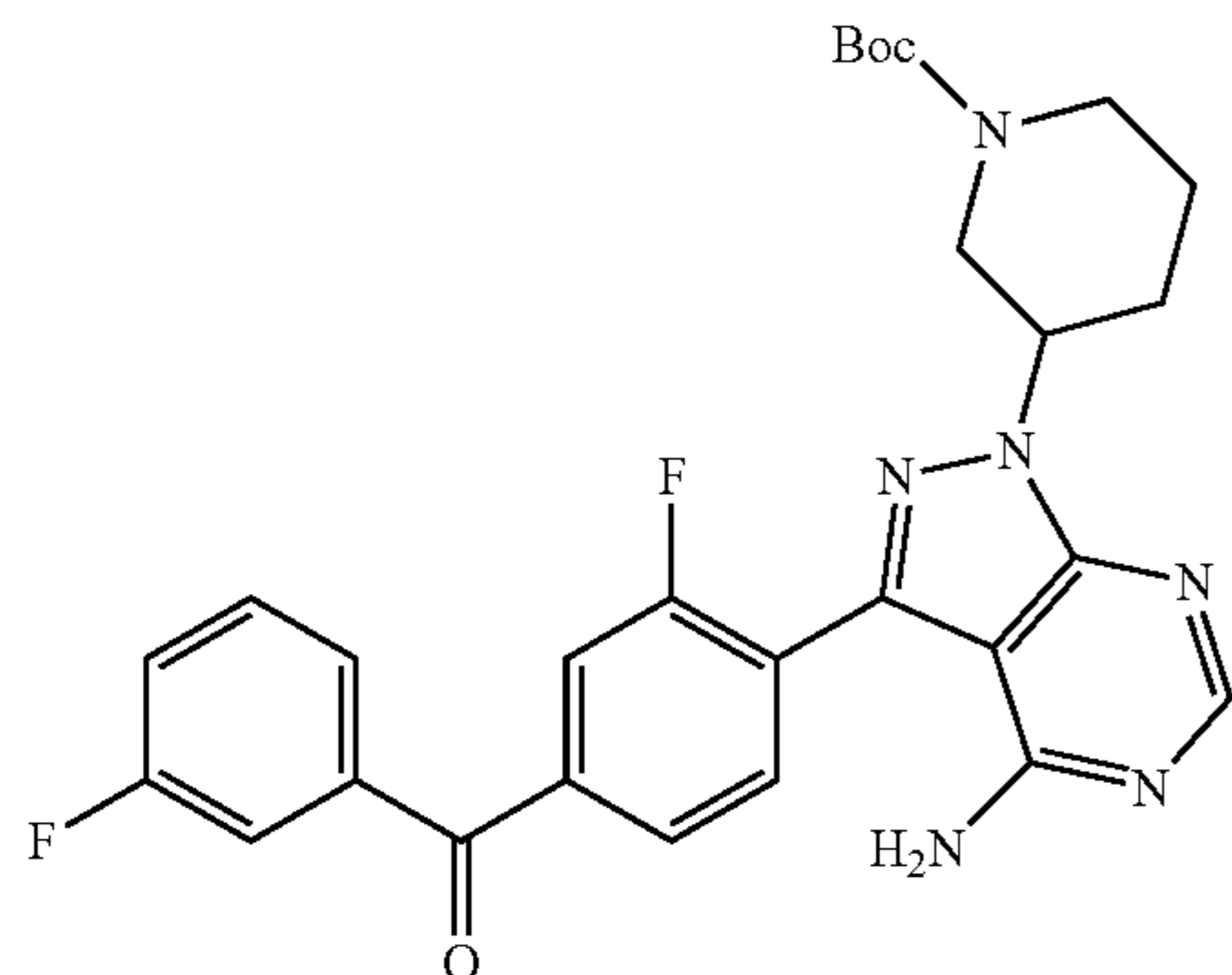
tert-butyl 3-(4-amino-3-(2-fluoro-4-(3-fluorobenzoyl)phenyl)-1H-pyrazolo[3,4-d]pyrimidin-1-yl)piperidine-1-carboxylate
