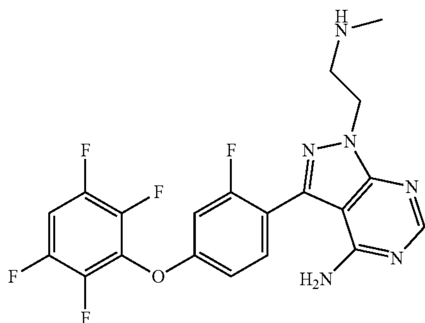
3-(2-fluoro-4-(2,3,5,6-tetrafluorophenoxy)phenyl)-1-(2-(methylamino)ethyl)-1H-pyrazolo[3,4-d]pyrimidin-4-amine
