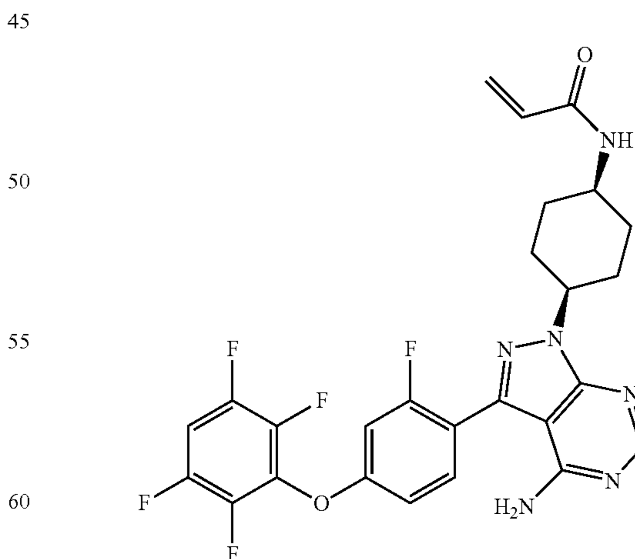
N-((1s,4s)-4-(4-amino-3-(2-fluoro-4-(2,3,5,6-tetrafluorophenoxy)phenyl)-1H-pyrazolo[3,4-d]pyrimidin-1-yl)cyclohexyl)acrylamide
