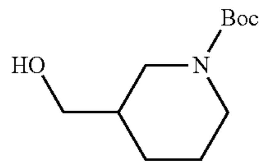
tert-butyl 3-(hydroxymethyl)piperidine-1-carboxylate
