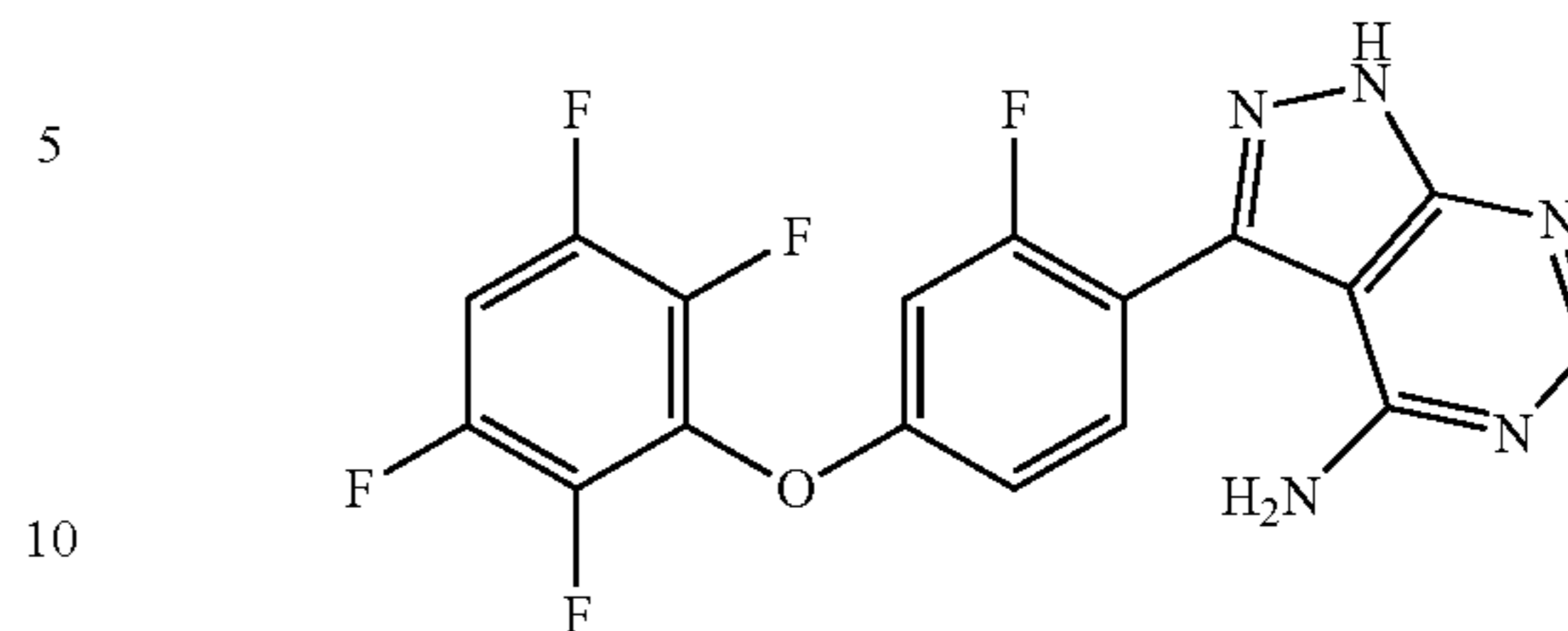
3-(2-fluoro-4-(2,3,5,6-tetrafluorophenoxy)phenyl)-1H-pyrazolo[3,4-d]pyrimidin-4-amine
