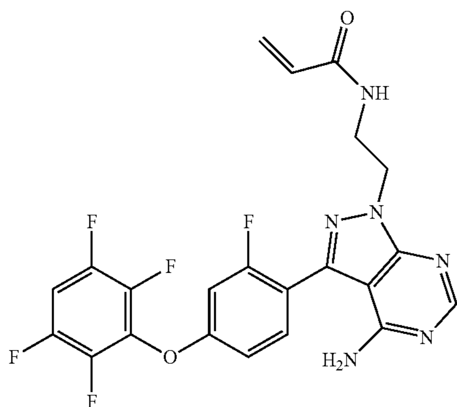
N-(2-(4-amino-3-(2-fluoro-4-(2,3,5,6-tetrafluorophenoxy)phenyl)-1H-pyrazolo[3,4-d]pyrimidin-1-yl)ethyl)acrylamide
