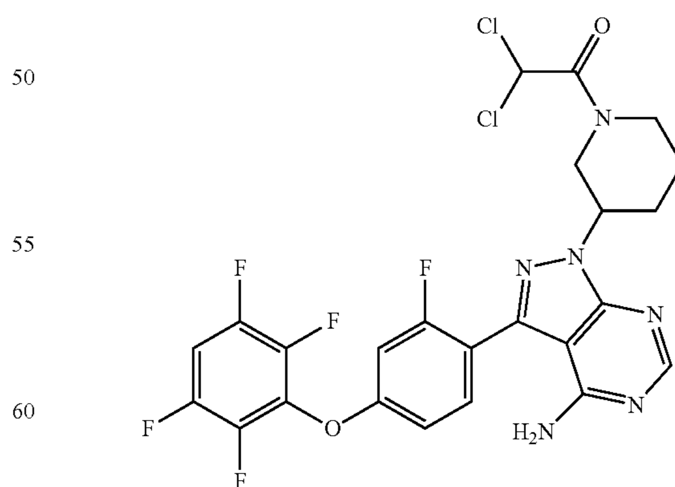
1-(3-(4-amino-3-(2-fluoro-4-(2,3,5,6-tetrafluorophenoxy)phenyl)-1H-pyrazolo[3,4-d]pyrimidin-1-yl)piperidin-1-yl)-2,2-dichloroethanone
