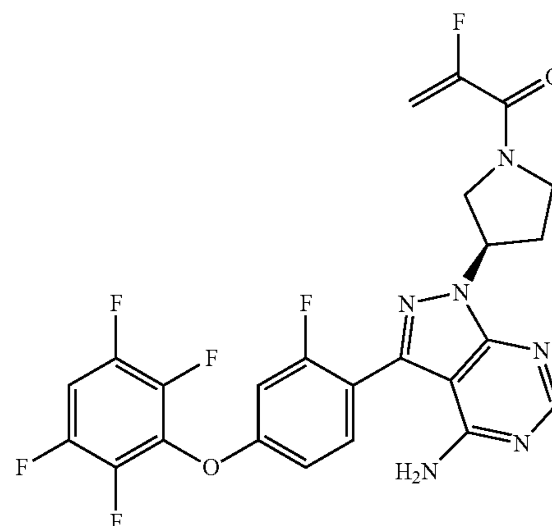
1-((R)-3-(4-amino-3-(2-fluoro-4-(2,3,5,6-tetrafluorophenoxy)phenyl)-1H-pyrazolo[3,4-d]pyrimidin-1-yl)pyrrolidin-1-yl)-2-fluoroprop-2-en-1-one
