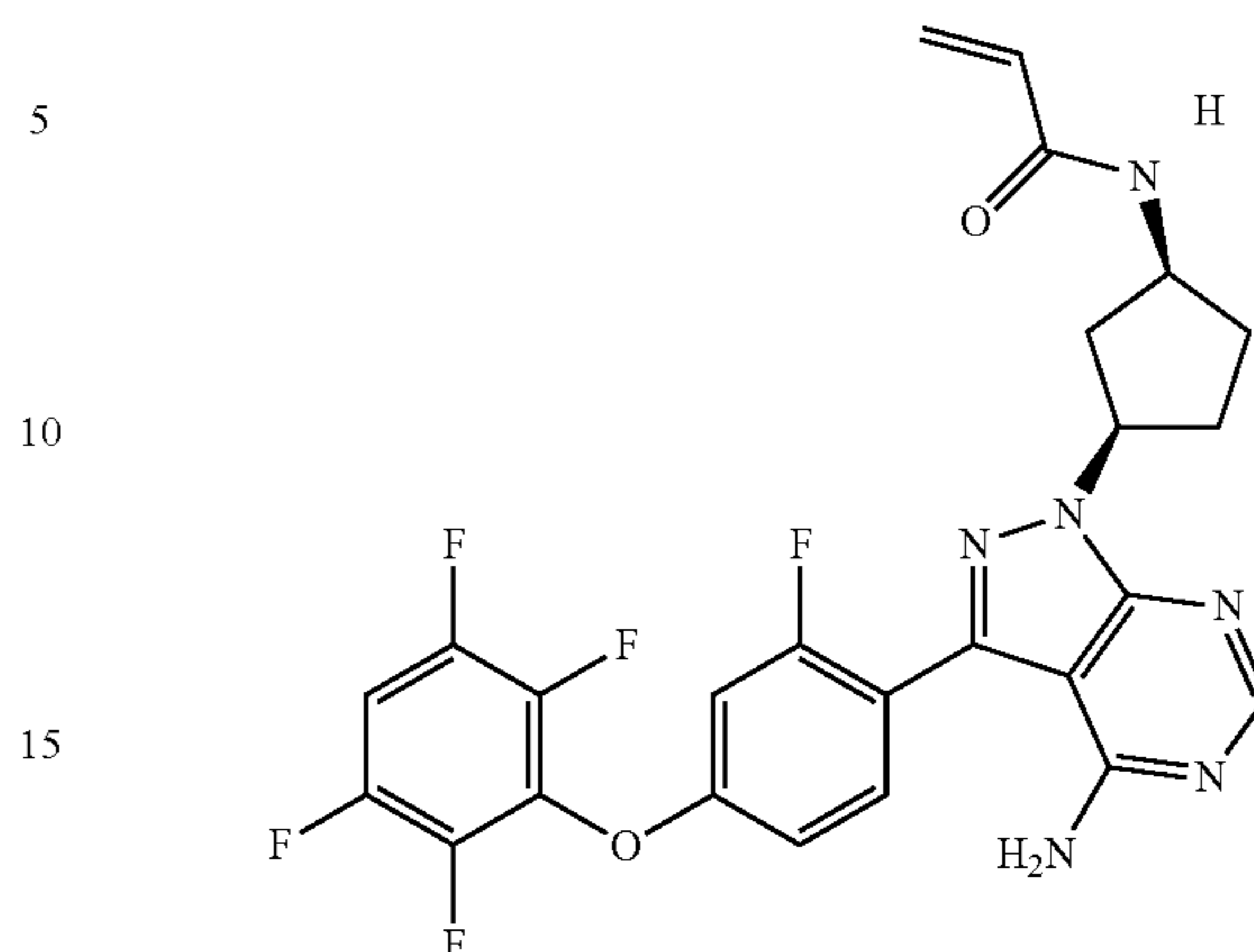
N-((1s,3r)-3-(4-amino-3-(2-fluoro-4-(2,3,5,6-tetrafluorophenoxy)phenyl)-1H-pyrazolo[3,4-d]pyrimidin-1-yl)cyclopentyl)acrylamide
