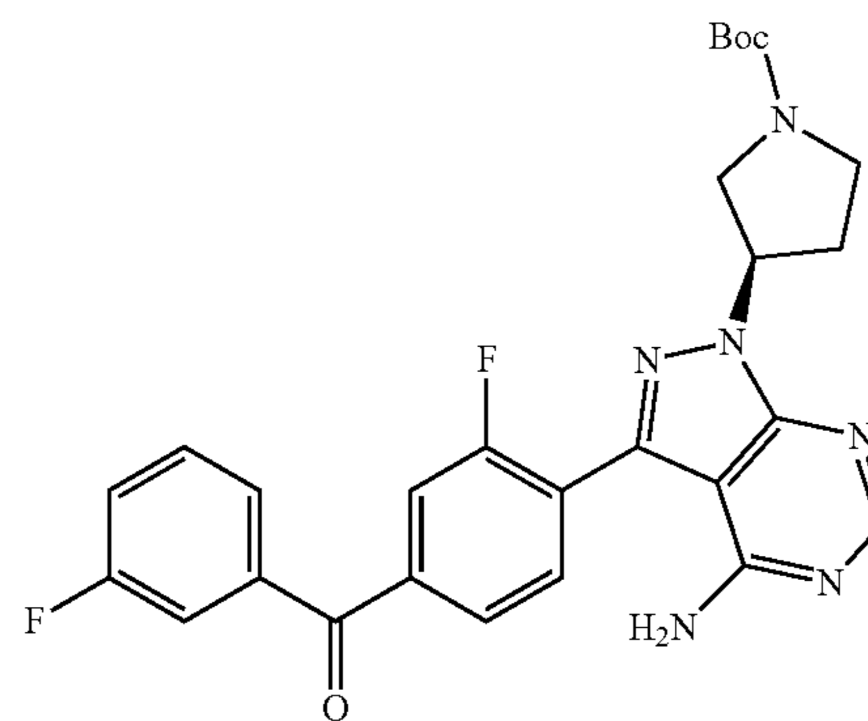
(3R)-tert-butyl 3-(4-amino-3-(2-fluoro-4-(3-fluorobenzoyl)phenyl)-1H-pyrazolo[3,4-d]pyrimidin-1-yl)pyrrolidine-1-carboxylate
