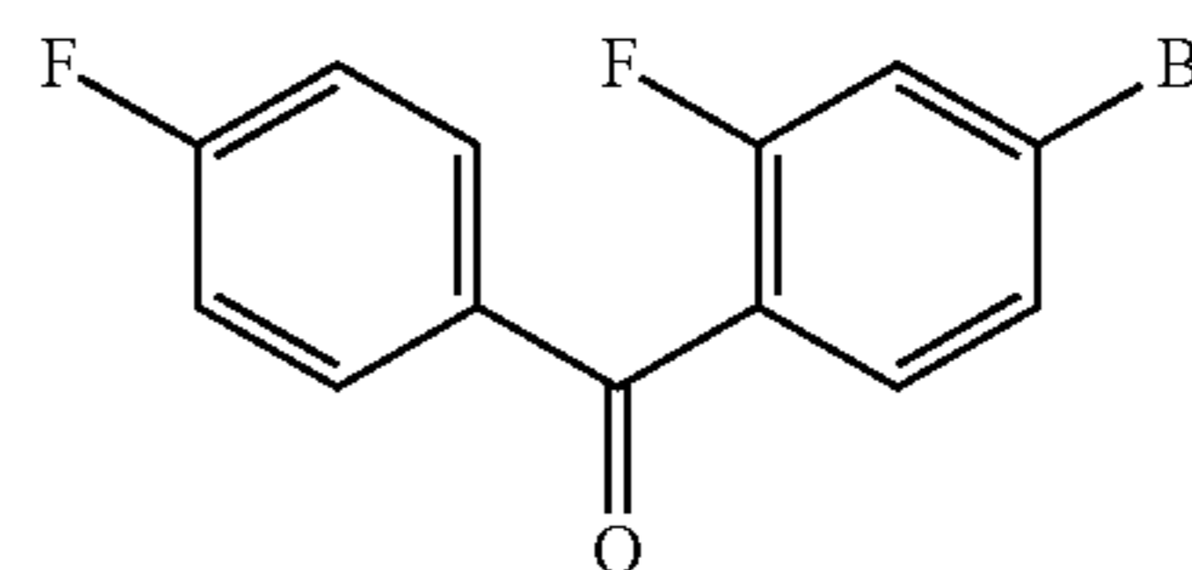
(4-bromo-2-fluorophenyl)(4-fluorophenyl)methanone
