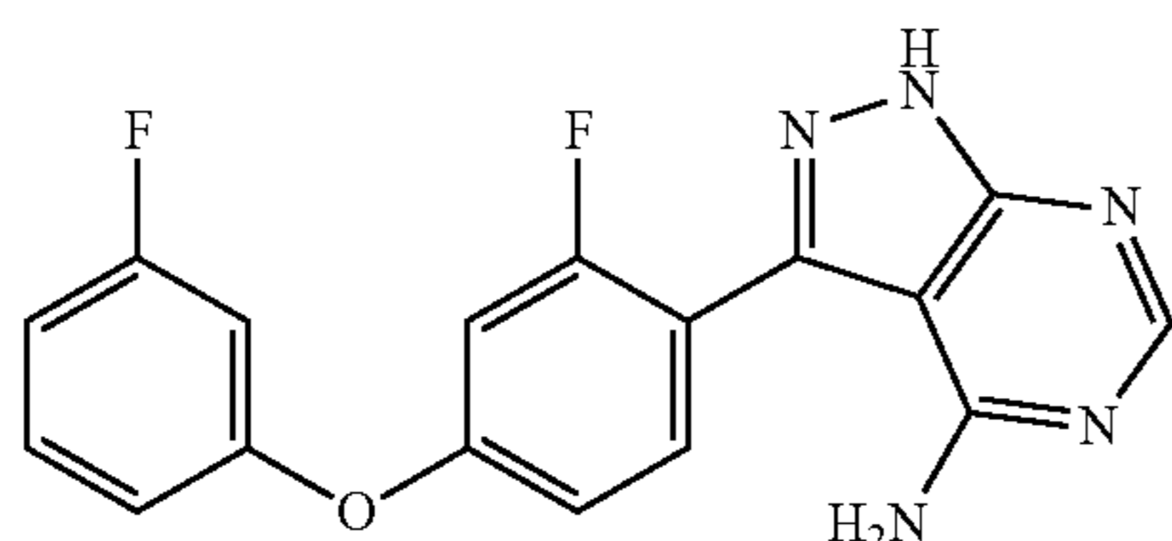
3-(2-fluoro-4-(3-fluorophenoxy)phenyl)-1H-pyrazolo[3,4-d]pyrimidin-4-amine
