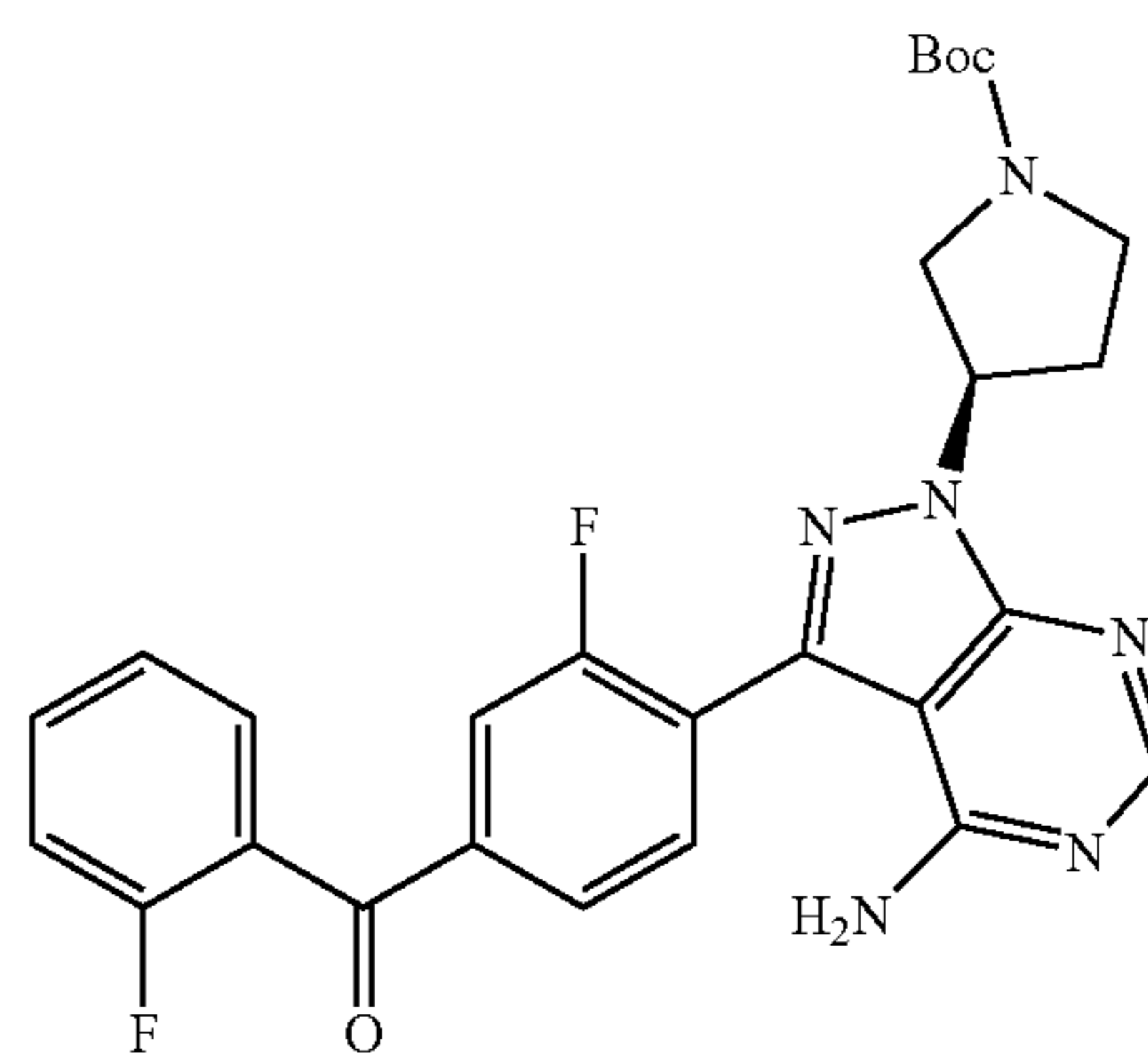
(3R)-tert-butyl 3-(4-amino-3-(2-fluoro-4-(2-fluorobenzoyl)phenyl)-1H-pyrazolo[3,4-d]pyrimidin-1-yl)pyrrolidine-1-carboxylate
