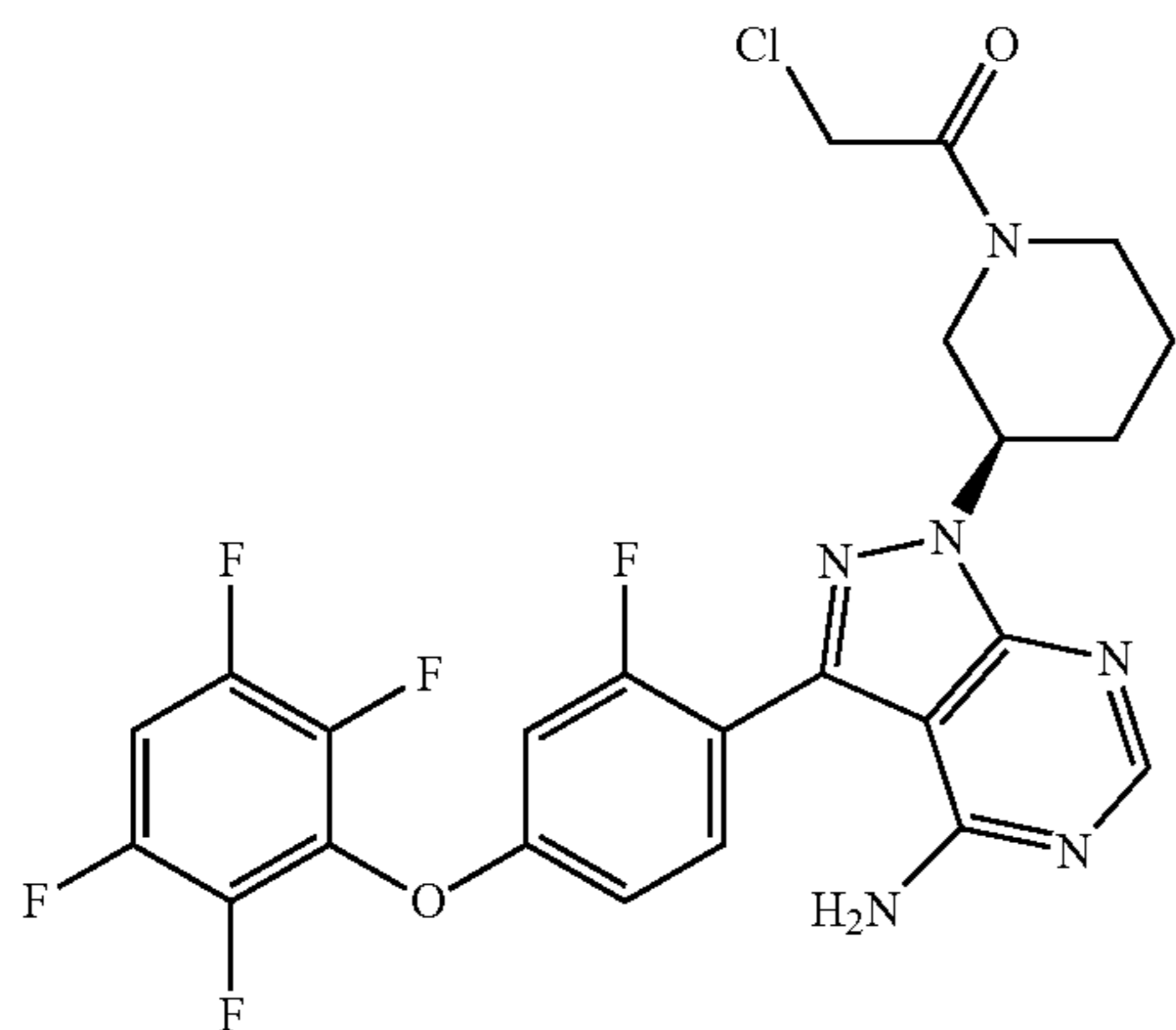
1-((R)-3-(4-amino-3-(2-fluoro-4-(2,3,5,6-tetrafluorophenoxy)phenyl)-1H-pyrazolo[3,4-d]pyrimidin-1-yl)piperidin-1-yl)-2-chloroethanone
