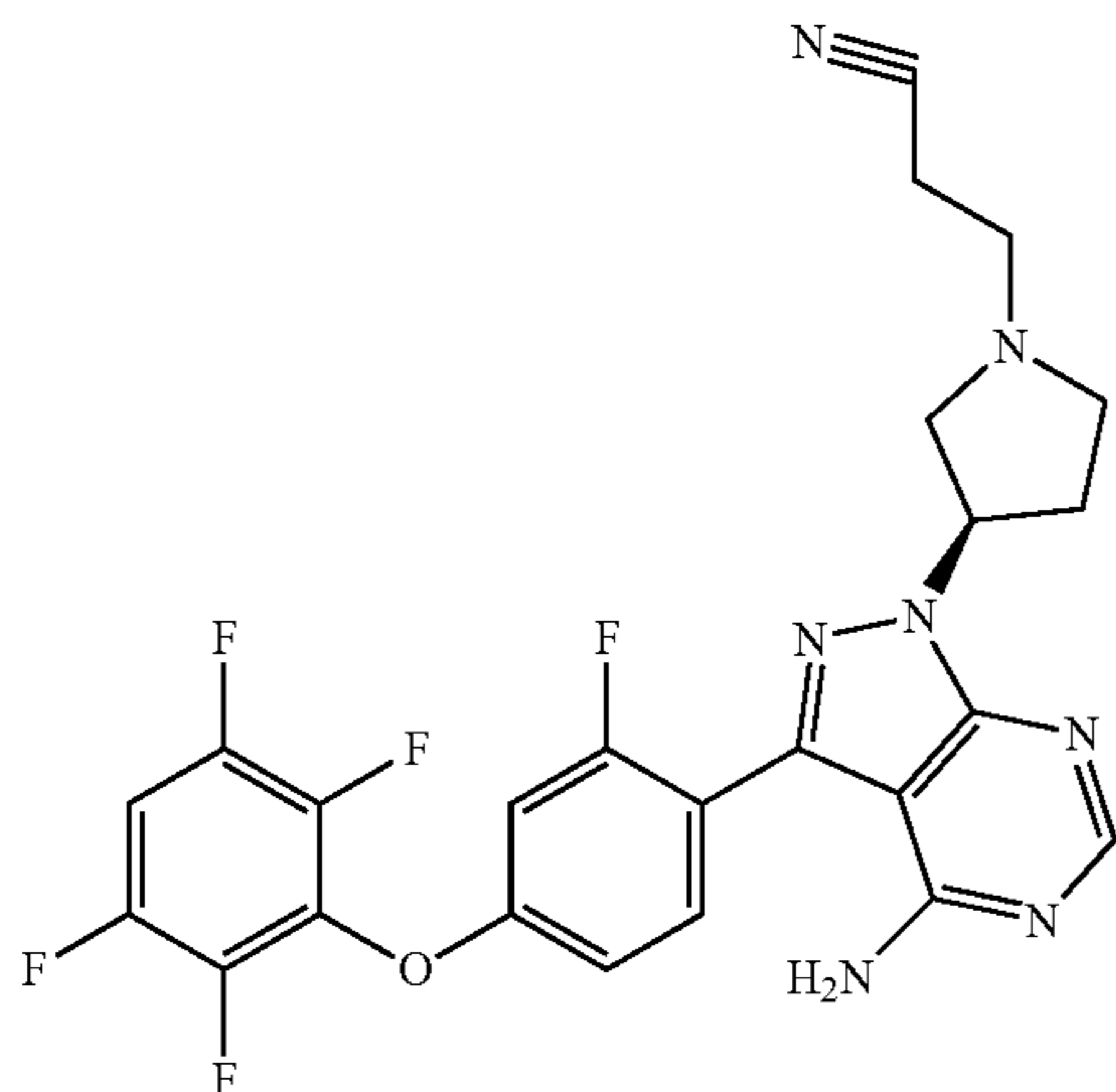
3-((R)-3-(4-amino-3-(2-fluoro-4-(2,3,5,6-tetrafluorophenoxy)phenyl)-1H-pyrazolo[3,4-d]pyrimidin-1-yl)pyrrolidin-1-yl)propanenitrile
