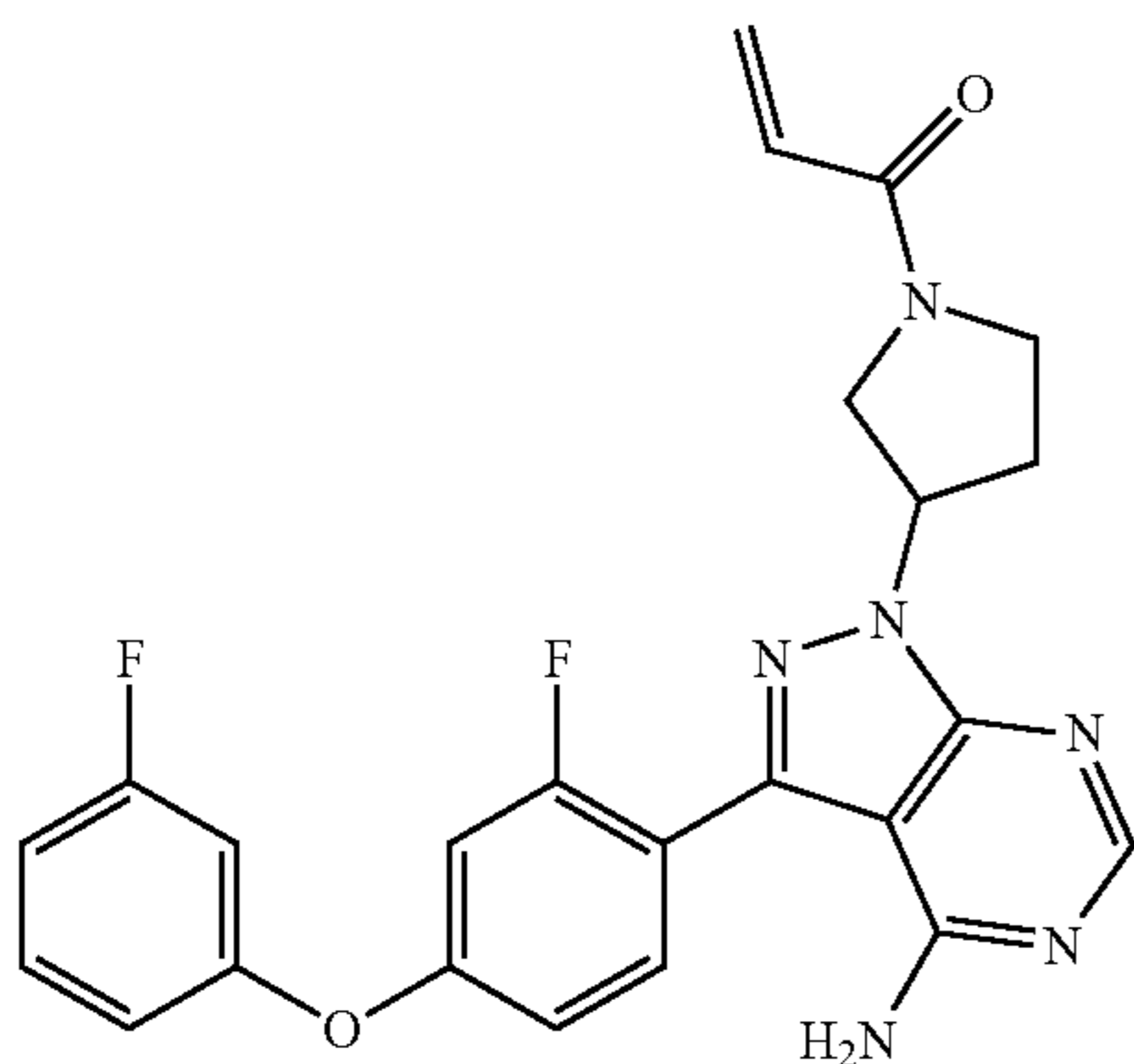
1-(3-(4-amino-3-(2-fluoro-4-(3-fluorophenoxy)phenyl)-1H-pyrazolo[3,4-d]pyrimidin-1-yl)pyrrolidin-1-yl)prop-2-en-1-one
