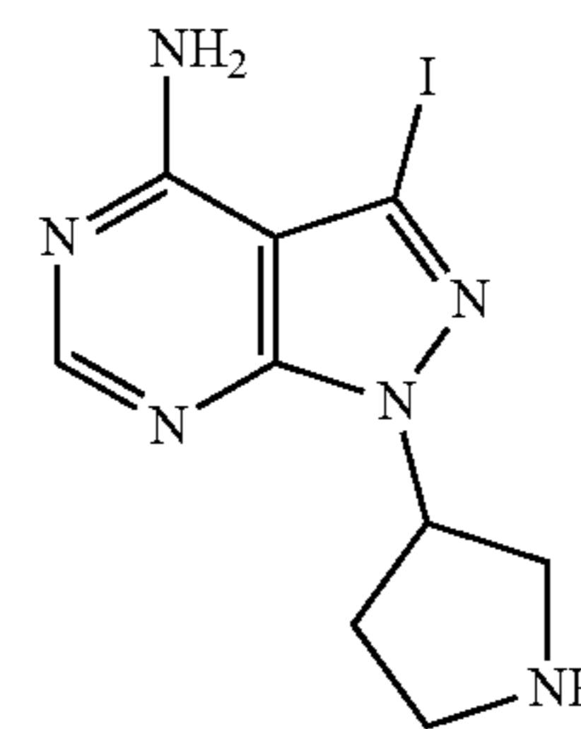
3-iodo-1-(pyrrolidin-3-yl)-1H-pyrazolo[3,4-d]pyrimidin-4-amine
