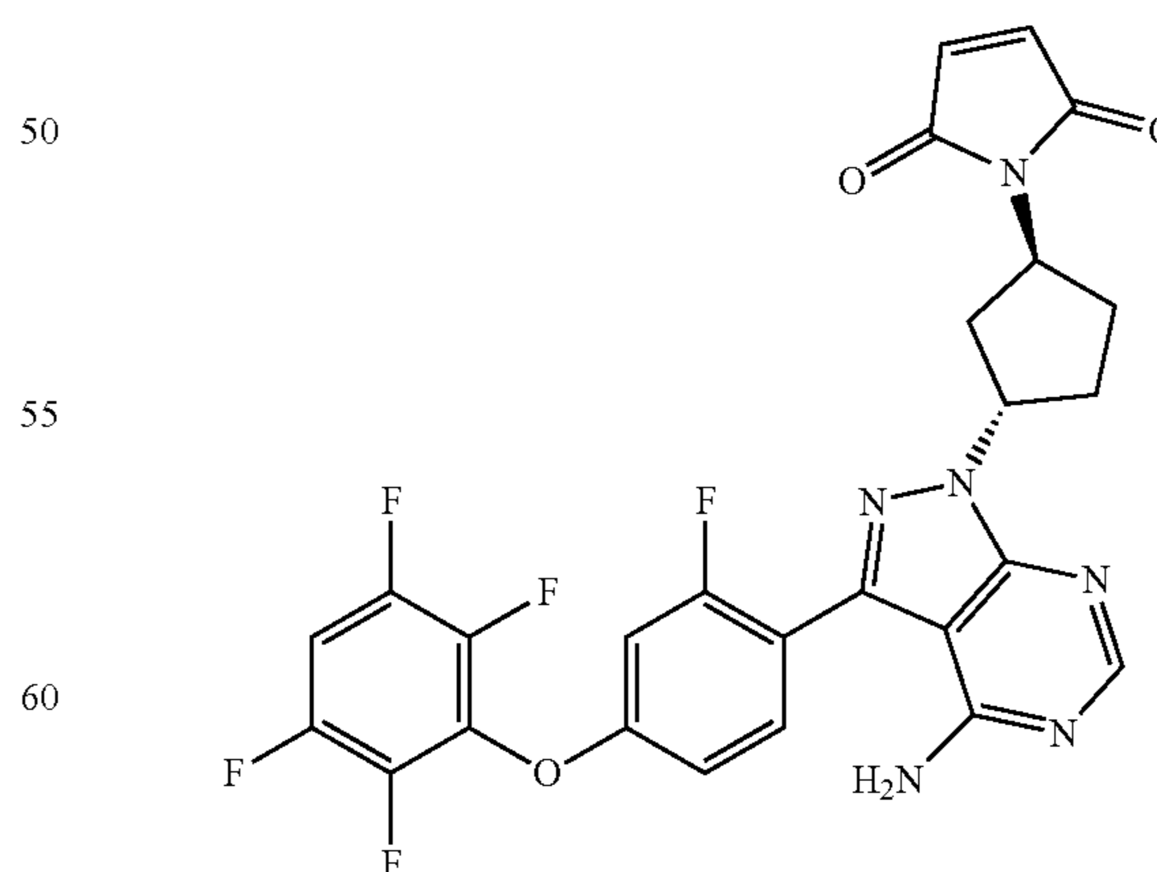
1-((1S,3S)-3-(4-amino-3-(2-fluoro-4-(2,3,5,6-tetrafluorophenoxy)phenyl)-1H-pyrazolo[3,4-d]pyrimidin-1-yl)cyclopentyl)-1H-pyrrole-2,5-dione
