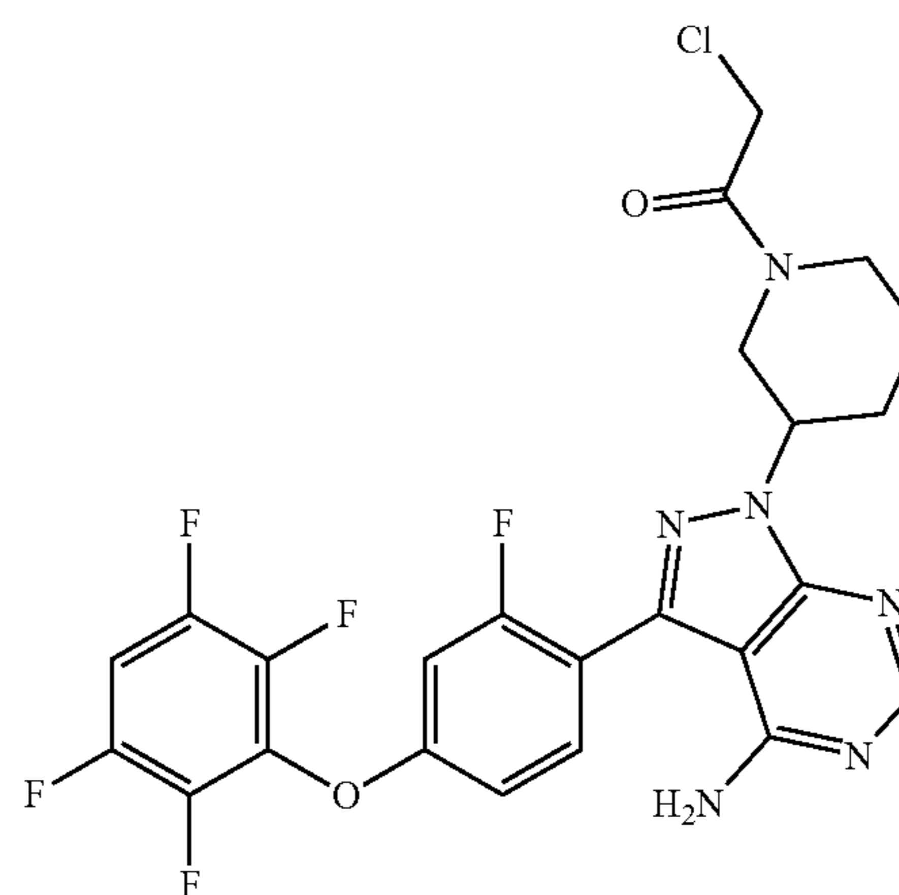
1-(3-(4-amino-3-(2-fluoro-4-(2,3,5,6-tetrafluorophenoxy)phenyl)-1H-pyrazolo[3,4-d]pyrimidin-1-yl)piperidin-1-yl)-2-chloroethanone
