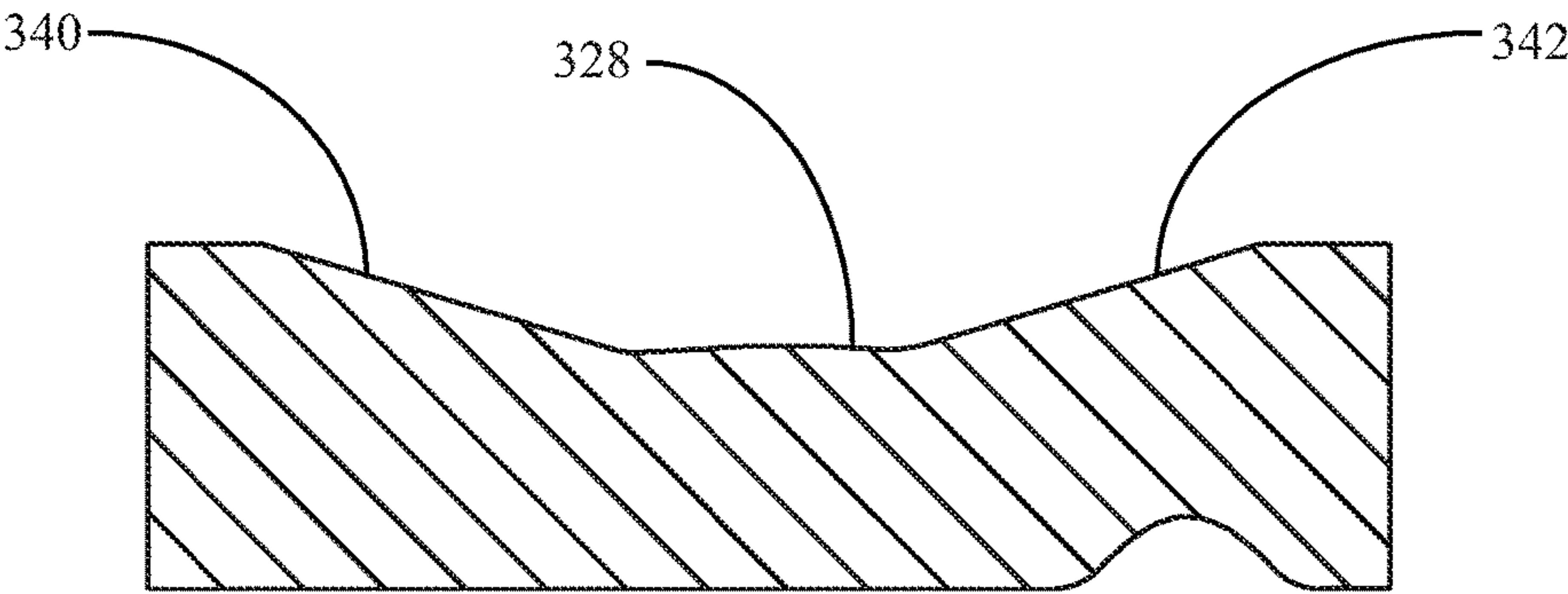
SEC. Z-Z
