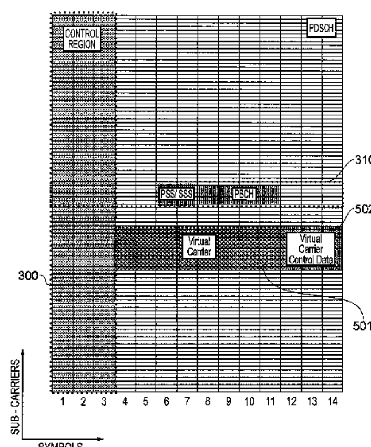
DOWNLINK SUB-FRAME WITH VIRTUAL CARRIER
