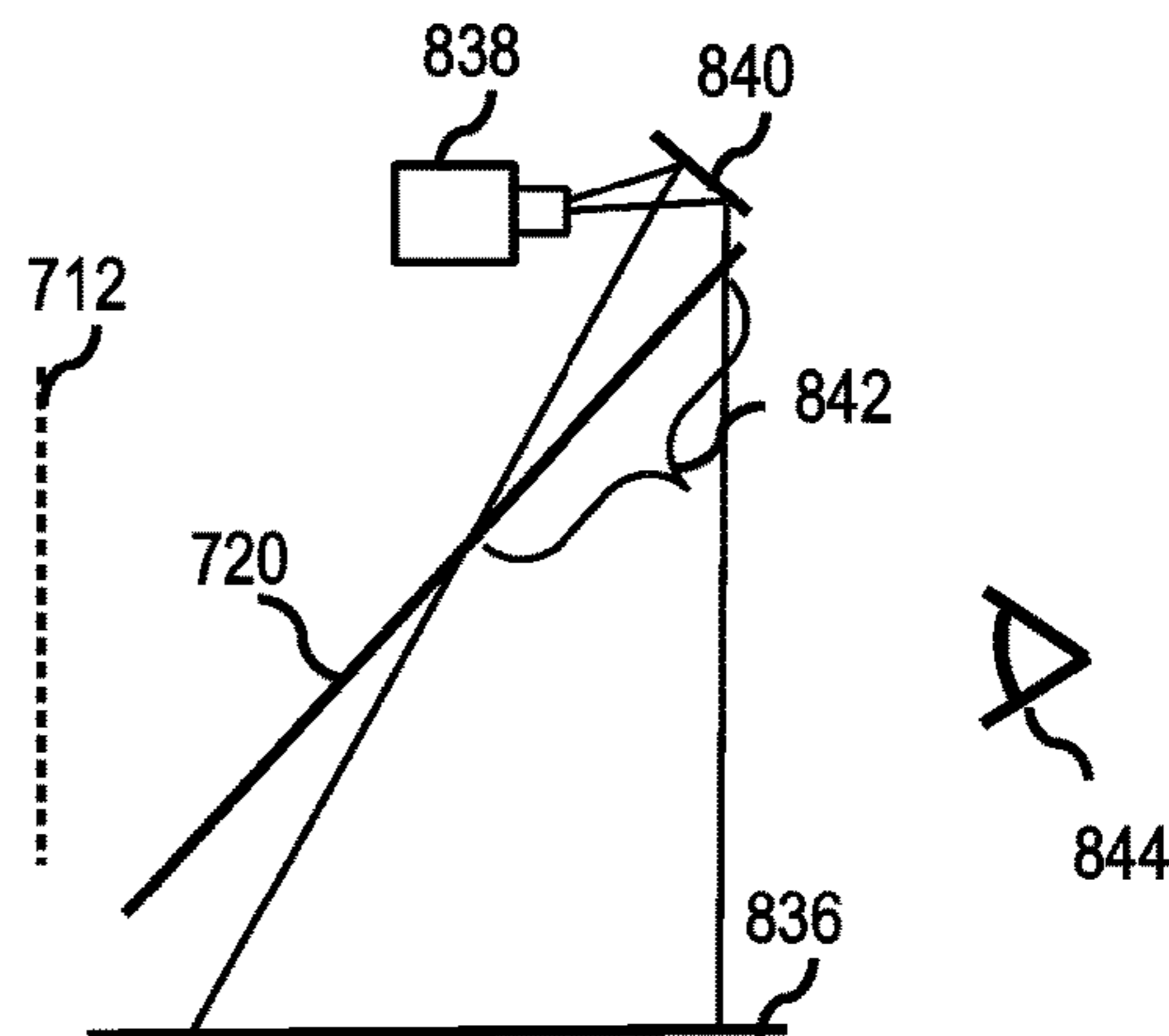
FIG. 84 PRIOR ART
