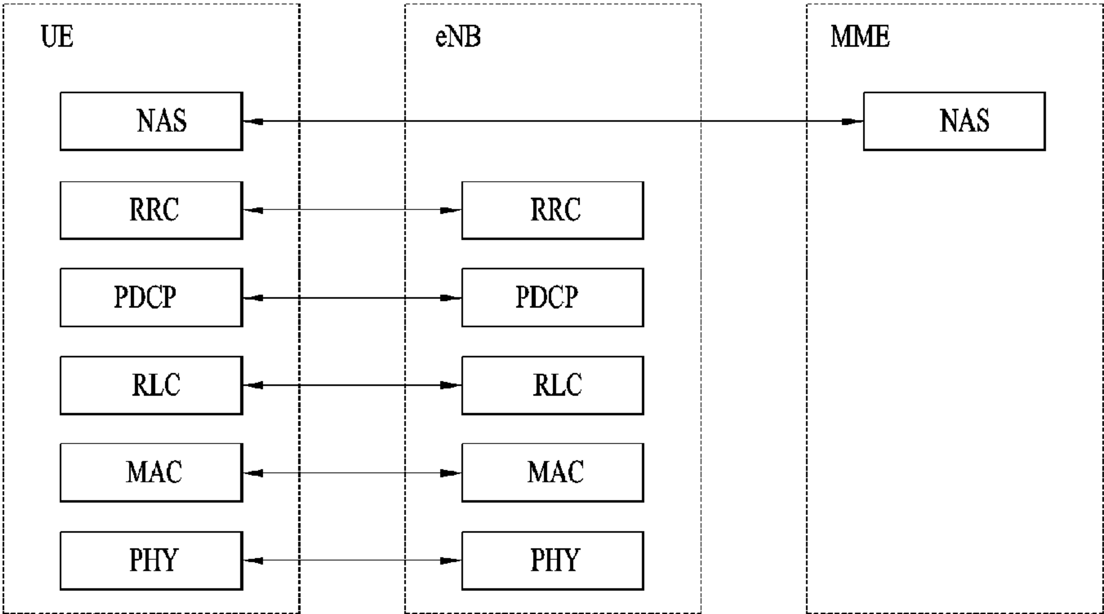
(a) Control-plane protocol stack
