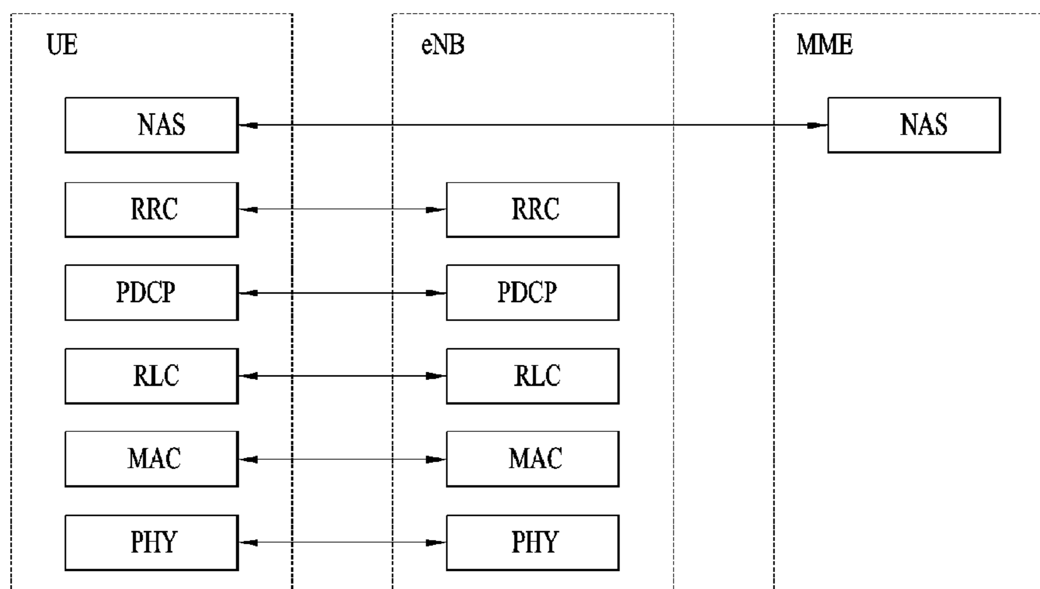
(a) Control-plane protocol stack
