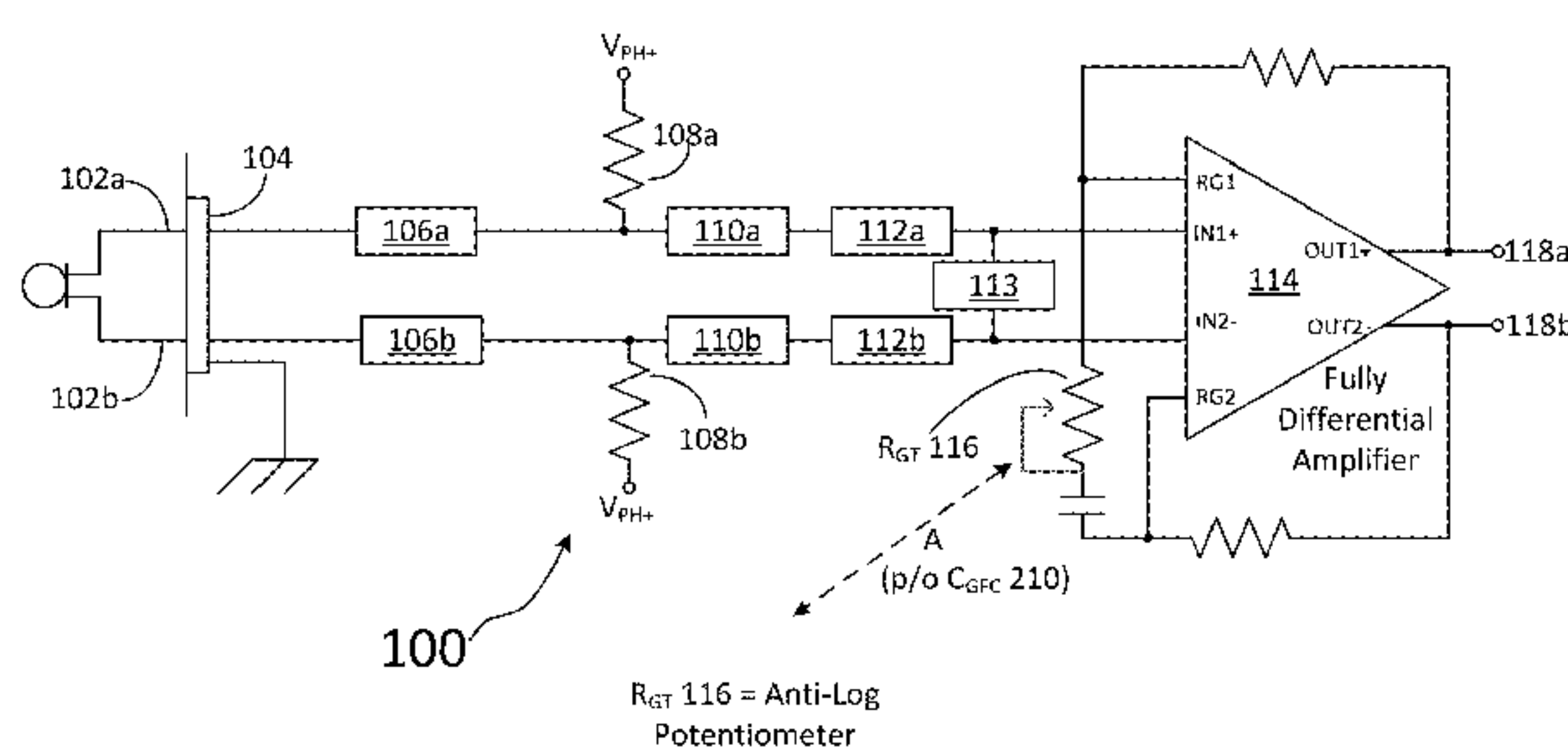
Gain Trim Circuit
