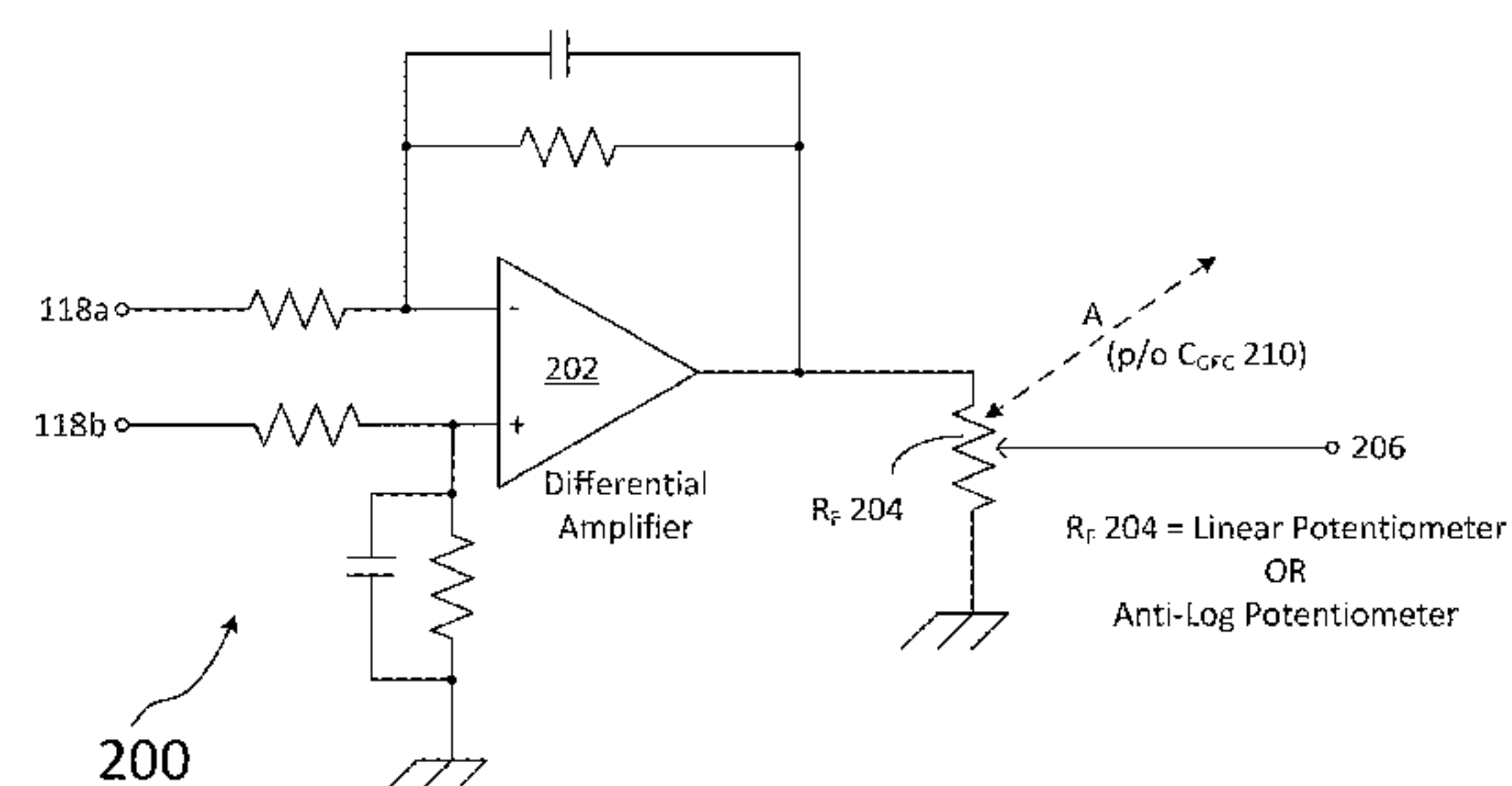
Fader Circuit
