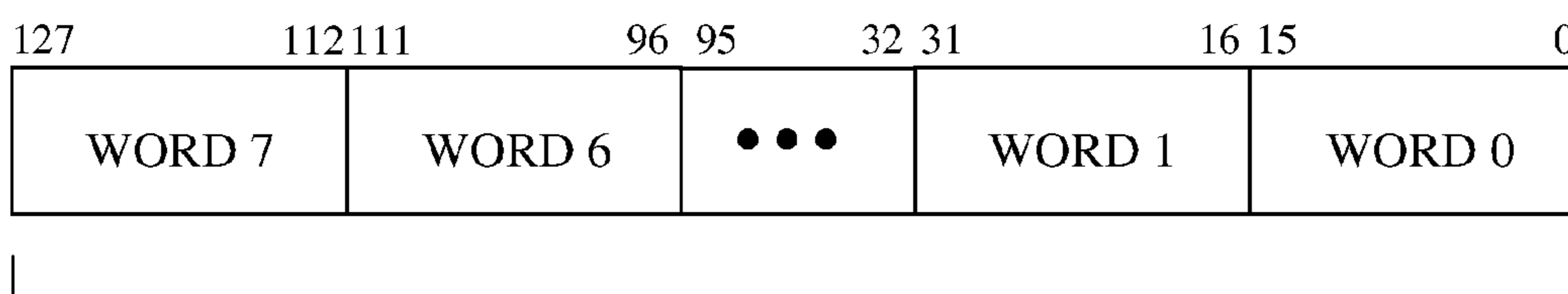
320 PACKED WORD
