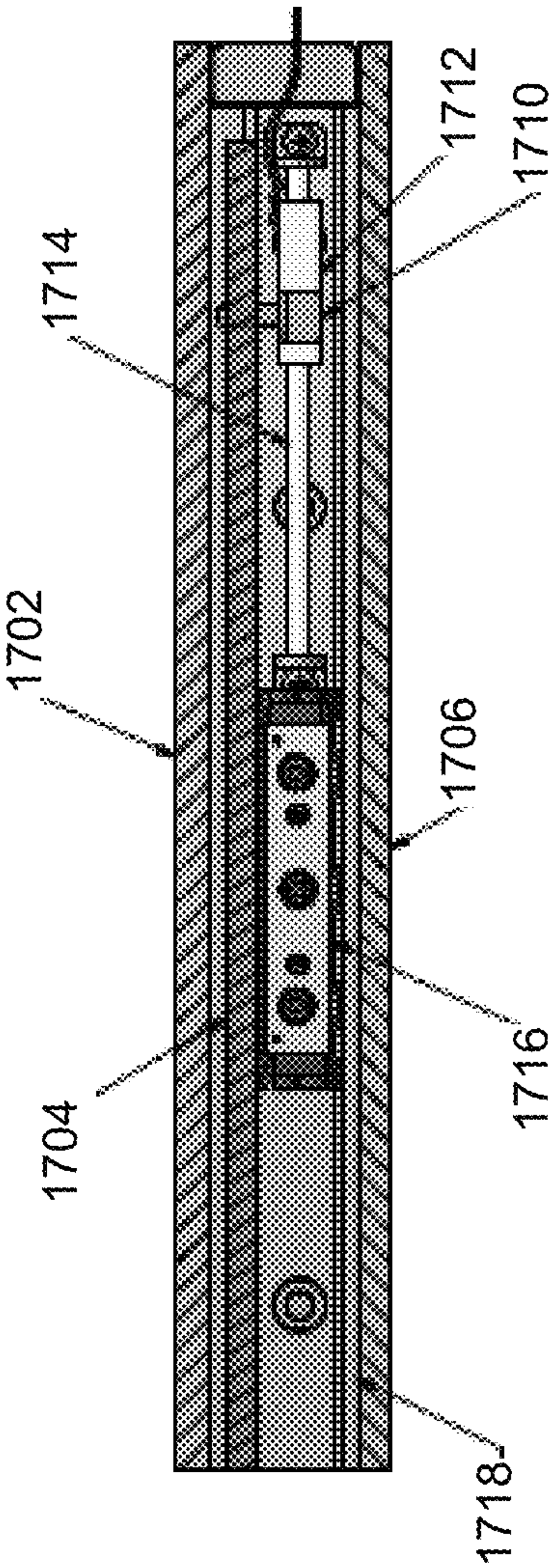
SECTION B-B
