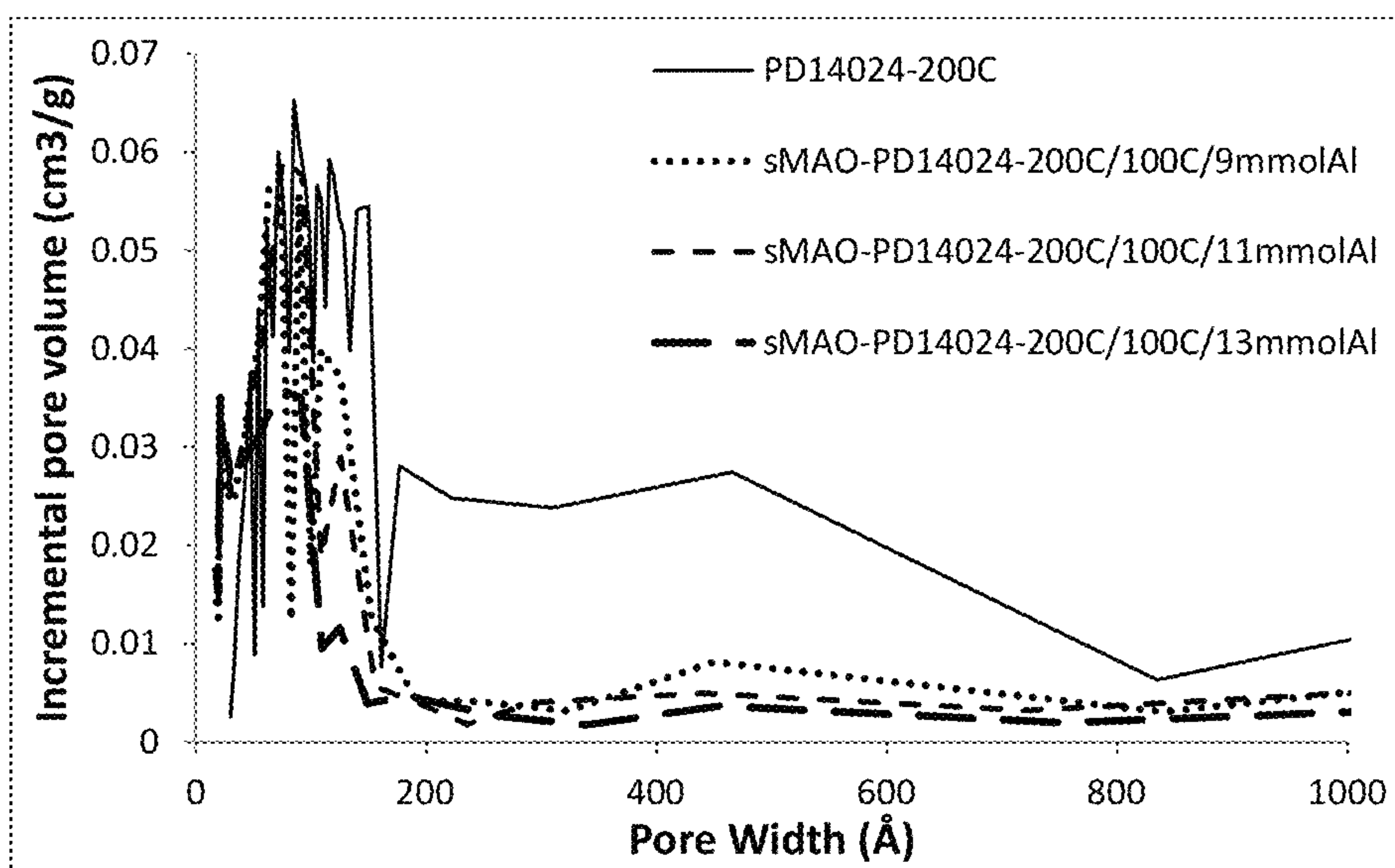
FIG. 3: Plot of Pore Diameter Distribution for PD 14024 Silica
