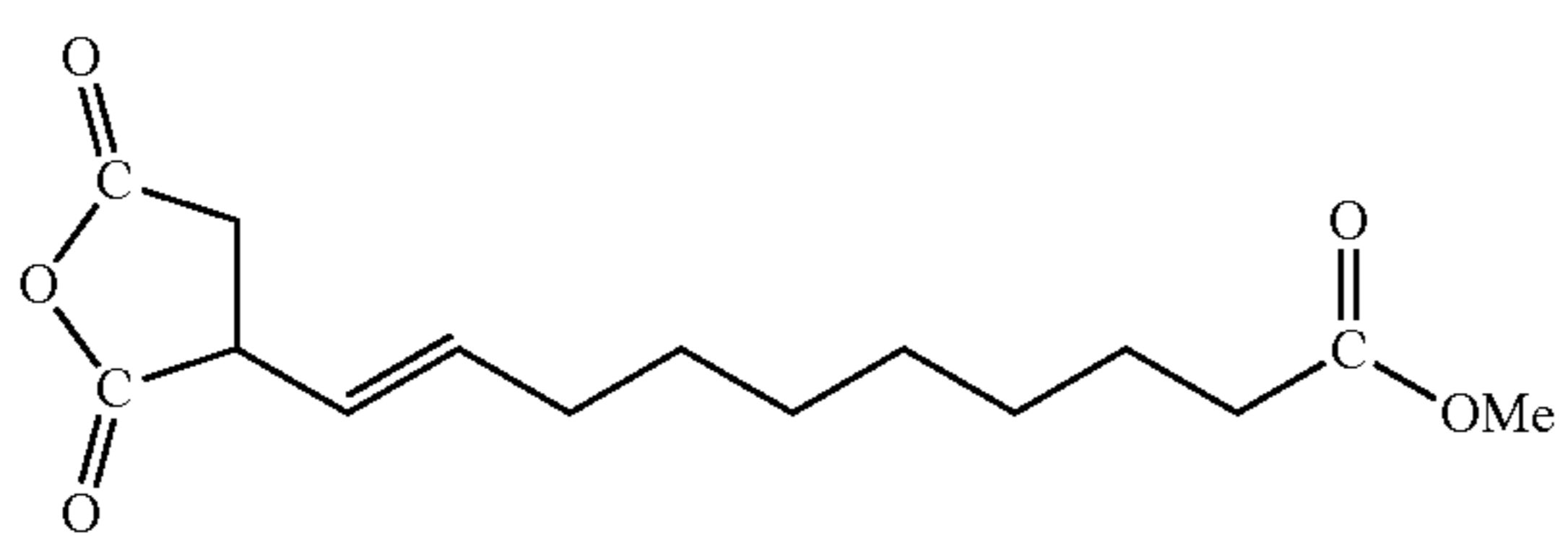
Maleinated 9-DAMe
