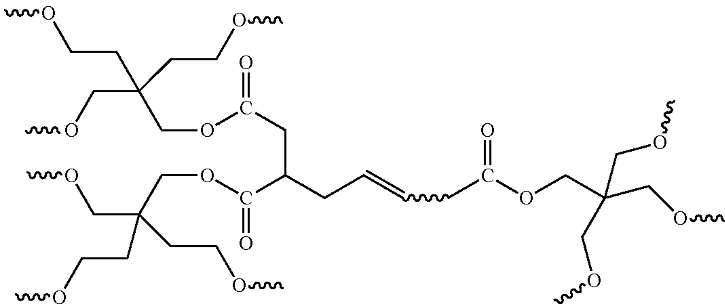
PE Product's Structural Features
