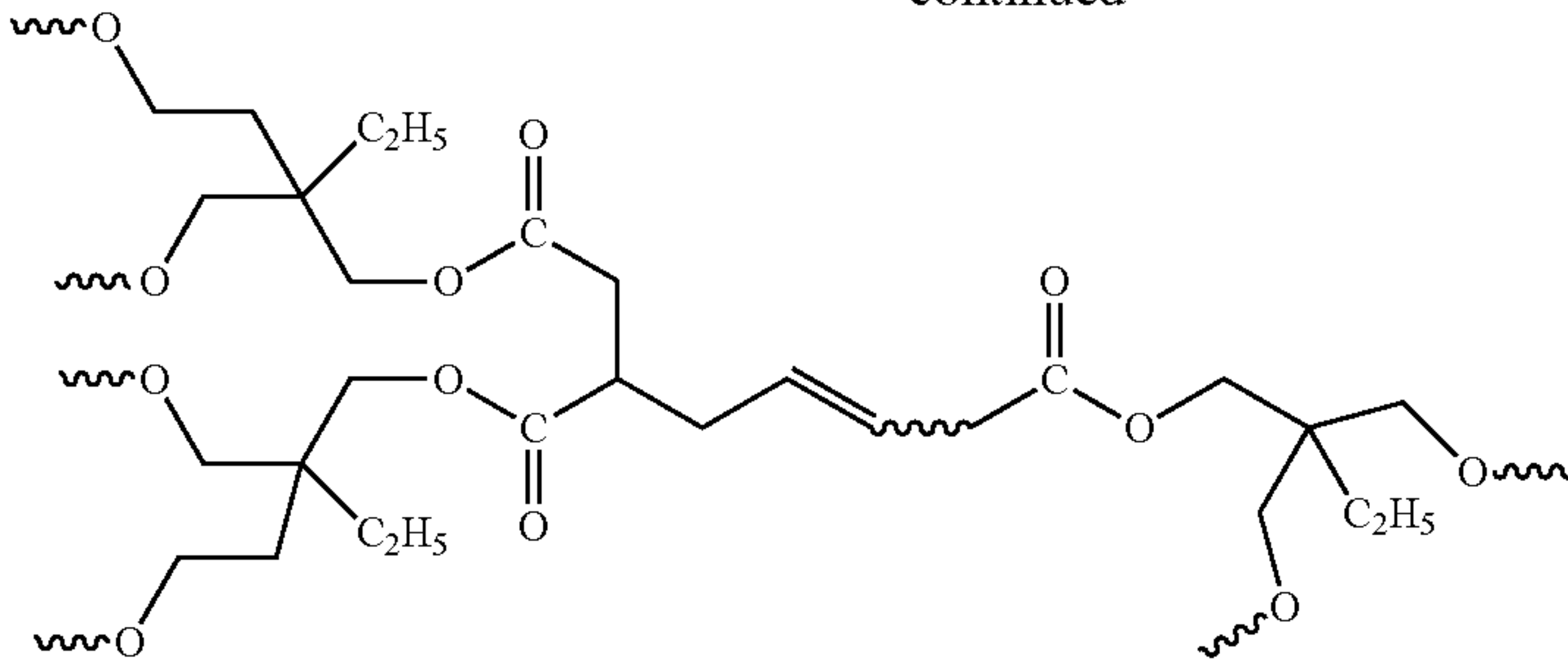
THMP Product's Structural Features
