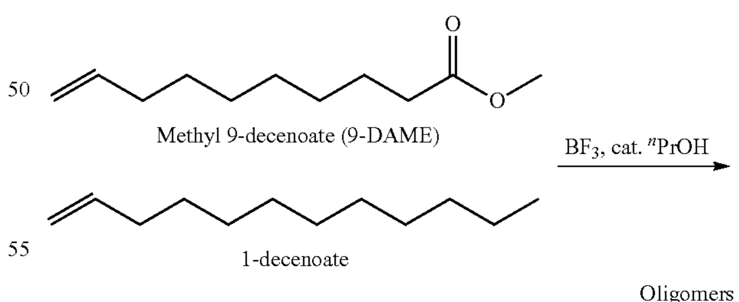
Scheme 1. BF 3 -mediated co-oligomerization of methyl 9-decenoate and 1-dodecene.
