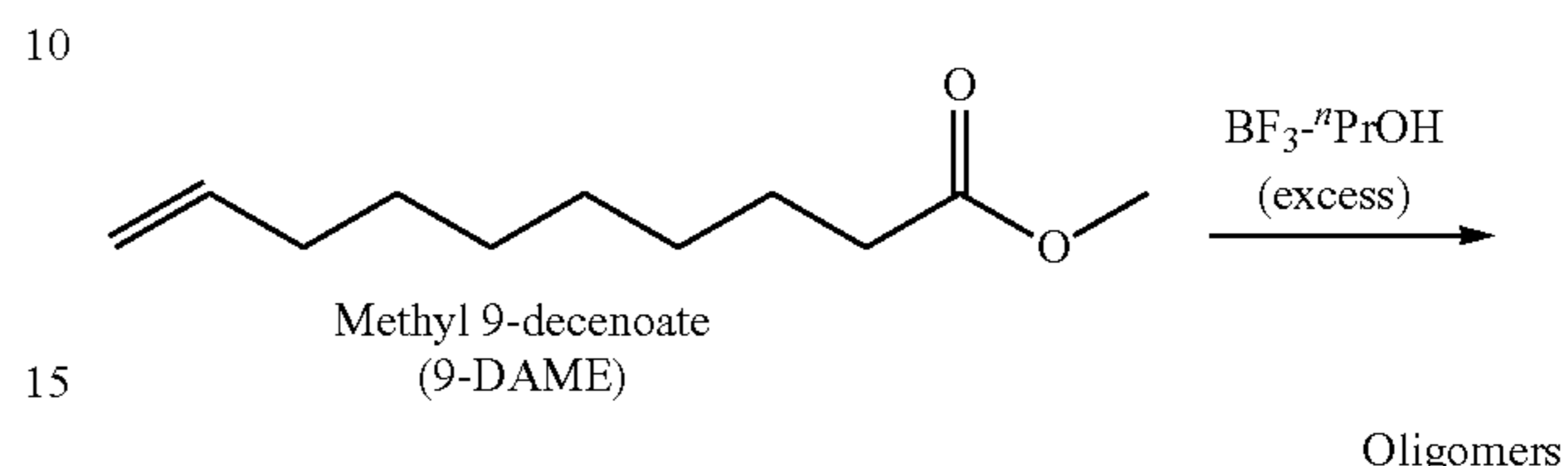
Scheme 1. BF 3 -mediated homo-oligomerization of methyl 9-decenoate (9-DAME).
