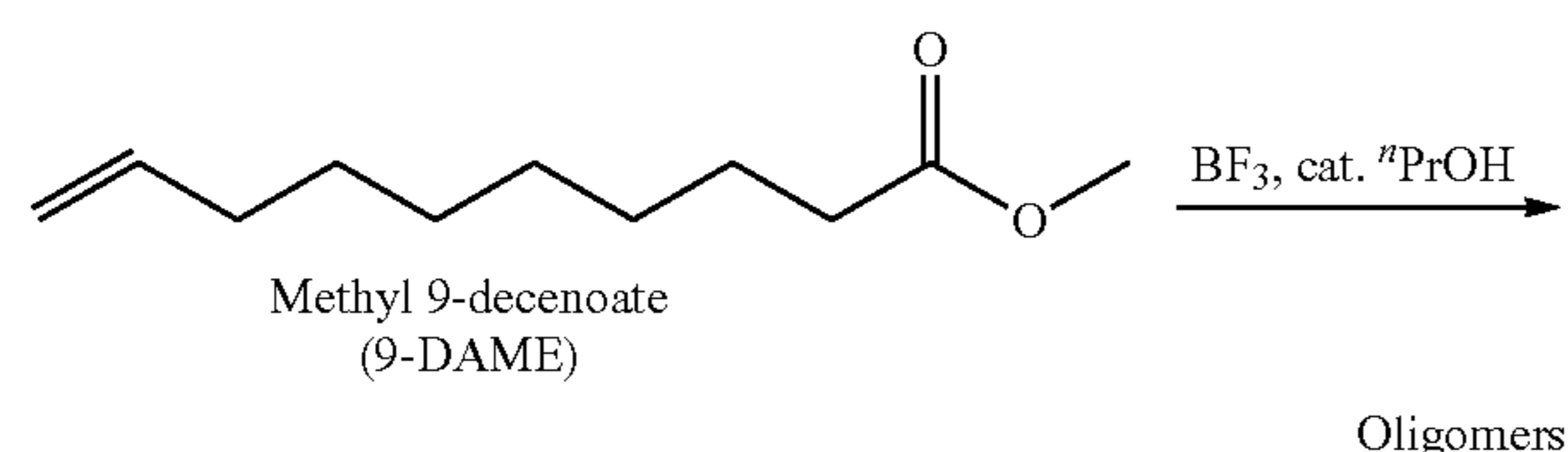
Scheme 1. \text{BF}_3 -mediated homo-oligomerization of methyl 9-decenoate.
