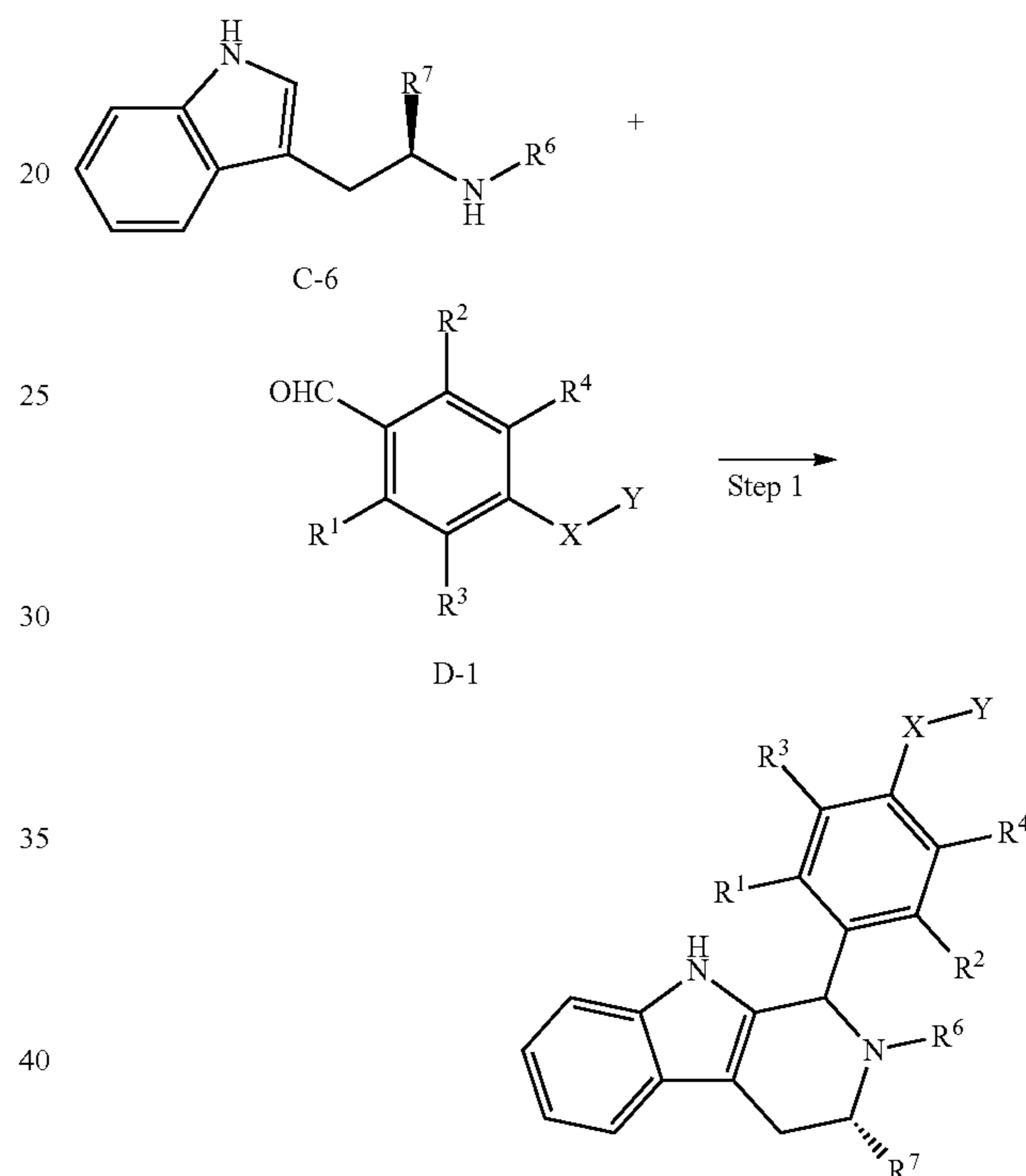
SCHEME D
