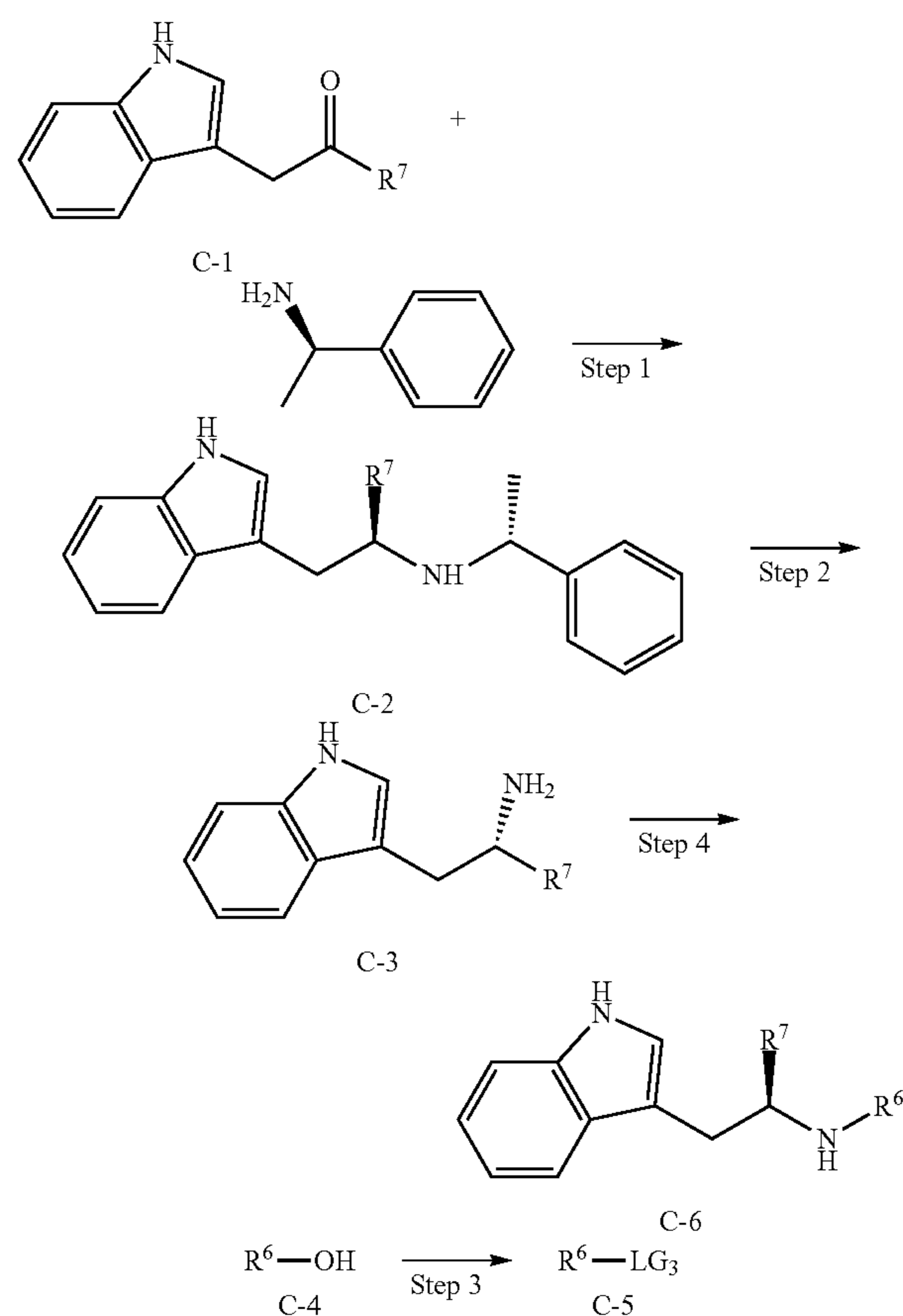
SCHEME C
