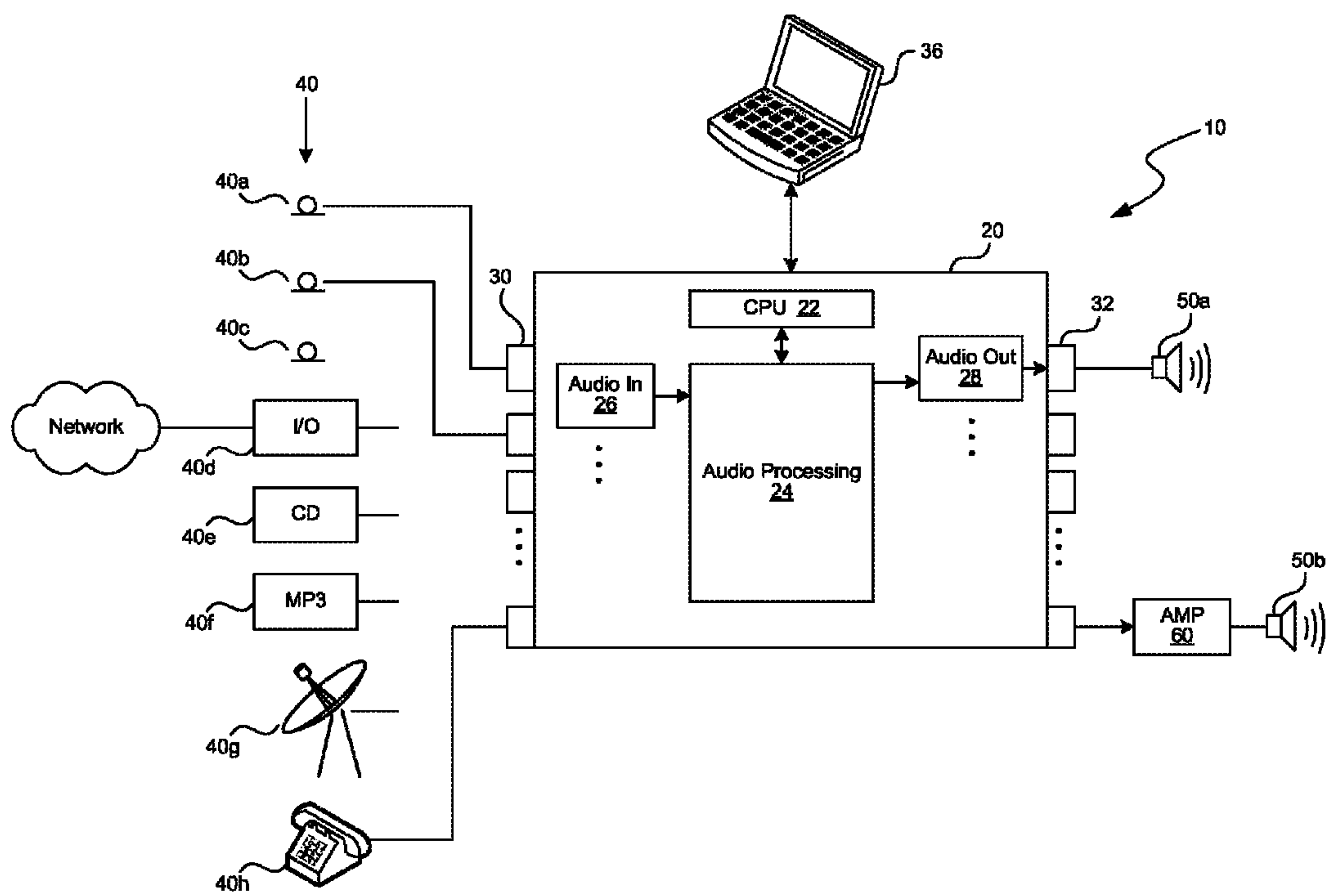
FIG. 1 (Prior Art)
