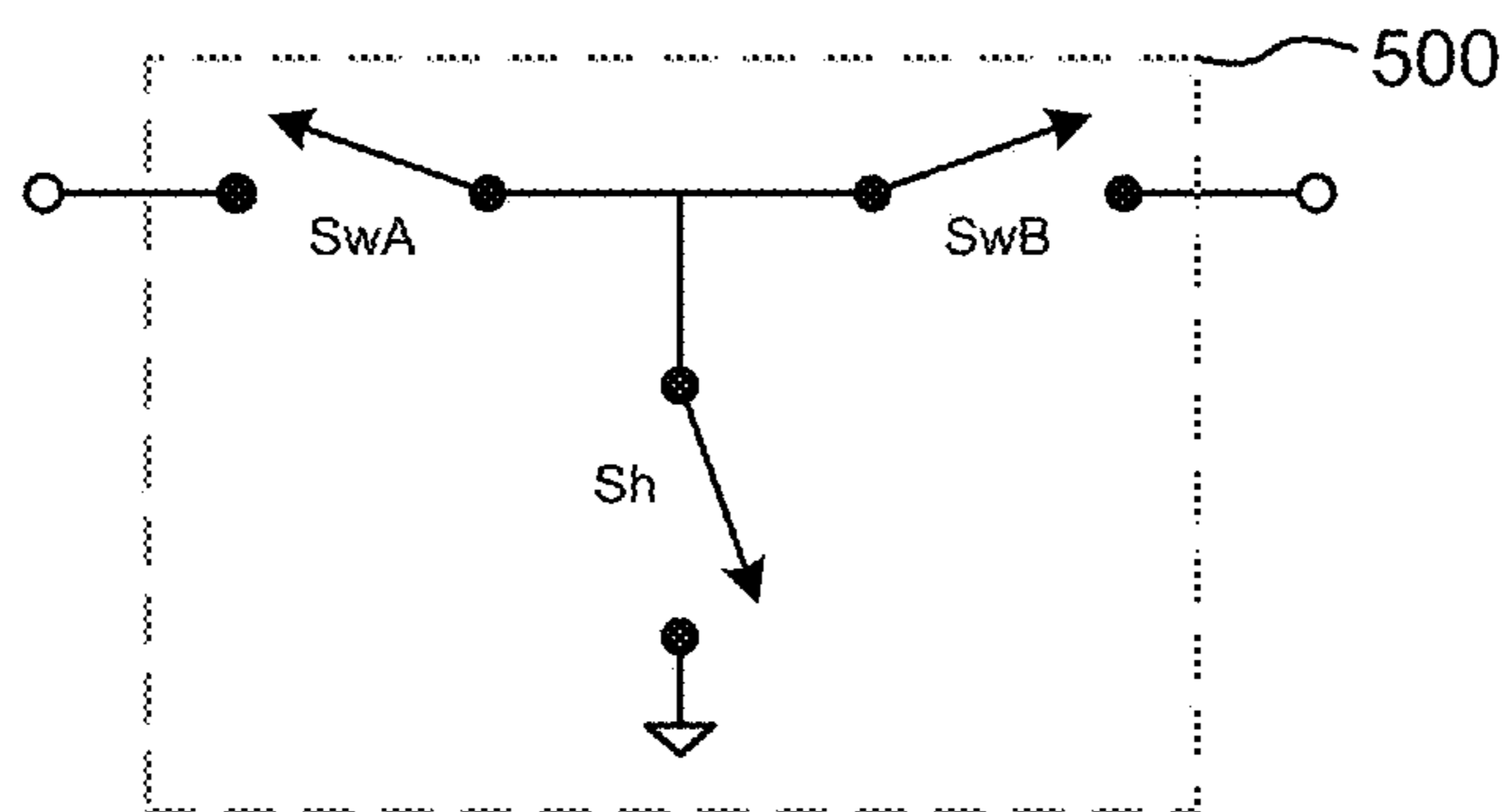
FIG. 5 Alternative Bypass Circuit
