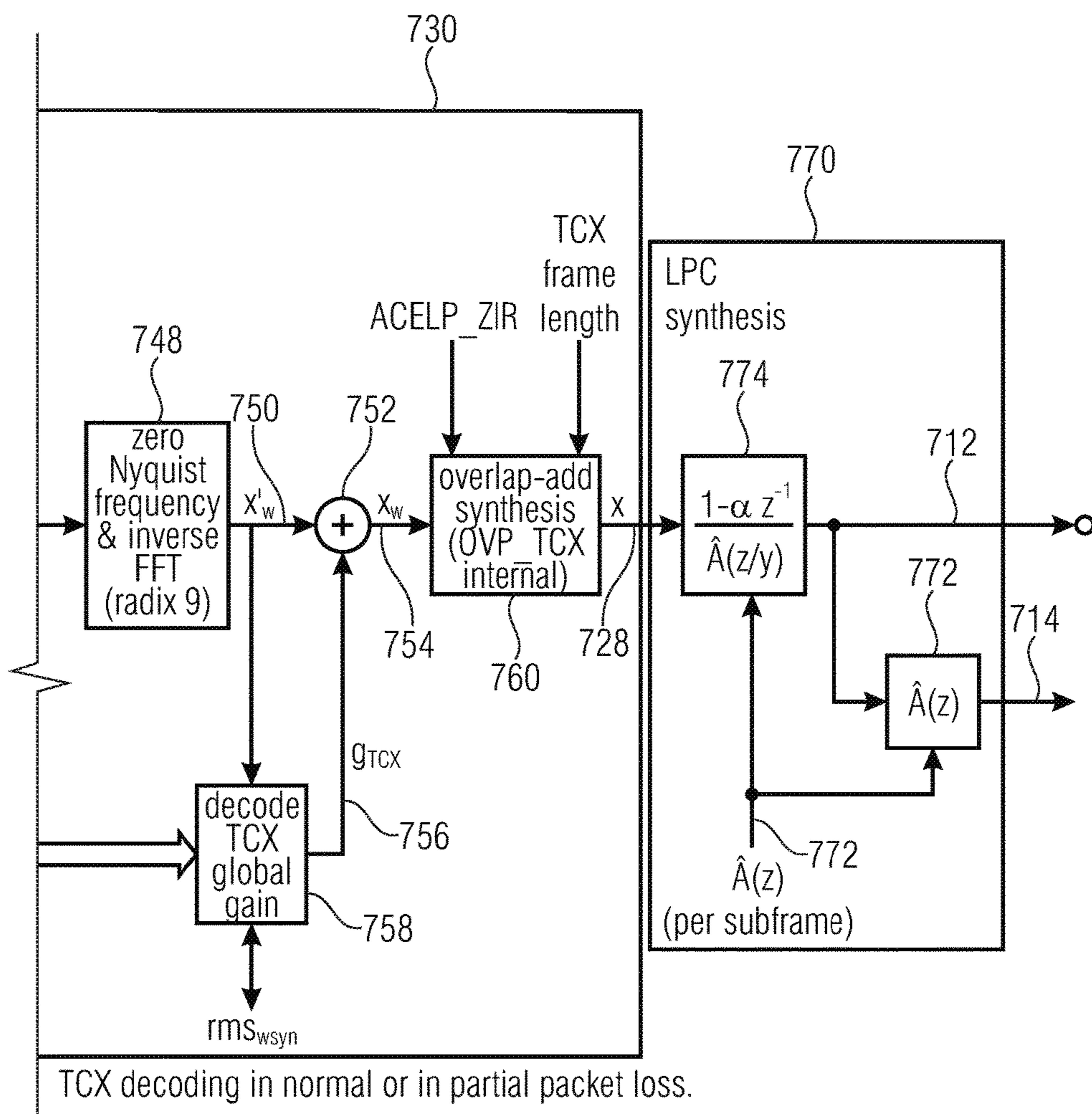
Block diagram of the TCX decoder
