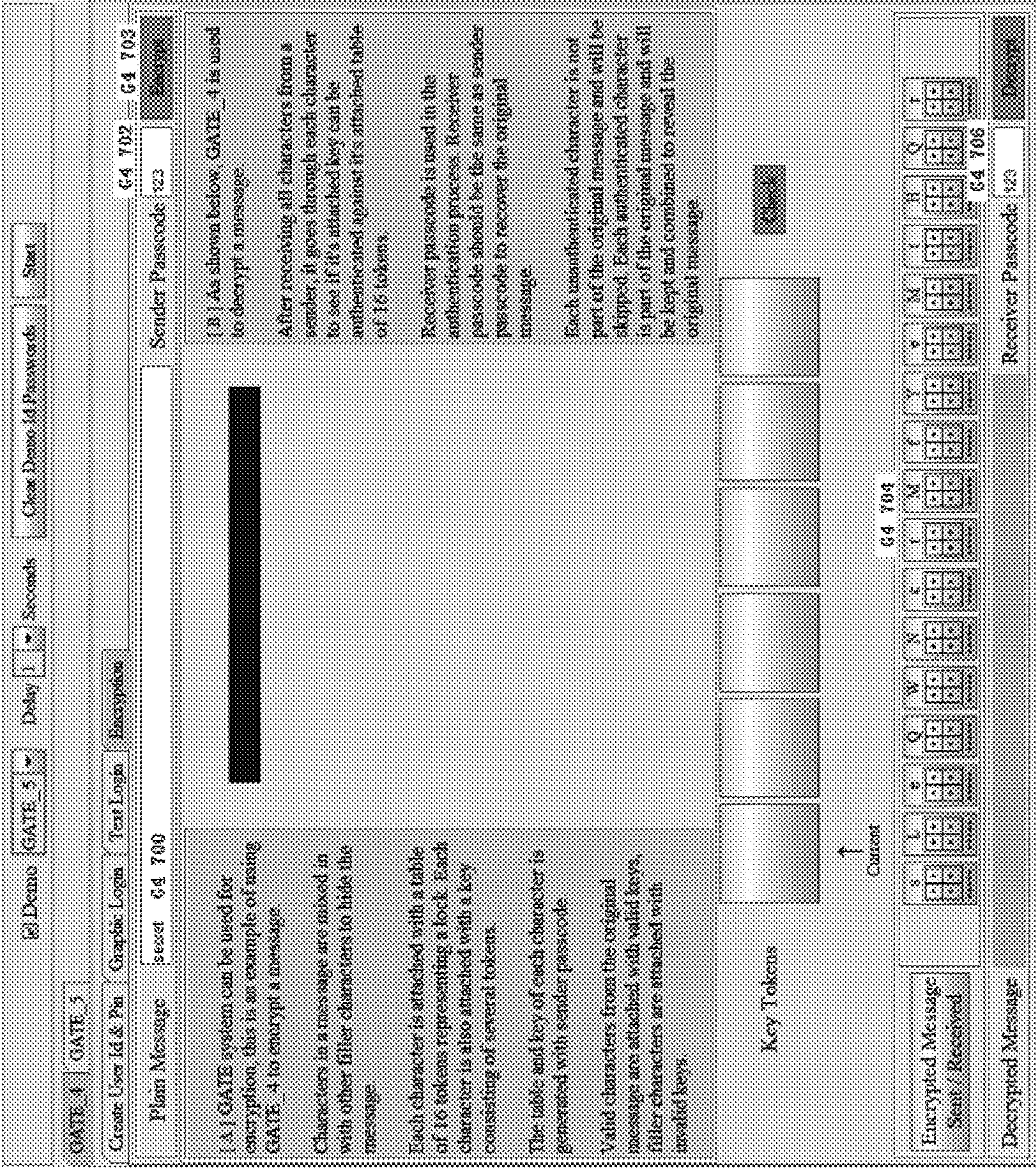
Fig. 14 GATE_4_Encryption
