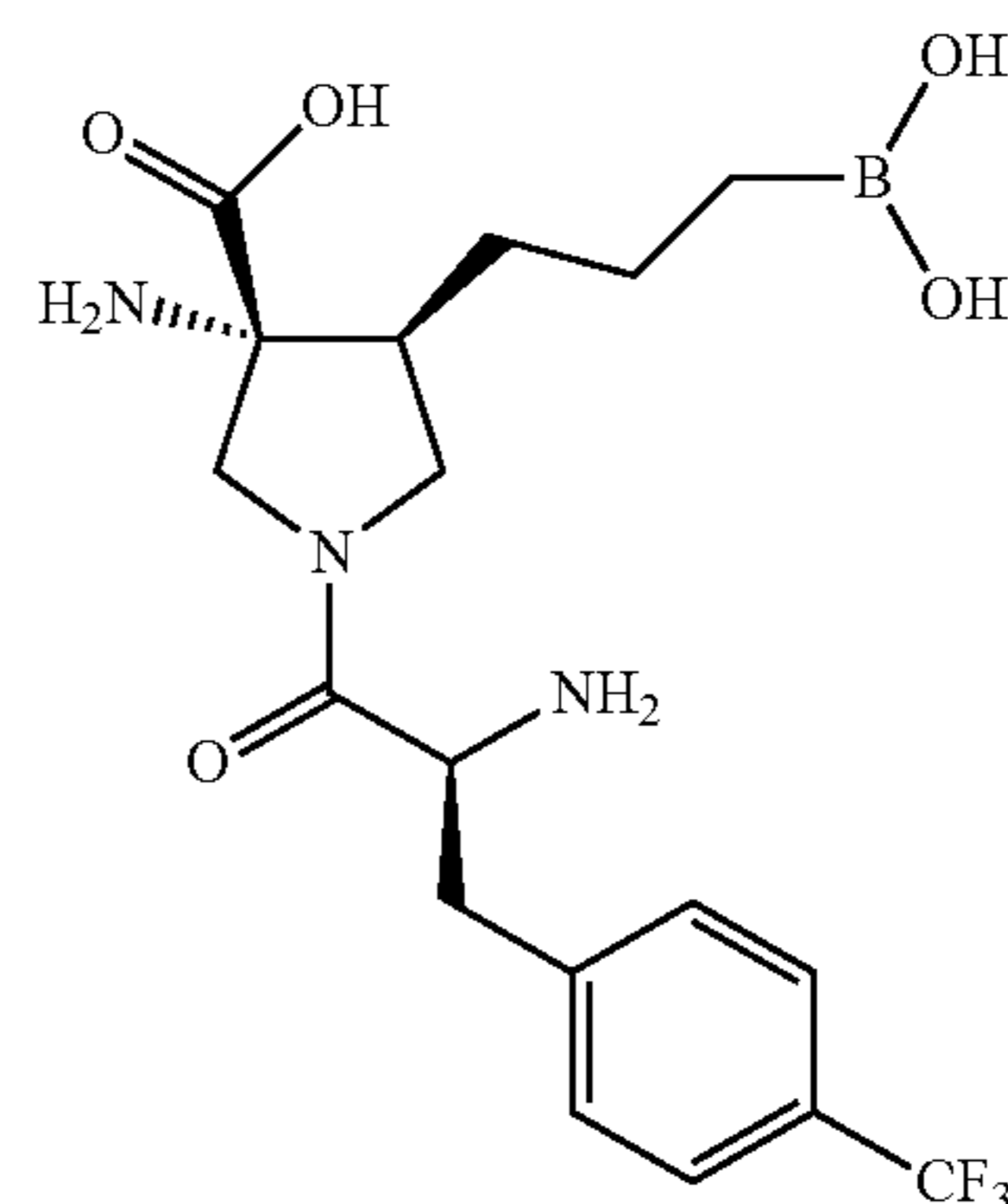
Trifluoromethyl phenylalanine AUC = 5783
