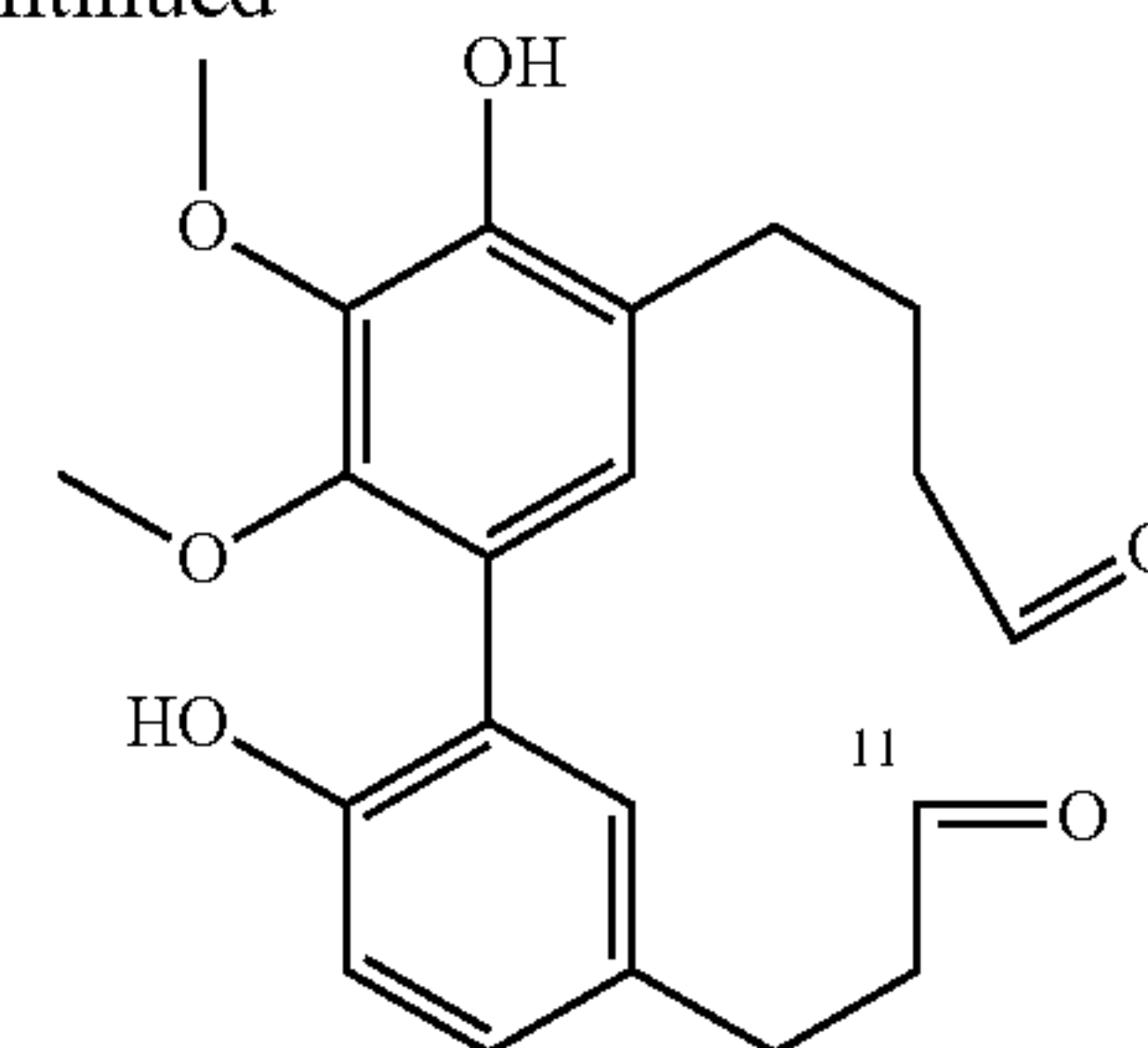
Dialdehyde A
