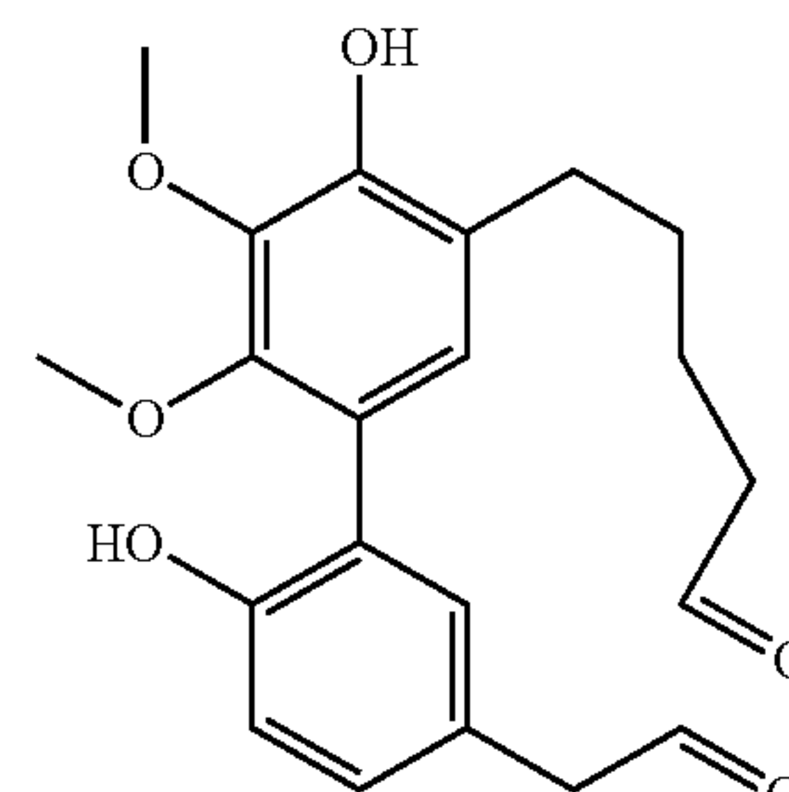
dialdehyde B
