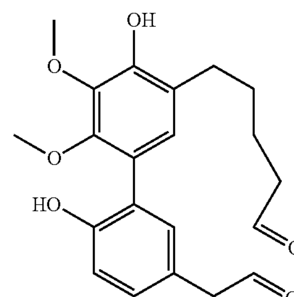
dialdehyde B
