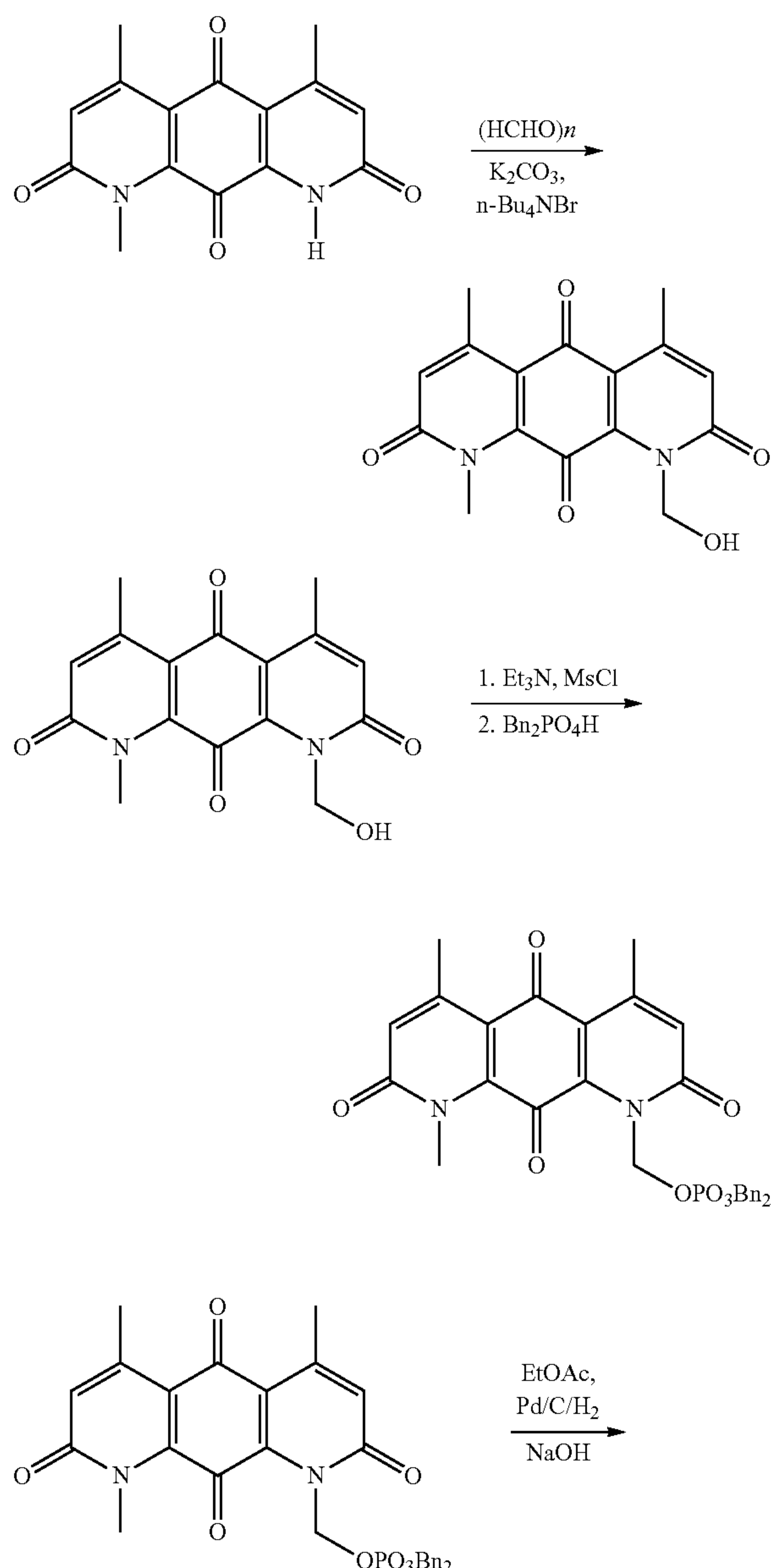
Scheme 7.1. Preparation of DNQ-P1.
