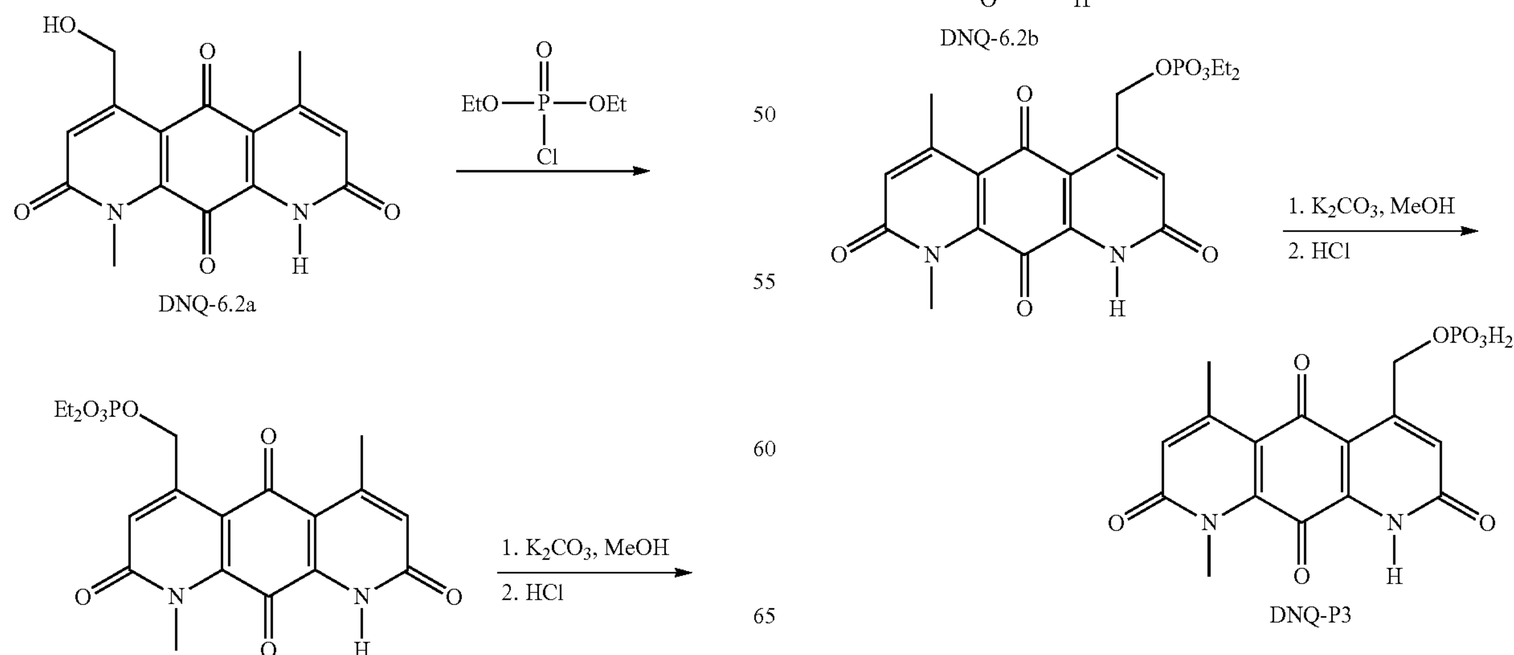
Scheme 7.3. Preparation of DNQ-P2 and DNQ-P3.
