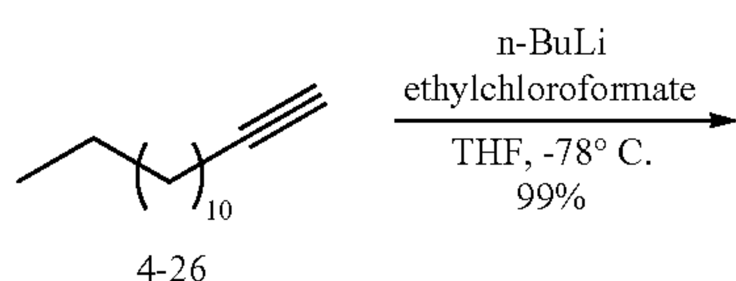
Scheme 4.2. Synthesis of alkynes 4-19 and 4-21 for preparation of 4-10 and 4-13.
