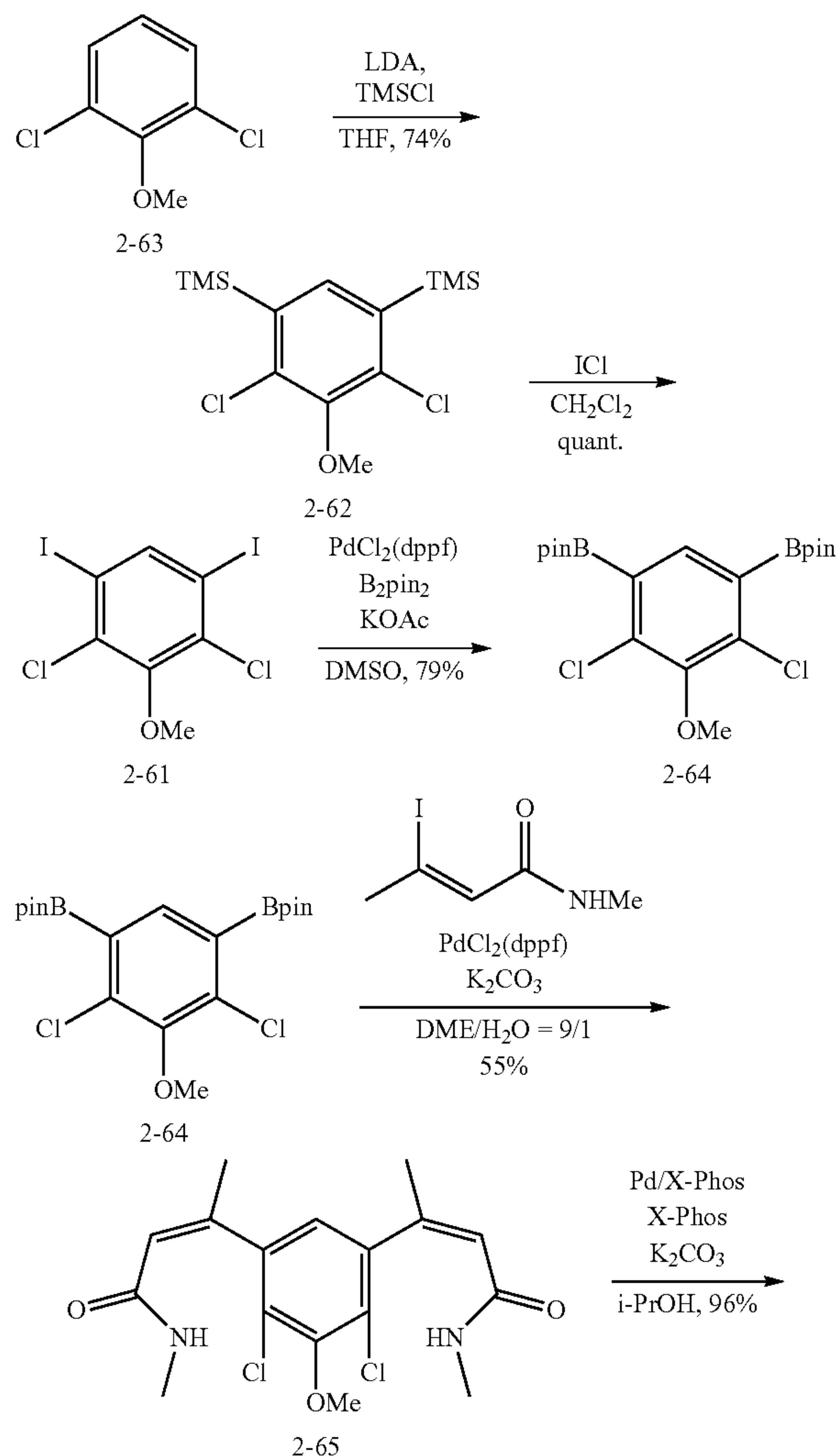
Scheme 1.12. Synthesis of SCH 538415.
