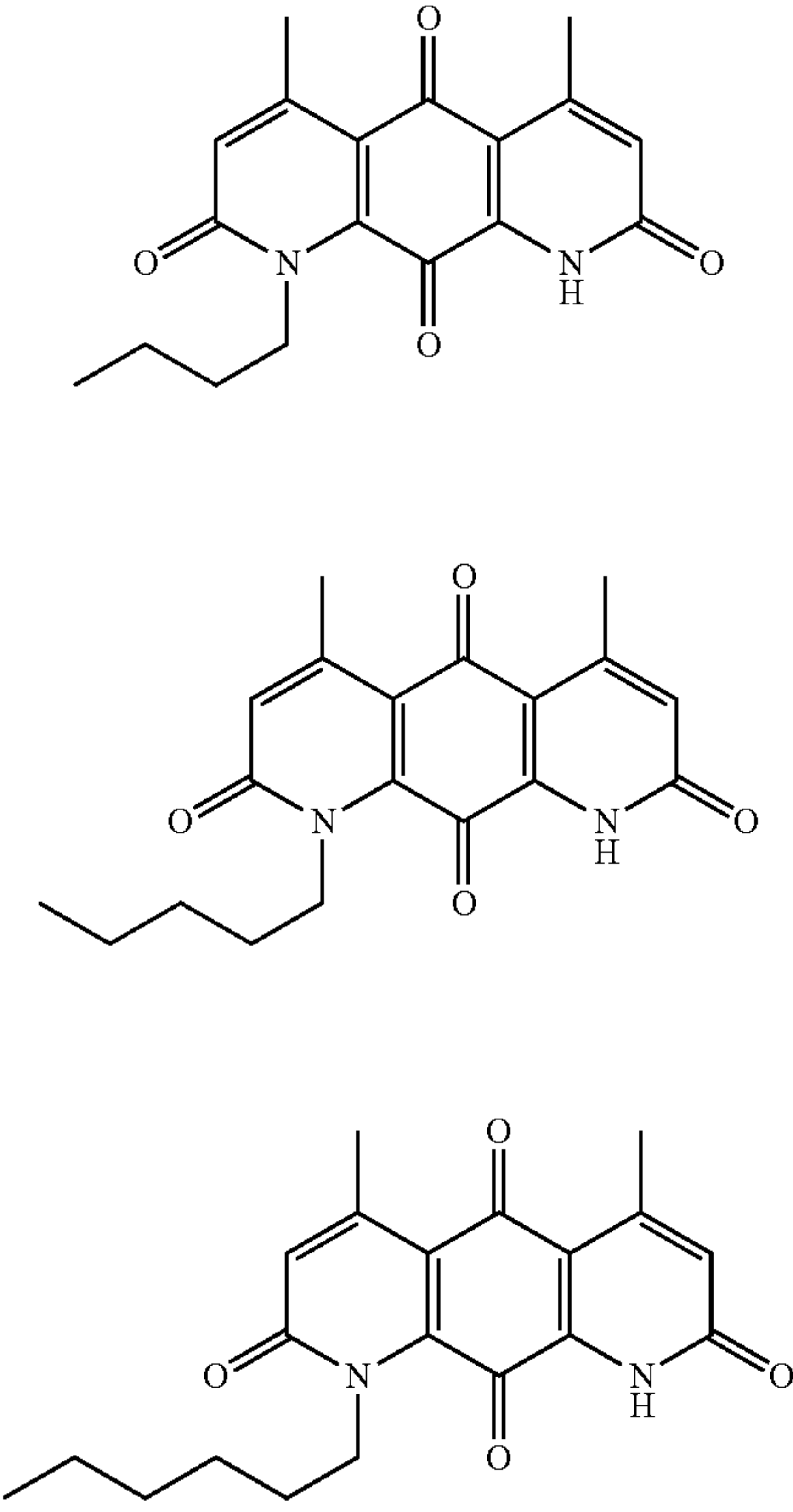
Scheme 4.3. New DNQ derivatives.
