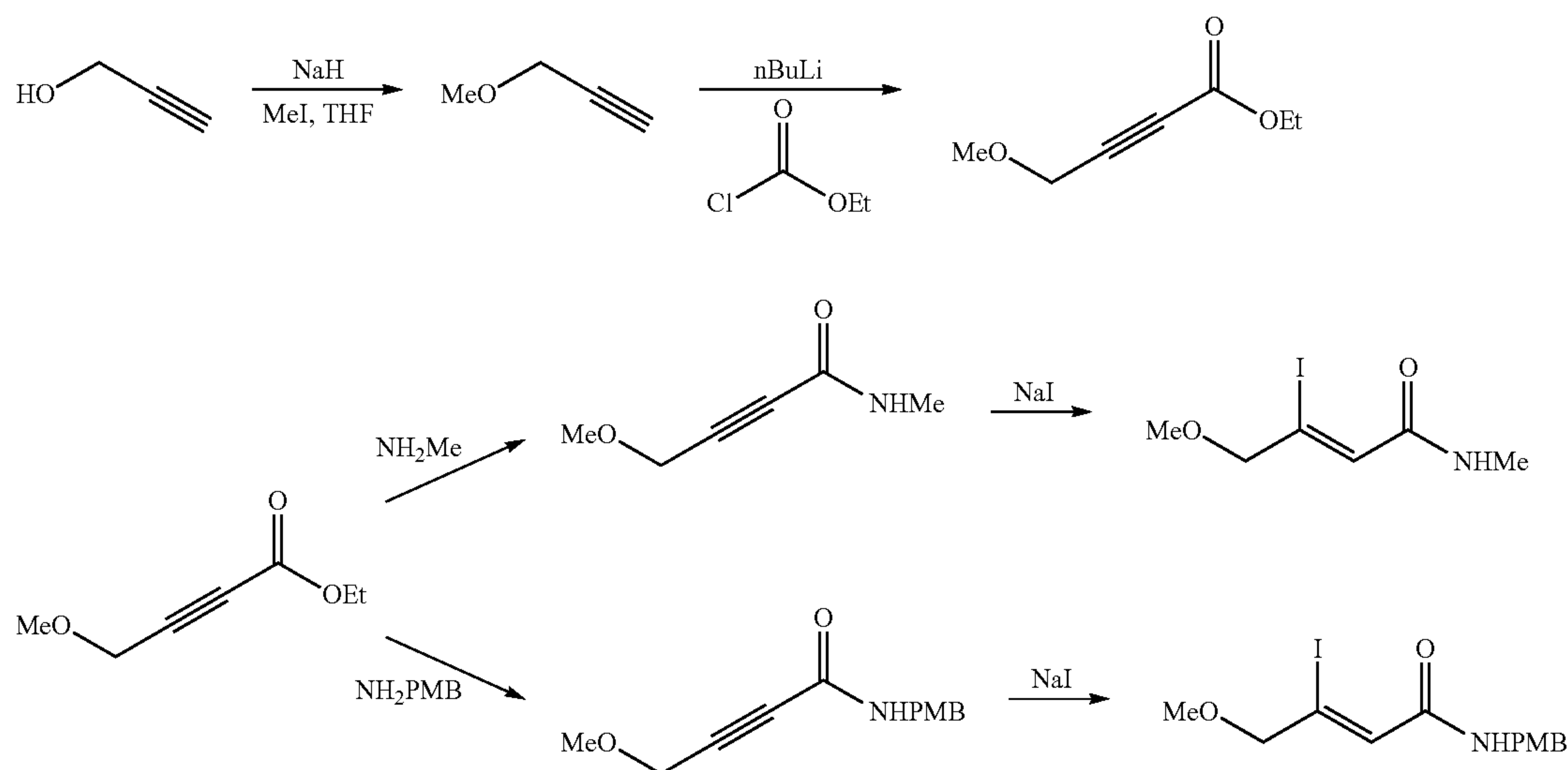
Scheme 7.2. Preparation of DNQ-P2 and DNQ-P3 Intermediates.
