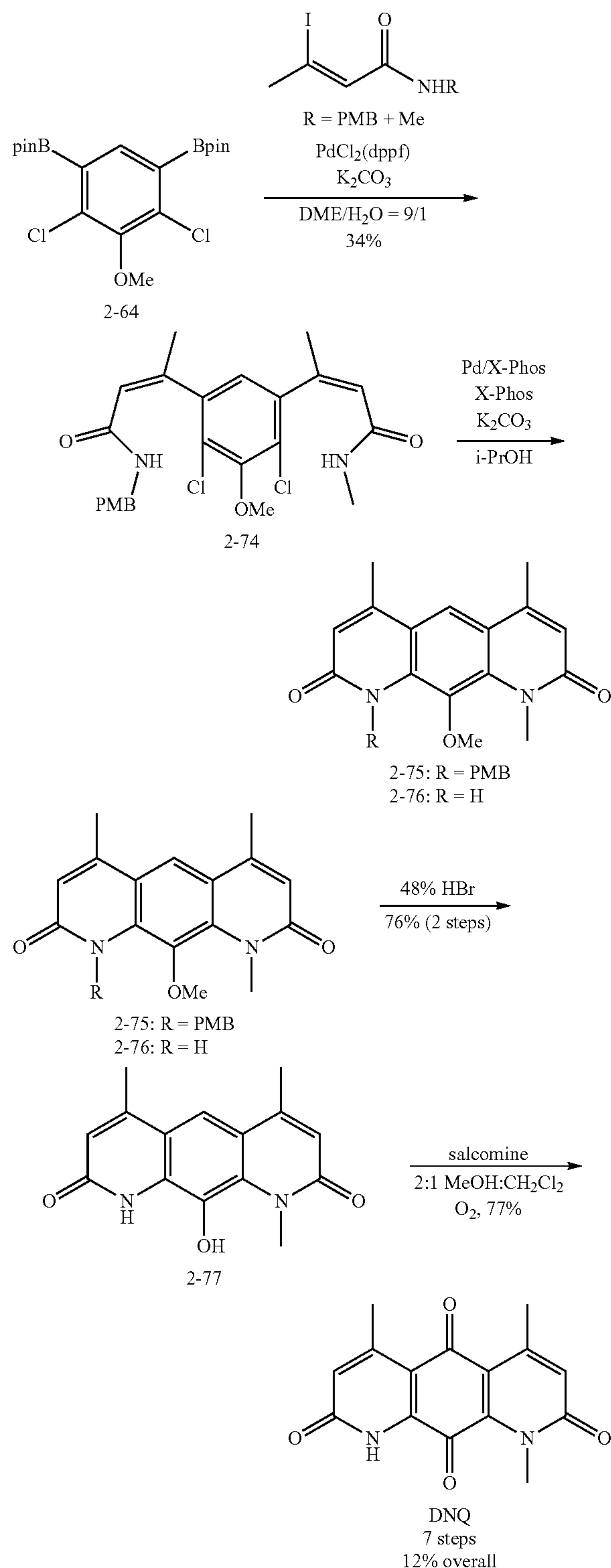
Scheme 1.14. Robust and scalable synthesis of DNQ.
