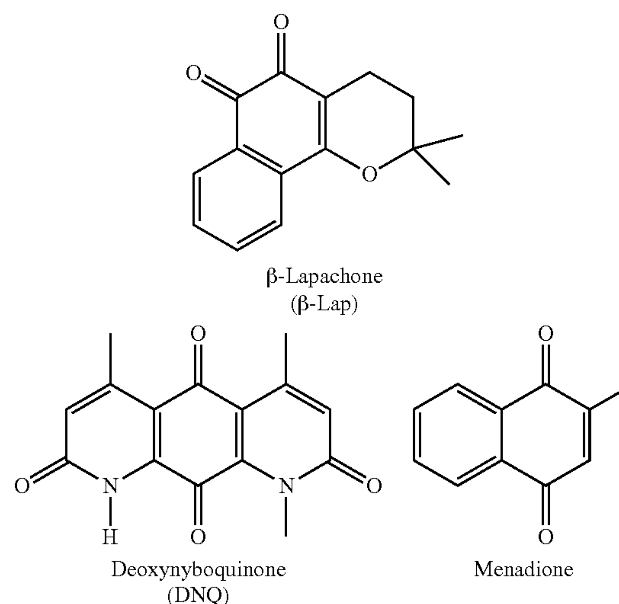
Scheme 1. Example of Quinone Compounds.
