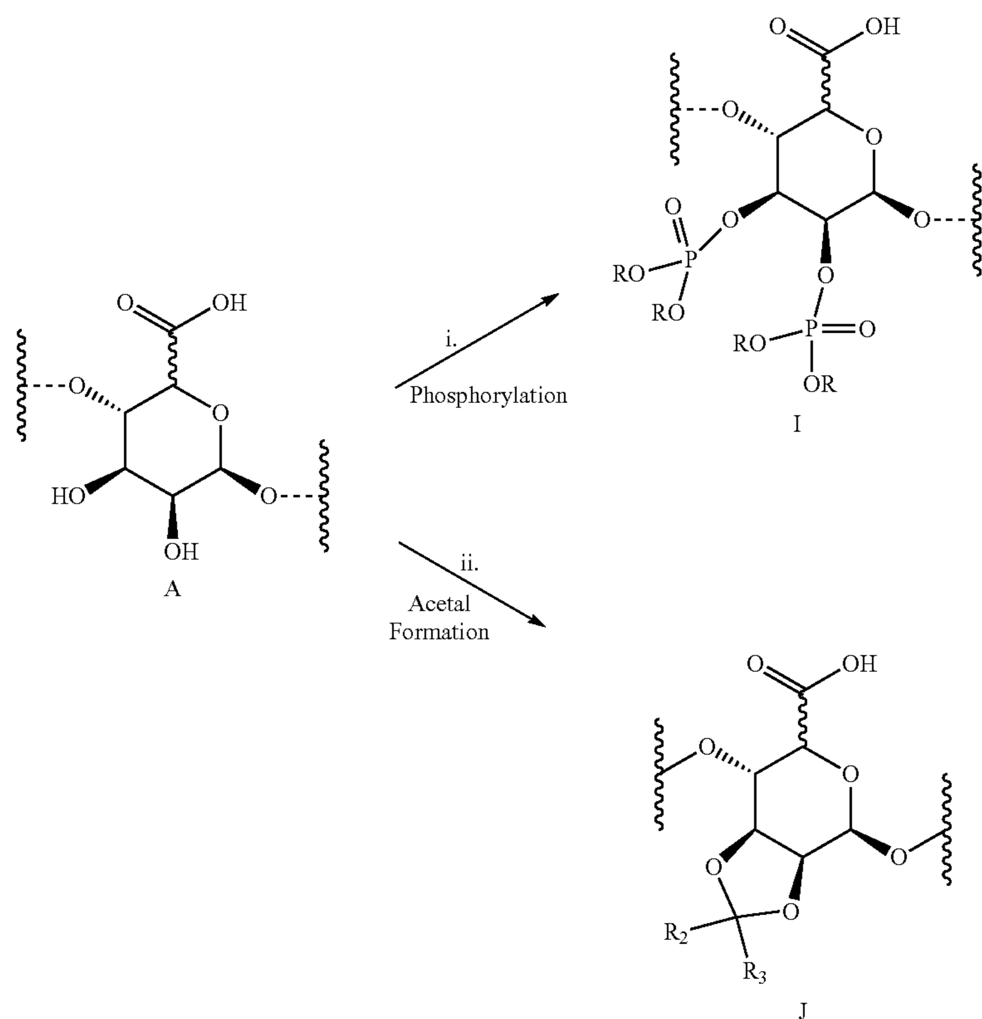
Scheme 3.
