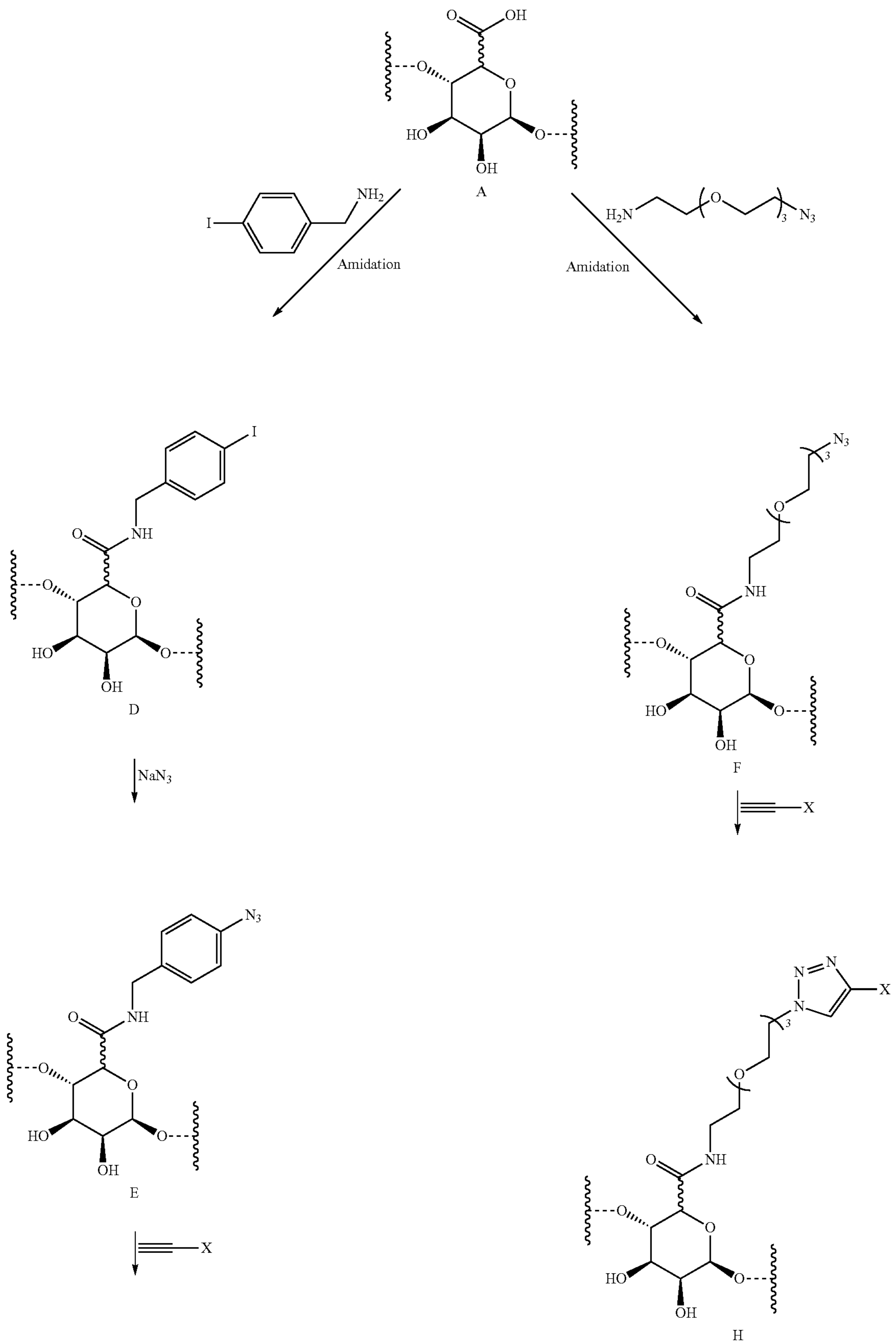
Scheme 2.
