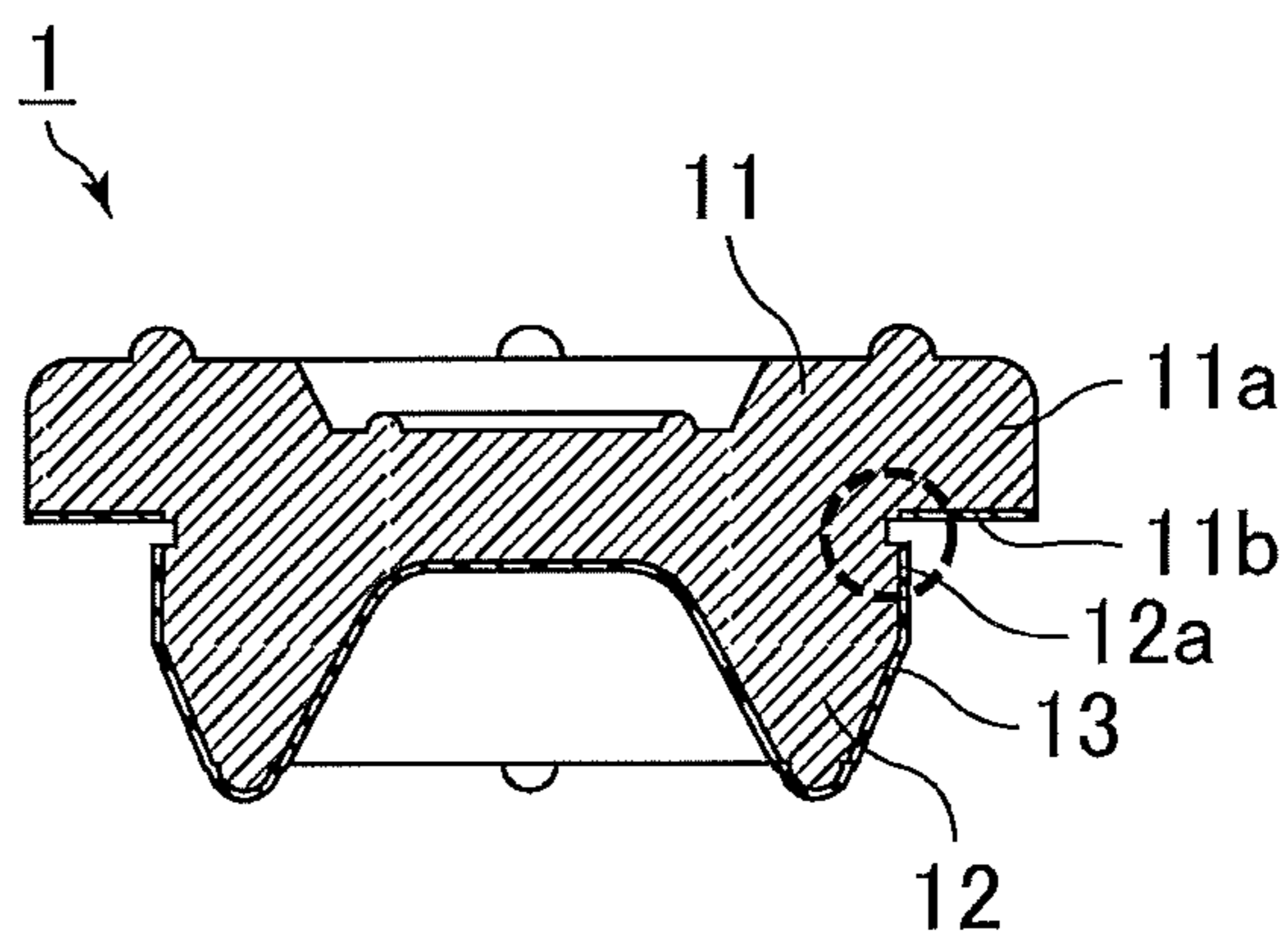
A-A cross-sectional view
