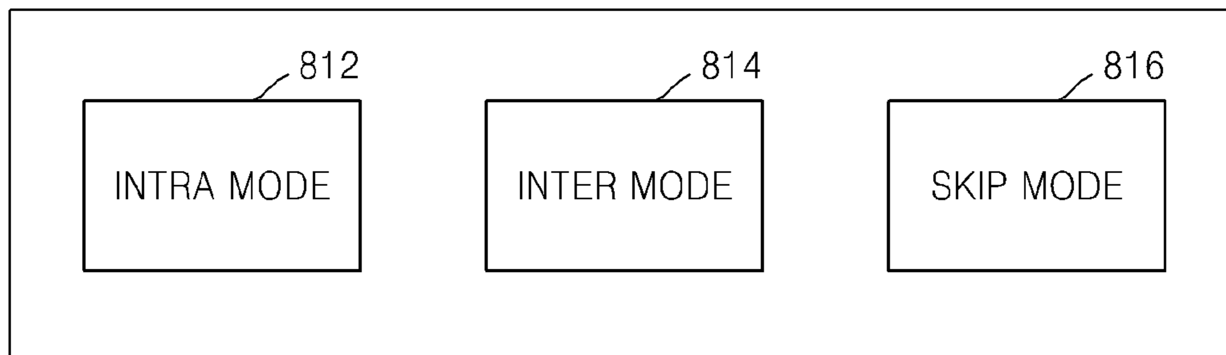
'PREDICTION MODE'-INFORMATION (810)
