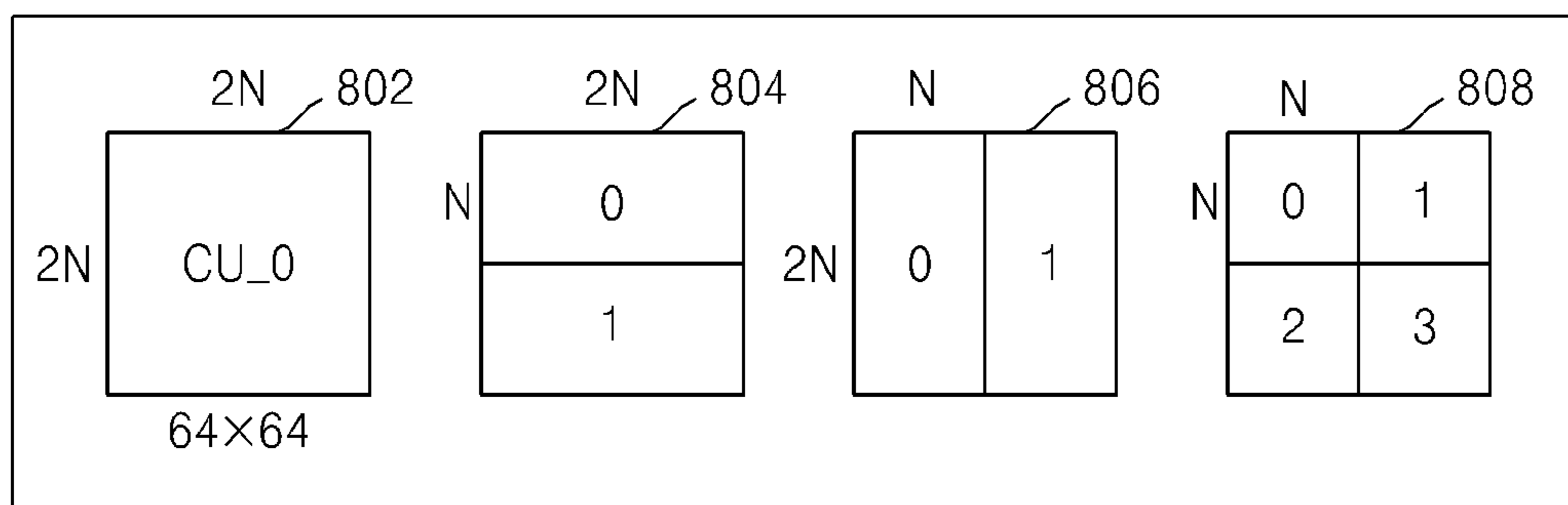
'PARTITION TYPE'-INFORMATION (800)
