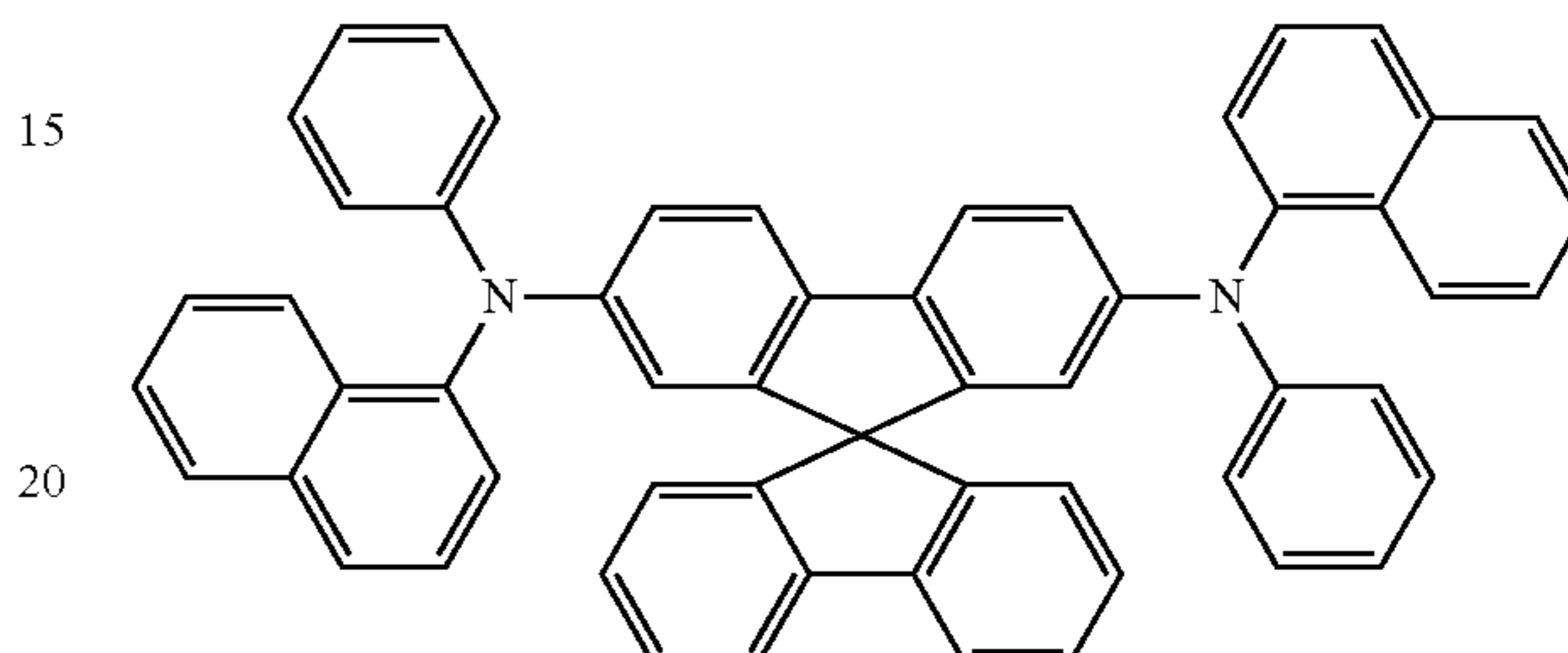
Spiro-TPD
