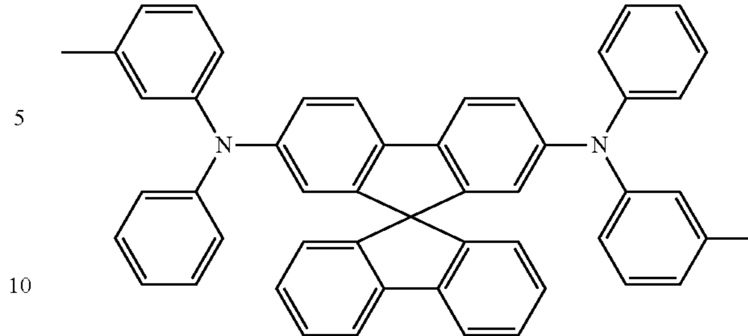
Spiro-TPD
