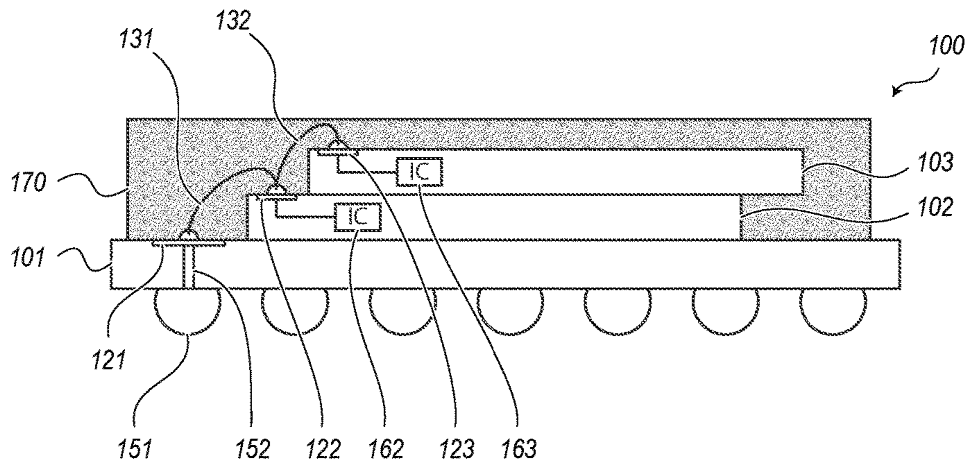
Figure 1 (Prior Art)
