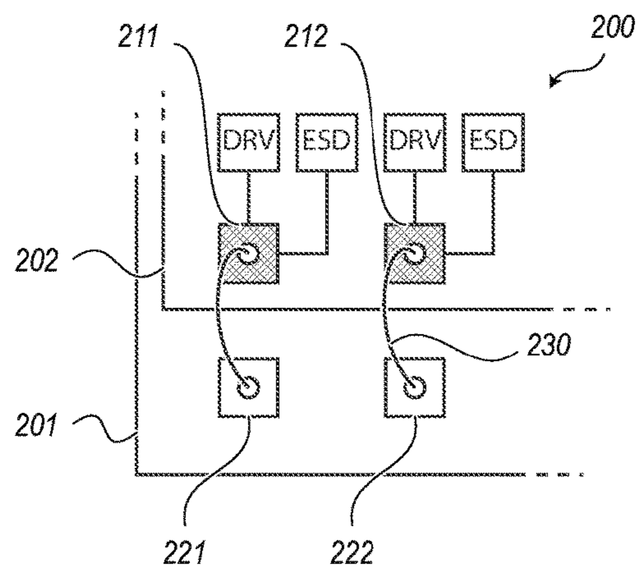
Figure 2 (Prior Art)
