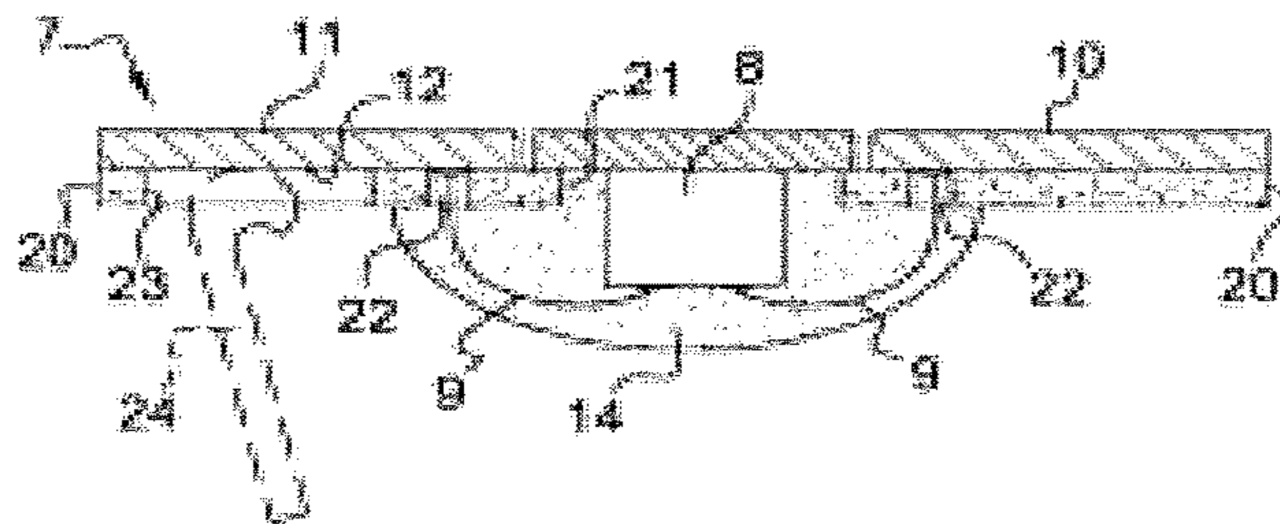
Fig. 2 Prior art cross section A-A
