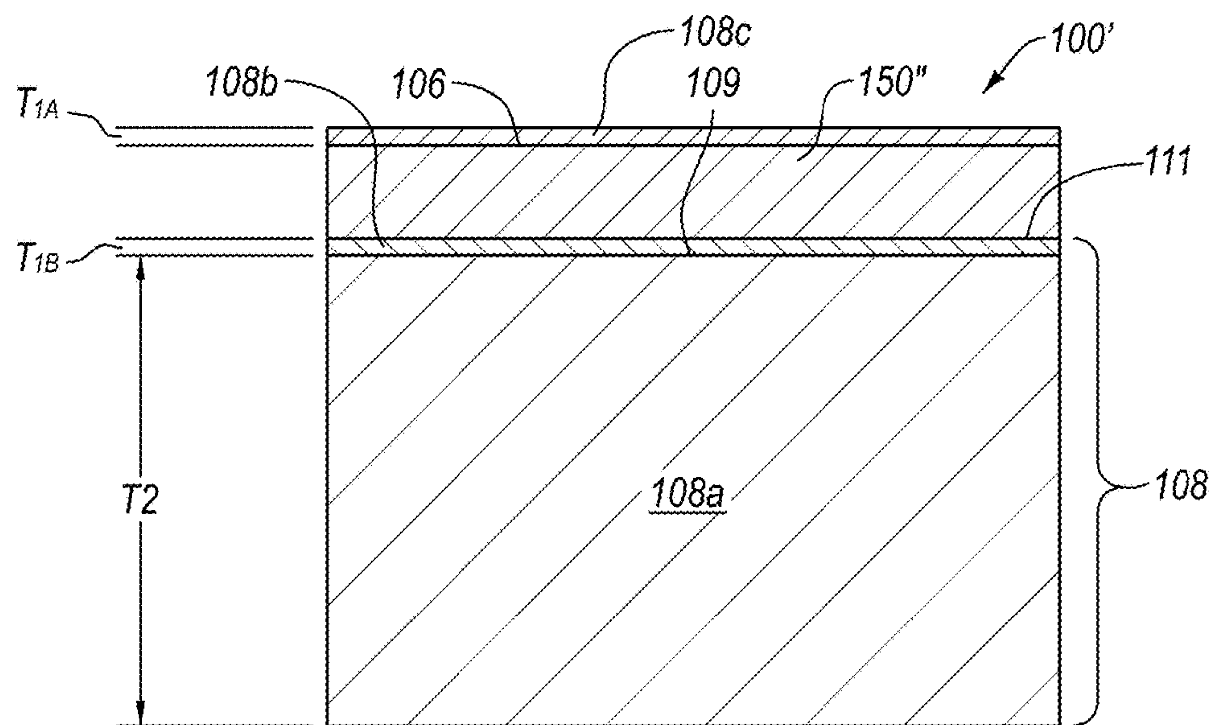
FIG. 3D
