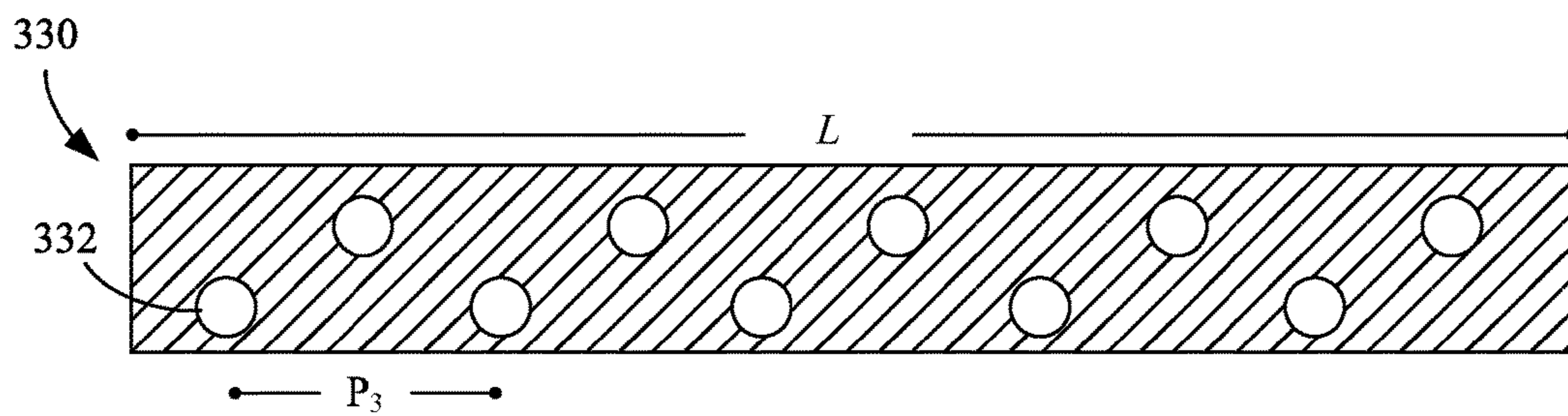
FIG. 3D
