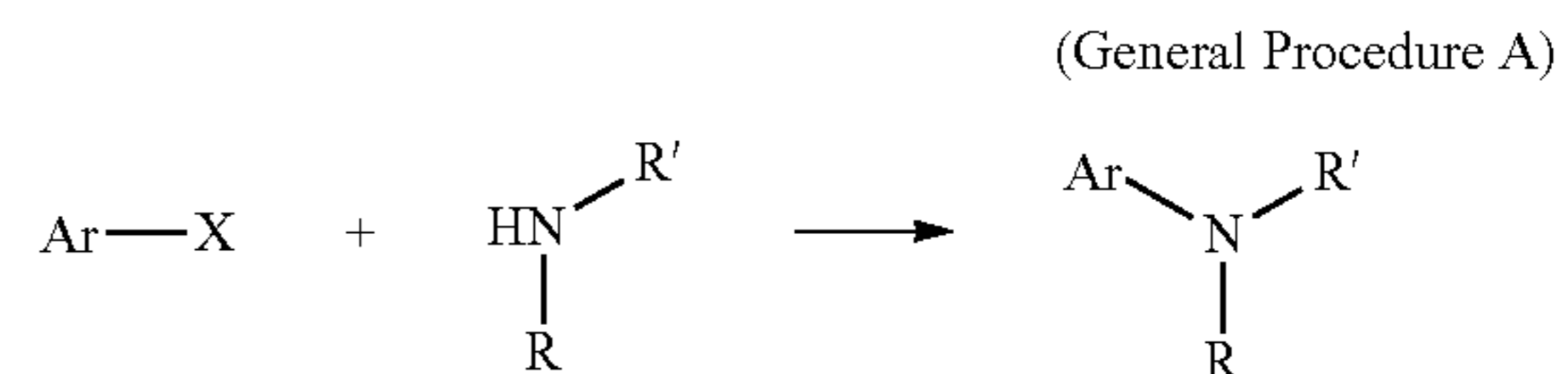
Scheme 1: Nucleophilic displacement of an aryl or heteroaryl halide with an amine
