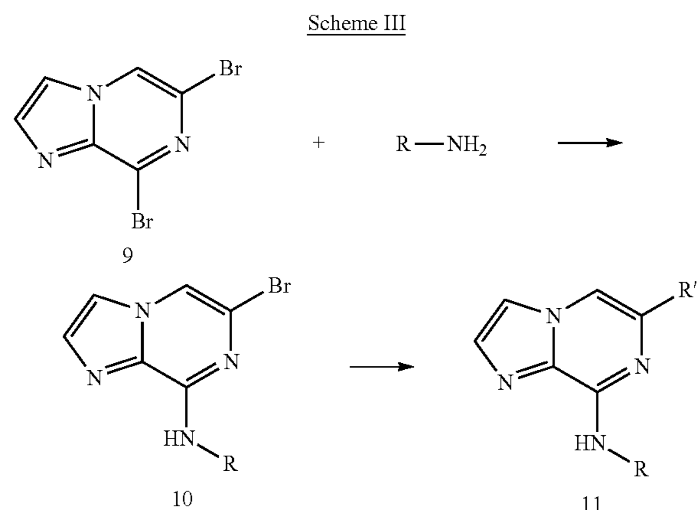
Scheme 1: Nucleophilic displacement of an aryl or heteroaryl halide with an amine
