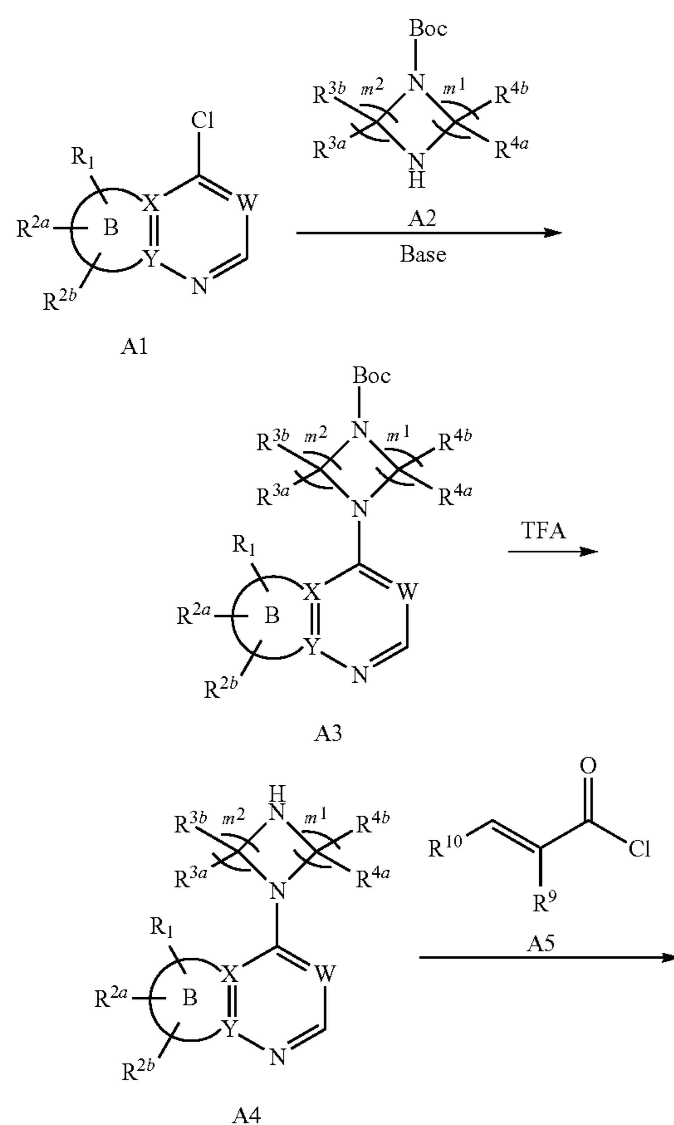
General Reaction Scheme 1
