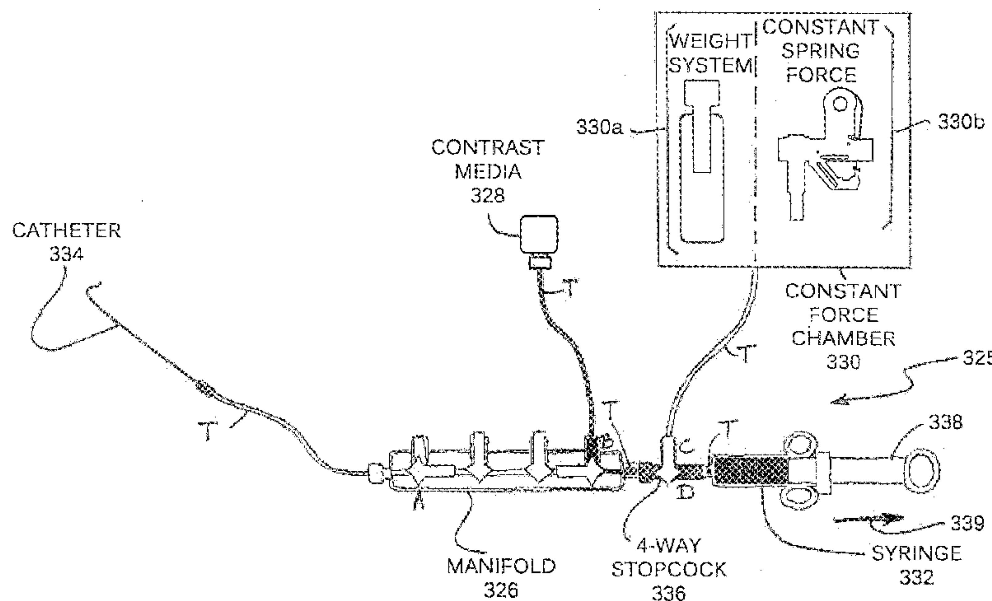
Exemplary Constant Force Modulator -- Filling Injector
