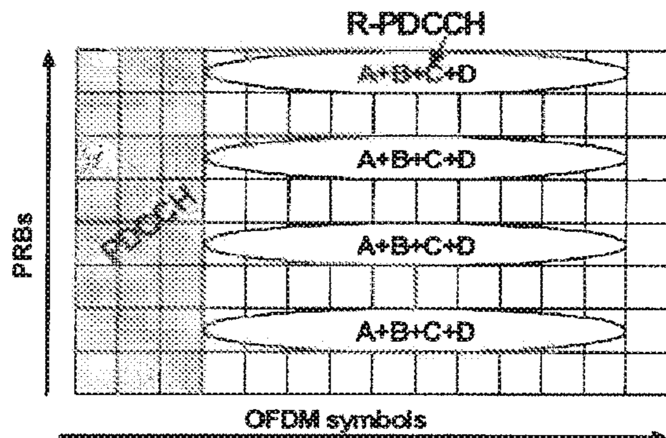
a) Frequency diversity R-PDCCH transmission
