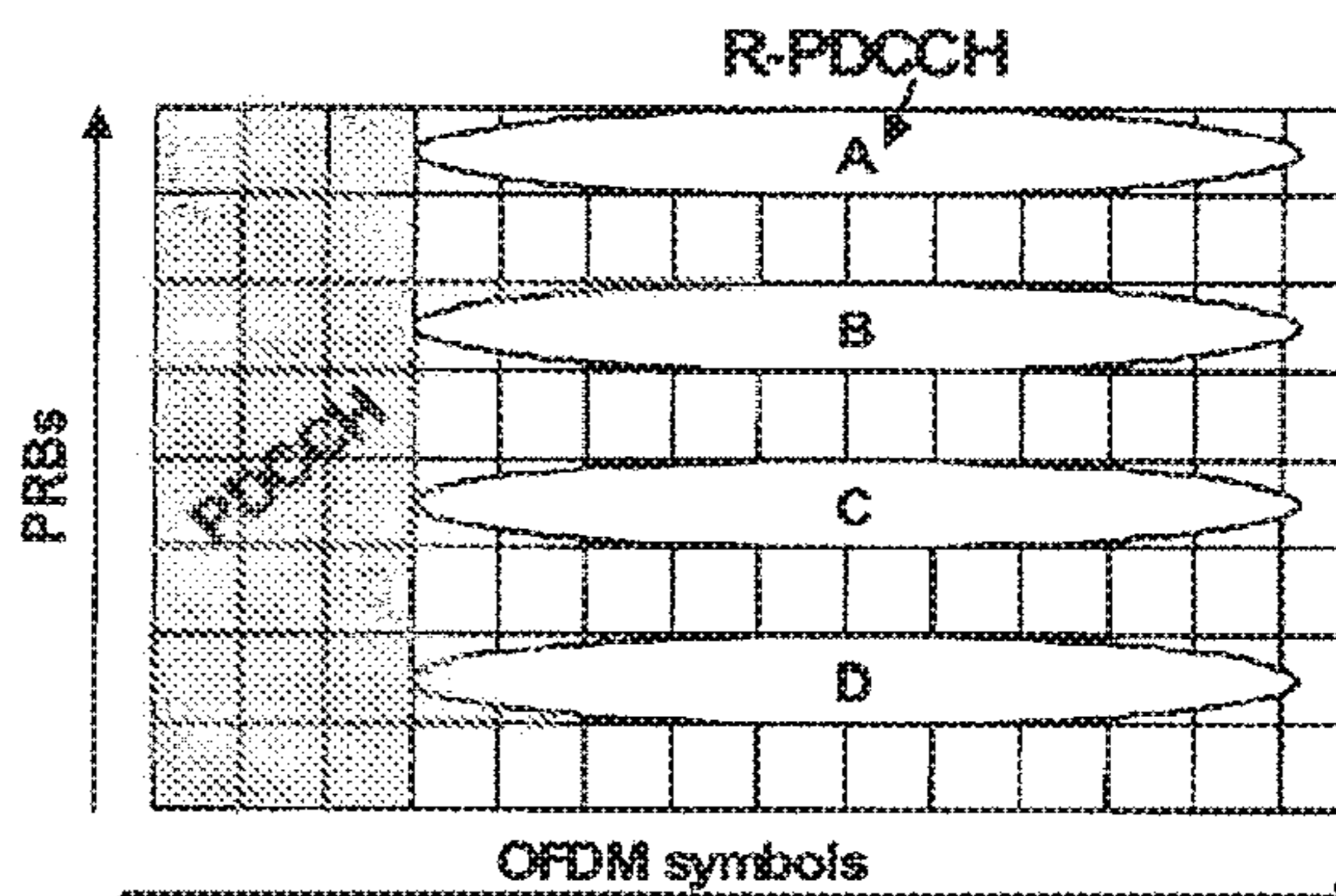
b) Frequency selective R-PDCCH transmission
