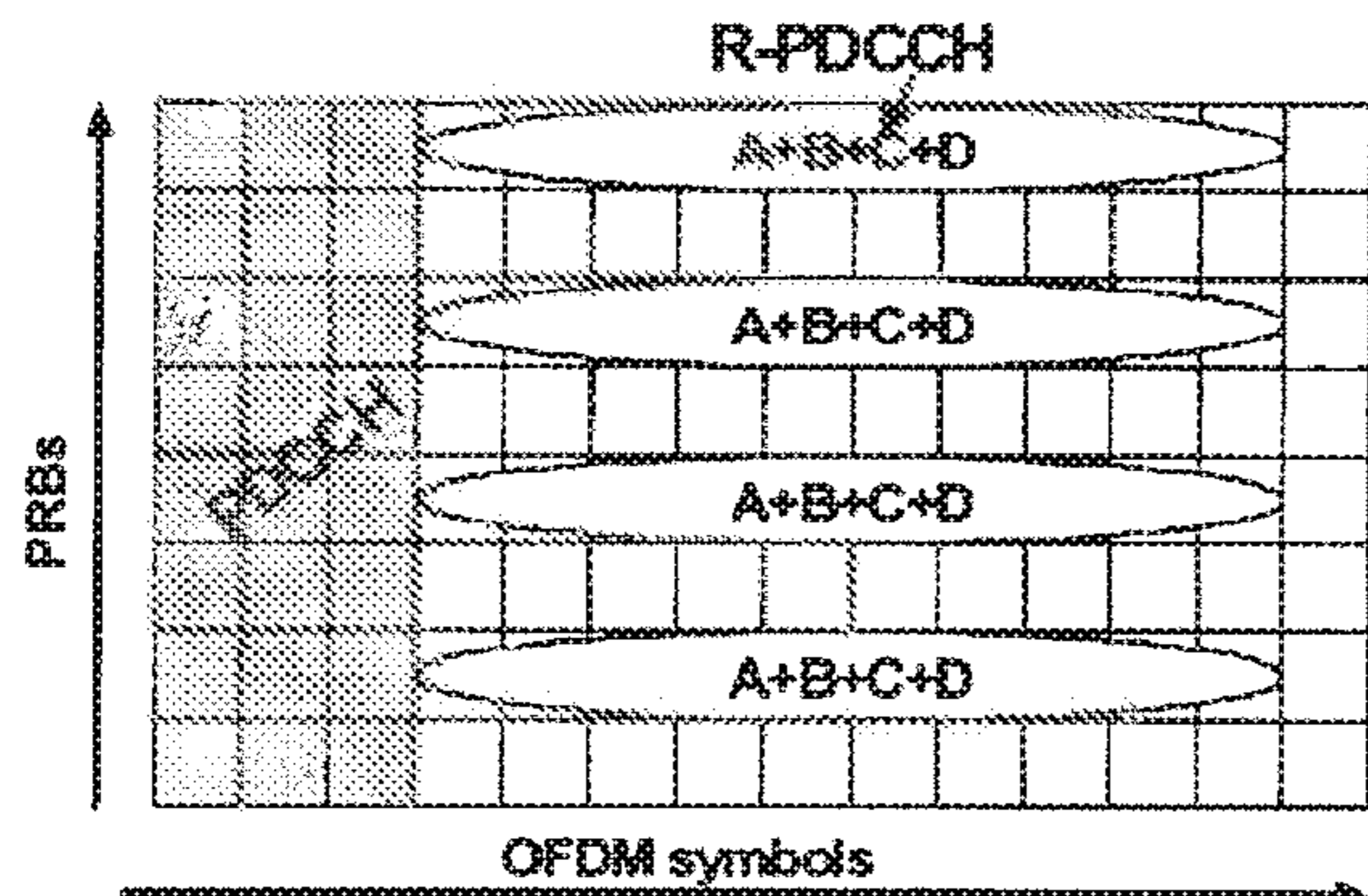
a) Frequency diversity R-PDCCH transmission
