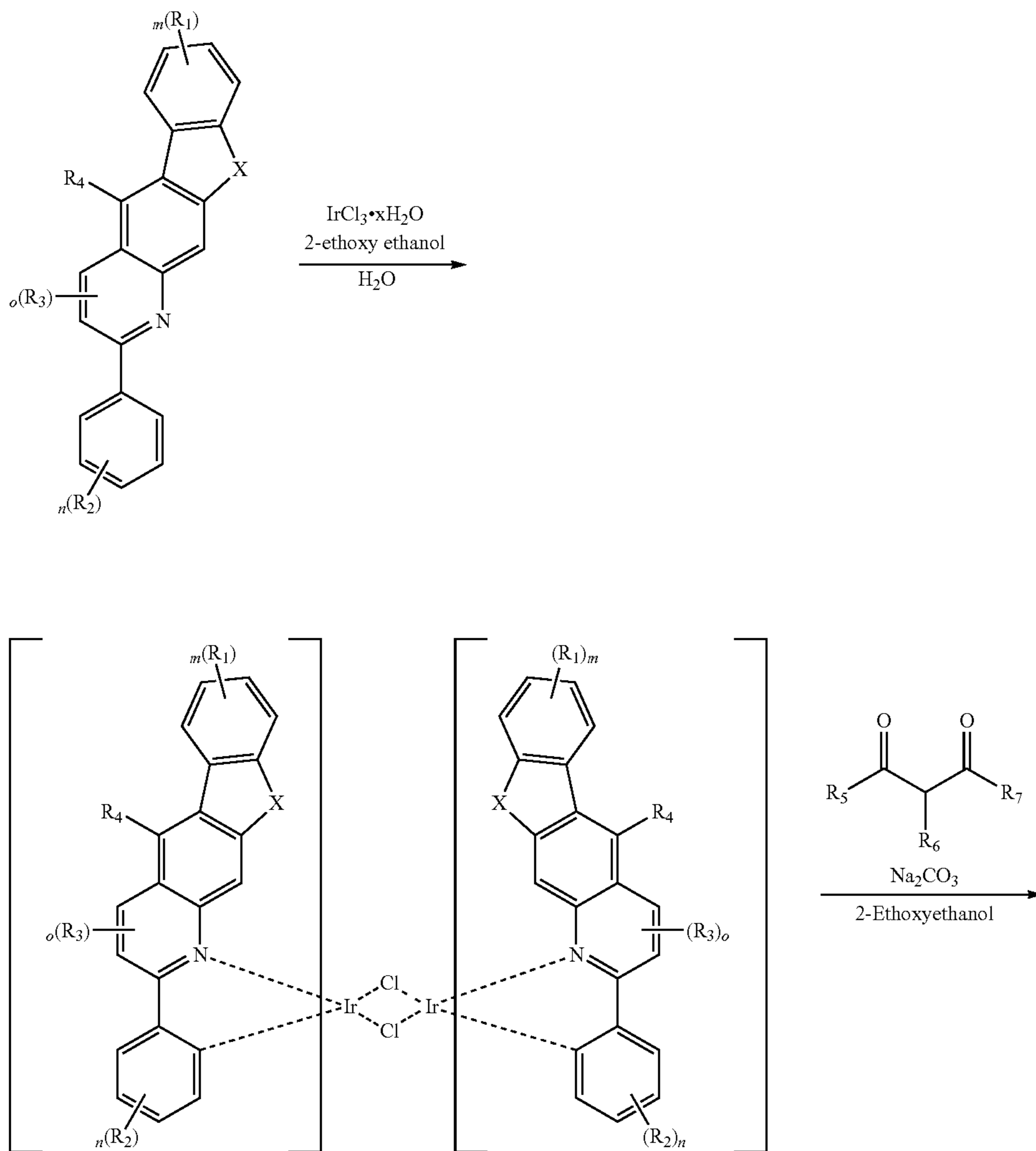
[Reaction Scheme 1]
