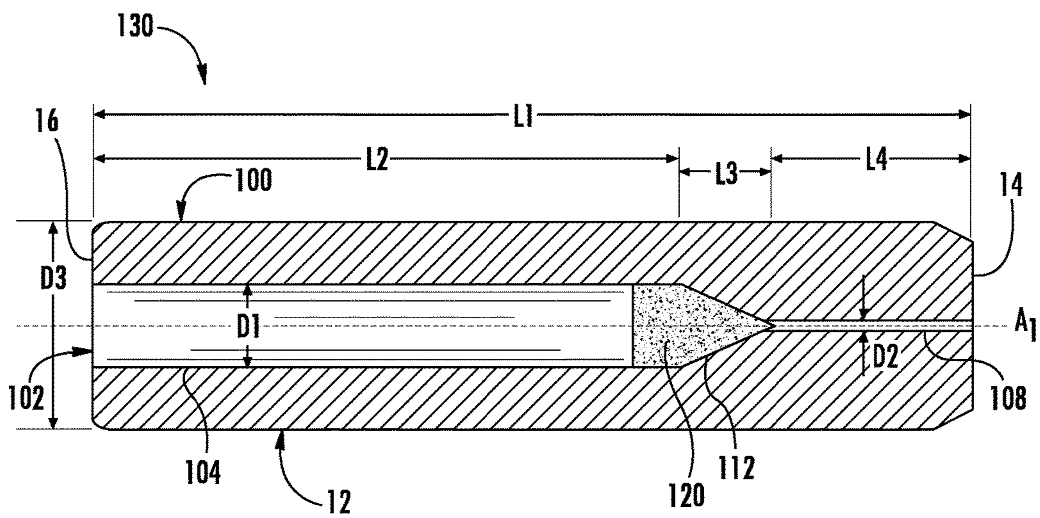
FIG. 4 PRIOR ART
