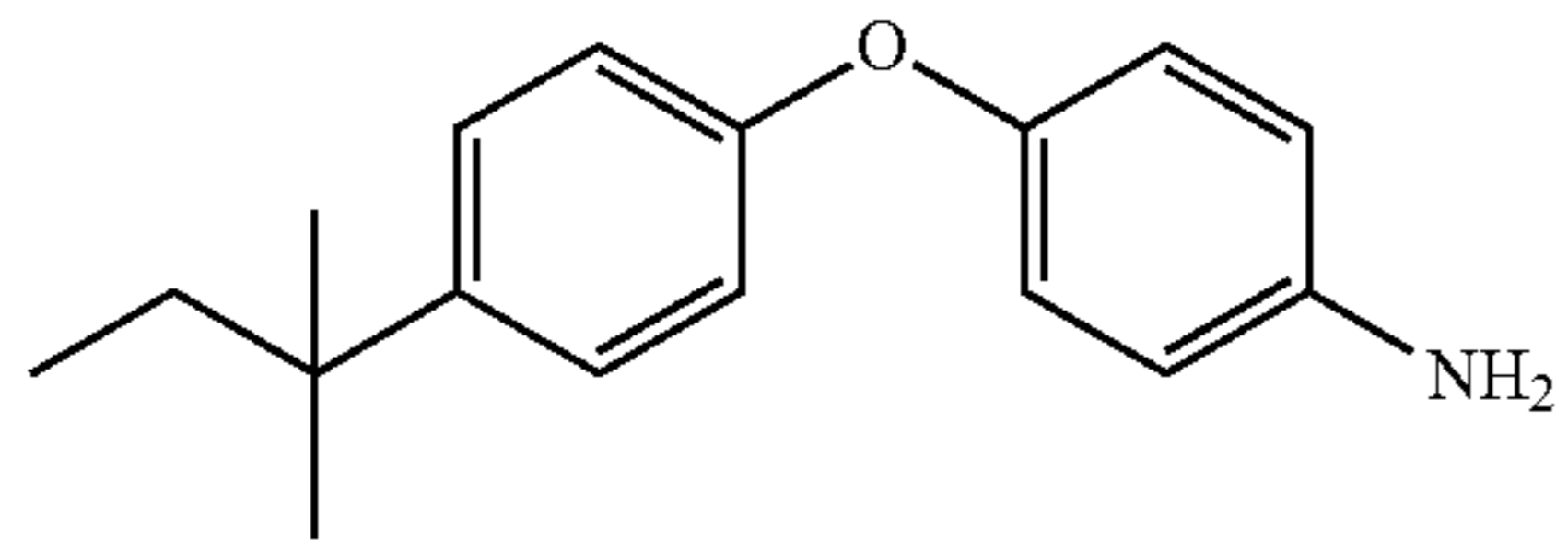
4-(4-(tert-pentyl)phenoxy)aniline
