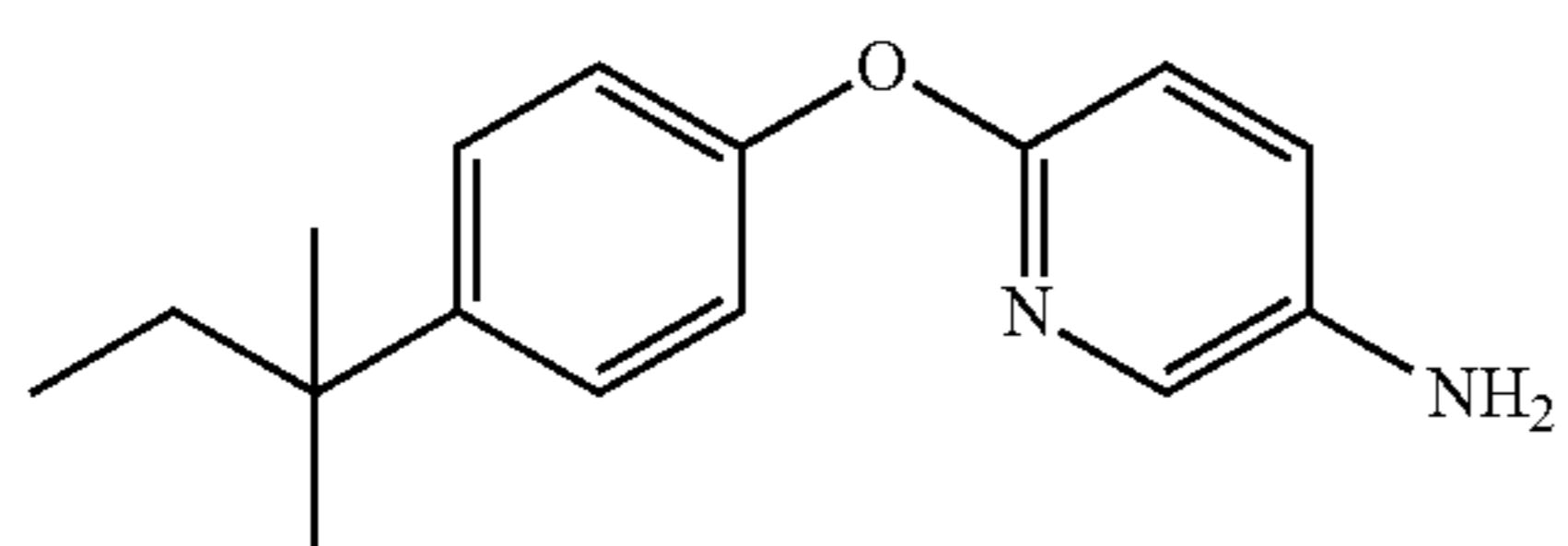
6-(4-(tert-pentyl)phenoxy)pyridin-3-amine
