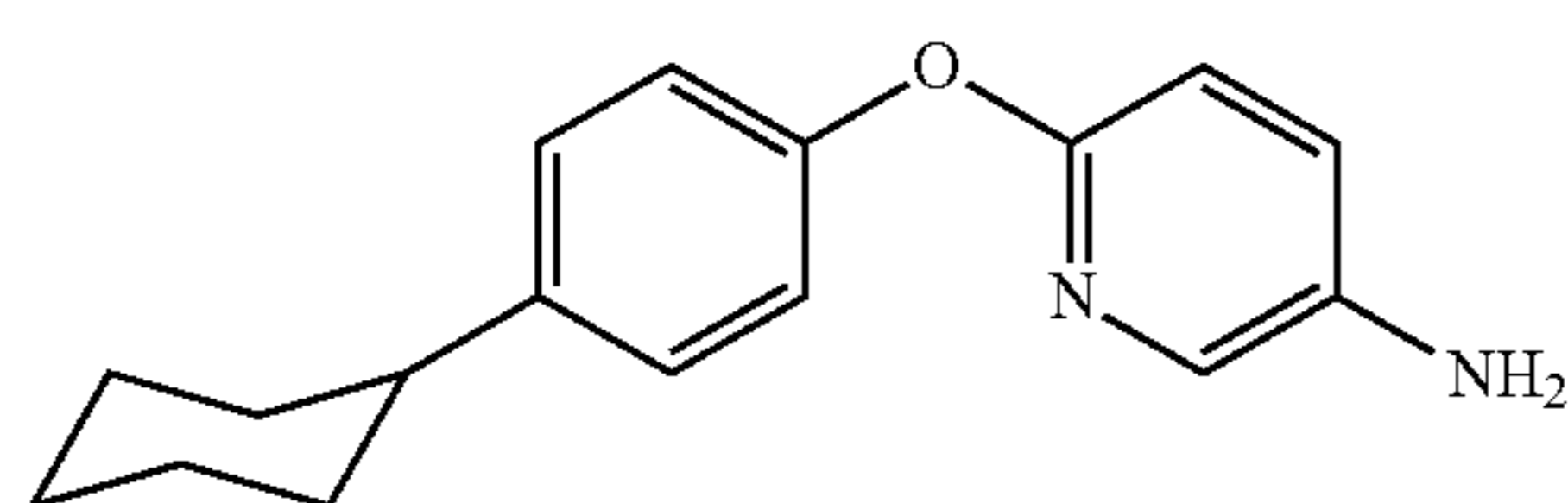
6-(4-cyclohexylphenoxy)pyridin-3-amine
