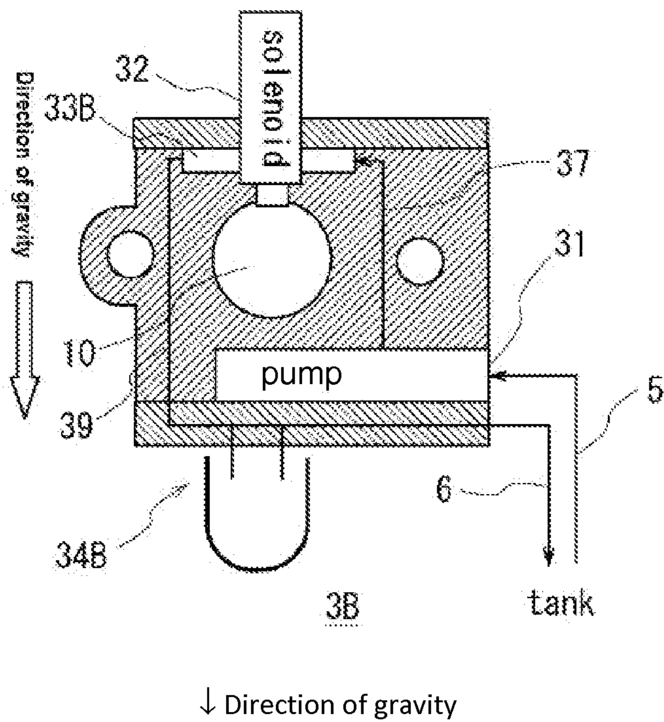
Fig. 3 (Prior Art)
