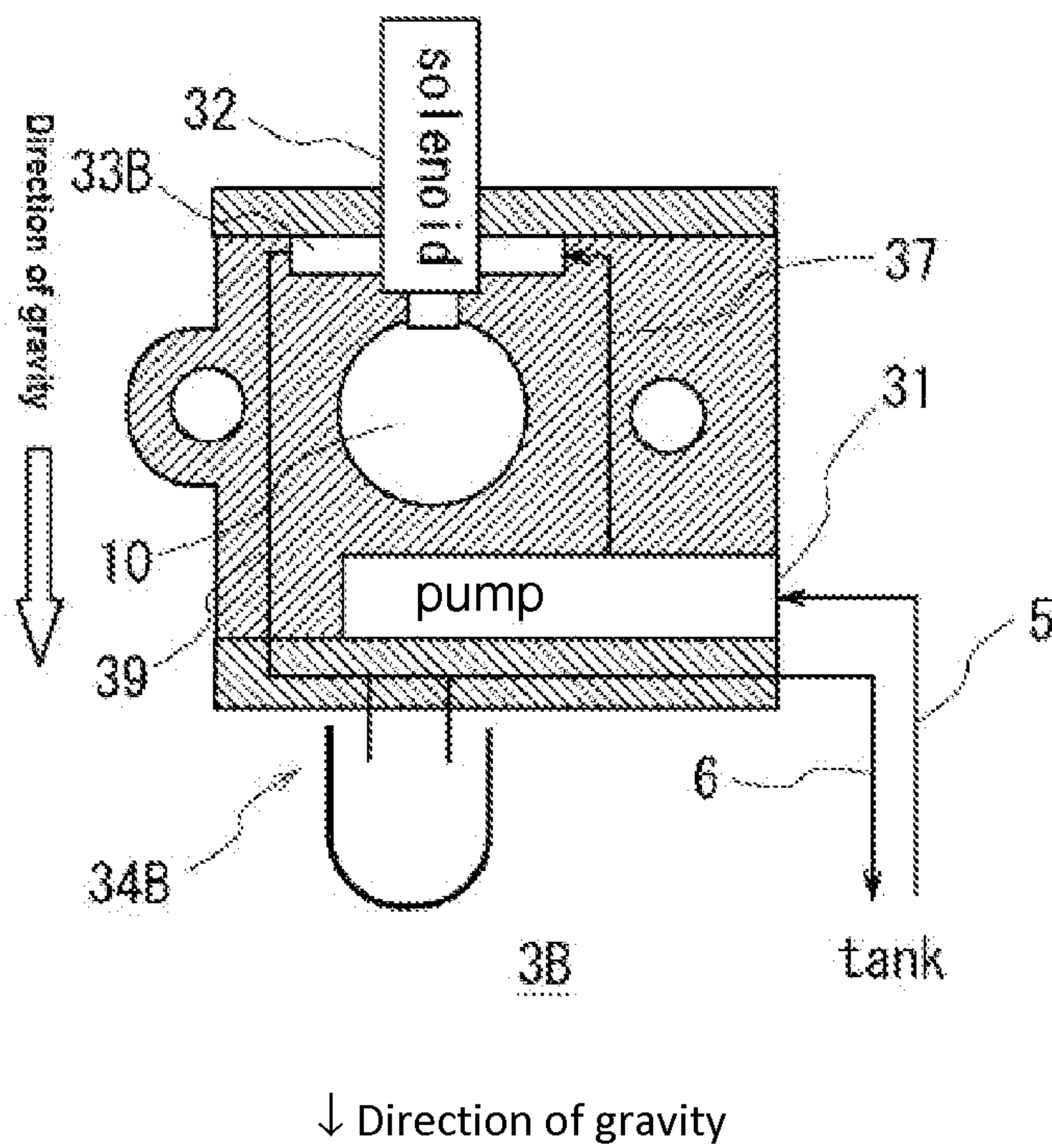
Fig. 3 (Prior Art)
