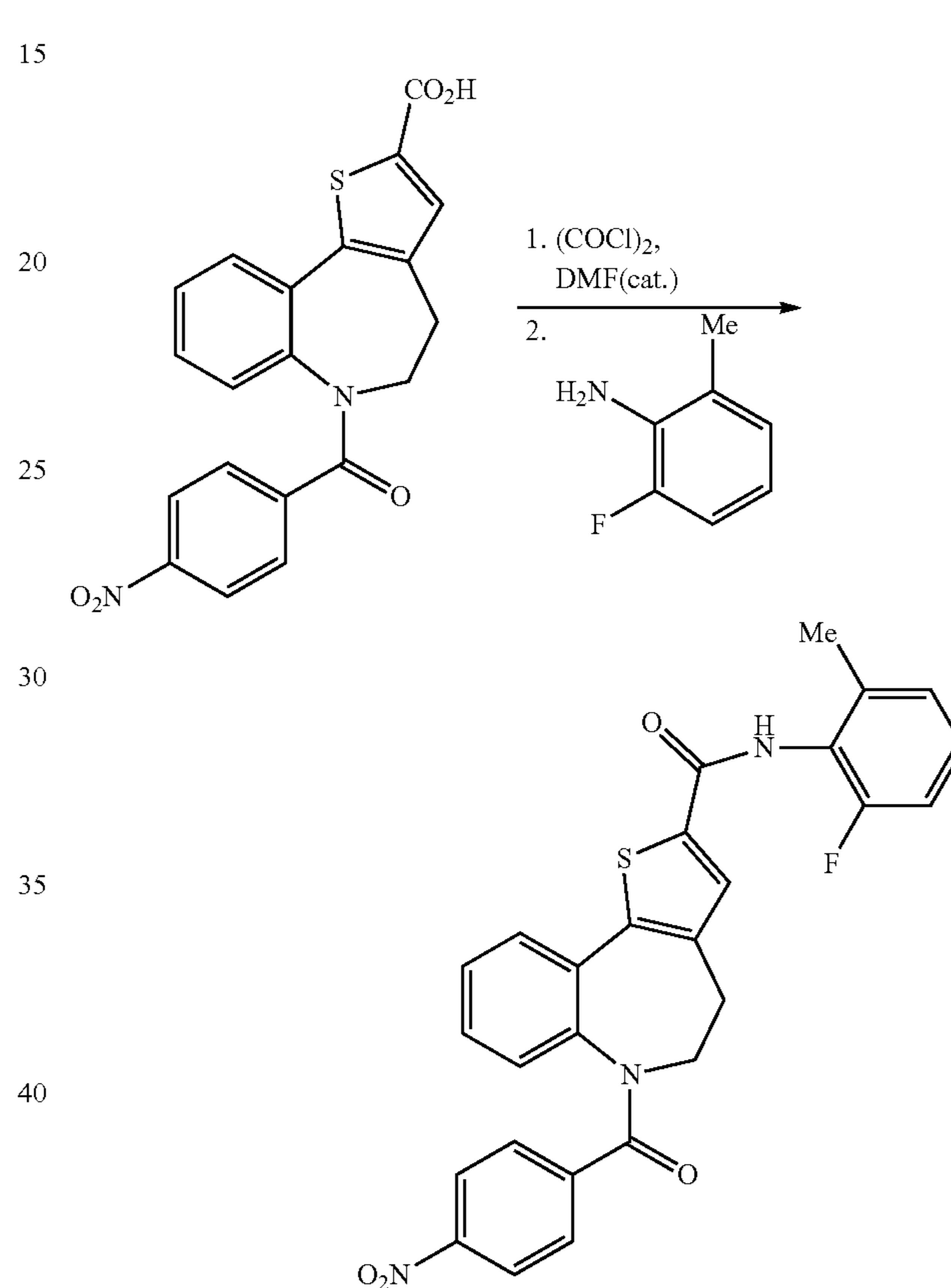
N-(2-Fluoro-6-methylphenyl)-6-(4-nitrobenzoyl)-5,6-dihydro-4H-benzo[b]thieno[2,3-d]azepine-2-carboxamide
