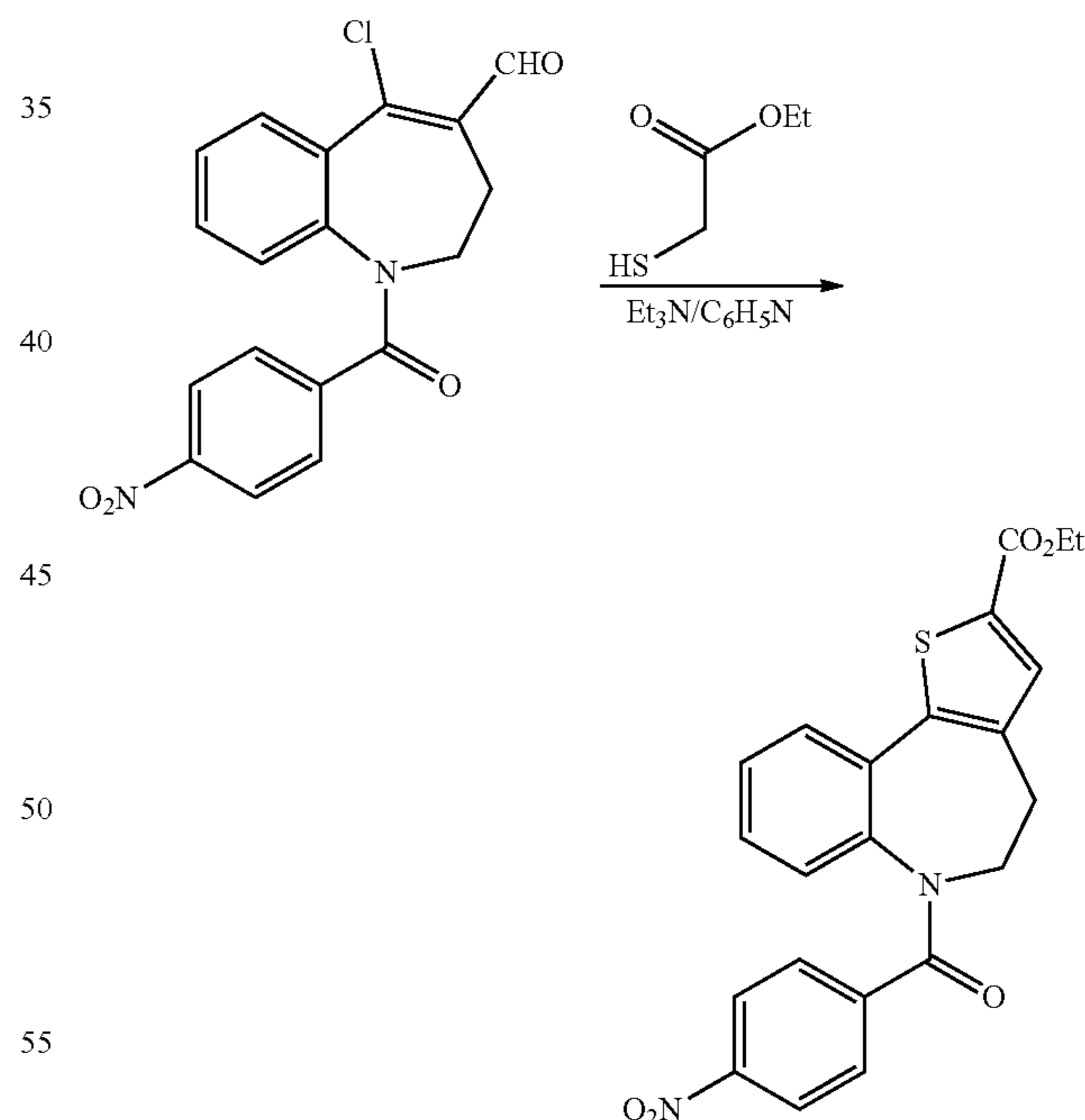
5-Chloro-1-(4-nitrobenzoyl)-2,3-dihydro-1H-benzo[b]azepine-4-carbaldehyde
