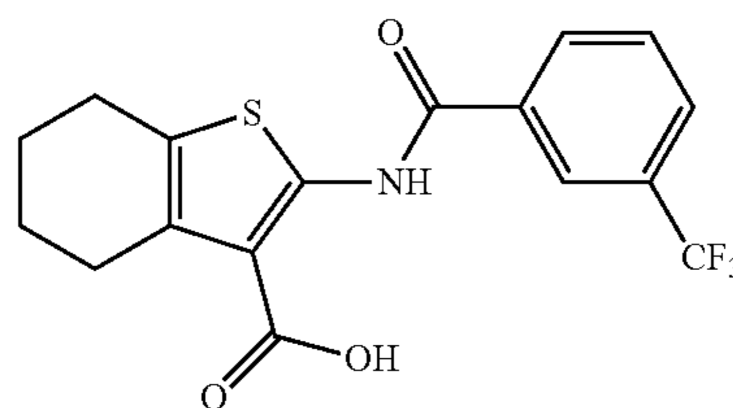
2-(3-(Trifluoromethyl)benzamido)-4,5,6,7-tetrahydrobenzo[b]thiophene-3-carboxylic acid
