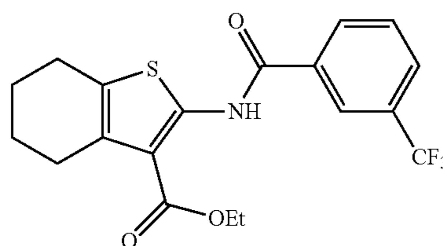
Ethyl 2-(3-(trifluoromethyl)benzamido)-4,5,6,7-tetrahydrobenzo[b]thiophene-3-carboxylate
