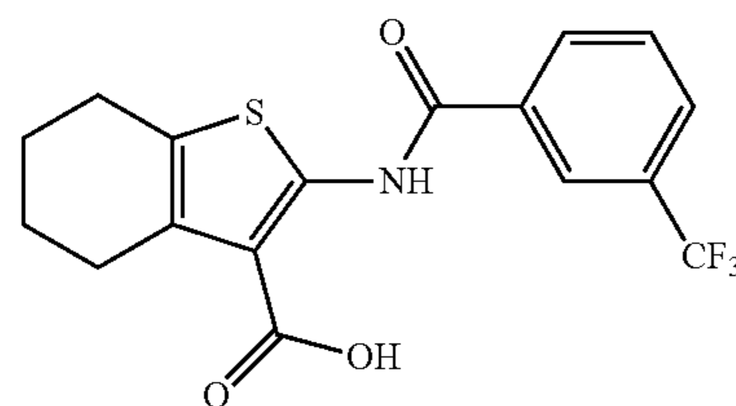
2-(3-(Trifluoromethyl)benzamido)-4,5,6,7-tetrahydrobenzo[b]thiophene-3-carboxylic acid
