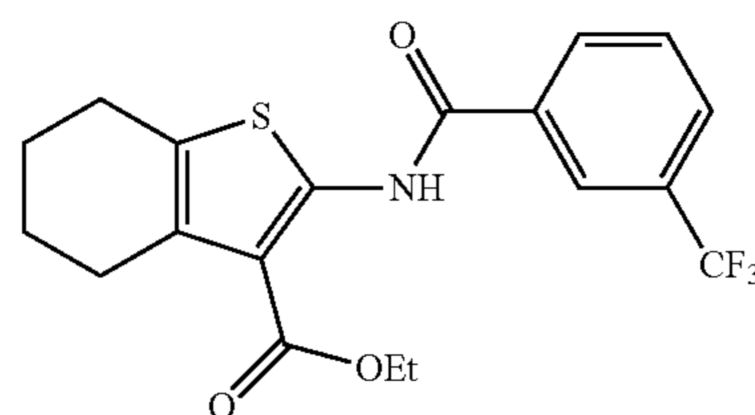
Ethyl 2-(3-(trifluoromethyl)benzamido)-4,5,6,7-tetrahydrobenzo[b]thiophene-3-carboxylate
