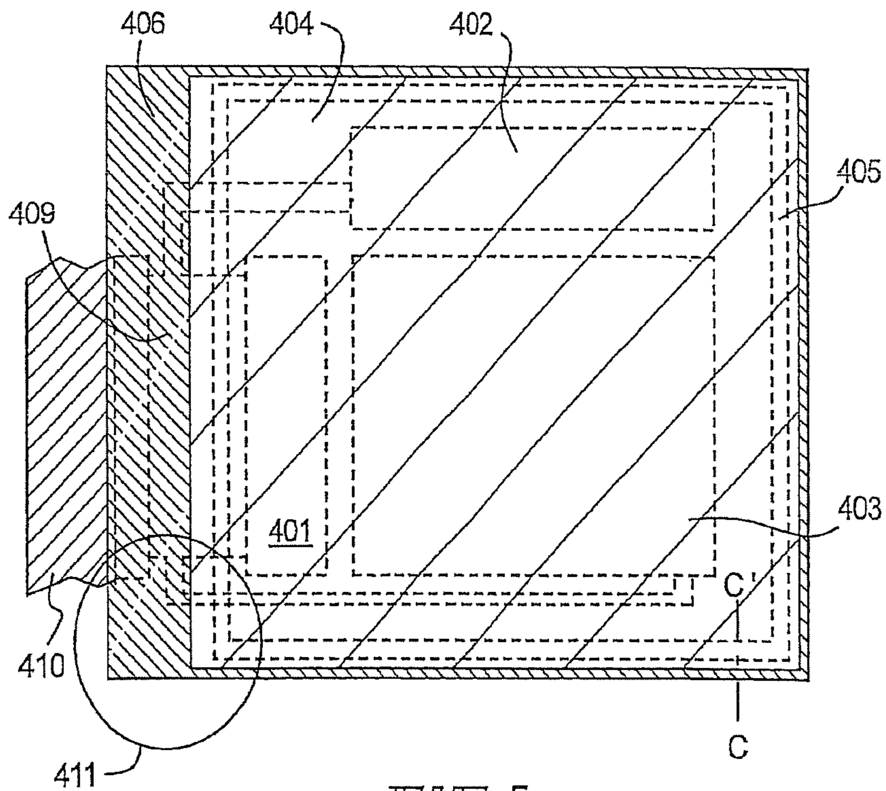
FIG. 5 PRIOR ART
