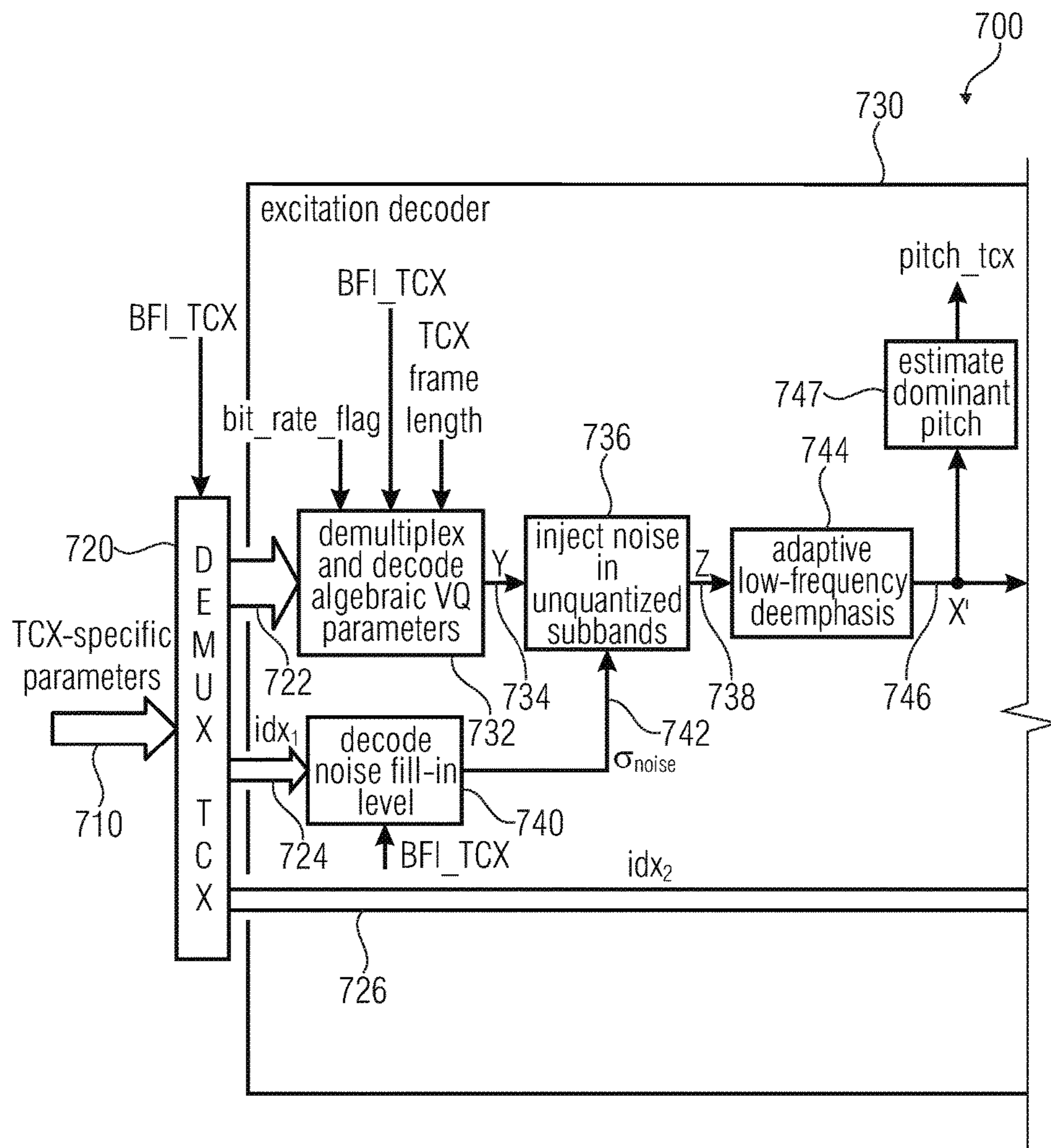
Block diagram of the TCX decoder
