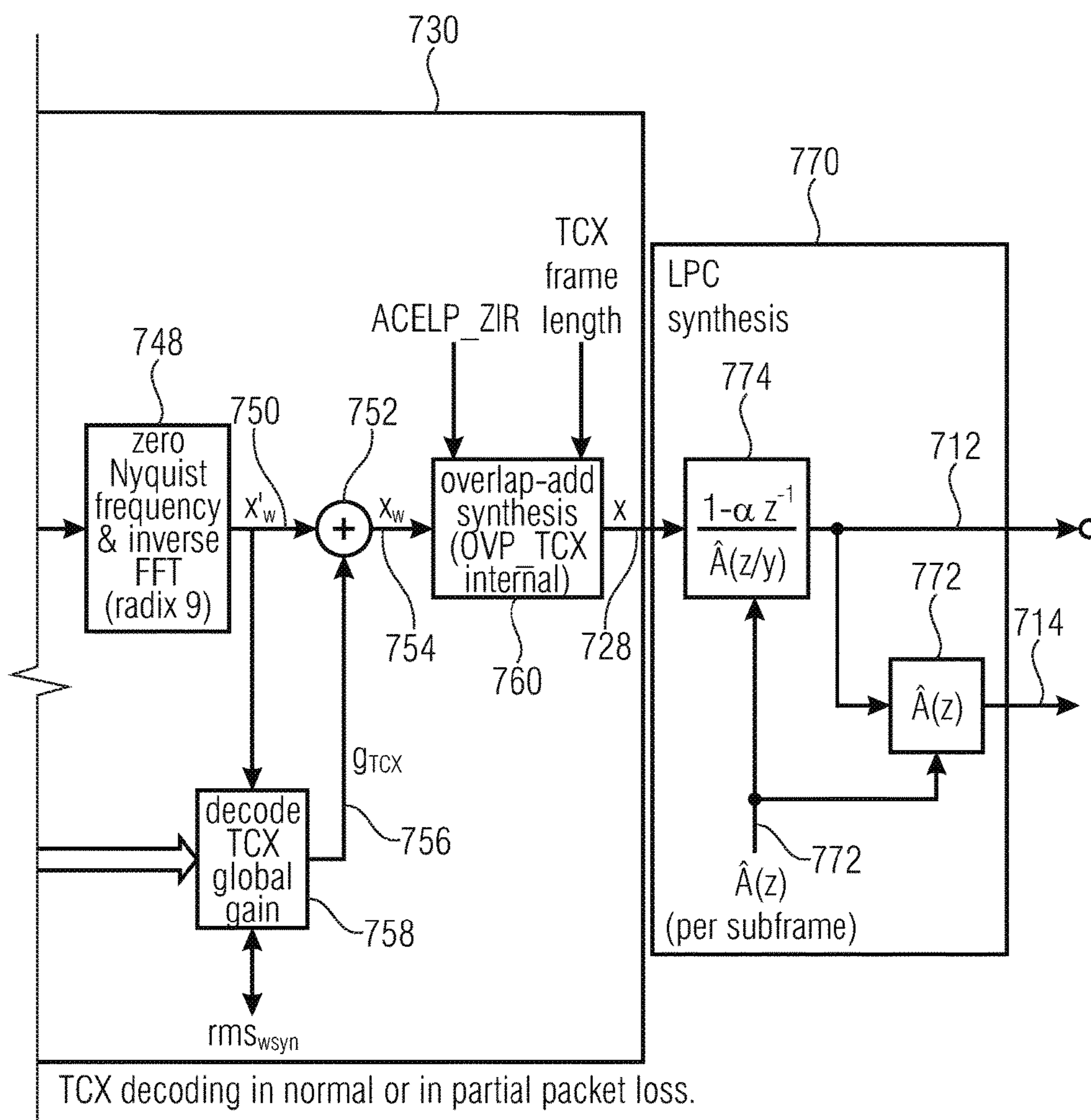
Block diagram of the TCX decoder
