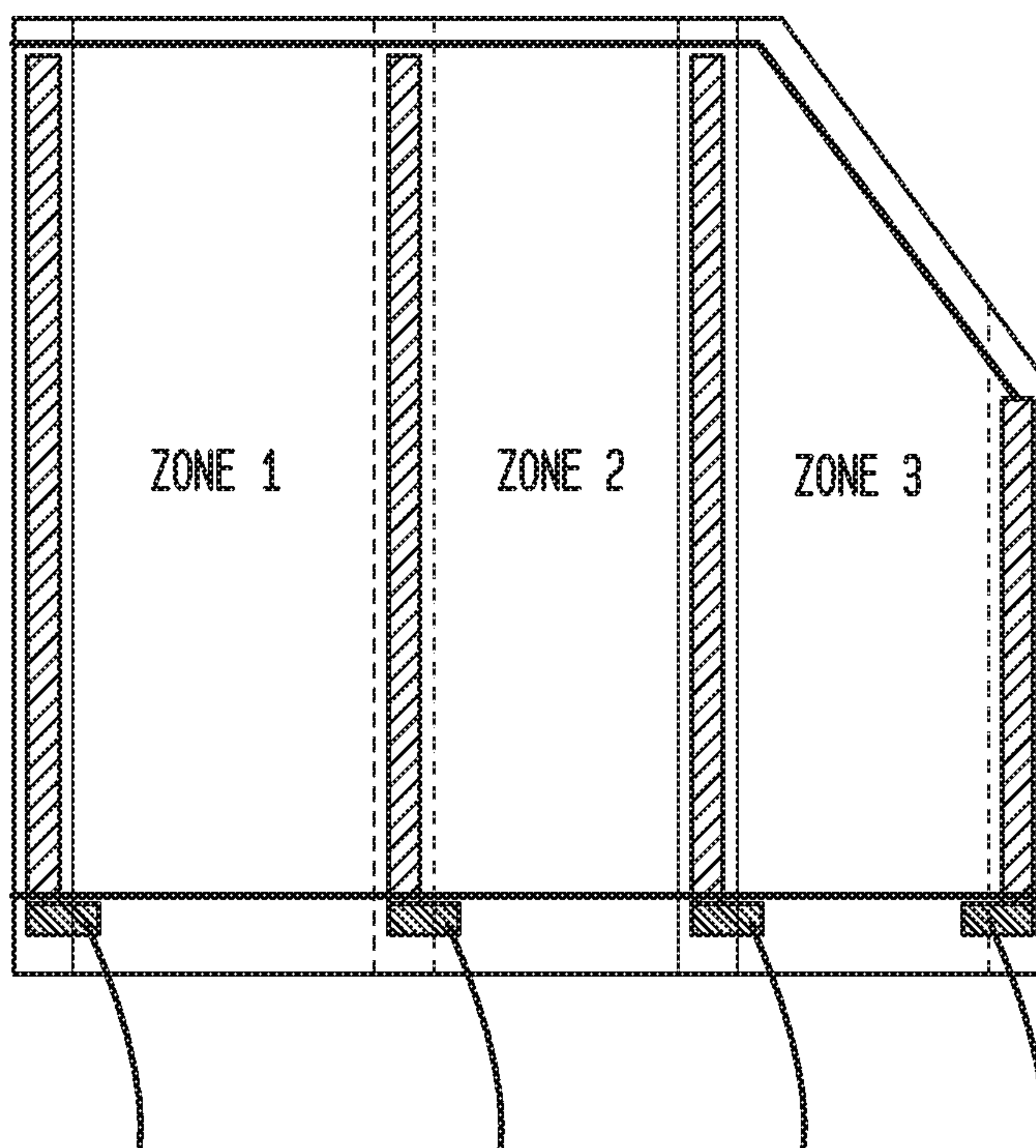
UNEQUAL 3-ZONE, NON-RECTANGULAR 4-BUSBAR DEVICE
